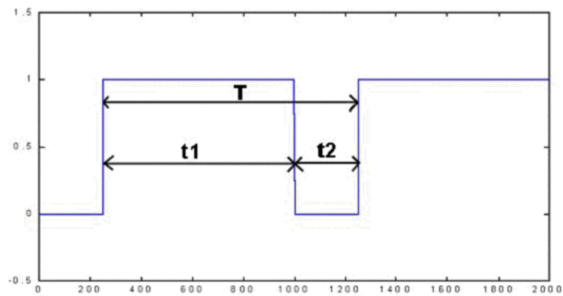
Figure 86-Le signal PWM
