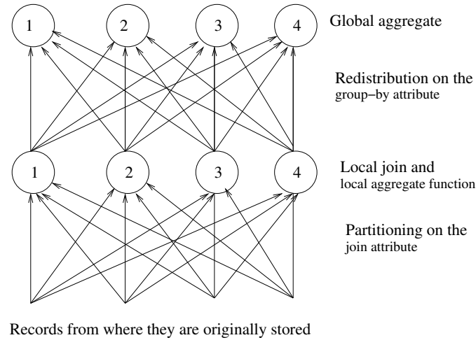
FIG. 3.1 – Join partition method (JPM) (Taniar et al. 2000).
