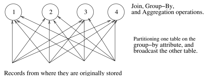
FIG. 3.2 – Aggregation partition method (APM) (Taniar et al. 2000).
