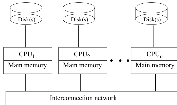
FIG. 2.5 – A Shared-Nothing architecture .
