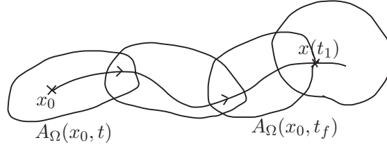
Figure 1.19: x_1 \in \partial A_\Omega(x_0, t_f) .
