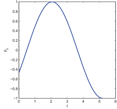
Figure 2.13: p_y for (2.27)–(2.29)
