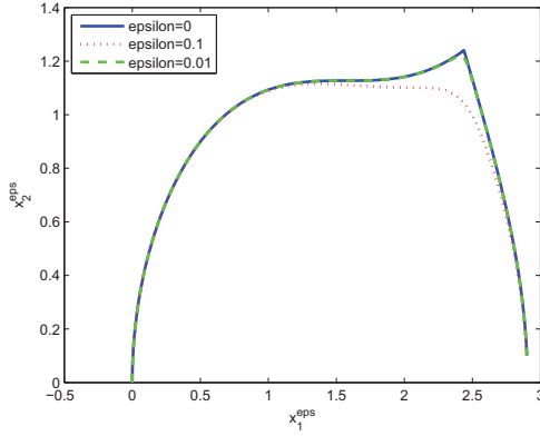
Figure 3.16: Trajectory
