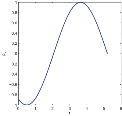
Figure 2.12: p_x for (2.27)–(2.29)
