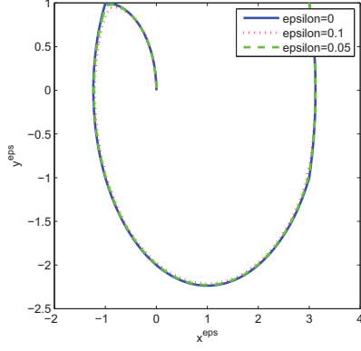
Figure 2.18: (x^\varepsilon, y^\varepsilon)
