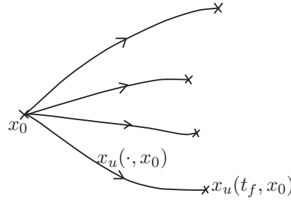
Figure 1.13: End-point mapping.
