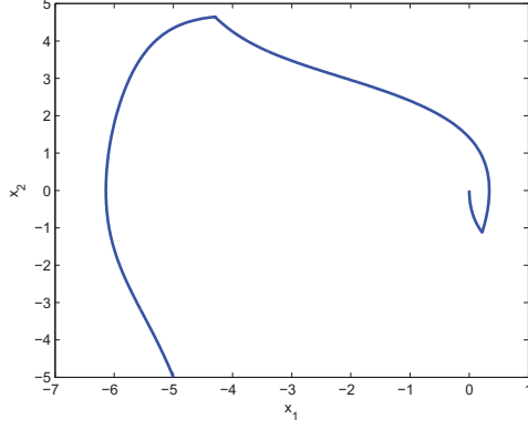
Figure 2.1: Optimal trajectory
