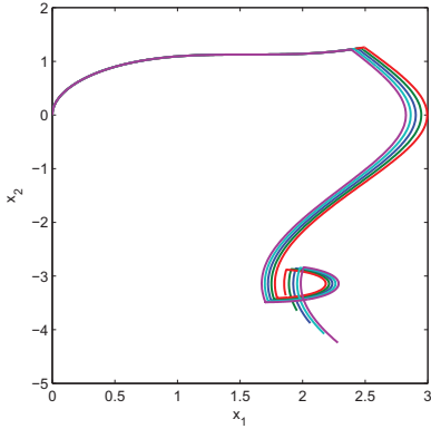
Figure 3.14: Extremal field, t \in [0, 11]
