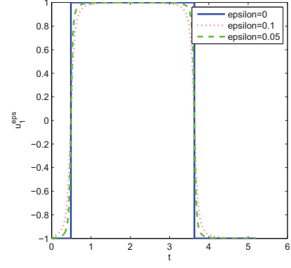
Figure 2.19: u_1^\varepsilon
