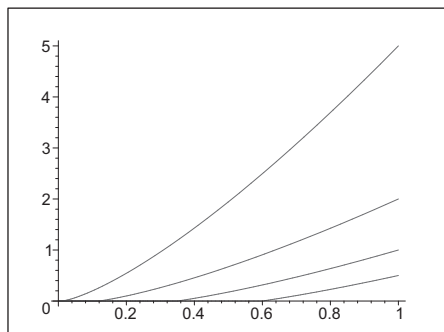
Figure 1.17: Newton's problem solution
