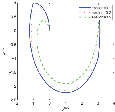
Figure 2.14: (x^\varepsilon, y^\varepsilon)
