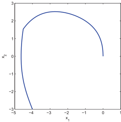
Figure 3.3: Optimal trajectory
