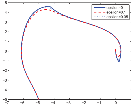
Figure 2.5: Trajectory
