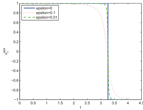
Figure 3.18: Control
