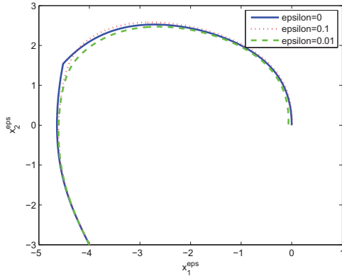
Figure 3.7: Trajectory
