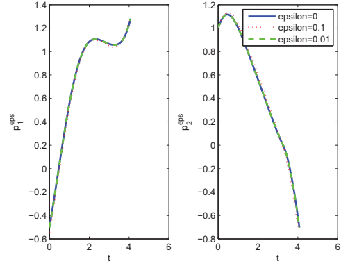
Figure 3.17: Adjoint vector
