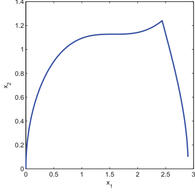
Figure 3.12: Optimal trajectory
