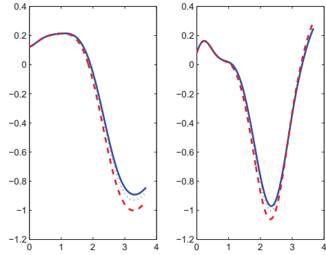
Figure 2.6: Adjoint vector
