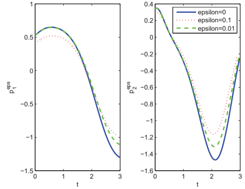
Figure 3.8: Adjoint vector
