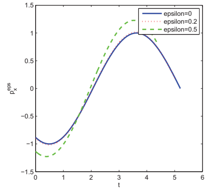
Figure 2.15: p_x^\varepsilon
