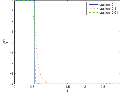
Figure 3.9: Control
