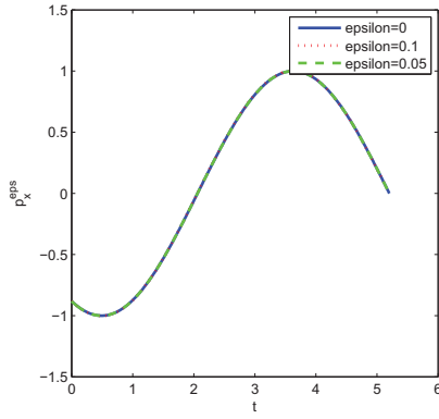
Figure 2.20: p_x^\varepsilon
