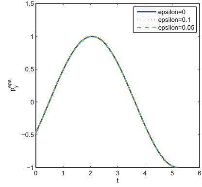
Figure 2.21: p_y^\varepsilon
