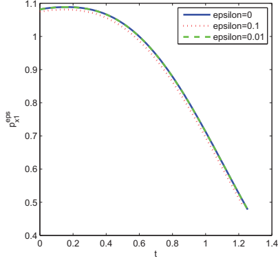
Figure 2.24: Adjoint vector p_{x_1}^\varepsilon
