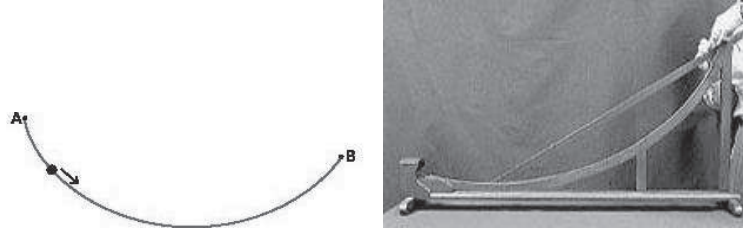
Figure 1.2: Brachistochrone problem.
