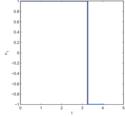
Figure 3.13: Optimal control
