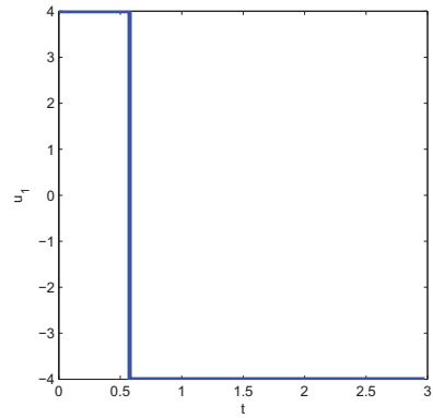
Figure 3.4: Optimal control
