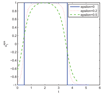
Figure 2.17: u_1^\varepsilon
