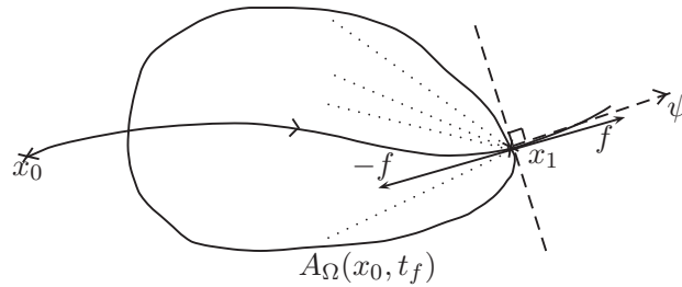
Figure 1.22: \langle \psi, f(x(t_f), u(t_f)) \rangle \geq 0
