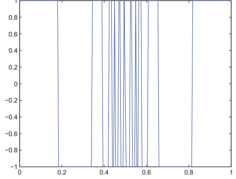
Figure 2.9: Control u_2^\epsilon ( \epsilon = 0.01 )
