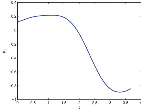
Figure 2.3: Adjoint vector p_1
