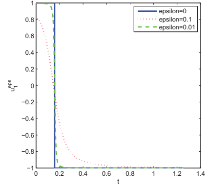
Figure 2.23: Control u_1^\varepsilon(\cdot)
