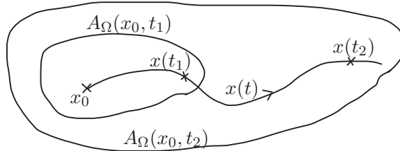
Figure 1.18: Accessible set A_\Omega(x_0, \leq t) .
