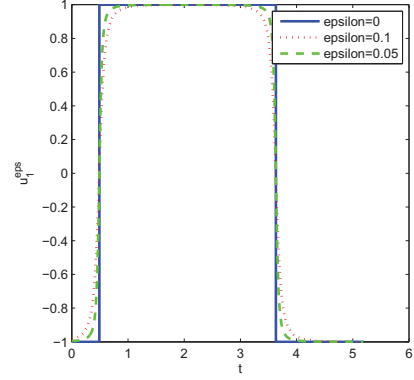
Figure 2.11: Optimal control for (2.27)–(2.29)
