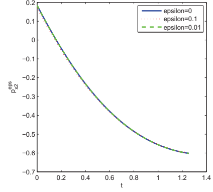
Figure 2.25: Adjoint vector p_{x_2}^\varepsilon
