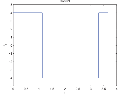
Figure 2.2: Optimal control
