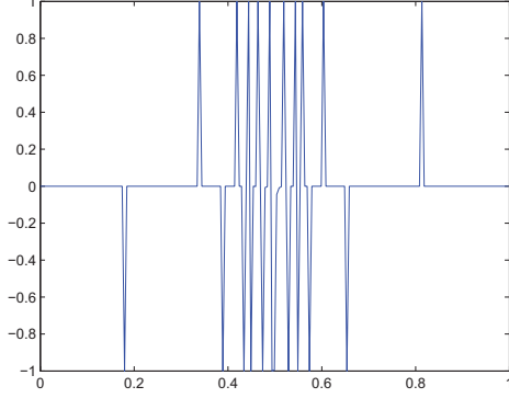
Figure 2.8: Control u_1^\epsilon ( \epsilon = 0.01 )
