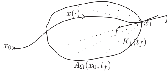
Figure 1.21: Cone K_1(t_f)
