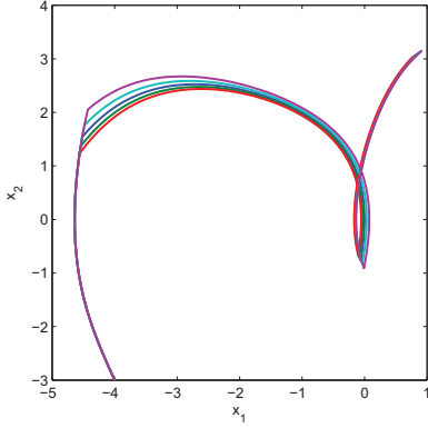
Figure 3.5: Extremal field for t \in [0, 4]
