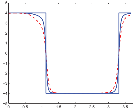
Figure 2.7: Control
