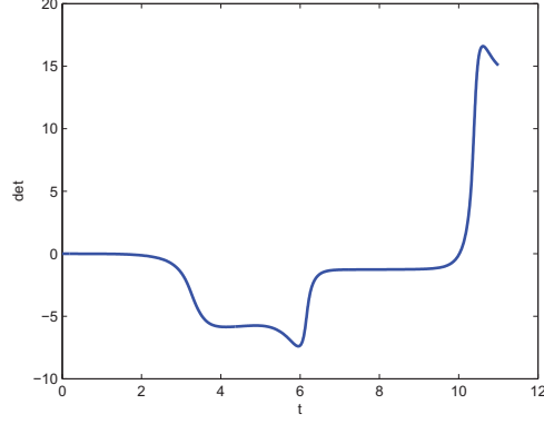
Figure 3.19: \det(\delta x_1^\varepsilon(t), \delta x_2^\varepsilon(t), f_1^\varepsilon(t), f_2^\varepsilon(t)) , \varepsilon = 0.1
