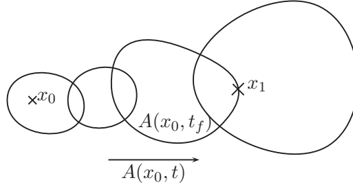
Figure 1.11: Minimal time.
