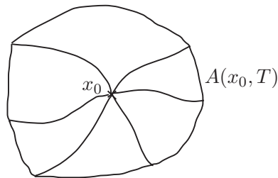
Figure 1.8: Accessible set.
