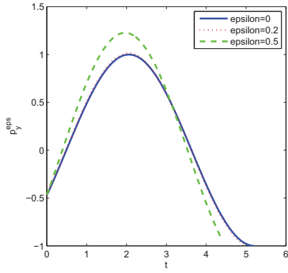
Figure 2.16: p_y^\varepsilon
