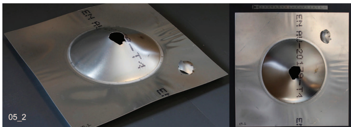
Fig. A2-6. Tested plate 05_2 (0.5 bar)
