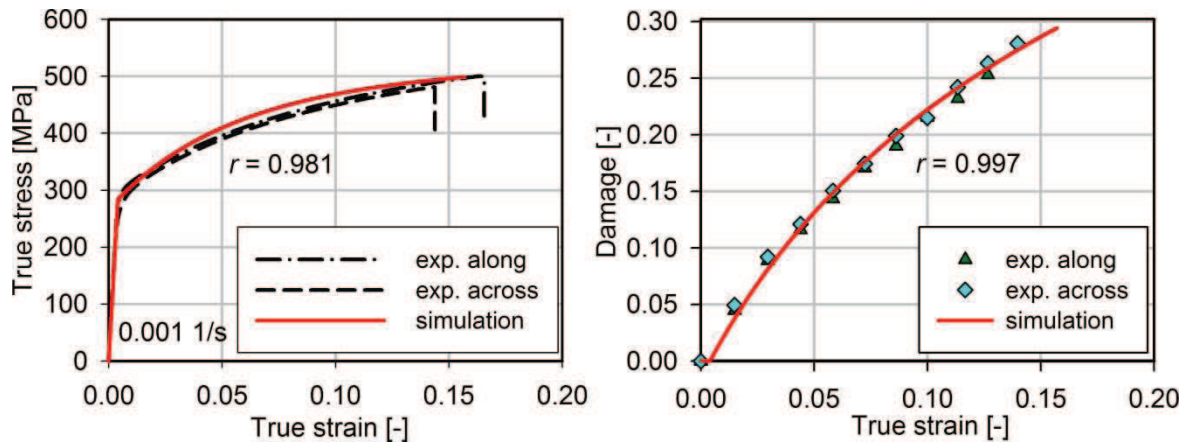
Fig. 5-20. Verification of numerical results, tension test 0.001 1/s
