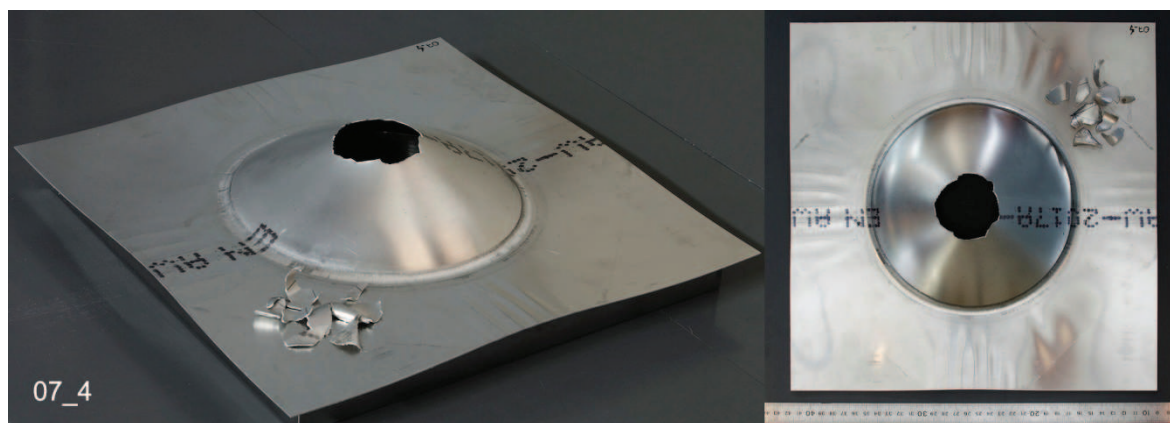
Fig. A2-16. Tested plate 07_4 (0.7 bar)
