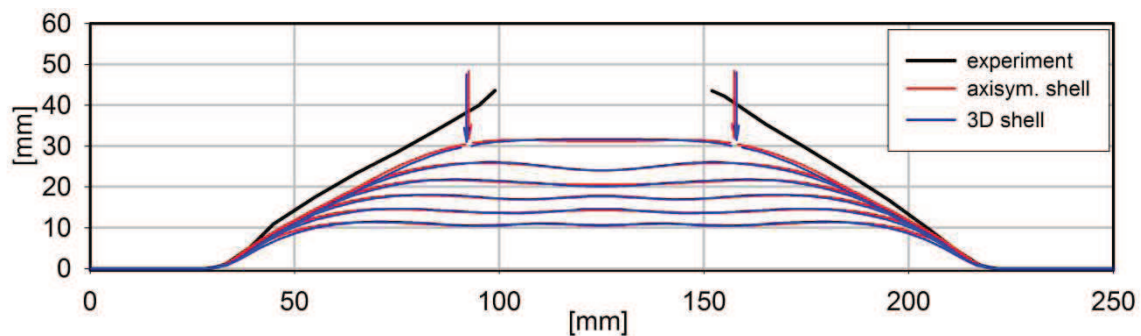
Fig. 8-24. Dynamic analysis – test 07_1, time steps: t_1 = 0.14 ms, t_2 = 0.16 ms, t_3 = 0.18 ms, t_4 = 0.2 ms, t_5 = 0.22 ms, t_6 = 0.24 ms
