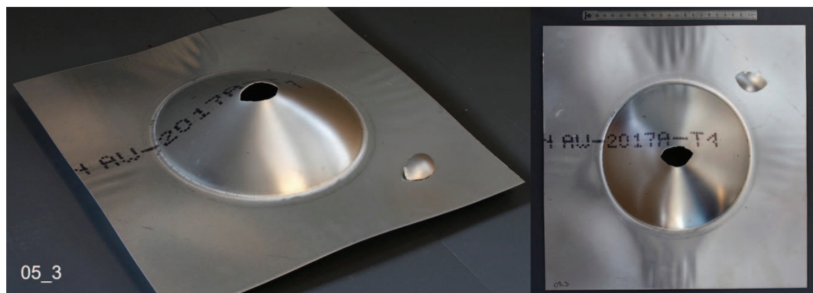
Fig. A2-7. Tested plate 05_3 (0.5 bar)
