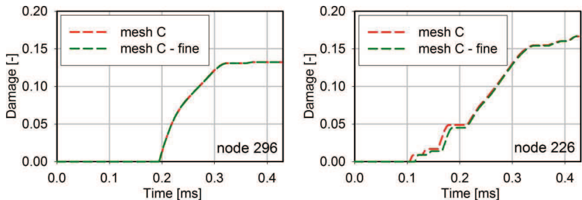
Fig. 8-13. Mesh C dense influence analysis – damage variable
