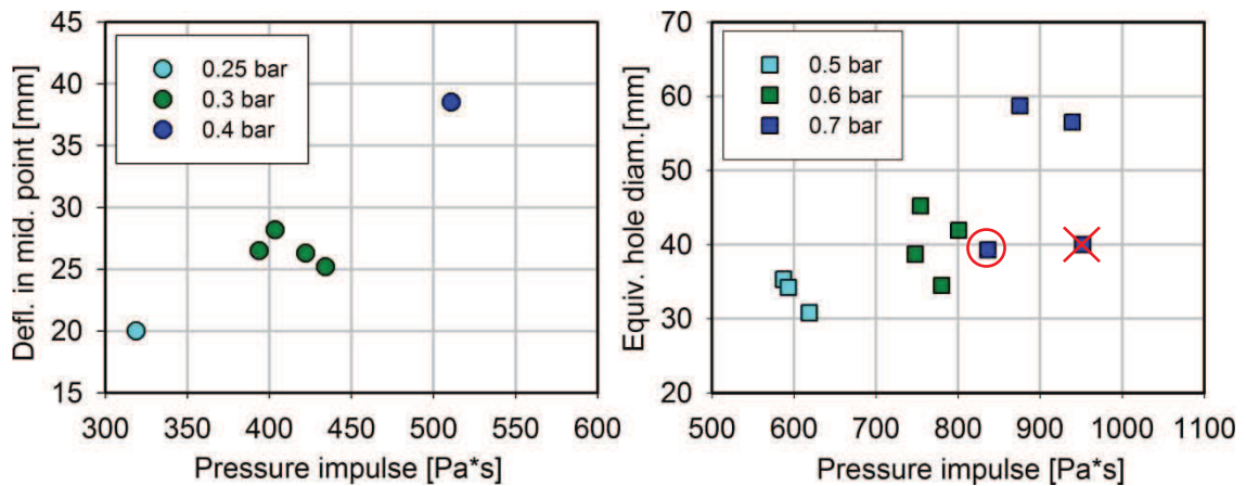
Fig. 4-18. Plates geometry referred to pressure impulses
