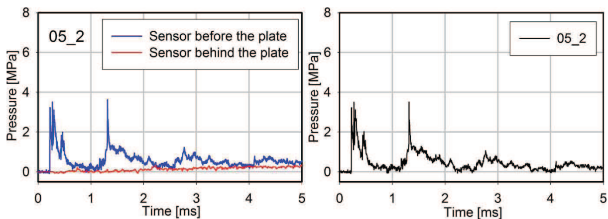
Fig. A1-7. Registered and active pressure time histories, test 05_2 (0.5 bar)
