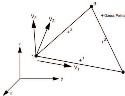
Fig. 3-2. Three-node bilinear thin-triangular shell element [177]
