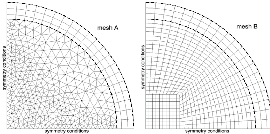
Fig. 8-1. Finite element mesh A and mesh B
