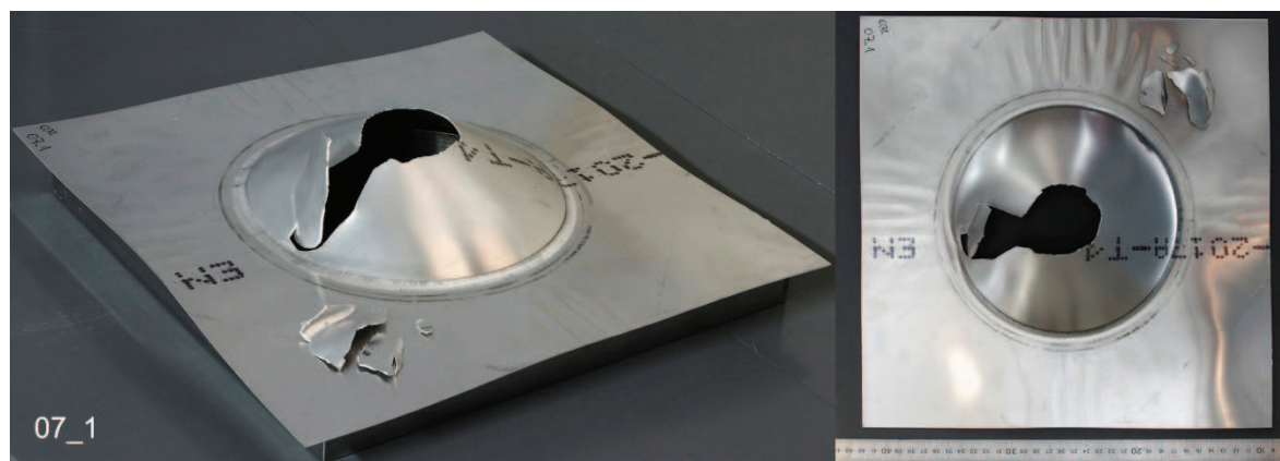
Fig. A2-13. Tested plate 07_1 (0.7 bar)
