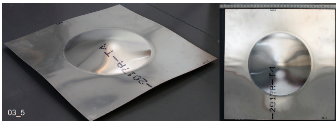
Fig. A2-4. Tested plate 03_5 (0.3 bar)
