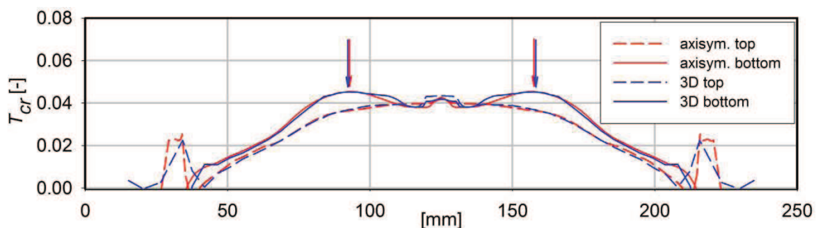
Fig. 8-25. Stress triaxiality dependency criterion parameter in the plate's cross-section in the fracture moment, t = 0.24 ms, uncoupled study, test 07_1
