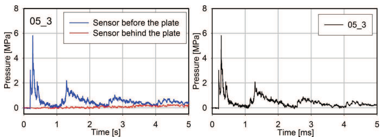
Fig. A1-8. Registered and active pressure time histories, test 05_3 (0.5 bar)
