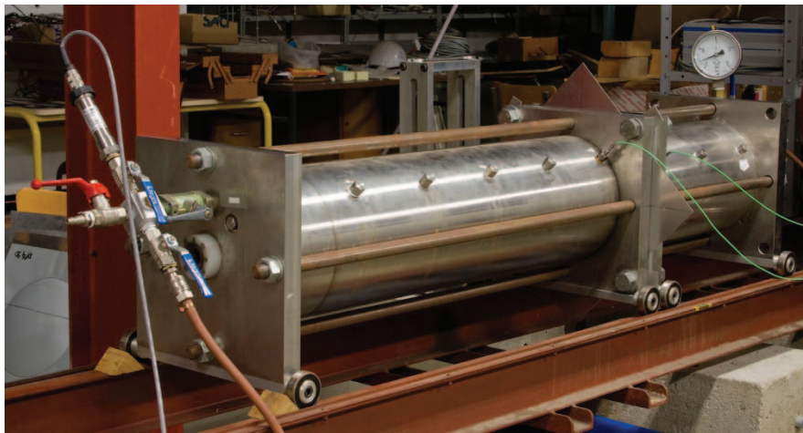
Fig. 4-1. Research stand – the tube used in experiments
