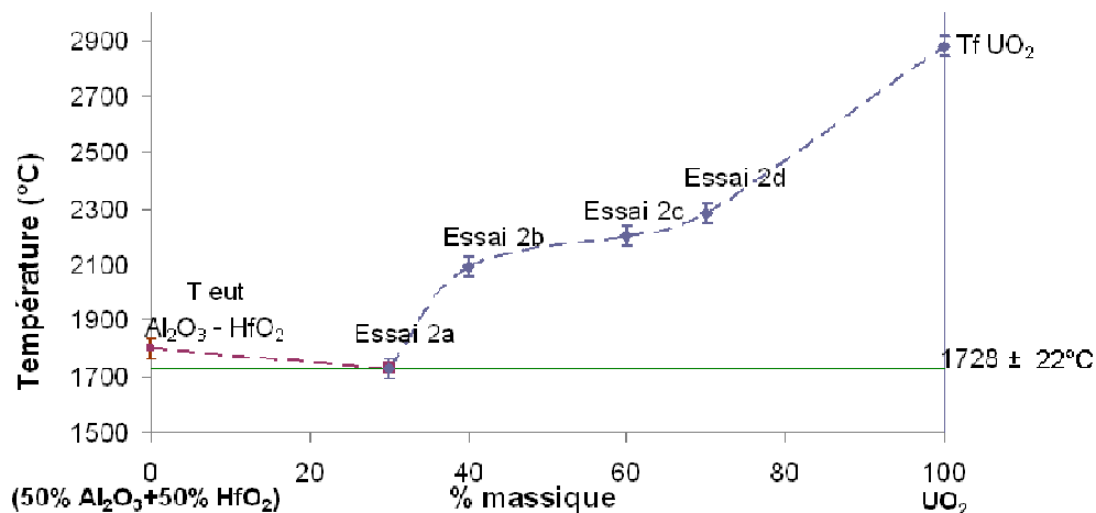
Figure 6-53: Pseudo-binaire \text{UO}_2 - (50\% \text{Al}_2\text{O}_3 + 50\% \text{HfO}_2)
