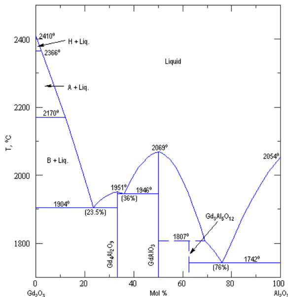
Figure 3-6 : Diagramme de phase \text{Al}_2\text{O}_3 - \text{Gd}_2\text{O}_3 [3.29]
