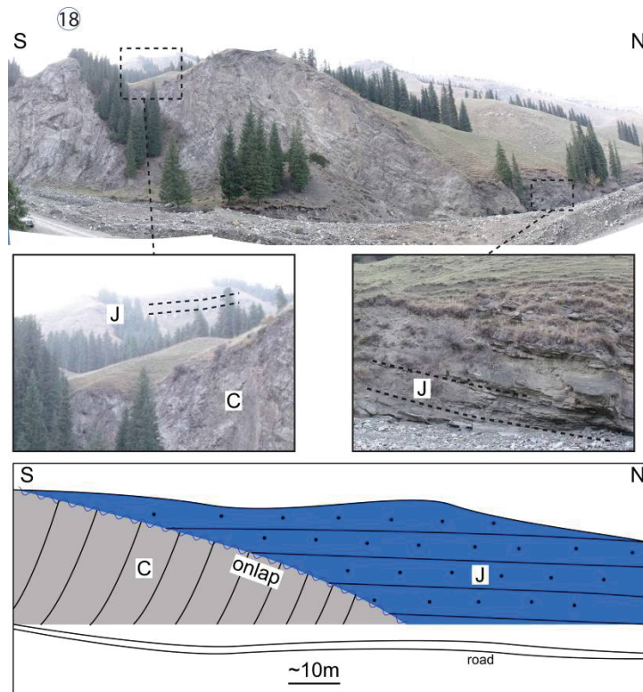
Figure 4-19. The Jurassic series onlaps the Carboniferous basement without visible Cenozoic deformation. See Figure 4-1, N°18 for the location.
