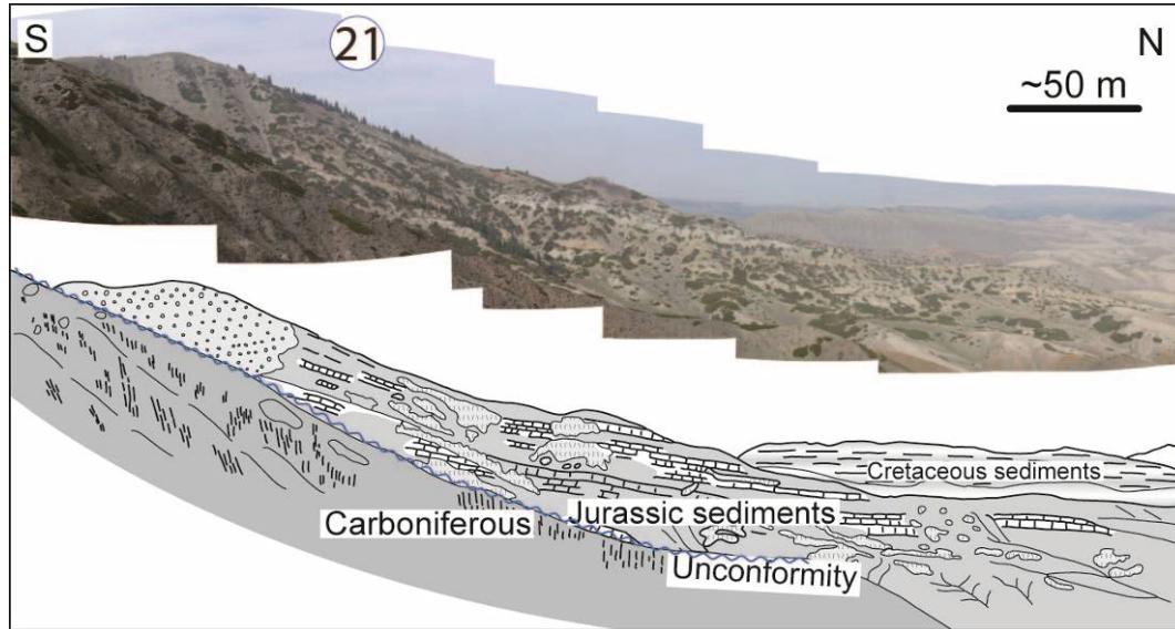
Figure 4-23. Jurassic series overlie on the Paleozoic basement with a monocline towards north at the southern end of Wusu area.
