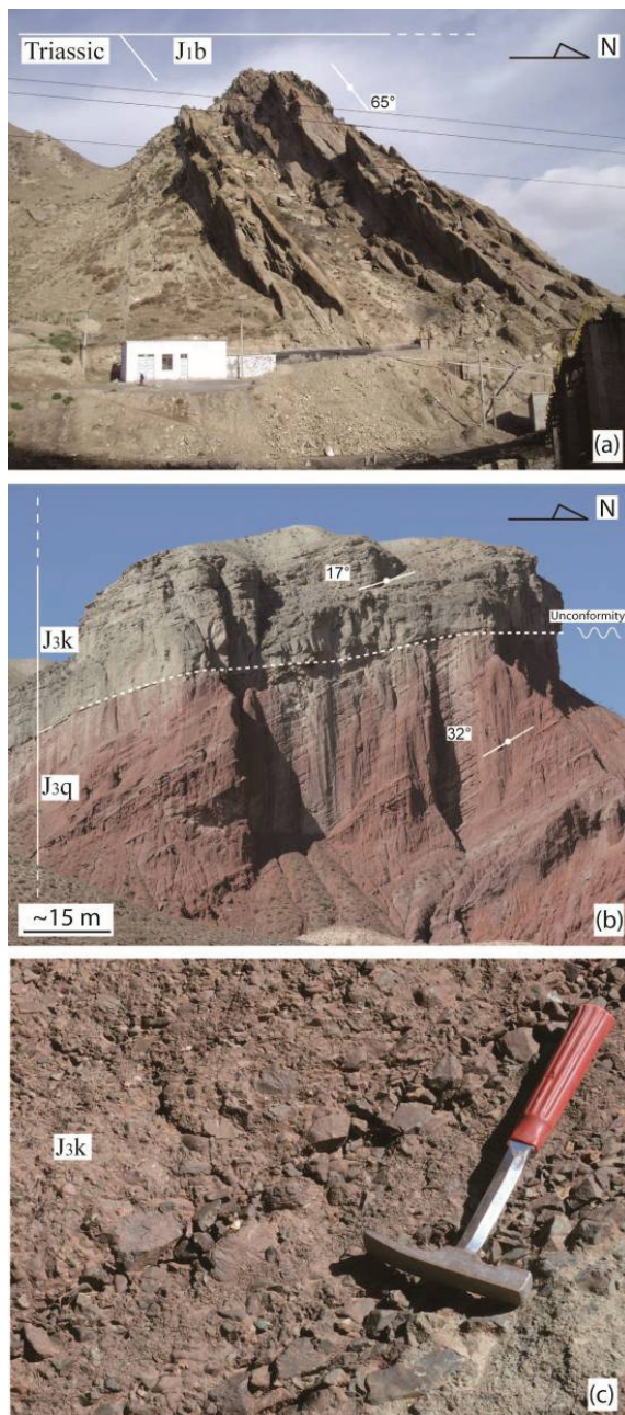
Figure 3-3. Landscape pictures of representative features of the Mesozoic series (see position in the Fig.1) (a) Coarse-grained conglomerate bars in the lowermost Jurassic (southern Qingshui He area); (b) Uppermost Jurassic breccias (J3k) unconformably overlie the Upper Jurassic Qigu formation (Hutubi He area); (c) Detailed view of the Uppermost Jurassic breccias (west to Hutubi He area).
