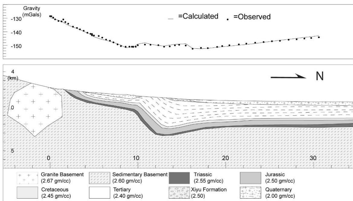
Figure 5-15. Modeling of Bouguer anomalies along the Wusu section. In the upper panel, natural gravity data has been fitted to Bouguer anomaly data using densities indicated in the figure legend to construct structural section.
