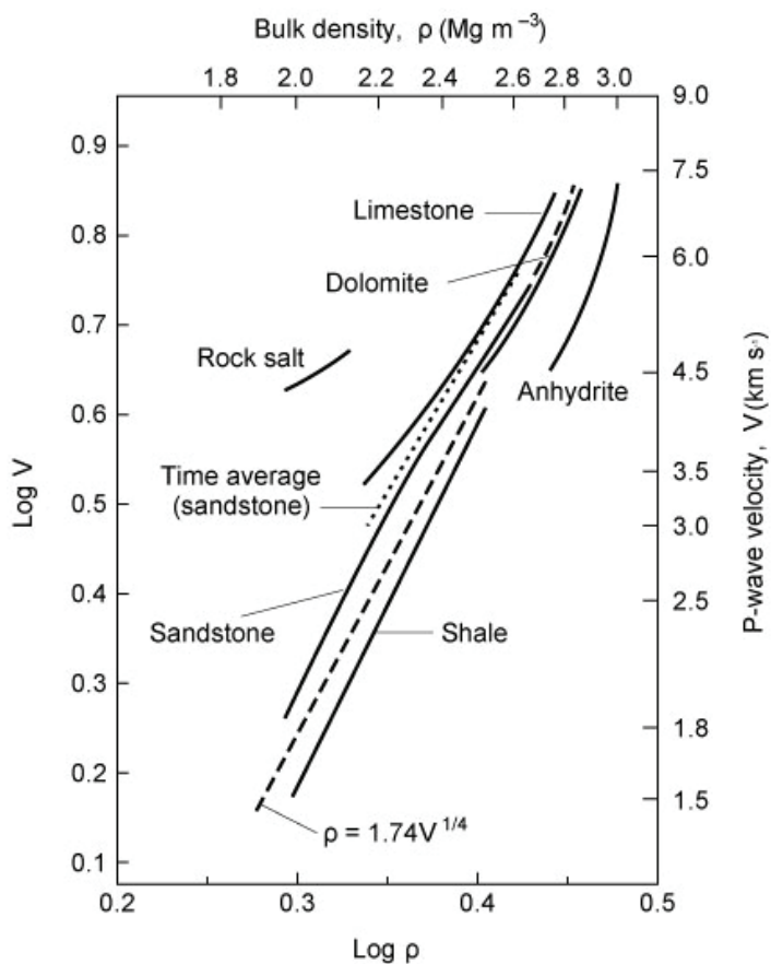
Figure A-11. Logarithm of P-wave velocity against density for various rock types, show the best-fitting linear relationship between density and log velocity (after Gardner et al., 1974).
