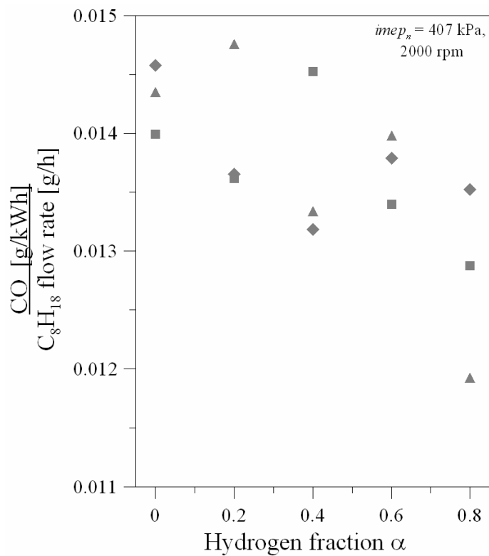
Figure 10.b Normalized CO emissions versus \alpha ( imep_n = 407 kPa, N = 2000 rpm, \phi < 1 ): \blacklozenge CASE A P_{in} = 70 kPa, \beta = 0 ; \blacksquare CASE A P_{in} = 70 kPa, \beta = 0.1 ; \blacktriangle CASE A P_{in} = 70 kPa, \beta = 0.2 .
