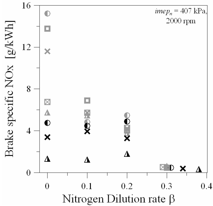
Figure 6.b Brake specific NO x versus nitrogen mole fraction used for the dilution \beta ( imep_n = 407 kPa, N = 2000 rpm): \boxtimes \alpha = 0 CASE A and B; \square \alpha = 0.2 CASE A and B; \circ \alpha = 0.4 CASE A and B; \bullet \alpha = 0.4 CASE C and D; \times \alpha = 0.6 CASE A and B; \times \alpha = 0.6 CASE C and D; \triangle \alpha = 0.8 CASE A and B; \blacktriangle \alpha = 0.8 CASE C and D.
