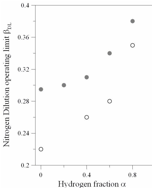
Figure 1.b Evolution of the nitrogen dilution operating limit \beta_{DL}
