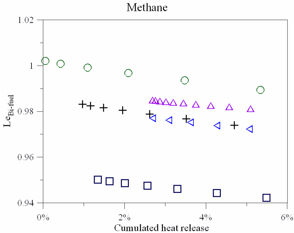
Figure 9. Le_{Bi-fuel} versus the percentage of cumulated heat release for mixtures with methane (conditions 1-5): 1: \blacktriangleleft CH_4/Air ; 2: \blacktriangle CH_4/air/20\%N_2 ; 3: \bigcirc CH_4/40\%H_2/Air ; 4: \blacktriangleleft CH_4/40\%H_2/20\%N_2/Air ; 5: \square CH_4/60\%H_2/20\%N_2/Air .
