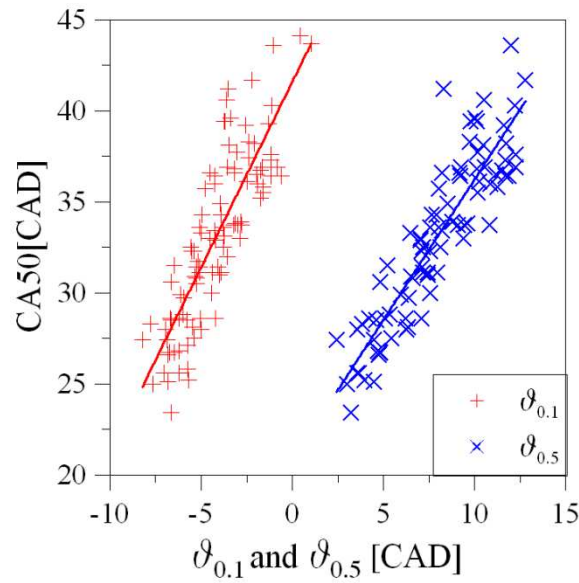
Figure 3. \theta_{0.1} and \theta_{0.5} versus the CA50 (condition 17).
