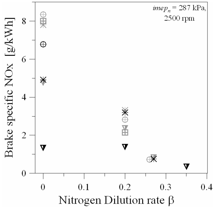
Figure 6.a Brake specific NO x versus nitrogen mole fraction used for the dilution \beta ( imep_n = 287 kPa, N = 2500 rpm): \square \alpha = 0 CASE A and B; \oplus \alpha = 0.4 CASE A and B; \oplus \alpha = 0.4 CASE C and D; * \alpha = 0.6 CASE A and B; * \alpha = 0.6 CASE C and D; \nabla \alpha = 0.8 CASE A and B; \nabla \alpha = 0.8 CASE C and D.
