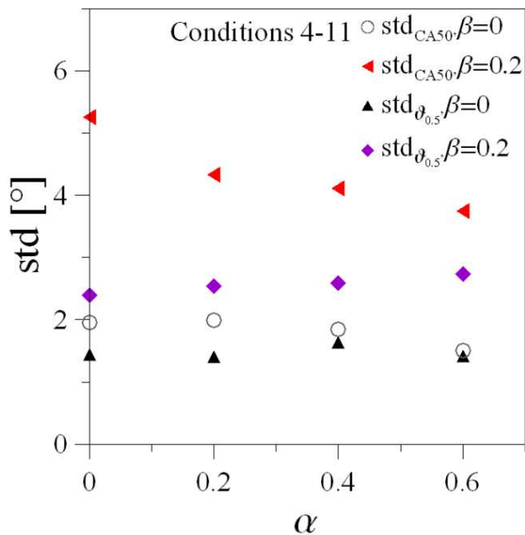
Figure 10.a std_{\theta_{0.5}} and std_{CA50} as a function of \alpha (conditions 4-11).
