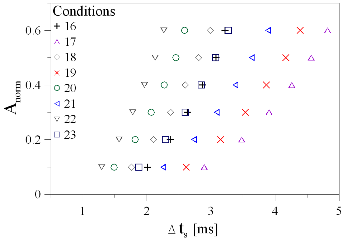
Figure 7.a Temporal evolution of A_{\text{norm}} (conditions 16-23).
