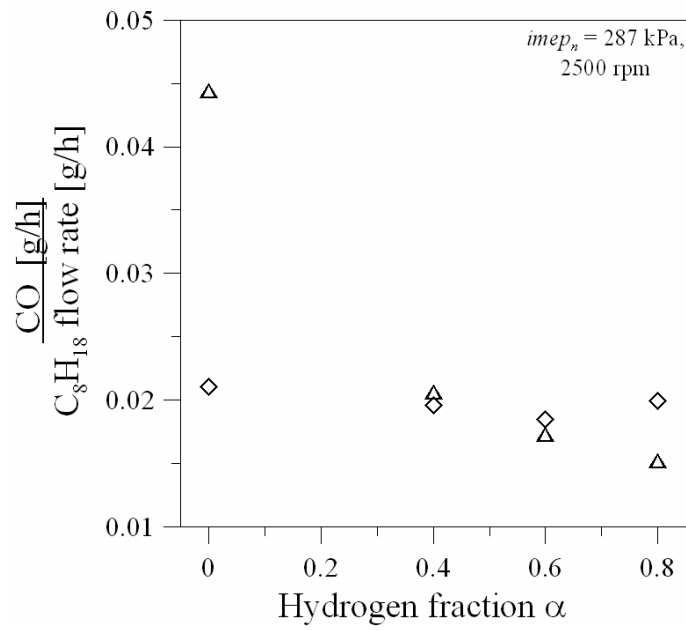
Figure 10.a Normalized CO emissions versus \alpha ( imep_n = 287 kPa, N = 2500 rpm, \phi < 1 ): \diamond CASE A P_{in} = 55 kPa, \beta = 0 ; \triangle CASE A P_{in} = 55 kPa, \beta = 0.2 .
