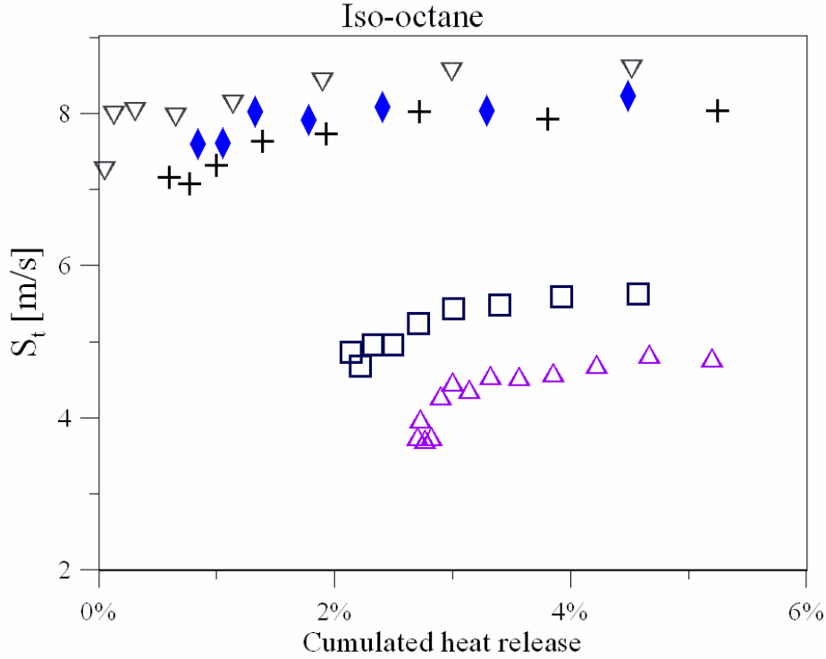
Figure 16. S_t versus the percentage of cumulated heat release
