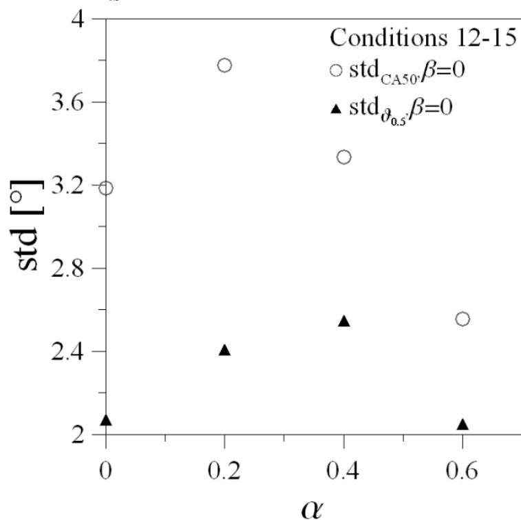
Figure 10.b std_{\theta_{0.5}} and std_{CA50} as a function of \alpha (conditions 12-15).
