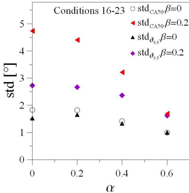
Figure 10.c \text{std}_{\theta_{0.5}} and \text{std}_{\text{CA50}} as a function of \alpha (conditions 16-23).
