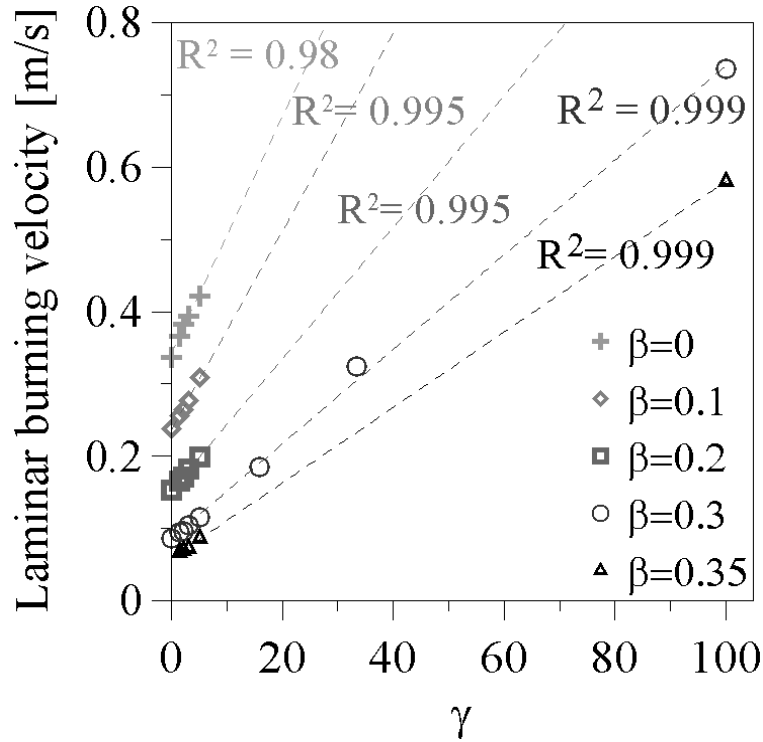
Figure 8. Experimental laminar burning velocity versus hydrogen mass fraction, \gamma ( P=0.1 MPa, T=300 K).
