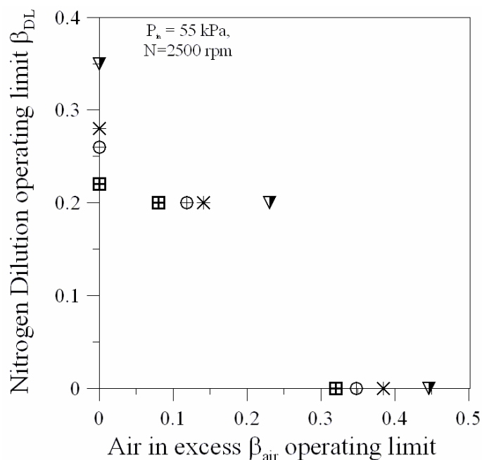
Figure 2.a Evolution of the nitrogen dilution operating limit \beta_{DL}
