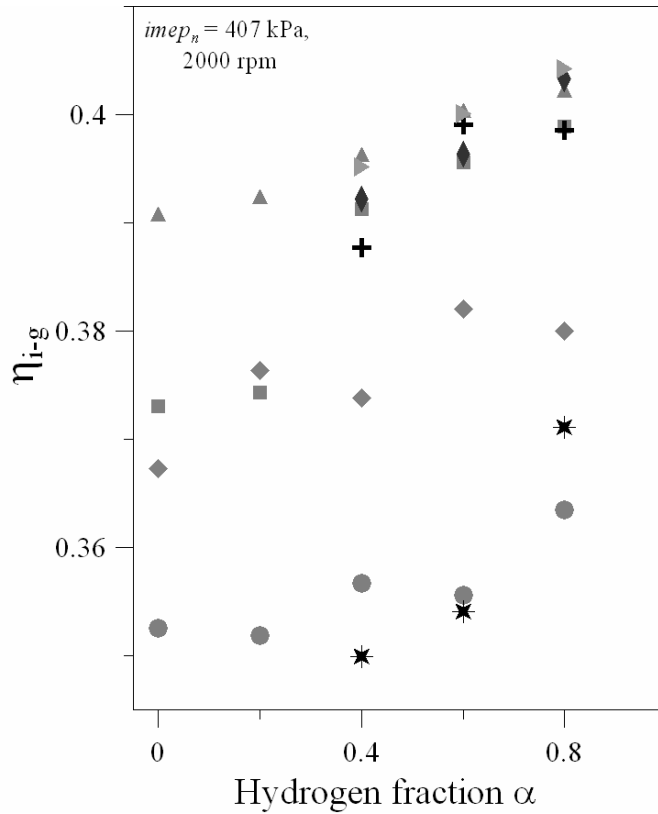
Figure 15.b \eta_{i-g} versus \alpha ( imep_n = 407 kPa, N = 2000 rpm):
