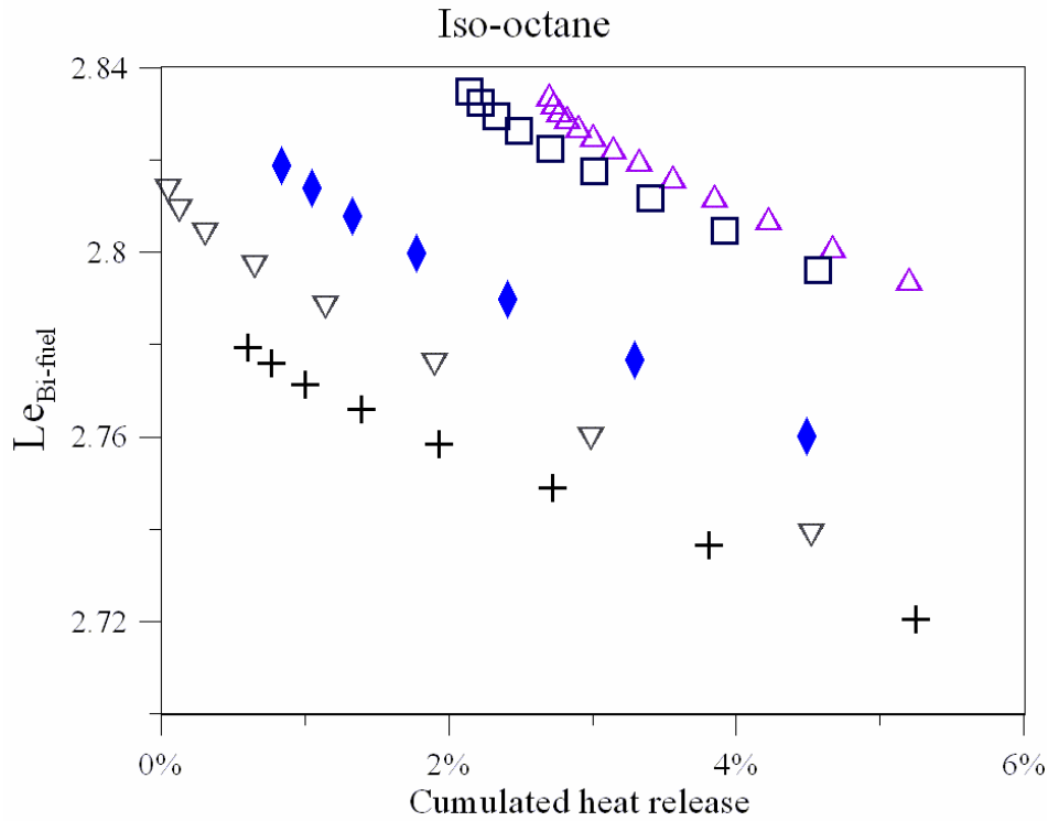
Figure 10. Le_{Bi-fuel} versus the percentage of cumulated heat release for mixtures with iso-octane (conditions 6-10): 6: + C_8H_{18}/Air ; 7: \triangle C_8H_{18}/air/20\%N_2 ; 8: \nabla C_8H_{18}/60\%H_2/Air ; 9: \blacklozenge C_8H_{18}/60\%H_2/5\%N_2/Air ; 10: \square C_8H_{18}/60\%H_2/20\%N_2/Air .
