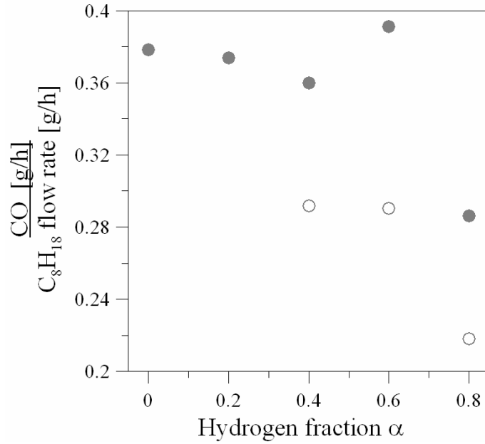
Figure 10.c Normalized CO emissions versus \alpha ( \phi = 1 ): imep_n = 287 \text{ kPa} , N = 2500 \text{ rpm} : \bigcirc CASE B P_{in}=55\text{kPa} , \phi = 1 . imep_n = 407 \text{ kPa} , N = 2000 \text{ rpm} : \bullet CASE B P_{in}=70\text{kPa} , \phi = 1 .
