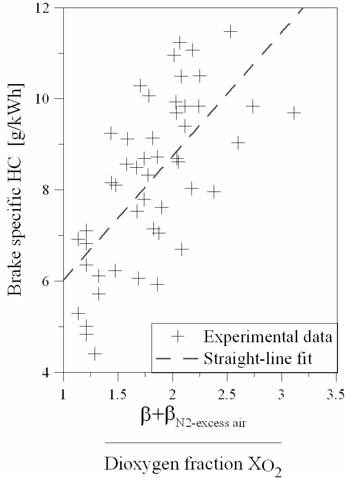
Figure 4. Brake specific HC versus \frac{\beta + \beta_{N_2\text{-excess air}}}{X_{O_2}}
