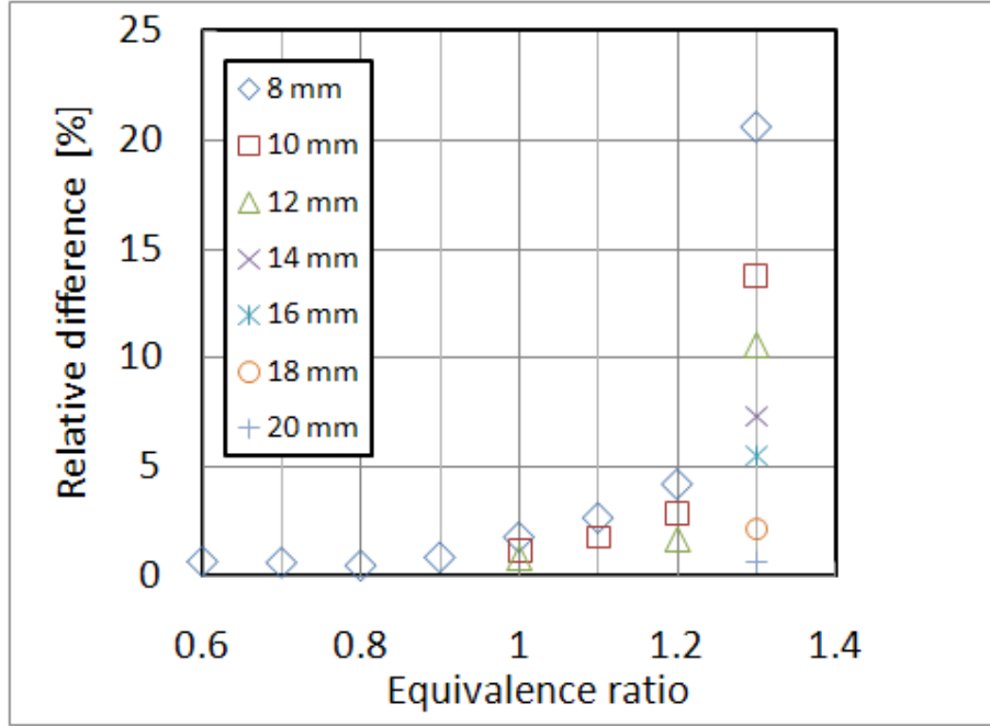
Figure 6. Relative error \left( \alpha = 100 \cdot \frac{|S_{u_{linear}}^0 - S_{u_{nonlinear}}^0|}{S_{u_{nonlinear}}^0} \right) obtained comparing linear and non-linear methodologies. Non-linear methodology is taken as the reference. Initial flame radius is varied from 8 mm to 20 mm (methane/air – P = 0.1 MPa – 300K).
