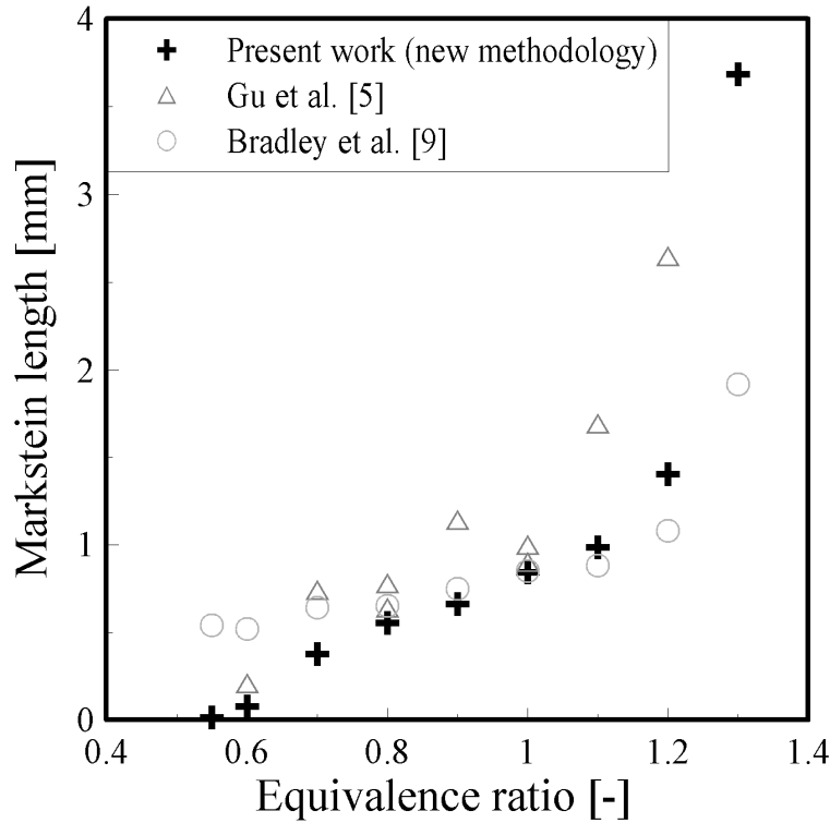
Figure 9.b Markstein length versus equivalence ratio ( \text{CH}_4/\text{air} mixtures - P=0.1\text{MPa} - T=300\text{K} ).
