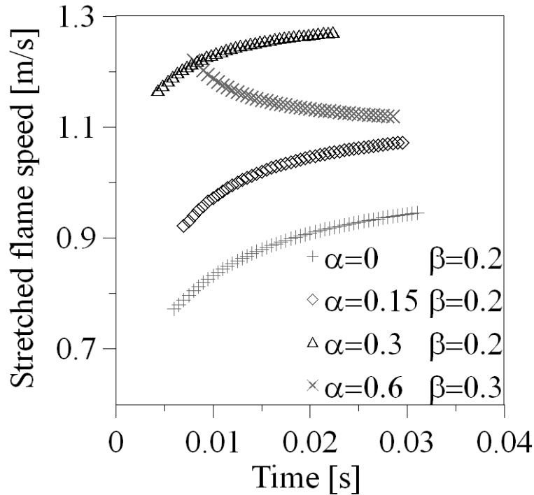
Figure 4. Temporal evolution of the stretched flame speed for four different mixtures (symbol frequency = 3), ( P=0.1 MPa, T=300 K).
