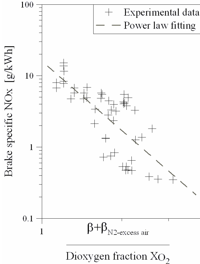
Figure 8. Brake specific \text{NO}_x versus \frac{\beta + \beta_{N_2\text{-excess air}}}{X_{O_2}} using a logarithmic scaling ( \text{imep}_n = 287 \text{ kPa} , N = 2500 \text{ rpm} and \text{imep}_n = 407 \text{ kPa} , N = 2000 \text{ rpm} ).
