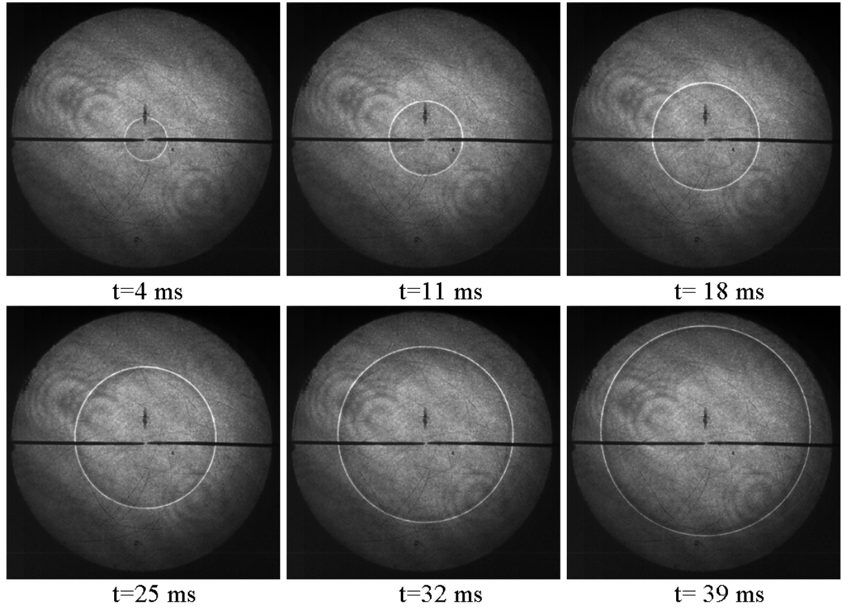
Figure 1. Examples of flame propagation shadowgraphs ( \alpha = 0.3 , \beta = 0.3 , P = 0.1 MPa, T = 300 K, 6000 images/second).
