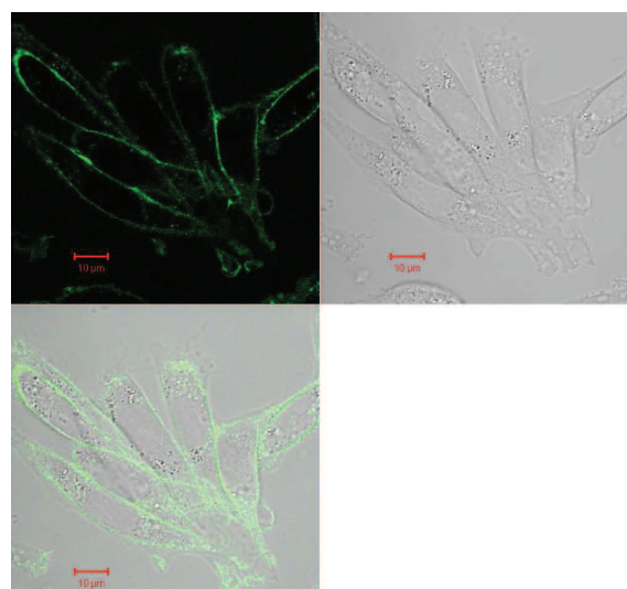
Formyl
