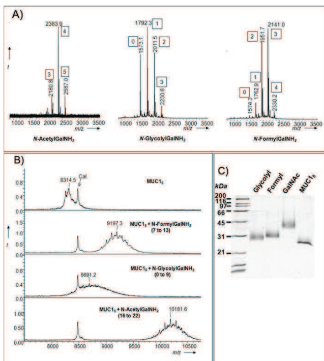
Fig. 4 Mass spectra (MALDI-TOF) of A) STP 5 and B) MUC1 8 glycosylated via the enzymatic cycle, with a representation of the [M+2H]^{2+} ions; the number of units added for each analog is given for each product. C) Coomassie-stained gel after SDS-PAGE of glycosylated and non-glycosylated MUC1 8 .
