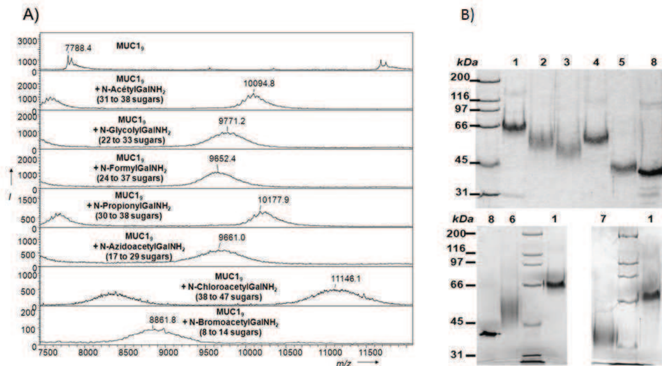
Fig. 2 Panel A) Mass spectra (MALDI-TOF) of MUC1 9 glycosylated by the GalNAc transferase ppGaNT1 starting from UDP-analogs, with a representation of the [M+3H]^{3+} ions; the extent of transferred sugars for each analog is indicated on each spectrum. Panel B) Coomassie-stained gels after SDS-PAGE of glycosylated MUC1 9 is shown with N -acetyl (1), N -glycolyl (2), N -formyl (3), N -propionyl (4), N -azidoacetyl (5), N -chloroacetyl (6), N -bromoacetyl (7) galactosamine derivatives and non-glycosylated MUC1 9 (8).
