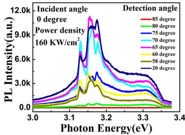
Fig 4.4 The RT PL spectra in the ZnO NWs under different detection angles with the excitation power density of 160 \text{ kW/cm}^2 .
