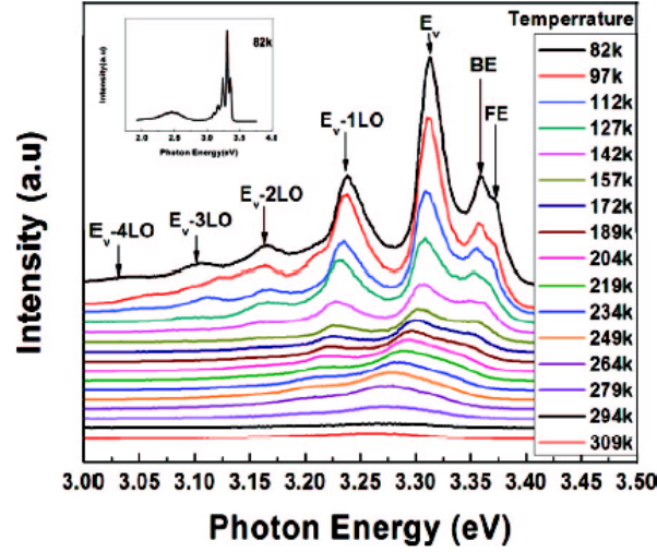
Fig 3.4 Photoluminescence spectra of the ZnO nanobolt arrays measured at different temperatures (from 82 to 309 K). The inset is a typical PL spectrum measured at 82K.
