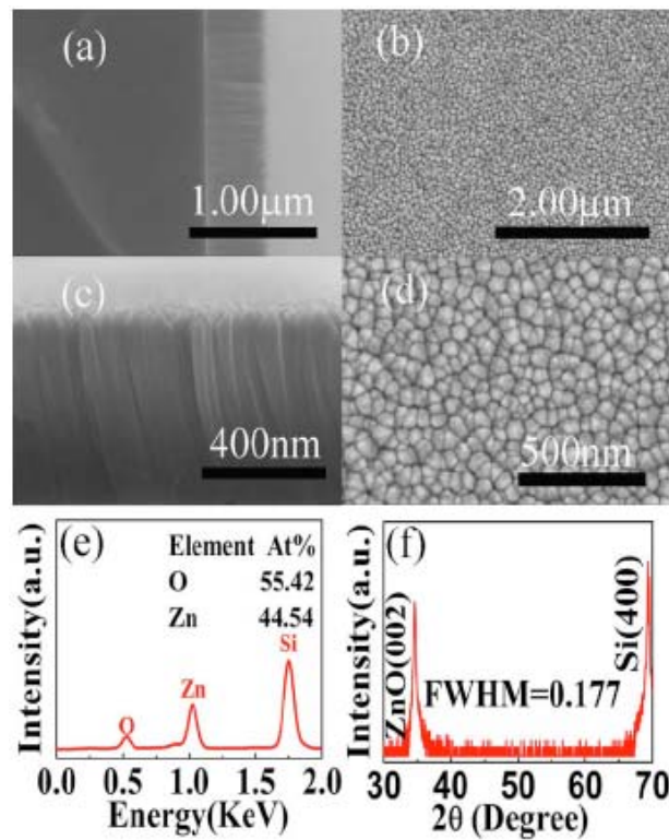
Fig 5.1(a) Cross-sectional SEM image of the ZnO NW arrays fabricated on Si substrate, (b) Top view image of the ZnO NW arrays, (c) Magnified cross-sectional SEM image of the ZnO NW arrays, (d) Magnified surface image of the ZnO NW arrays. (e) The EDX spectrum shows the composition of Zn and O element. (f) The XRD pattern of the ZnO NW arrays fabricated on the Si (100) substrate.
