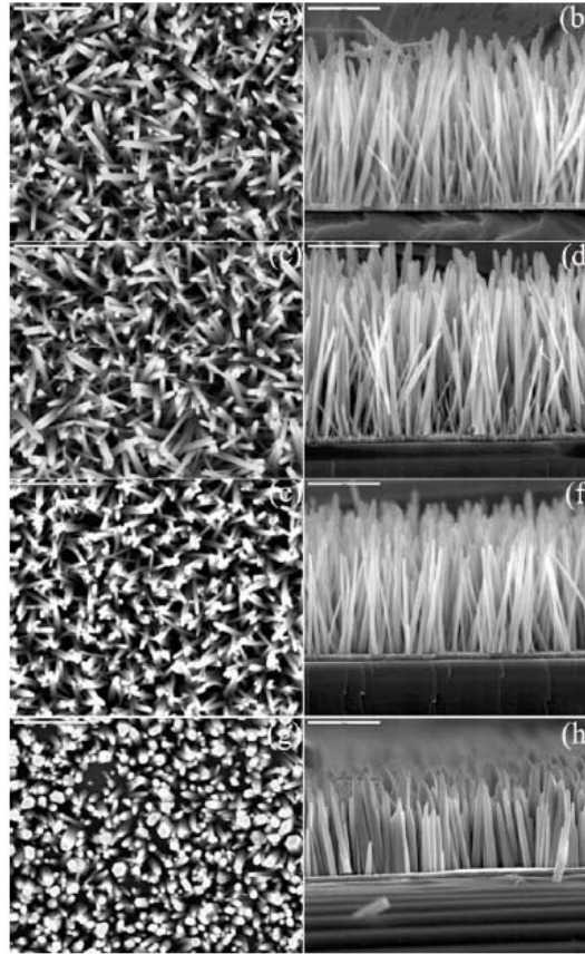
Fig 3.12 (a-b), (c-d), (e-f), (g-h) SEM images for samples E , F , G and H , respectively. The scale bar is 1 \mu\text{m} .
