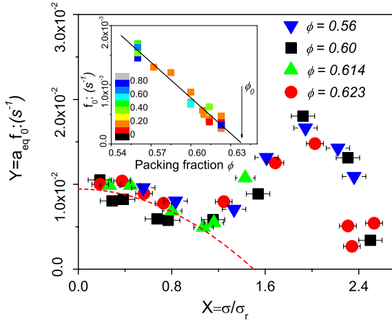
FIG. 4 (color online). Rescaled ageing parameter a_{eq}f_0 as function of rescaled of shear stress \frac{\sigma}{\sigma_r} , dotted line: y = \frac{1}{1 + (\frac{X}{1.5})^2} with t_* \cong 106 s. Inset : initial fluidity f_0 as a function of packing fraction for different shear stresses, the color index reflects the ratio \sigma/\sigma_M , fit line: y = F(\phi_0 - \phi) with F = 0.0203 and \phi_0 = 0.635 \pm 0.002 .
