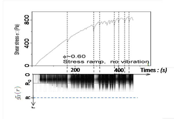
FIGURE 3.32: Response to a stress ramp on the sample surface. Shear stress as a function of times for a packing fraction \phi = 0.60 and \dot{\beta} = 0.00052 \text{ rad/s} with the juxtaposing of \bar{g}_I(r)
