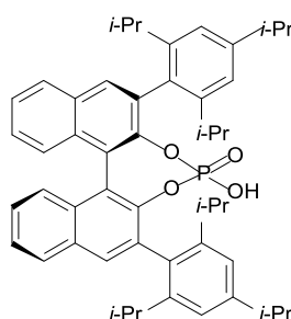
Figure 77 : (R) -TRIP
