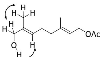
Figure 56
