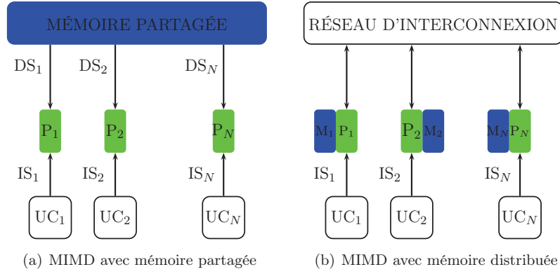
FIGURE 1.5 – Architecture MIMD (Multiple Instruction Multiple Data)
