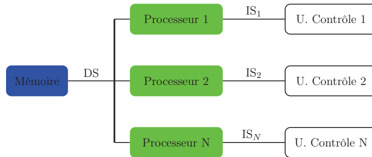
FIGURE 1.4 – Architecture MISD (Multiple Instruction Single Data)
