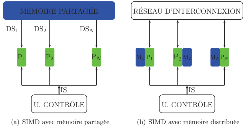
FIGURE 1.3 – Architecture SIMD (Single Instruction Multiple Data)
