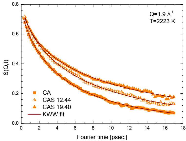
Figure 5.11 Comparison between the CA, CAS 12.44 and CAS 19.40 intermediate scattering function decay at 2223 K for Q=1.9 \text{ \AA}^{-1} .
