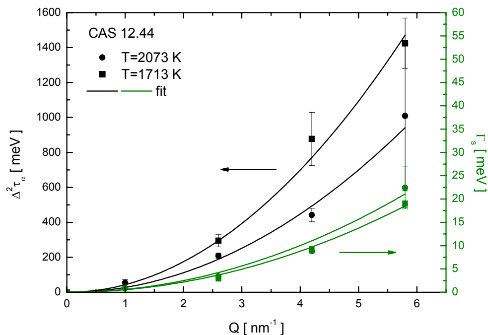
Figure 5.26 The quadratic behavior of the partial contributions to the longitudinal viscosity from the slow (structural) and the fast (instantaneous) components for the CAS 12.44 at 1713K and 2073K.
