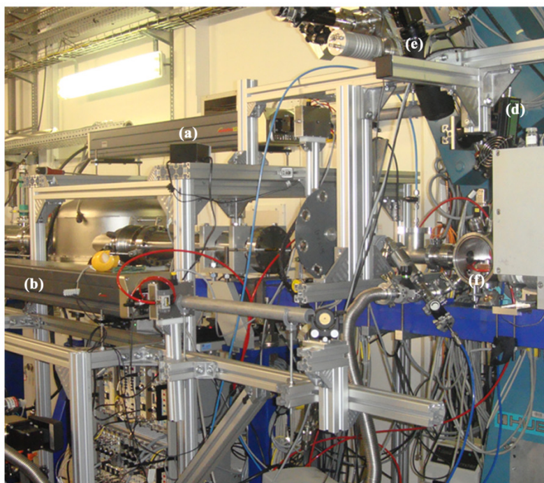
Figure 5.16 Aerodynamic levitation setup at ID16 for IXS experiments.
