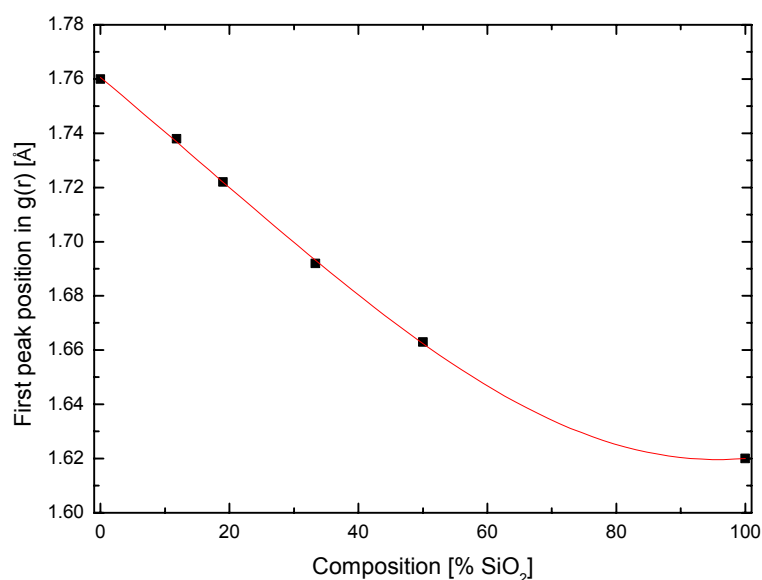
Figure 4.6 Evolution of the first peak in the total pair distribution function g(r) of (\text{CaAl}_2\text{O}_4)_{1-x}(\text{SiO}_2)_x glasses at room temperature as a function of \text{SiO}_2 concentration. The value corresponding to pure silica (100% \text{SiO}_2 ) is taken from Ref. [6].
