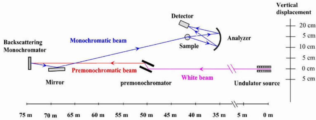
Figure 3.9 Sketch of the inelastic scattering beamline ID16 at the ESRF.
