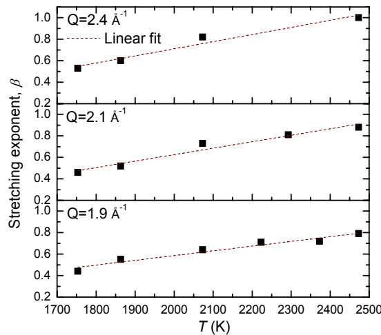
Figure 5.5 Temperature dependence of the stretching parameter \beta around the Q value corresponding to the first diffraction peak in CA ( Q = 2.1 \text{ \AA}^{-1} ), obtained from KWW fits to QENS data.
