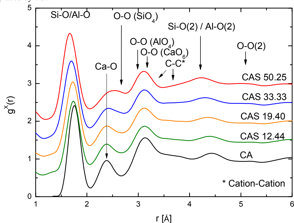
Figure 4.13 The total pair distribution function g^X(r) for the (\text{CaAl}_2\text{O}_4)_{1-x}(\text{SiO}_2)_x glasses at room temperature as obtained by Fourier transforming the corresponding total structure factors. For clarity, the CAS compositions have been displaced by 0.5.
