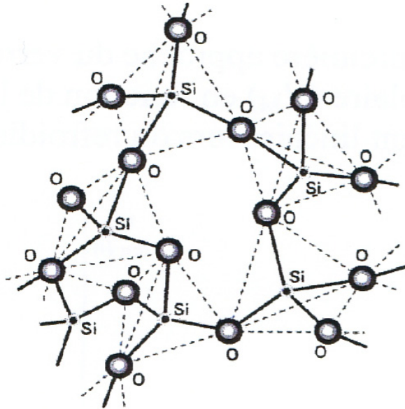
Figure 1.9 3D representation of a glassy silicate [41].
