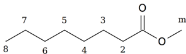
Fig. 2. Example of the nomenclature used in this kinetic mechanism for methyloctanoate.
