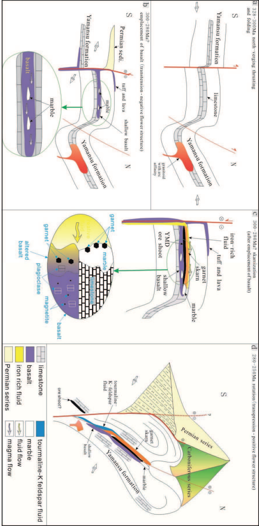
Fig. B-15: Hypothetical metallogenic model of the Yamansu iron deposit
