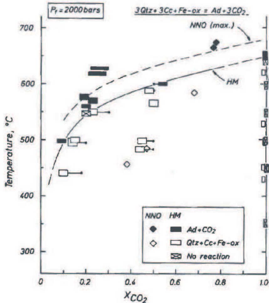
Fig. 1-8: Experimentally determined T- X_{\text{CO}_2} diagram for the reaction: 3\text{quartz}+3\text{calcite}+(1/4)\text{hematite}+(1/2)\text{magnetite}+(1/8)\text{O}_2=\text{andradite}+3\text{CO}_2 .
