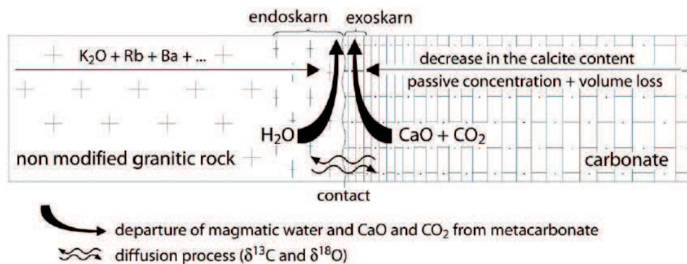
Fig. 1-7: (A) gain and loss of elements from the Oswald limestone, Santa Rita stock; (B) schema showing the elements' immigrate direction (Ague and van Haren, 1996; Durand, 2006; Durand et al., 2009).
