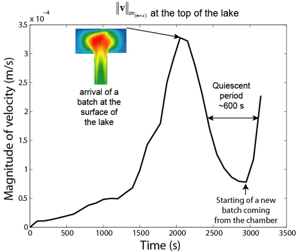
Figure 8. Characteristics of the lake surficial velocities: average values of the magnitude of velocity vector at the first meter of the lake obtained along cells in the x-direction average per time step (every 100 s).
