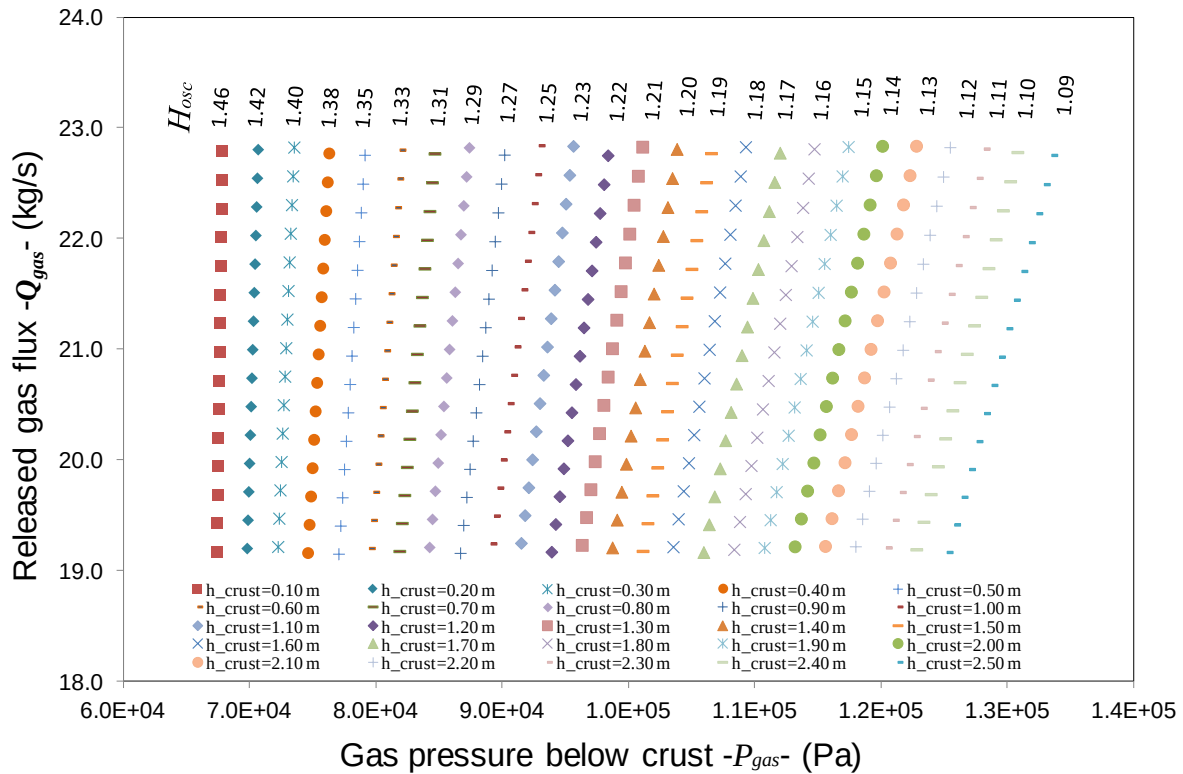
Figure 3. Released mass flux, Q_{gas} , at very P_{step} , through a crust of permeability varying from 3.01 \times 10^{-10} \text{ m}^2 to 2.16 \times 10^{-10} \text{ m}^2 as a function of the confined pressure, P_{gas} , for different thicknesses of the crust, h_{crust} . Q_{gas} is calculated through equation (4) and H_{osc} is obtained by multiplying the average crust velocity by a fixed time interval of 5 minutes
