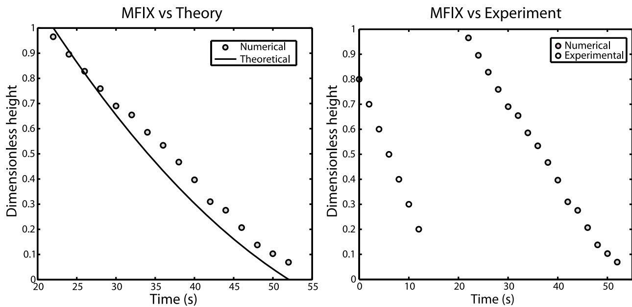
Figure A1. Dimensionless height of the plume cap versus time for the oil 47V20: (a) Gray circles represent our numerical results while the continuous black line is the theoretical curve based on Read [1984] and Youngs [1984] (equation (7)). (b) Open circles represent the results of the analogical experiment while gray circles represent our numerical results, both at early times. The height of the tank is 10 cm (1 in non-dimensional units).
