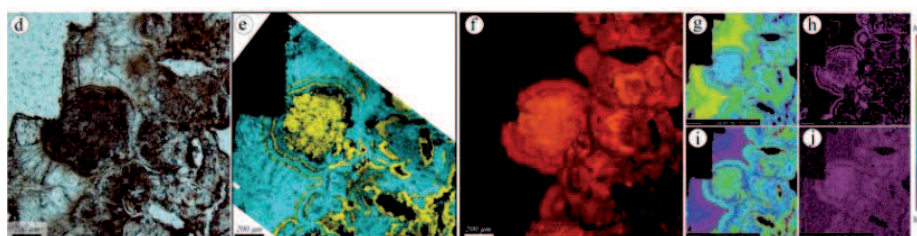
Figure B.3: Optical observations, Raman maps and analyses of the Svalbard carbonates. d- Optical view in transmitted light of layered carbonates from Svalbard, Norway. e- Raman map of (d) with in magnesite light blue and dolomite in yellow (laser power: 5 mW, obj. x100). f- Cathodoluminescence image, this image reveals the low content of Mn and Mg in the sample and, in particular, the zoned structure of the crust. g to j- Microprobe elemental maps of Mg, Ca, Fe and Mn. Note the detail of the magnesite deposit and the relation between the Ca-Mg and Fe maps and the cathodoluminescence image: The content of Mn and CL activation are correlated. (For the four maps, low contents are in purple and high contents in red).
