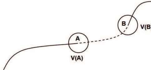
Figure 6.7: Hysteresis thresholding
