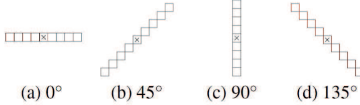
Figure E.2: 2D linear orientations, the \times marked the pixel (x, y) .
