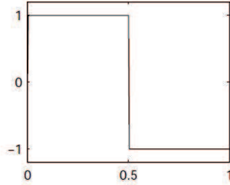
Figure C.1: Haar Wavelet.
