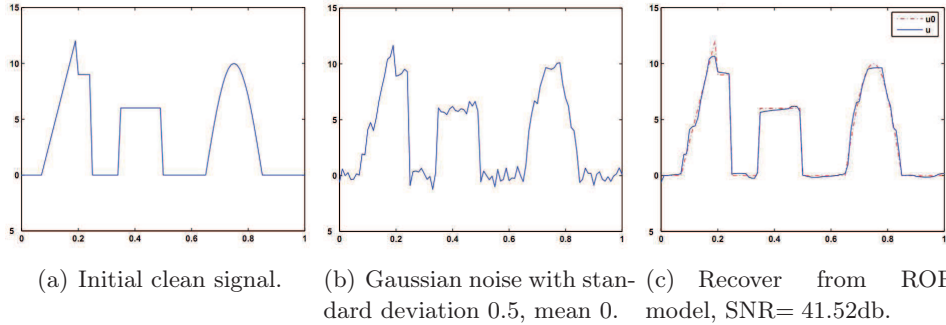
Figure B.1: One-dimensional ROF denoising, signal reproduced from [10].
