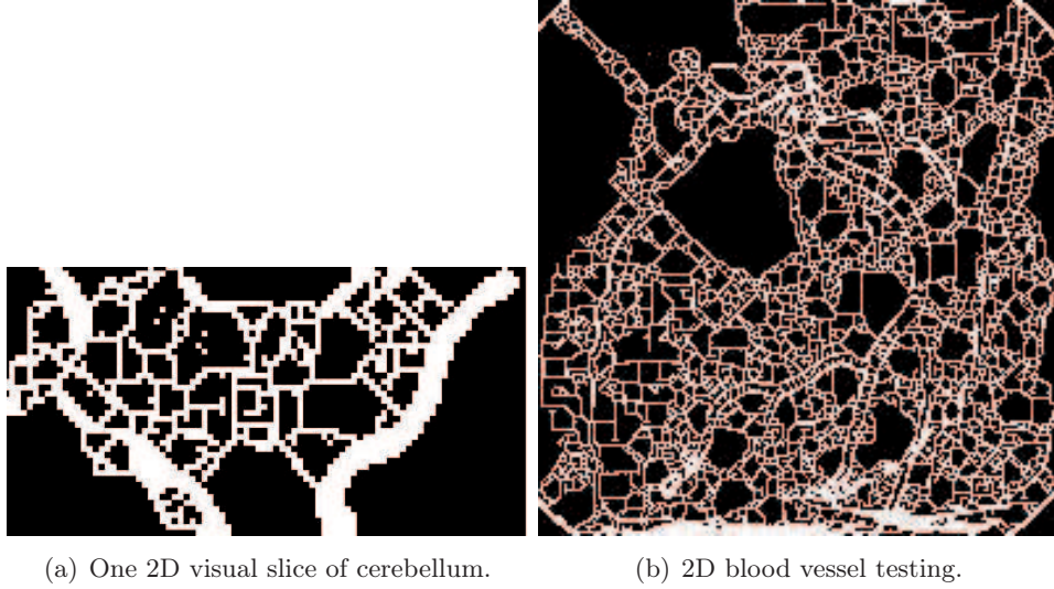
Figure 6.14: False detections occur when finding closed contours by Chamfer-distances, described in remark 2.
