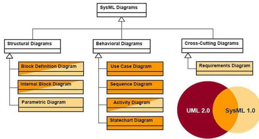
Figure I.6 : Organisation des diagrammes SysML
