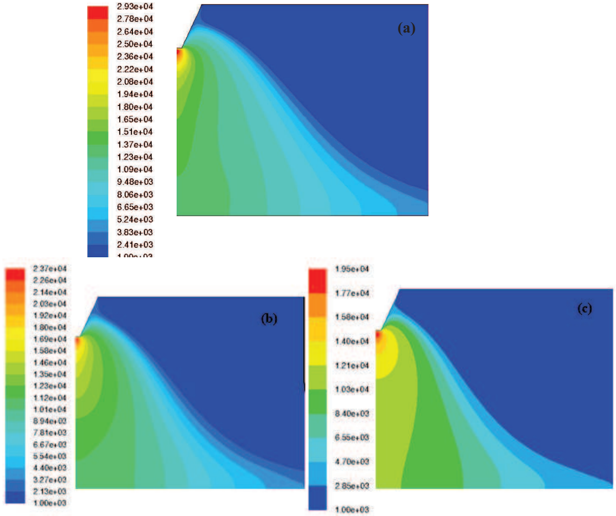
Figure 3. 12: Temperature profile of different current (100 A (a), 70 A (b), 50 A (c))
