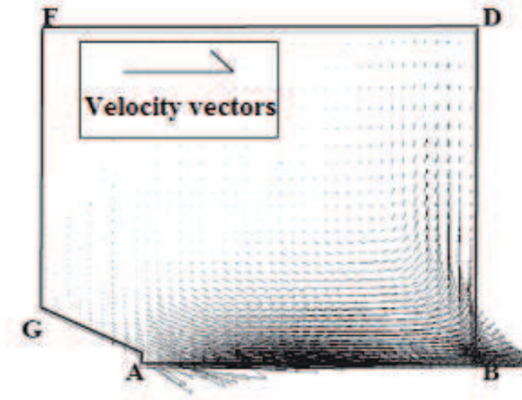
Figure 3. 11: Velocity field in free-burning argon arc.
