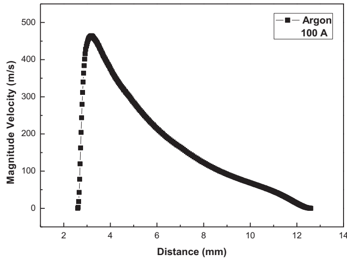
Figure 3. 4:Axial velocity of argon free-burning arc, ( I=100\text{ A} ).
