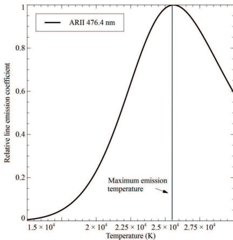
Figure 4. 3: Relative emission coefficient of the \text{Ar}^+ line at 476.4 nm as a function of the temperature.
