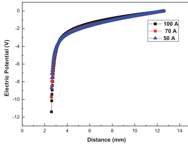
Figure 3. 14: Potential changes along axis (different currents).
