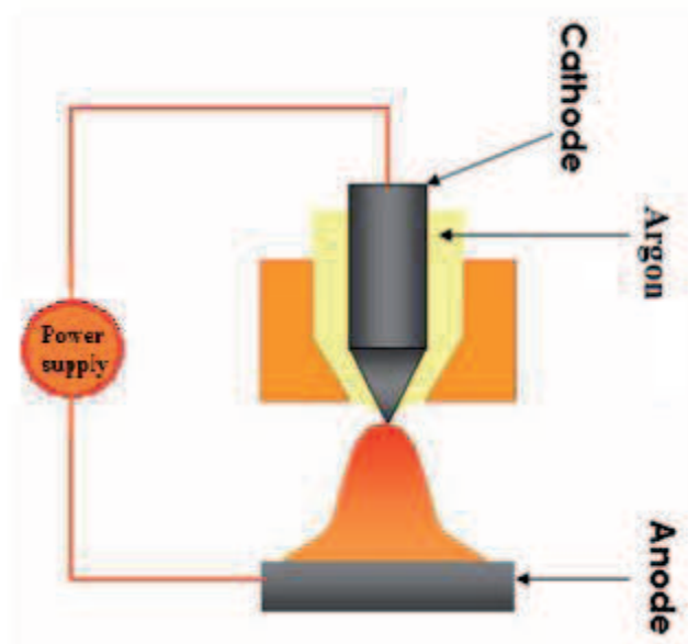
Figure 2. 2: Schematic TIG.
