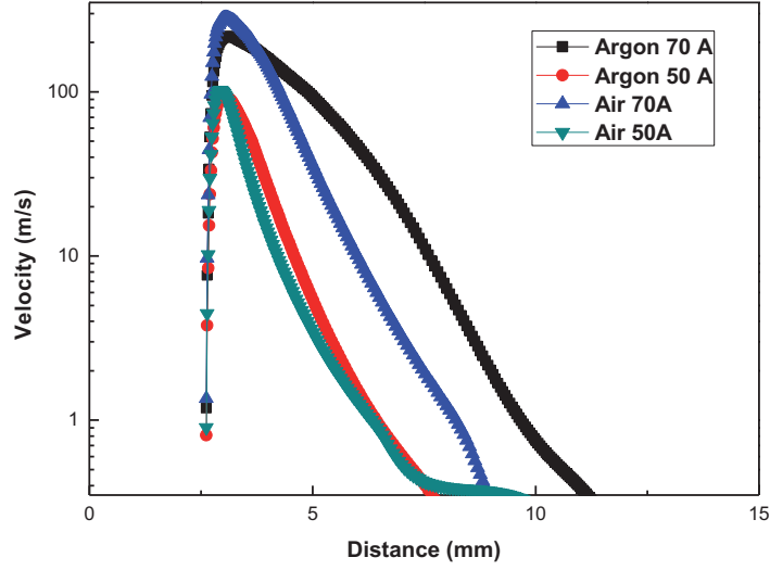
Figure 3. 17: Axial velocity with different current (Air/Argon).
