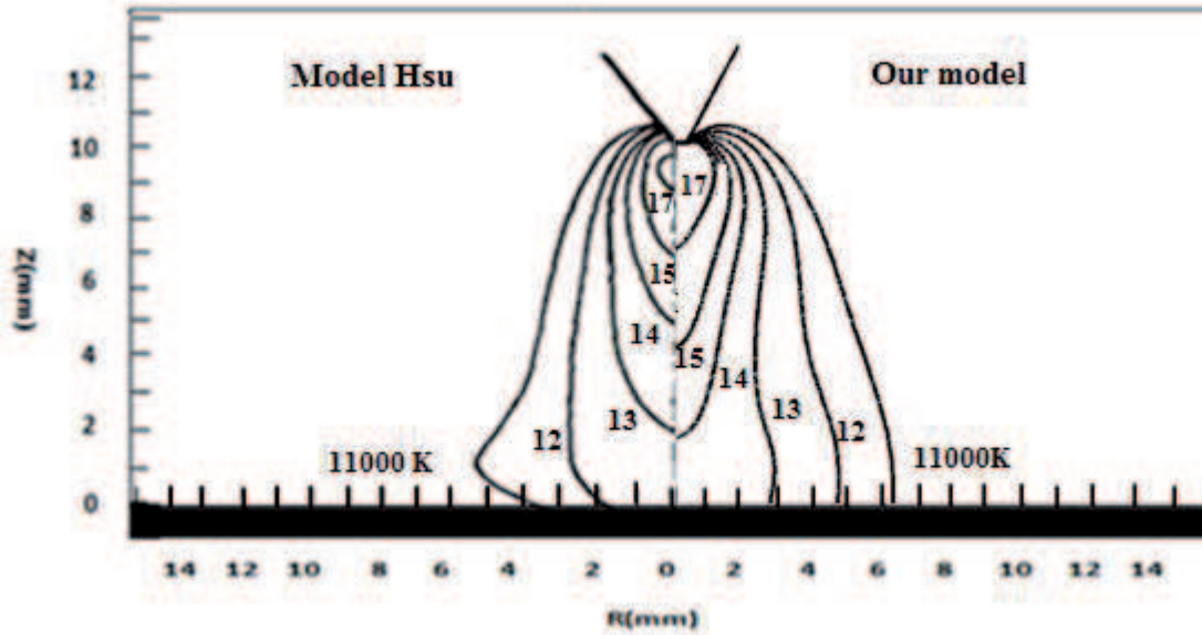
Figure 3. 2: Comparison between our calculated isotherms of free-burning argon arc and Hsu model ( I= 100\text{ A} , d =10\text{mm} ).
