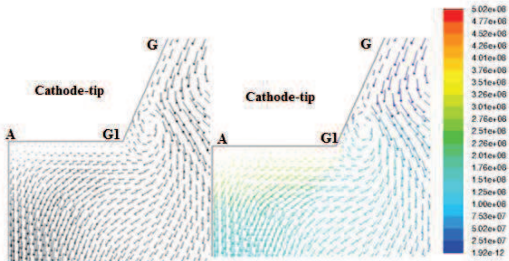
Figure 3. 9: Axial current density vectors on the cathode- tip100 A.
