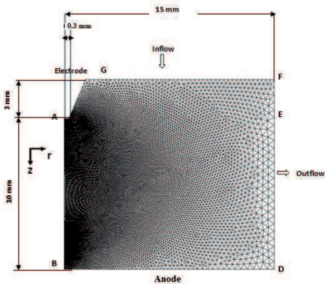
Figure 2. 3: Computational domain.
