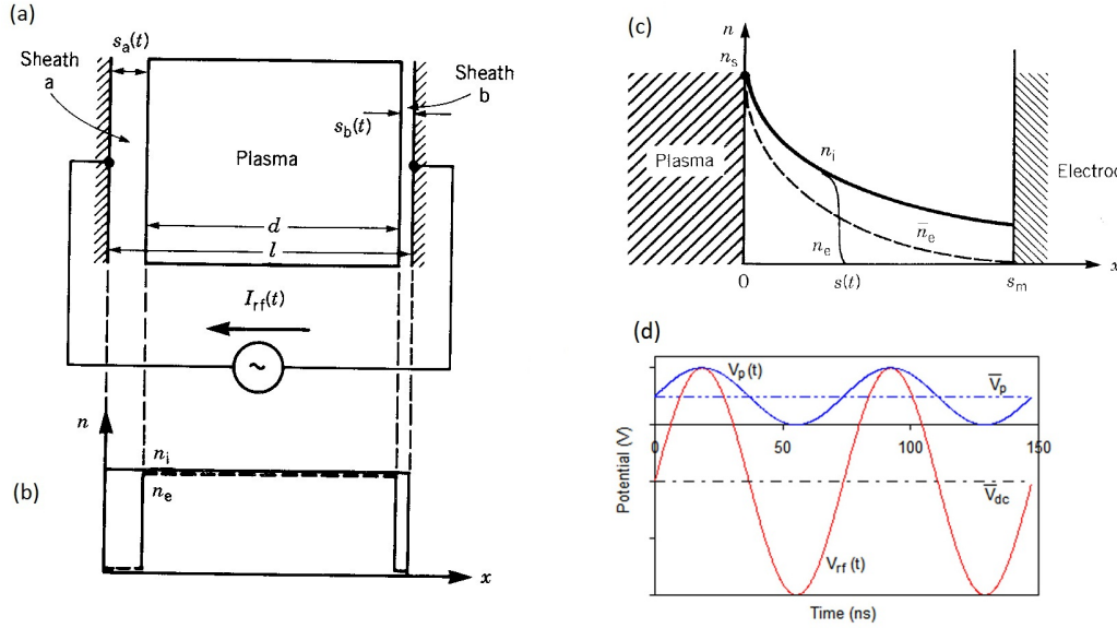
Figure 1.3: Sketch of a radio frequency driven plasma(a). Plot (b) displays the distribution of the electron and ion density along the plasma and the sheath, [128]. Next to it a more realistic distribution of the electron and ion densities in the sheath is given. This figure is reproduced from [127]. Furthermore, the development of the applied RF voltage V_p , the resulting plasma potential V_p , the corresponding time average \bar{V}_p , and the self bias \bar{V}_{dc} is shown,[71].
