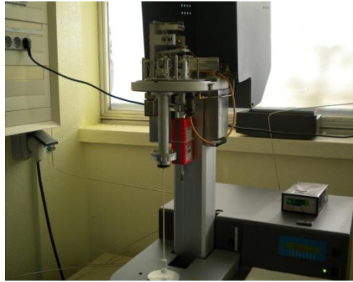
Figure II-11 ATD/ATG SETARAM 7.6 SETSYS 2400
