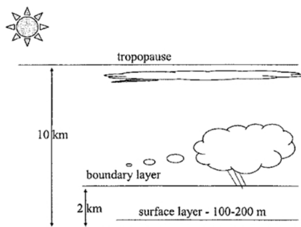
Figure 2.1.: The structure of the atmospheric boundary layer (ABL).
