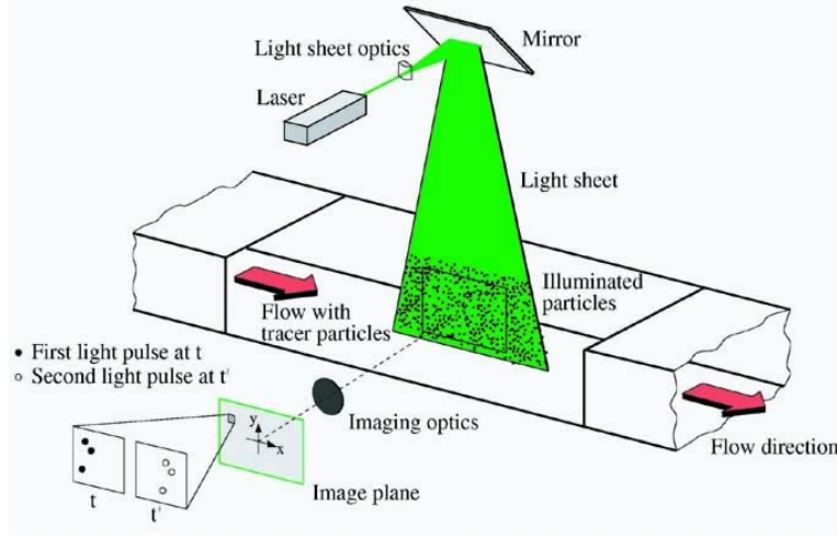
Figure A.1.: Principle of PIV. Image from [83]
