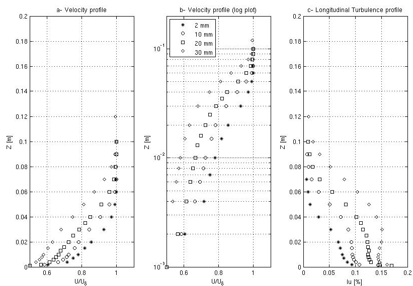
Figure 3.26.: Effect of the roughness height modelled by CFD.
