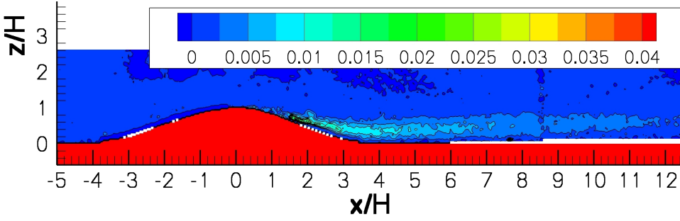
Figure 4.13.: The normalized Reynolds shear stress -\overline{u'w'}/U_0^2 [-] over a low hill.
