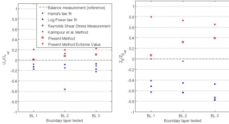
Figure 3.13.: Comparison of friction velocity u_* and aerodynamic roughness length z_0 determined by different methods.
