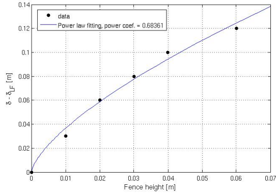
Figure 3.30.: Evolution of the boundary layer height ( \delta - \delta_{LF} ) with the fence height H_F .
