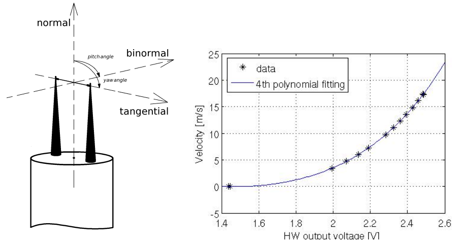
Figure A.3.: View of a single wire hot-wire (left). Example of a 4 th order polynomial fitting on calibration data (right).
