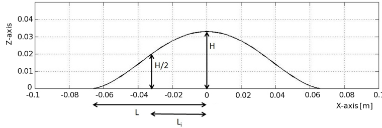
Figure 4.2.: Example of the hill shape obtained from the parametric equations (equation 4.11) with H = 33 mm and L/H = 2 .
