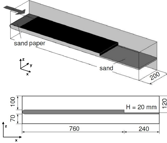
Figure C.3.: Wind tunnel set-up for the backward-facing step test case [33].
