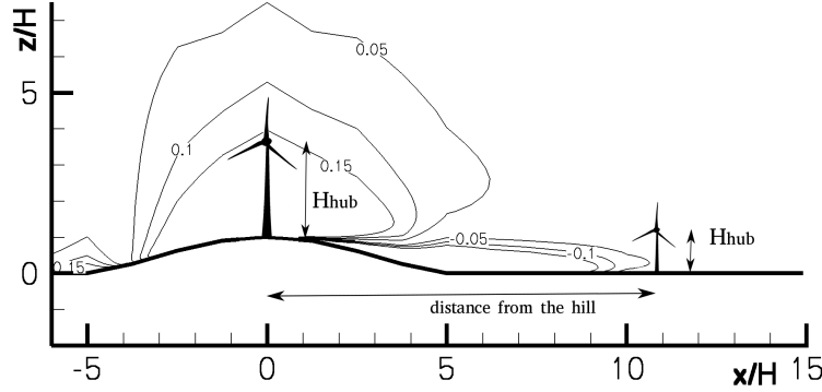
Figure 4.31.: Summary of a typical FSR ( \Delta S ) over a hill and the positioning of wind turbines.
