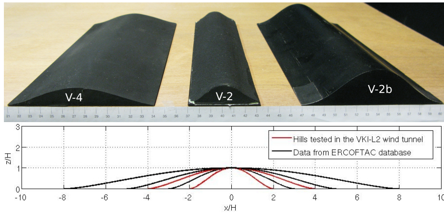
Figure 4.5.: Top: picture of the three hills tested in the VKI-L2 wind tunnel. Bottom: hill shapes investigated in this study, red contours are the hills tested in the wind tunnel, the data of the black contours hills are extracted from the ERCOFTAC database.
