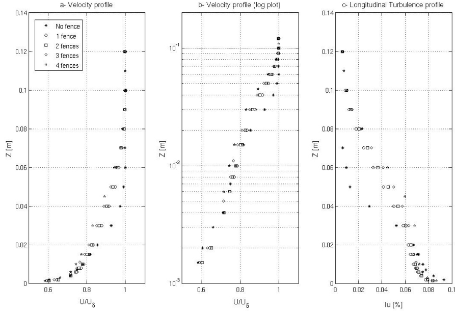
Figure 3.24.: Effect of the number of fences studied in VKI-L2 wind tunnel.
