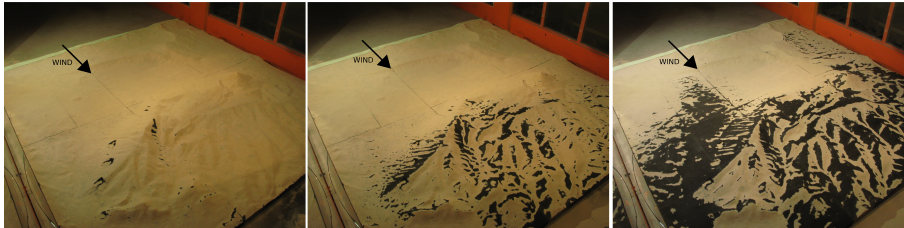
Figure 5.33.: Example of a model at the beginning of the test (left) after 1 min at 6 m/s (middle) and after 1 minute at 7 m/s (right).
