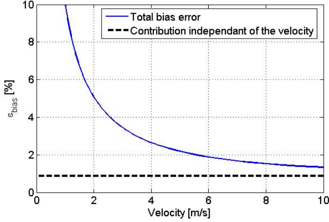
Figure A.2.: Example of the evolution of the bias error in function of the local speed (equation A.12).
