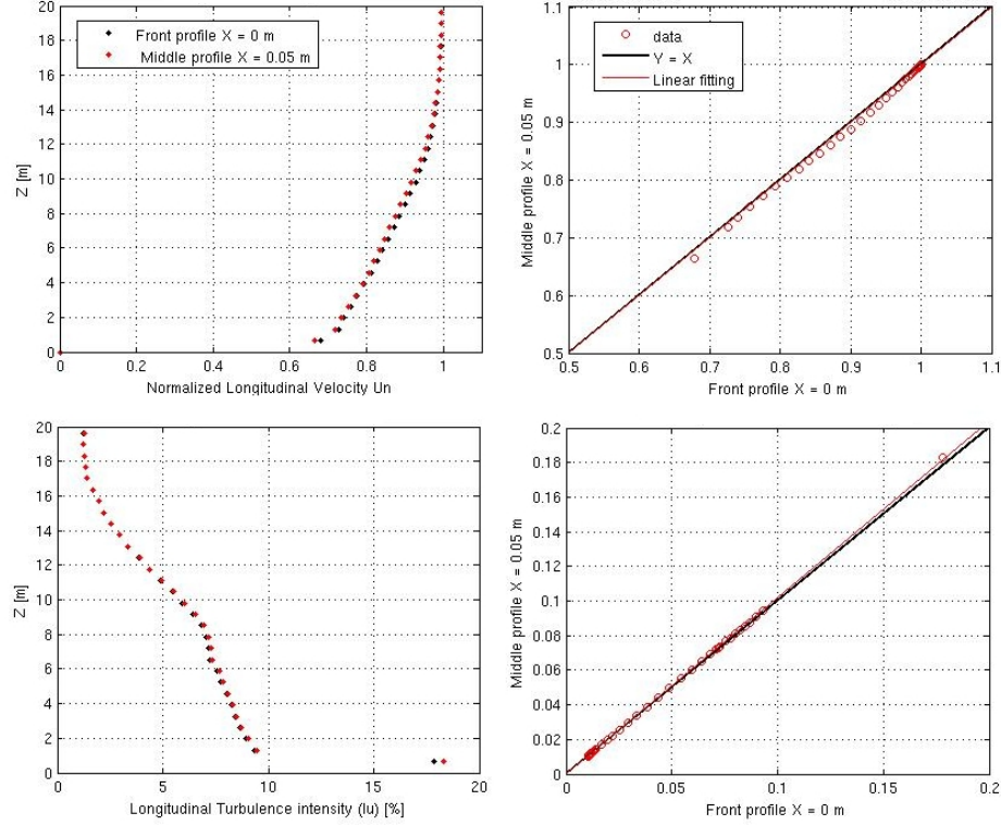
Figure 3.10.: Tests on the fully development state of the BL in VKI-L2 test section. Comparison of the normalized velocity profile (upper left) with the scatter plot (upper right) and of the turbulence profile (lower left) with scatter plot (lower right).
