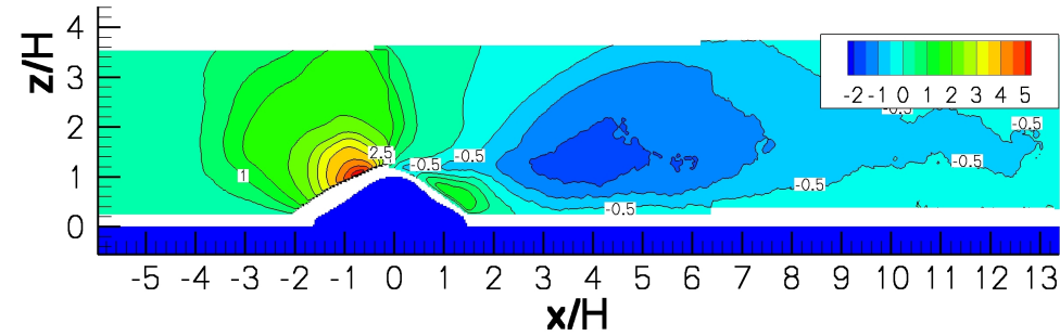
Figure 4.18.: The vertical wind velocity component W [m/s] over the steep hill.
