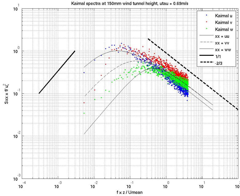
Figure 3.19.: Velocity spectra in the VKI-L1 wind tunnel performed at an altitude of Z = 0.15 m compared with Kaimal [52].
