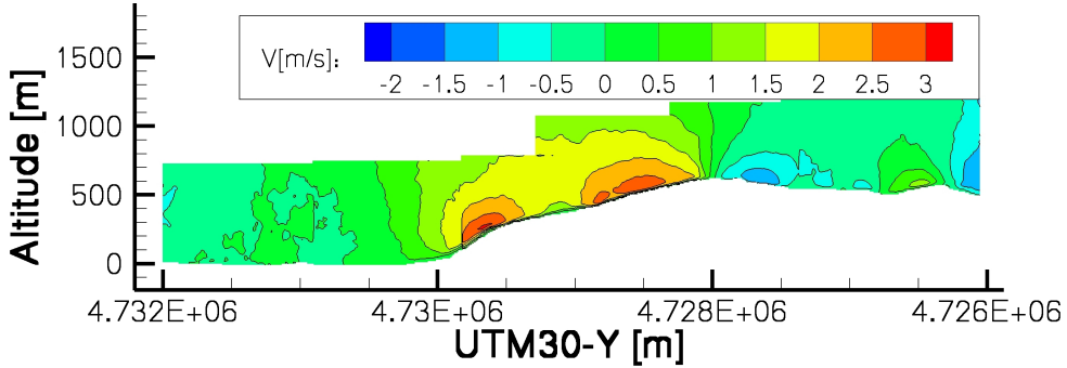
Figure 5.36.: Longitudinal velocity field over Alaiz terrain.
