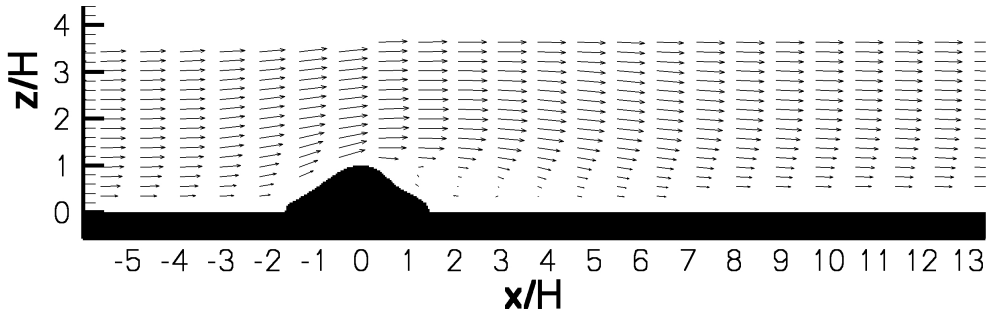
Figure 4.17.: The velocity vector field over the steep hill.
