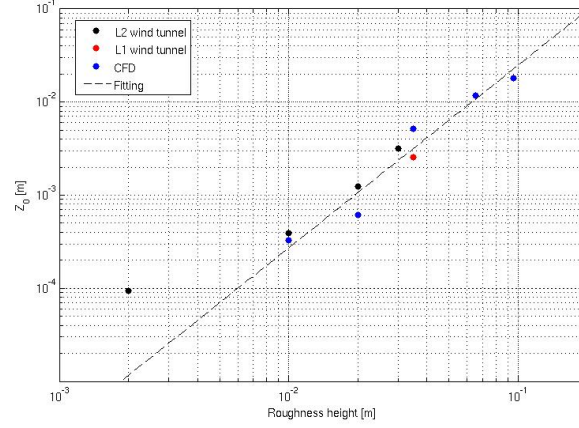
Figure 3.33.: Evolution of the aerodynamic roughness length z_0 with the roughness height H_R .
