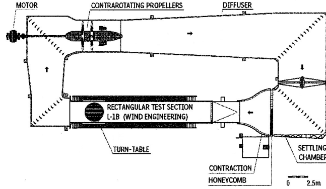
Figure 3.1.: VKI-L1 wind tunnel in wind engineering configuration.
