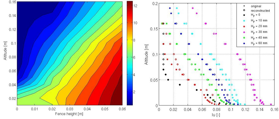
Figure 3.32.: Contour map of the longitudinal turbulence level in function of the altitude and the fence height [%] (left). Comparison between the original and reconstructed turbulence intensity profiles (right).
