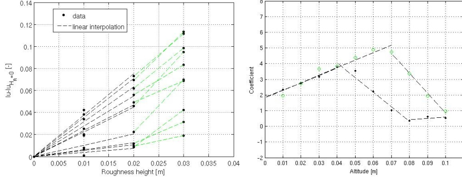
Figure 3.34.: Evolution of the longitudinal turbulence level ( Iu ) with the roughness element height H_R with a linear interpolation (left), and evolution of the linear interpolation coefficient with height (right)
