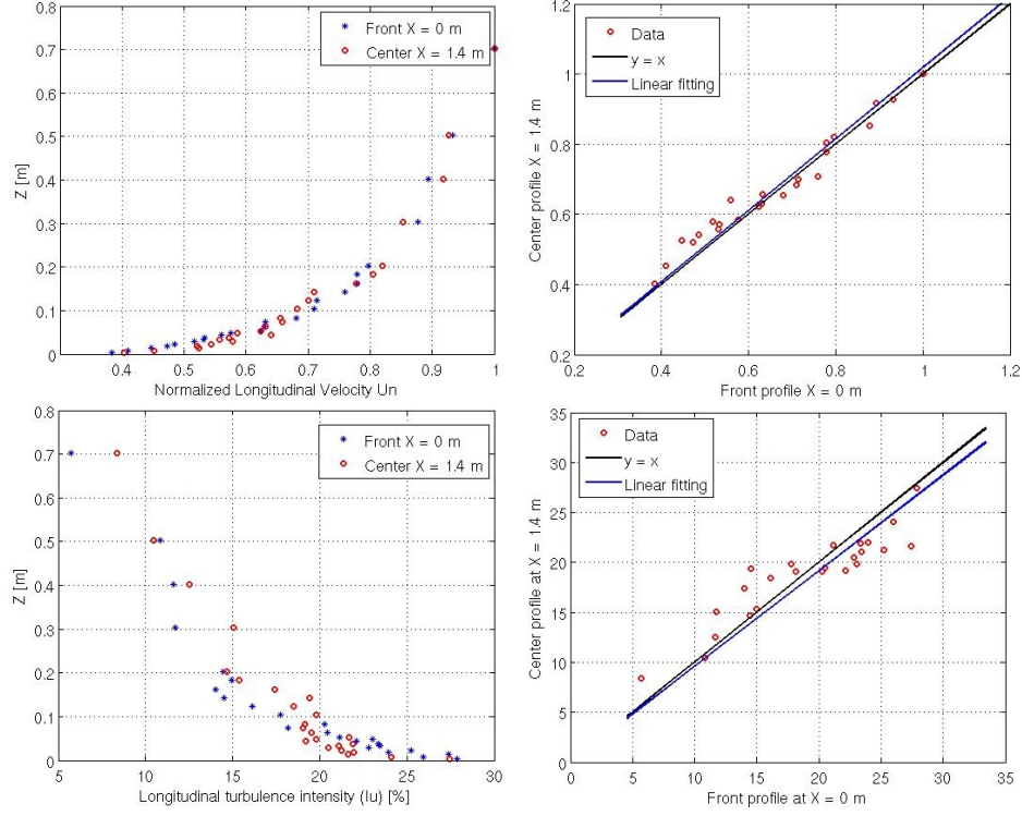
Figure 3.9.: Tests on the fully development state of the BL in VKI L1 test section. Comparison of the normalized velocity profile (upper left) with the scatter plot (upper right) and of the turbulence profile (lower left) with scatter plot (lower right).
