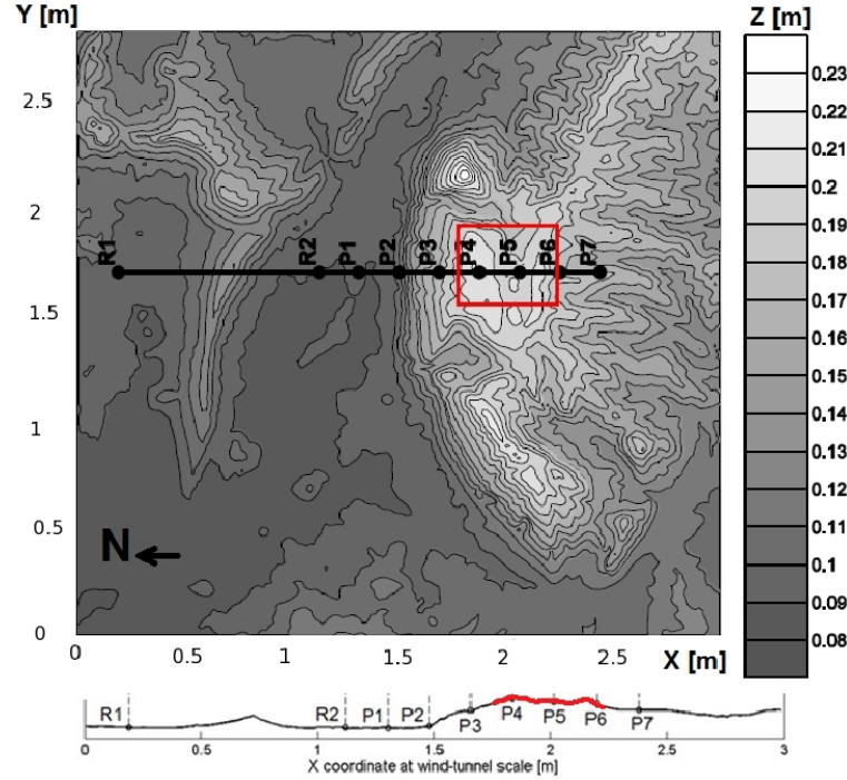
Figure C.6.: Alaiz model: top view and profile of the terrain following the measurement line. Red area: sand erosion zone. Points R1 and R2 are reference positions and points P1 to P7 are measurement position.
