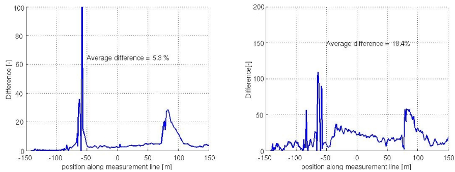
Figure 5.18.: Quantification of the Reynolds number effect on the FSR at 5 m. Percentage of error along the terrain for the FSR (left) and the turbulence kinetic energy increase \Delta k (right).
