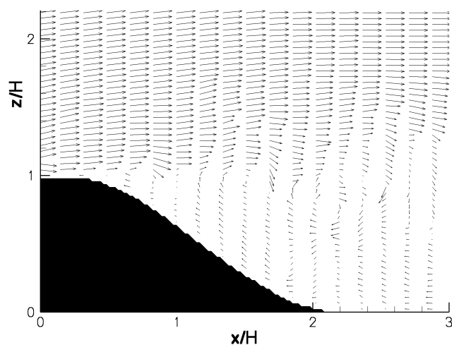
Figure 4.14.: The instantaneous velocity field in the near wake of the steep hill. Several vortices can be distinguished.
