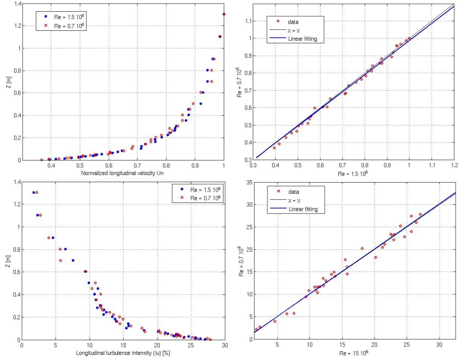
Figure 3.7.: Presentation of the Reynolds number dependency in VKI-L1 test section. Comparison of the normalized velocity profile (upper left) with the scatter plot (upper right) and of the turbulence profile (lower left) with scatter plot (lower right). The velocity profile is normalized at 1.3 m
