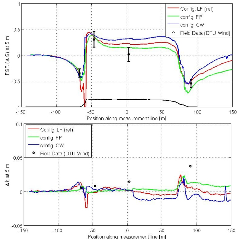
Figure 5.20.: \Delta S and \Delta k for three different inlet conditions.
