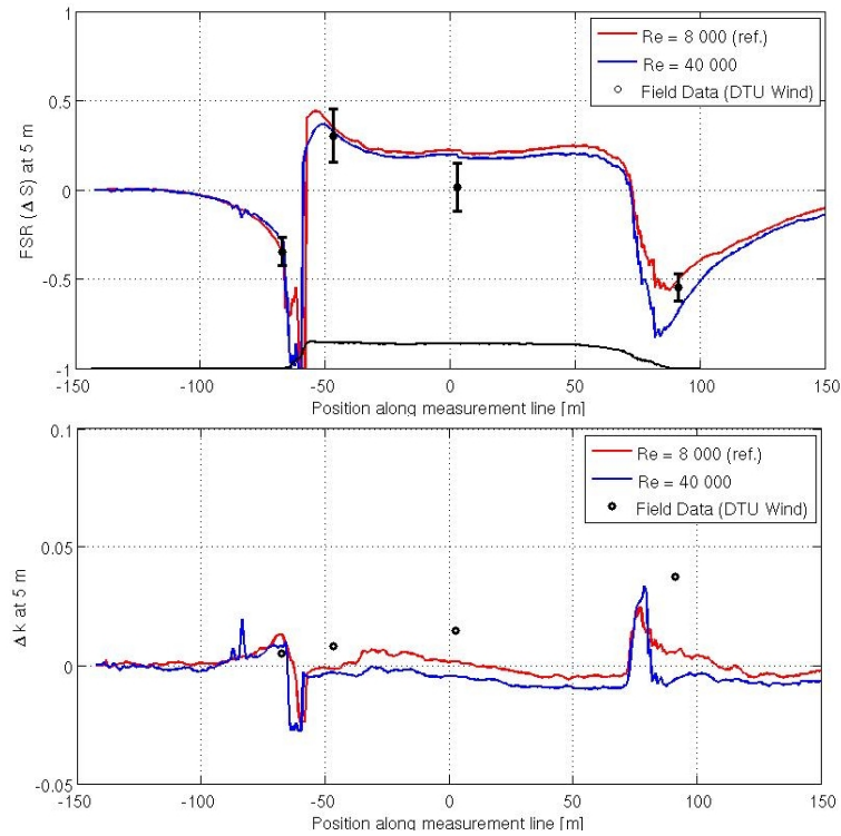
Figure 5.17.: \Delta S and \Delta k for two different Reynolds numbers.
