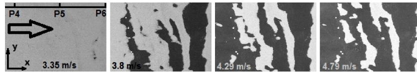
Figure C.7.: Example of an evolution of the erosion pattern with the free-stream velocity (red area on Figure C.6).
