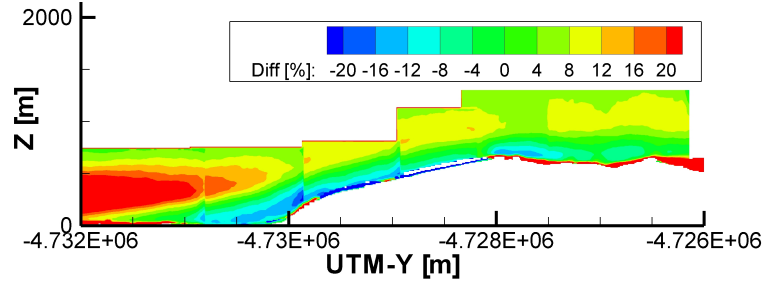
Figure 5.49.: Error plot of the discrepancy between the FSR from the experimental and from the numerical 3D simulations.
