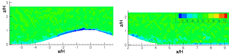
Figure 4.7.: Vorticity field ( \omega_Y ) (flood) in the near wake of a low hill (V-4).
