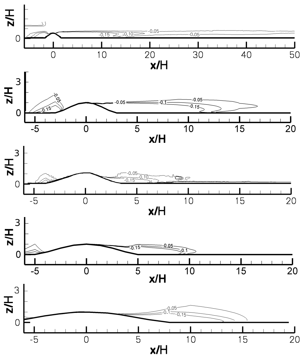
Figure 4.25.: Contours of the wake calculated from the FSR ( \Delta S ) with the criteria: \Delta S = -0.15 , \Delta S = -0.10 and \Delta S = -0.05 for the five hills (from top to bottom): L = 2H , L = 3H , L = 4H , L = 5H and L = 8H .
