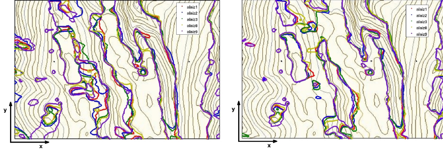
Figure C.8.: Superposition of the sand contours of five independent runs performed at two velocity steps 4.29 m/s (left) with 6.5% scatter and 4.79 m/s (right) with 5.5% scatter.
