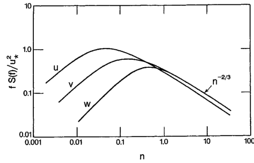
Figure 2.6.: Normalized neutral Kaimal spectra for u , v , and w in the surface layer [52].
