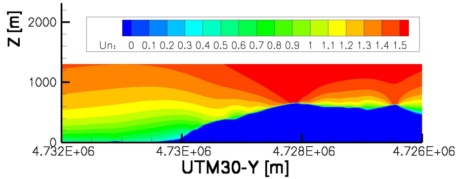
Figure 5.43.: Velocity ratio, U/U_{R1}(90m) , from the 2D CFD computation [63].
