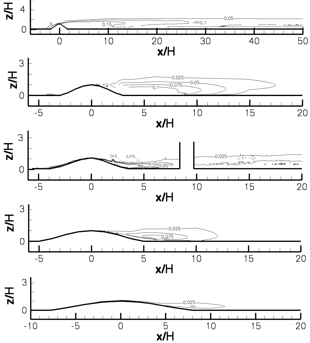
Figure 4.27.: Contours of the residual turbulence intensity Iu_w from equation 4.13. Iu_w = 0.05 means that the local turbulence is increased like Iu(z) = Iu_0(z) + 0.05 . Results are shown for five hills (from top to bottom): L = 2H , L = 3H , L = 4H , L = 5H and L = 8H .
