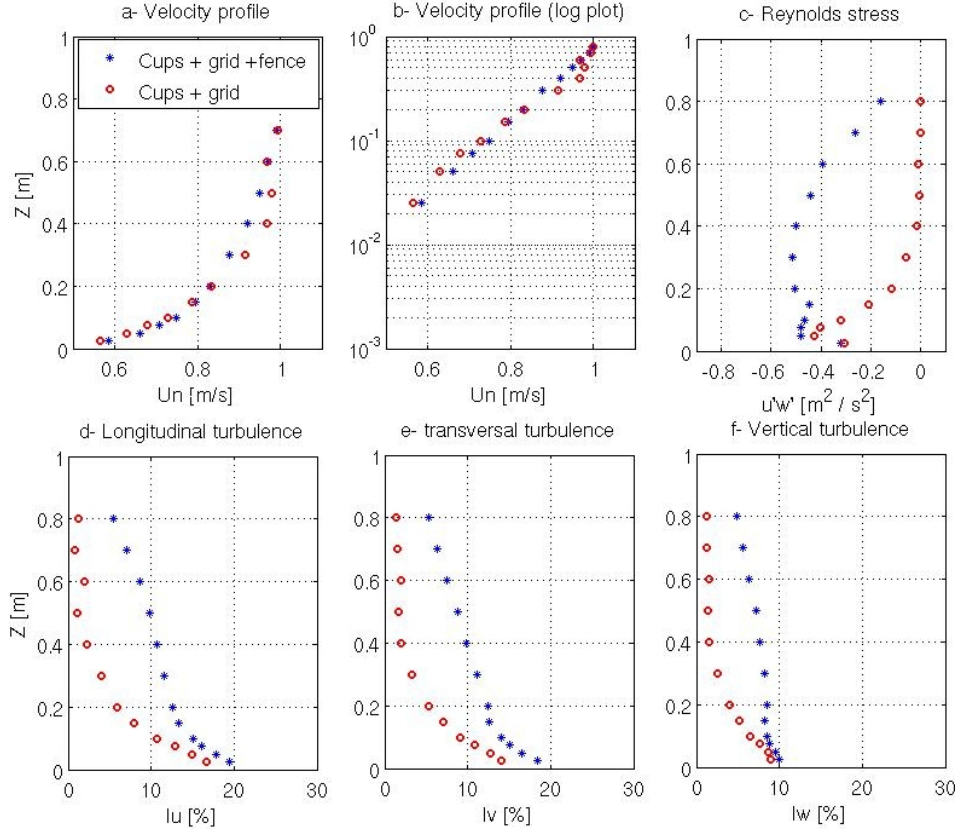
Figure 3.21.: Effect of the 0.15 m fence on the three components of the velocity and the turbulence. Study in VKI-L1 wind tunnel.
