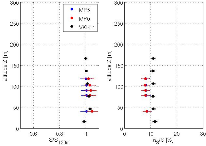
Figure 5.42.: Comparison of the velocity and turbulence profiles measured in the wind tunnel at position P4 with field data at MP0 and MP5 .
