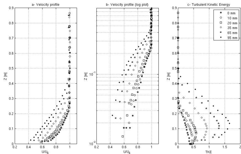
Figure 3.26.: Effect of the roughness height modelled by CFD.
