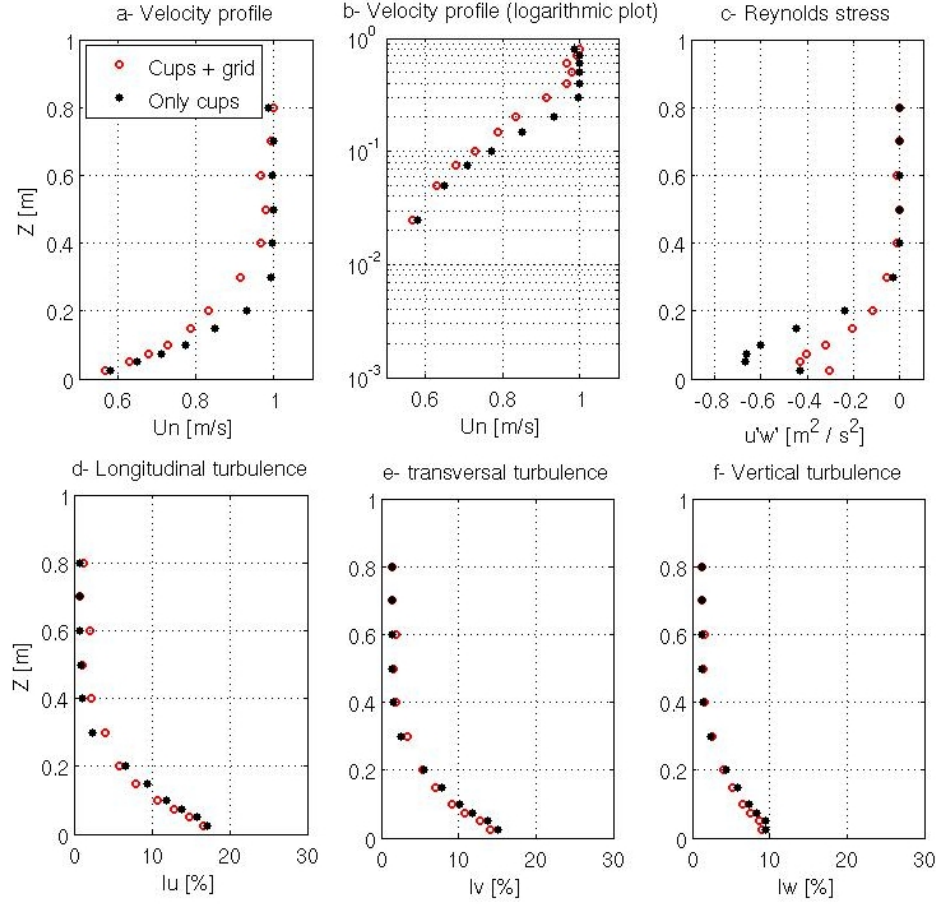
Figure 3.20.: Effect of the presence of the grid in VKI-L1 wind tunnel. Tree components measurements performed with a triple hot-wire A.2.2
