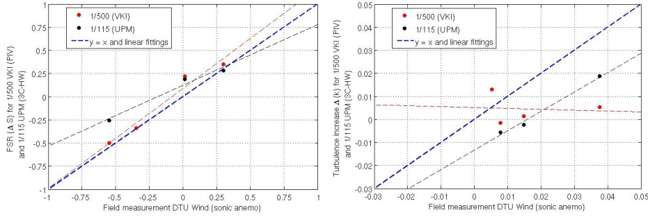
Figure 5.16.: Scatter plot of the FSR ( \Delta S ) (left) and the turbulent kinetic energy increase ( \Delta k ) (right) for the two wind tunnel experiments compare to the field measurements by sonic anemometers.
