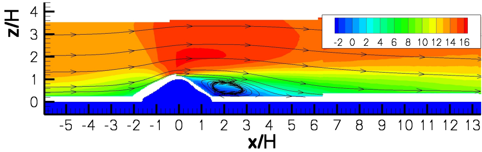
Figure 4.16.: The mean longitudinal velocity U [m/s] and the streamlines over the steep hill. Re \approx 17000 .
