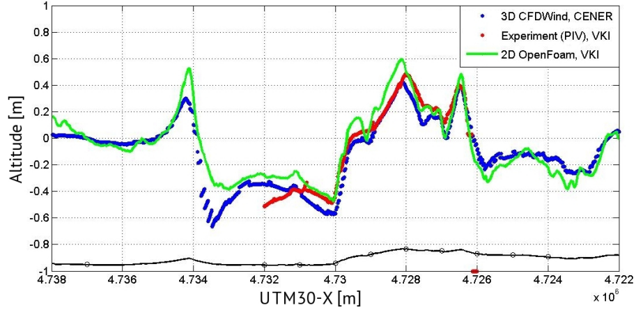
Figure 5.46.: Comparison of the FSR ( \Delta U ) at 90 m by experiments and 2D and 3D CFD computations.
