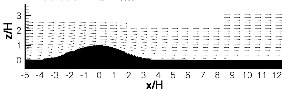
Figure 4.8.: The longitudinal wind velocity component U [m/s] and the streamlines over a low hill. Re \approx 16000 .
