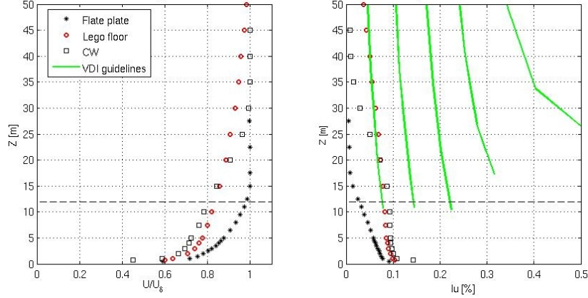
Figure 5.19.: The three different inlet conditions tested.
