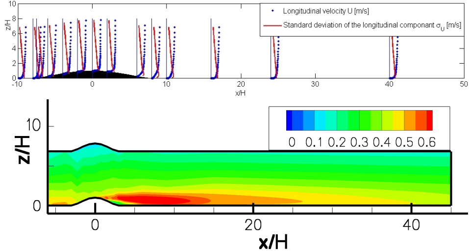
Figure 4.3.: Example of available data from an ERCOFTAC case [54]. Top: longitudinal velocity and longitudinal standard deviation component for a L = 8H hill. Bottom: contour line of the longitudinal standard deviation [m/s] for the L = 3H case obtained by linear interpolation.
