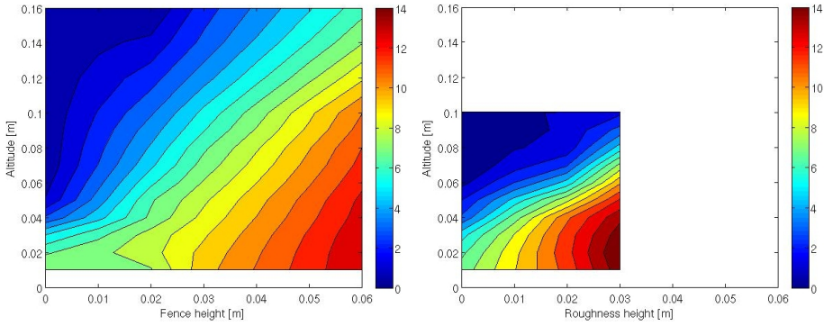
Figure 3.36.: Influence of the fence height (left) and of the roughness element height (right) on the longitudinal turbulence level.
