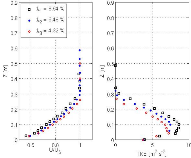
Figure 3.28.: Effect of the roughness density by CFD.
