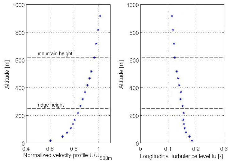
Figure 5.32.: Alaiz inlet conditions measured at position R1 .
