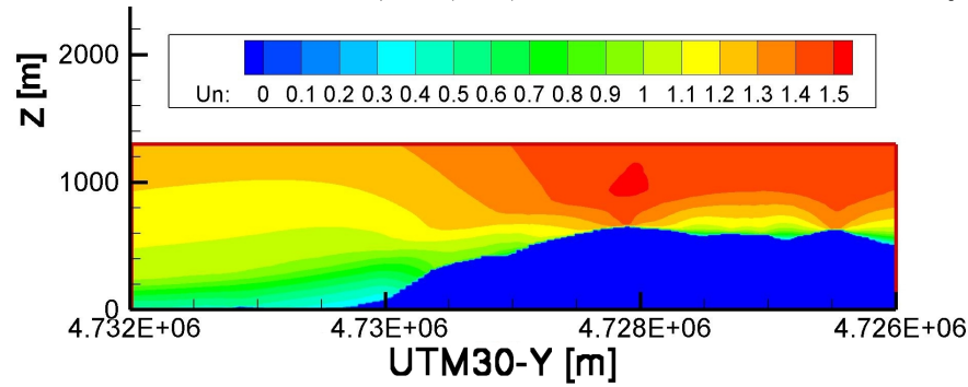
Figure 5.43.: Velocity ratio, U/U_{R1}(90m) , from the 2D CFD computation [63].
