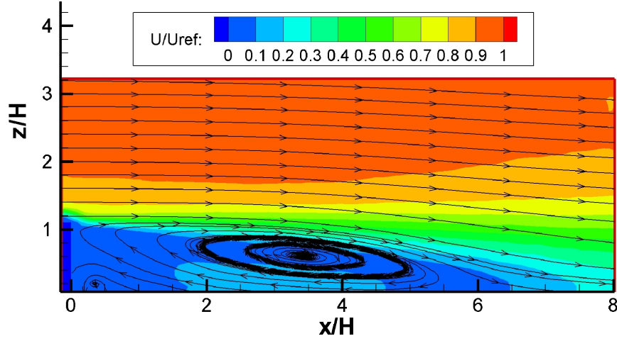
Figure C.4.: Time averaged velocity magnitude and velocity streamlines on the BFS at Re = 21800 [33].
