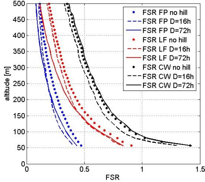
Figure 5.54.: FSR at the top of the mountain. Influence of the inlet conditions and of the position of the front ridge.
