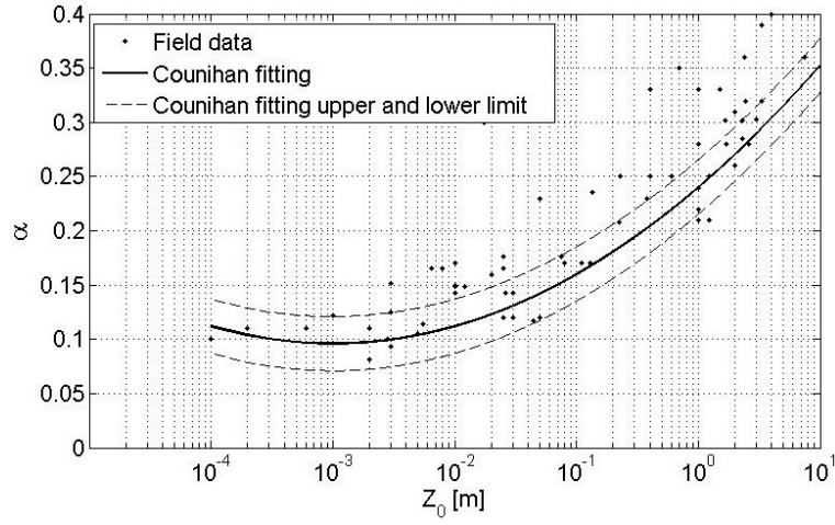
Figure 3.15.: Counihan [29] fitting of field data relating z_0 and \alpha .
