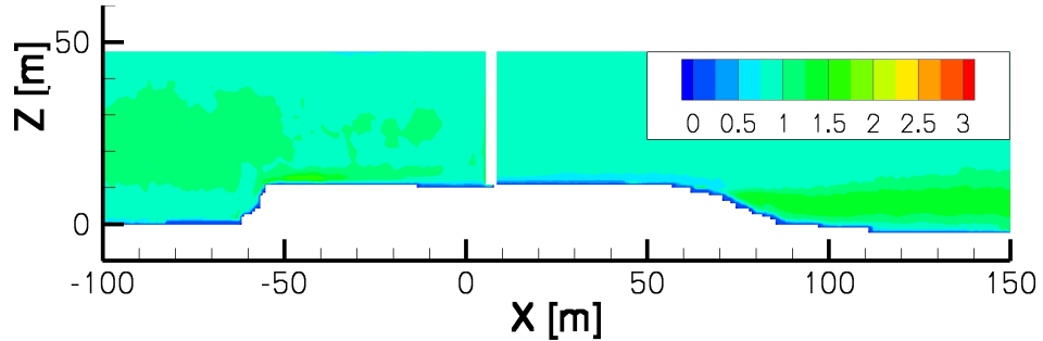
Figure 5.12.: Standard deviation of the longitudinal velocity component \sigma_U [m/s] around the hill.
