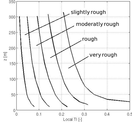
Figure 2.2.: The longitudinal turbulence intensity profile in function of the terrain roughness following the VDI guidelines.
