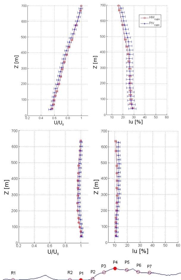
Figure 5.41.: Comparison of the normalized wind speed and the longitudinal turbulence intensity between PIV and HW profiles at positions P1 (top) and P4 (bottom). The reference speed U_0 is here defined at 100 m.
