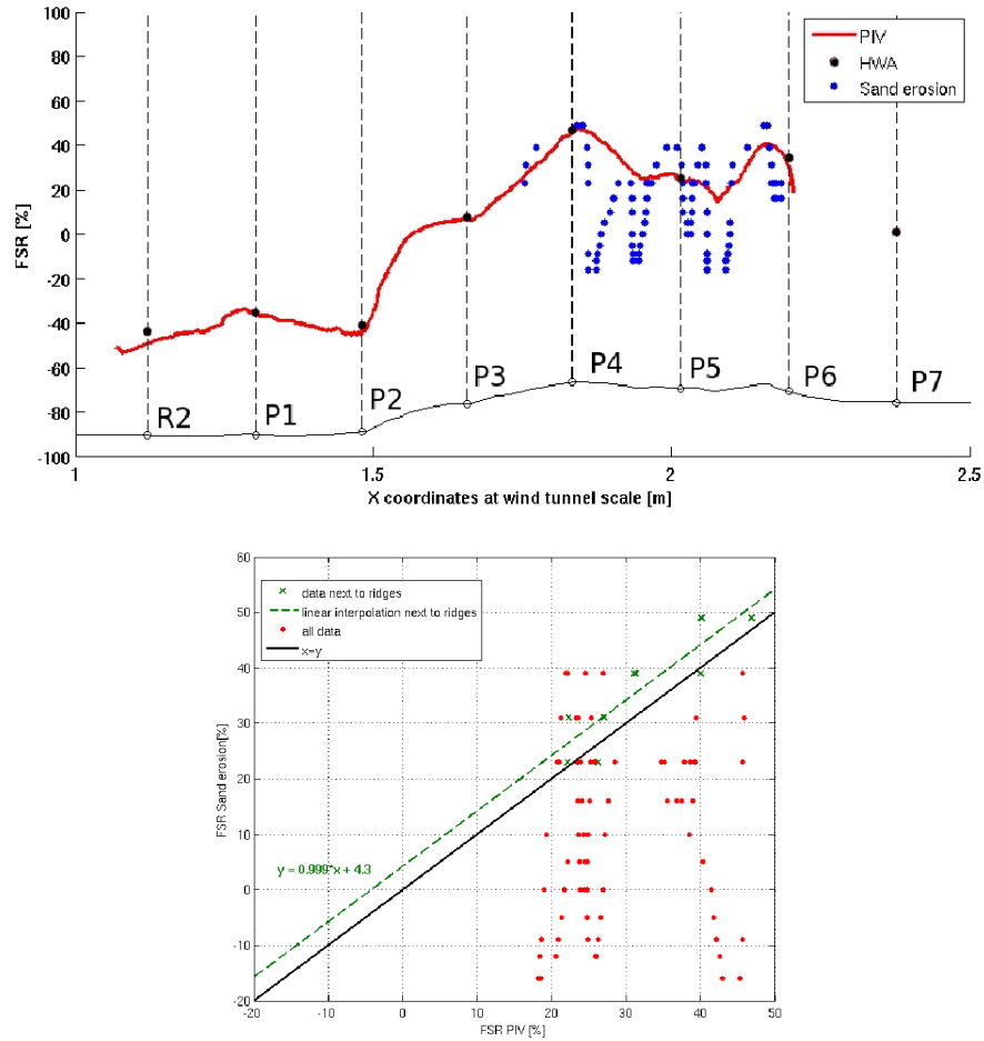
Figure C.11.: (top) Comparison between the fractional Speed-up Ratio calculated by PIV and extracted from the erosion technique. The FSR is plotted over the line described in Figure C.6. (bottom) Scatter plot between the PIV results and the sand erosion results.
