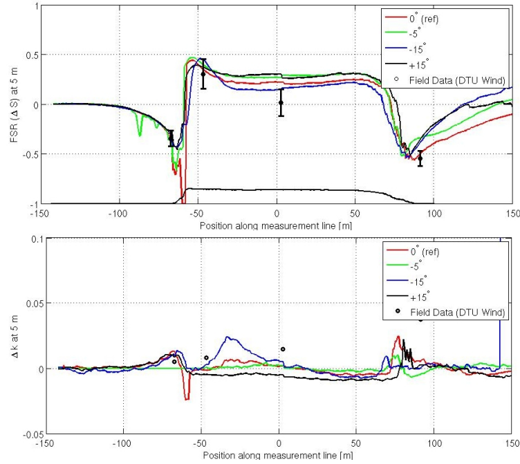
Figure 5.23.: \Delta S and \Delta k for different flow angles.
