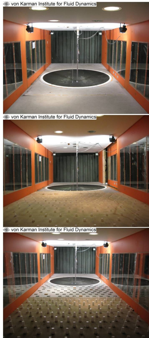
Figure 3.4.: View of the turntable of the wind tunnel with different boundary layer generators. Different terrain roughness can be simulated: offshore, rural or urban areas.
