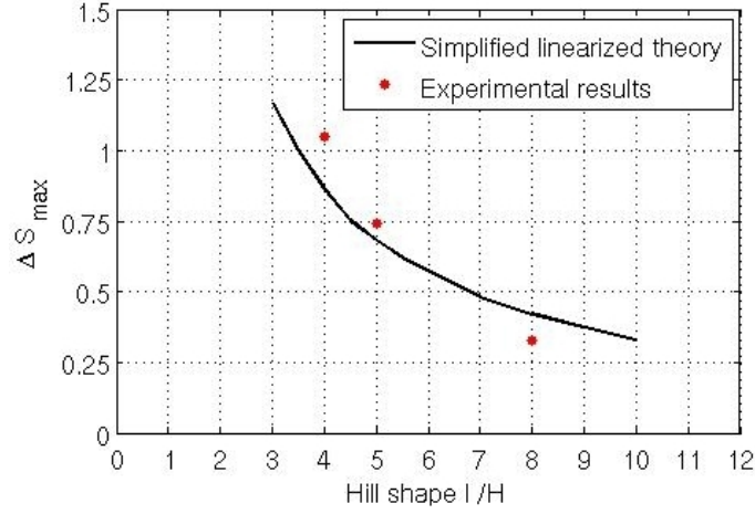
Figure 4.24.: Comparison between the maximum FSR ( \Delta S ) of the hills studied with the linearised theory from J-H, equation 4.7. Values are reported in table 4.2.
