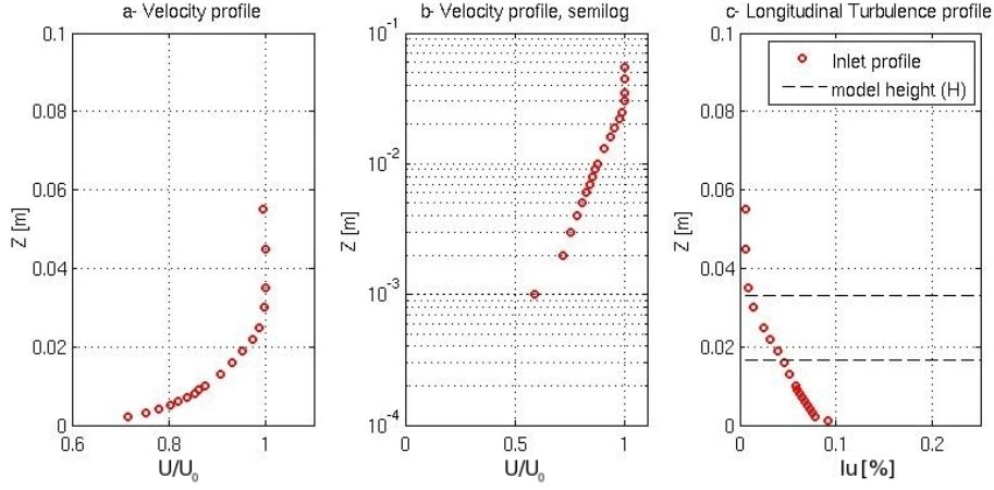
Figure 4.4.: Inlet velocity and longitudinal turbulence profile at the position of the hill. z_0 = 3.7210^{-6} m and u_* = 1.1 m/s. U_0 is the speed at the BL height \delta .
