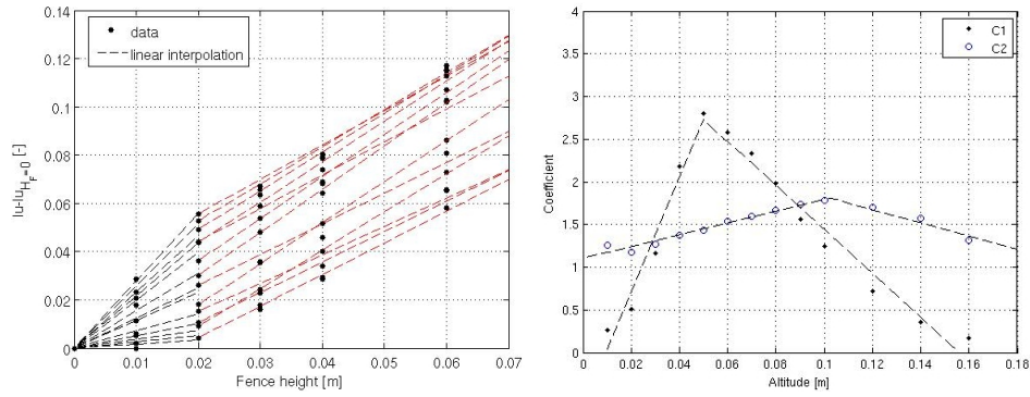
Figure 3.31.: Evolution of the longitudinal turbulence level ( I_u - I_{u_{H_F=0}} ) with the fence height H_F with a linear interpolation (left), and evolution of the linear interpolation coefficient with height (right).
