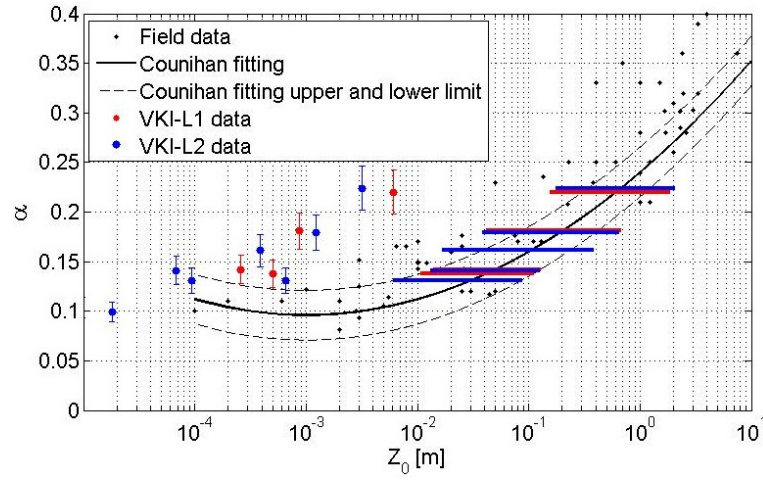
Figure 3.16.: Wind tunnel data added to the graph relating z_0 and \alpha , the red and blue points are the wind tunnel data without scaling and the red and blue lines are the possible scalings to fulfil Counihan fitting.
