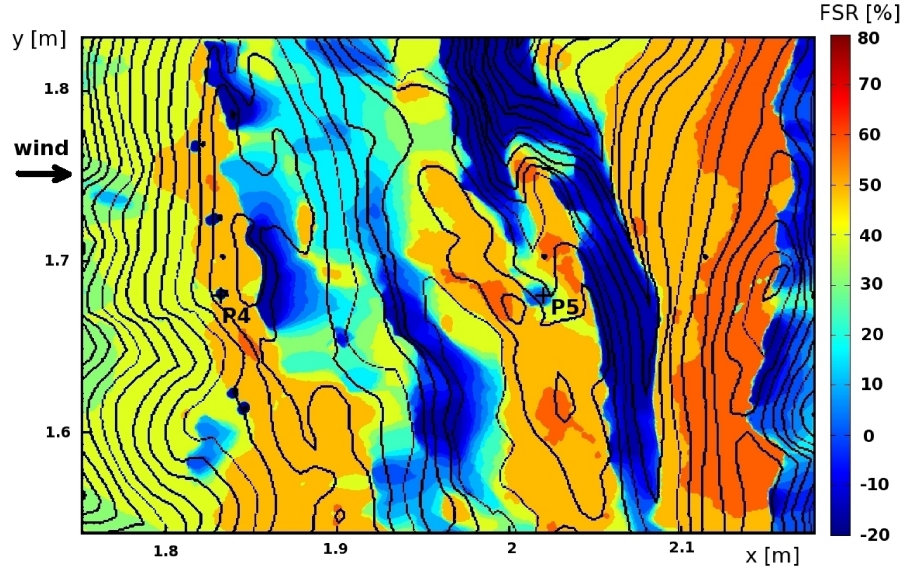
Figure 5.34.: Amplification factor map on Alaiz mountain, the dots are reference positions (masts). Axis are in meter at the wind tunnel scale (see figure 5.30)
