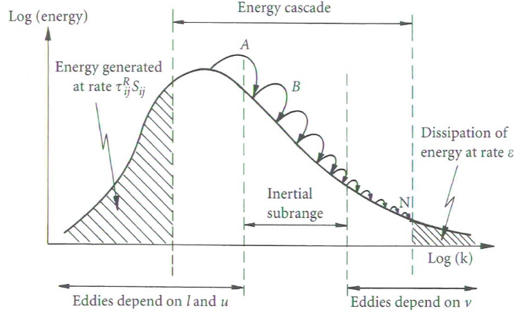
Figure 2.5.: The energy cascade (figure from Davidson [30]).
