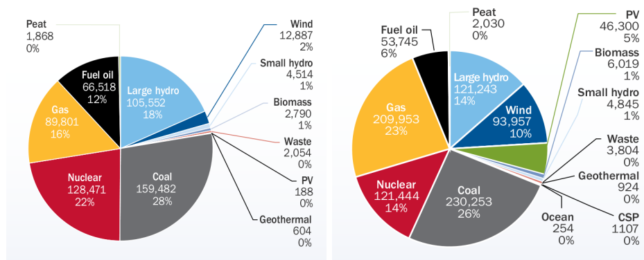
Figure 1.1.: EU power capacity mix in 2000 (left) and in 2011 (right).
