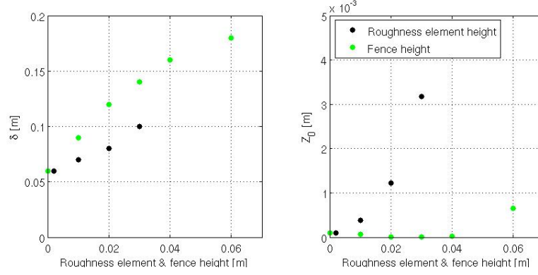
Figure 3.29.: Comparison of the effect of the fence height H_F and the roughness element height H_R on the BL height (left) and on the aerodynamic roughness length (right).
