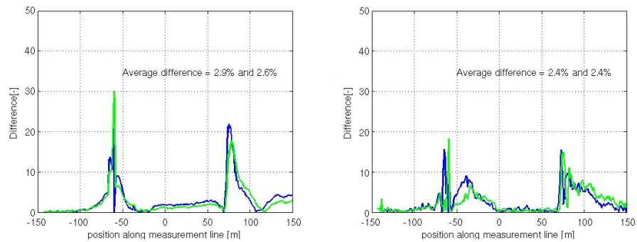
Figure 5.26.: Quantification of the effect of the reference height. Percentage of error along the terrain for the FSR (left) and the turbulence kinetic energy increase \Delta k (right).
