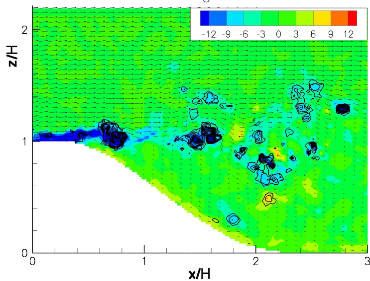
Figure 4.15.: Vortex detection in the near wake of the steep hill thanks to the vorticity field ( \omega_Y ) (flood), the \lambda_2 criteria (lines) and the instantaneous velocity field (vectors).
