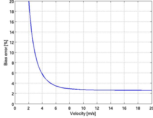
Figure A.7.: Typical bias error of hot-wire measurements in function of the local velocity.
