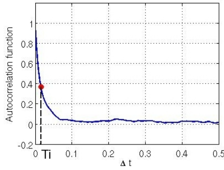
Figure 2.3.: Example of an autocorrelation function with the 1/e technique.
