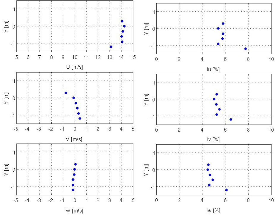
Figure 3.11.: Three velocity and turbulence intensity components of the test section transversal profile at h = 0.785 m above the turn-table of the VKI-L1 wind tunnel.
