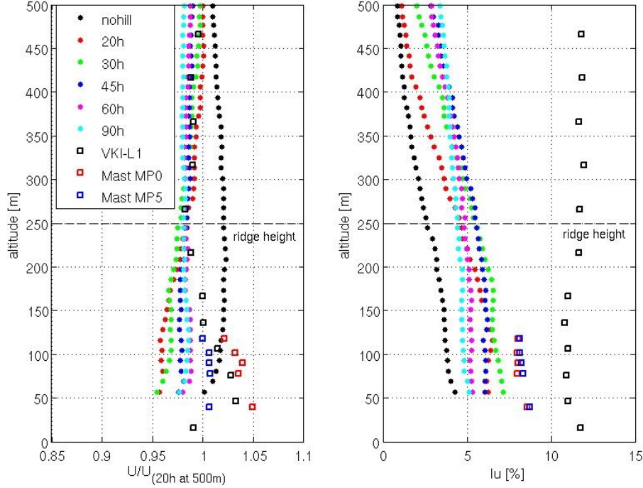
Figure 5.52.: Evolution of the velocity profile (left) and the longitudinal turbulence intensity (right) with increasing distance between the ridge and the mountain. Comparison with field data and experiment in VKI-L1 wind tunnel.
