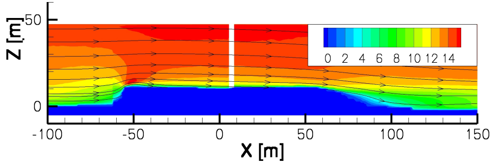
Figure 5.8.: Velocity field around Bolund hill. Velocity magnitude M [m/s] and velocity streamlines.
