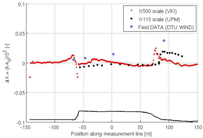
Figure 5.15.: Increase of turbulent kinetic energy at 5 m a.g.l. along Line B , comparison of field data with wind tunnel experiment.
