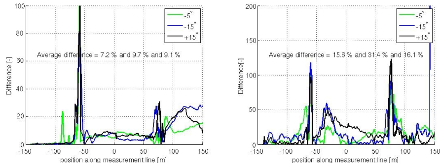
Figure 5.24.: Quantification of the effect of the flow angle. Percentage of error along the terrain for the FSR (left) and the turbulence kinetic energy increase \Delta k (right).
