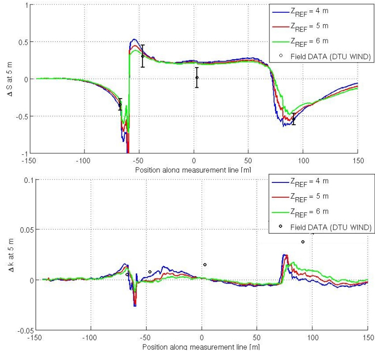
Figure 5.25.: \Delta S and \Delta k for different heights.
