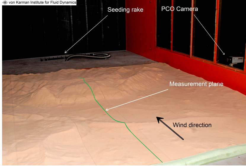
Figure 5.31.: The Alaiz mock-up in the test section with the PIV set-up.
