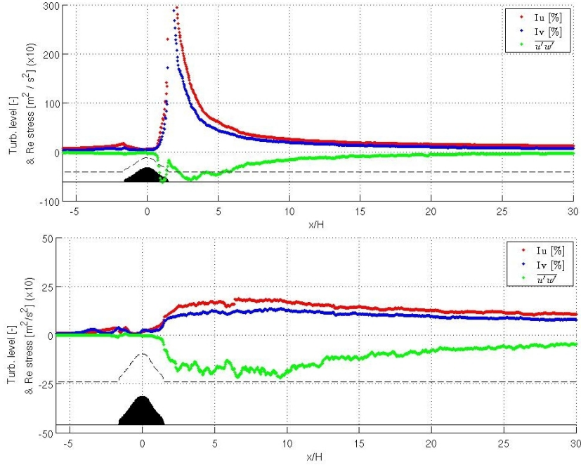
Figure 4.29.: Flow behaviour at z/H = 0.7 iso-height above the ground (top). The mean and fluctuating quantities near the surface are very much influenced by the presence of the hill (case V-2) in the near and far wake. Flow behaviour at z/H = 1.5 iso-height above the ground (bottom). At a higher altitude, the flow is weakly influenced by the presence of the hill.
