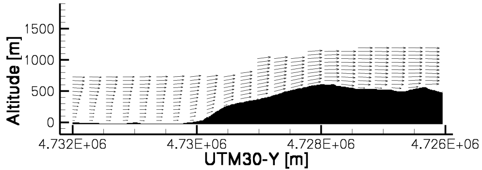
Figure 5.38.: Velocity vector field over Alaiz mountain at Re = 110000 .
