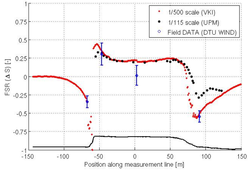
Figure 5.14.: FSR ( \Delta S ) at 5 m a.g.l. along Line B , comparison of field data with wind tunnel experiment.
