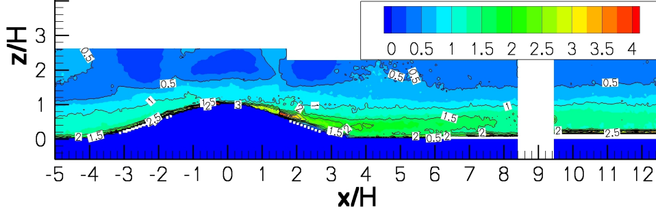
Figure 4.11.: The horizontal standard deviation of the velocity \sigma_U [m/s] over a low hill.
