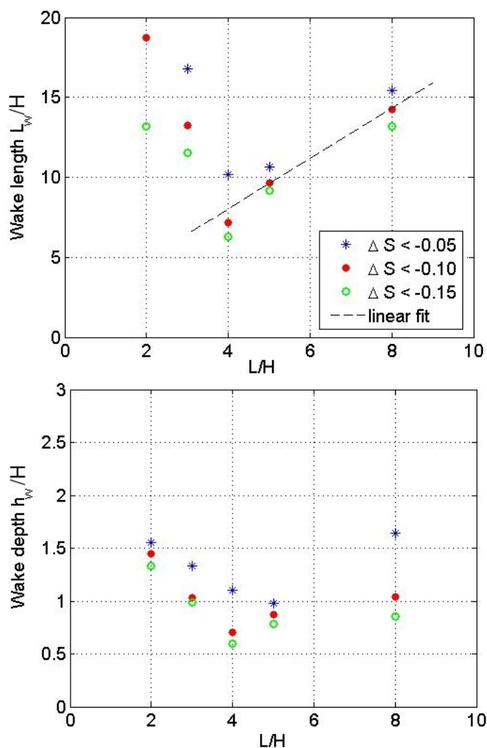
Figure 4.26.: The wake size is approximated by the distance where \Delta S = -0.15 , \Delta S = -0.10 or \Delta S = -0.05 . Top: wake longitudinal extension ( l_w ) in function of the hill aspect ratio ( L/H ). Bottom wake depth ( h_w ) in function of the hill aspect ratio ( L/H ).
