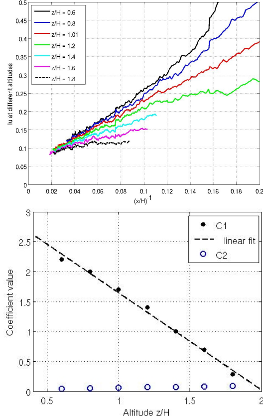
Figure 4.30.: Top: the turbulence level Iu evolution with the inverse of the distance for different height (hill “V-2”). Bottom: the evolution of the coefficients of the 1/x fitting with altitude.
