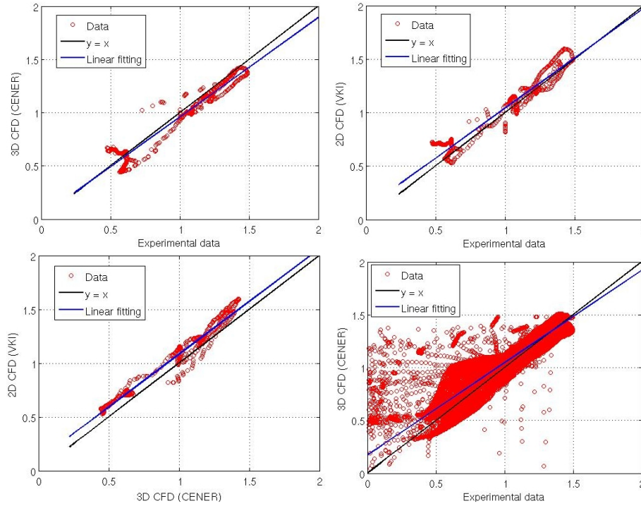
Figure 5.48.: Scatter plot for the comparison between experimental results and 2D and 3D CFD.
