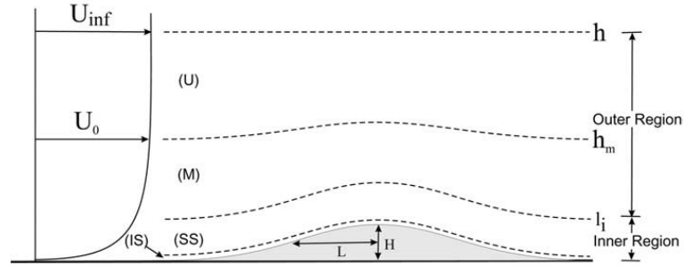
Figure 4.1.: Flow over two-dimensional low hill. Figure from [6]
