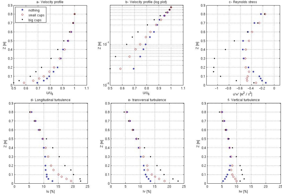
Figure 3.25.: Effect of the roughness height in the three components, study with a triple hot-wire in VKI-L1 wind tunnel.
