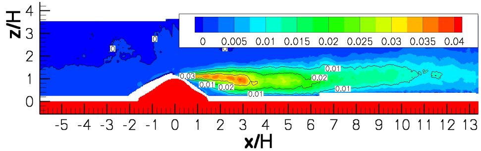
Figure 4.20.: The vertical standard deviation of the wind velocity \sigma_W [m/s] around the steep hill.
