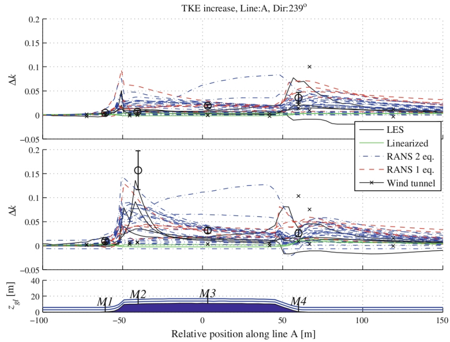
Figure 5.5.: Comparison of the turbulence increase \Delta k computed by linearised models, CFD, measured by wind tunnel experiments and measured in the fields (black dots) at 2 m and 5 m on the “line A”. From [8].
