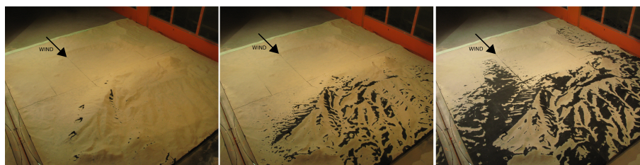
Figure C.1.: Example of a model at the beginning of the test (left) after 1 min at 6 m/s (middle) and after 1 minute at 7 m/s (right).
