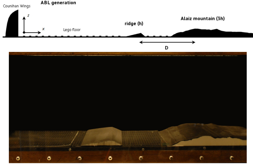
Figure 5.50.: Experimental set-up (top) and picture of the 2D model of Alaiz in the wind tunnel (bottom).
