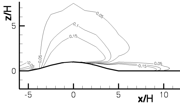
Figure 4.23.: Example of the velocity speed-up ( \Delta S ) on the top of the L=5H hill.
