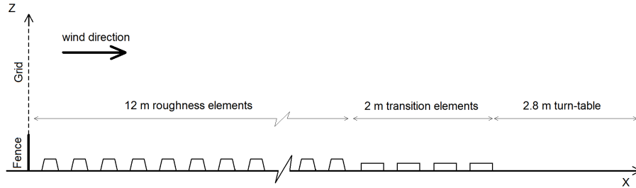
Figure 3.2.: Boundary layer generation set-up in VKI-L1 test section.
