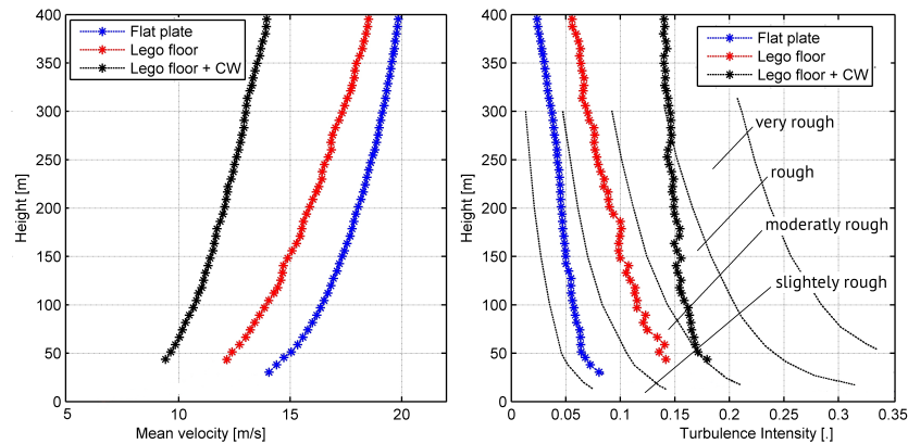
Figure 5.53.: Inlet profiles in the wind tunnel with VDI guidelines categories.
