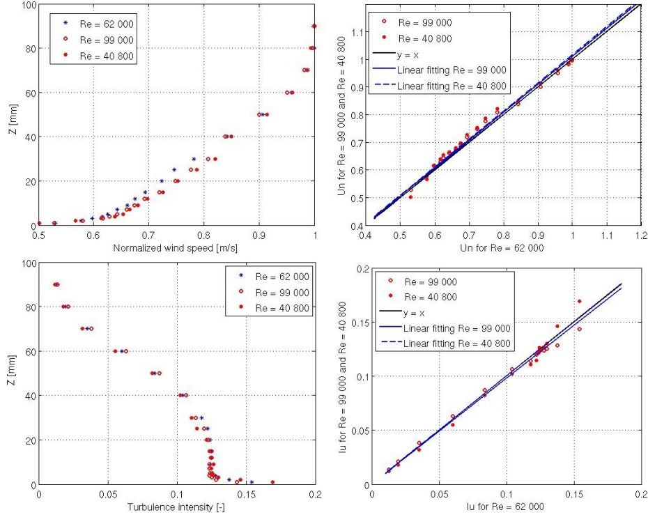
Figure 3.8.: Presentation of the Reynolds number dependency in VKI-L2 test section. Comparison of the normalized velocity profile (upper left) with the scatter plot (upper right) and of the turbulence profile (lower left) with scatter plot (lower right).
