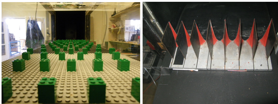
Figure 3.6.: View of the VKI-L2 wind tunnel test section with Lego floor, blocks and Counihan wings.
