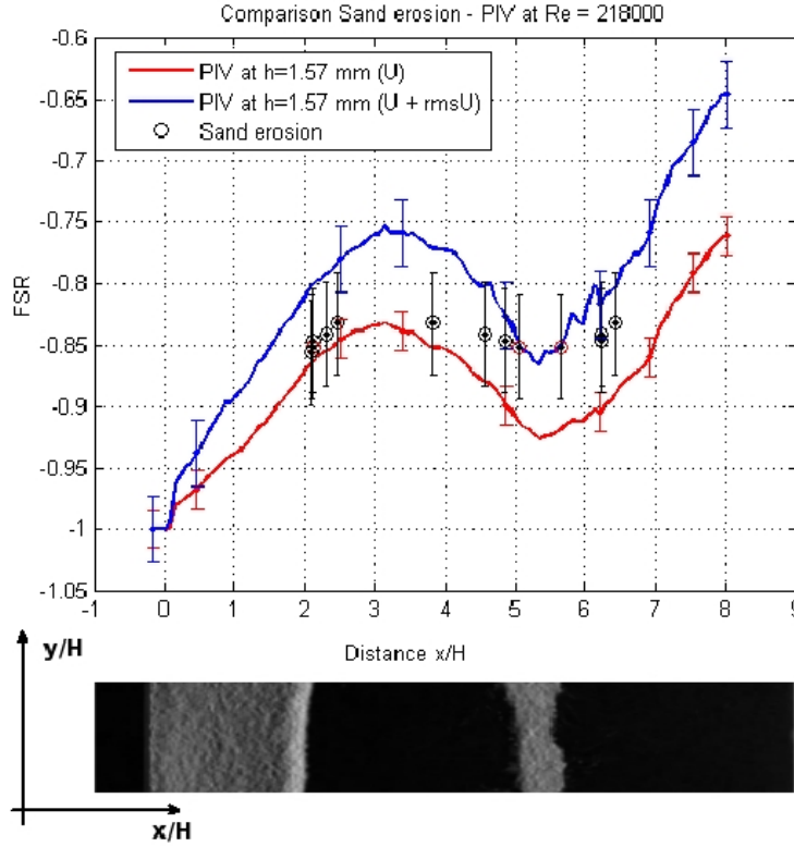
Figure C.5.: Comparison of the FSR computed from PIV measurements and from sand erosion tests (top). Top view of the sand erosion pattern after 1 min at 17 m/s (bottom).
