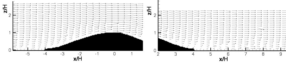
Figure 4.6.: The instantaneous velocity field around a low hill (V-4).
