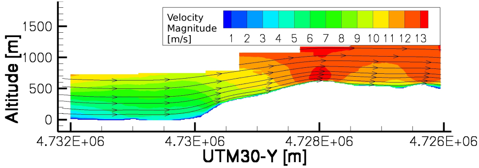
Figure 5.35.: Mean velocity magnitude field and velocity streamlines over Alaiz mountain at Re = 110000 .
