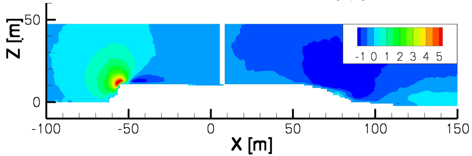
Figure 5.10.: Vertical wind speed W [m/s].
