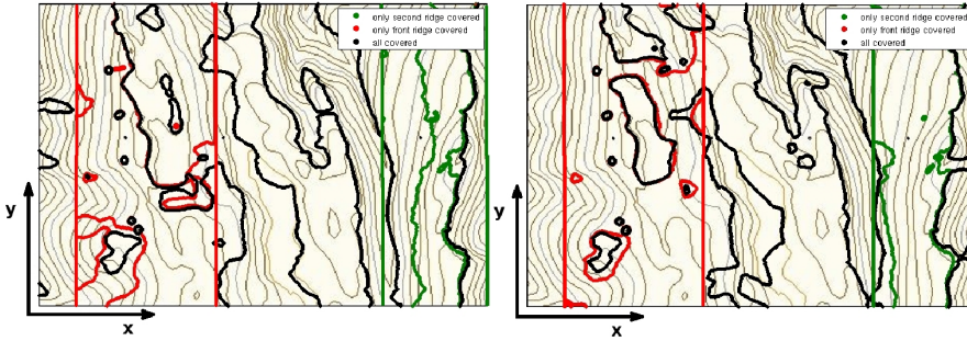
Figure C.9.: Effect of the area covered at two velocities: 4.29 m/s (left) and 4.79 m/s (right). Only first ridge covered (red), only second ridge covered (green) and all area covered (black).
