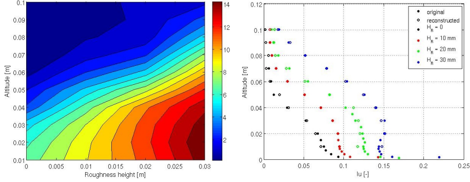
Figure 3.35.: Contour map of the longitudinal turbulence level in function of the altitude and the roughness height [%] (left). Comparison between the original and reconstructed turbulence intensity profiles (right).
