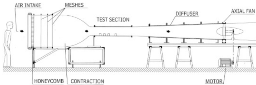
Figure 3.5.: VKI-L2 wind tunnel in the wind engineering configuration.
