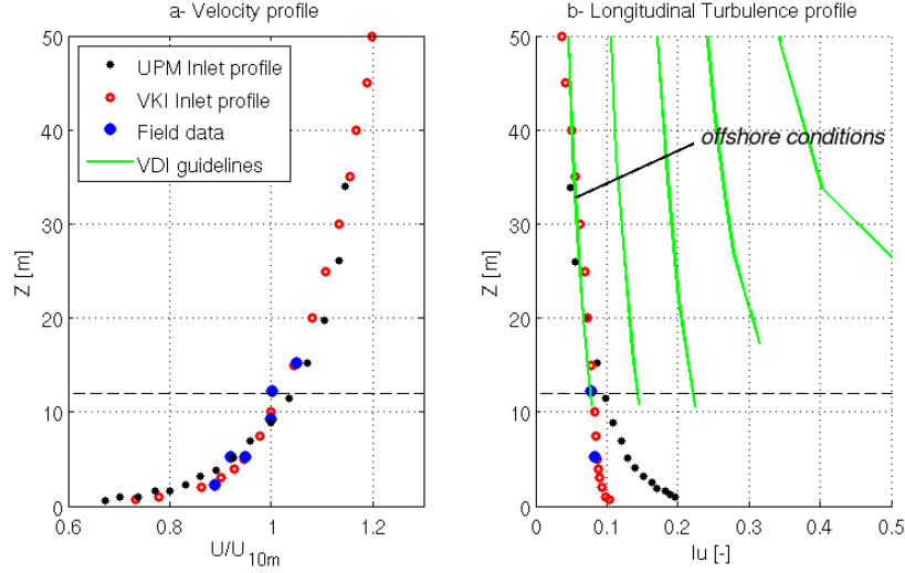
Figure 5.7.: Bolund inlet conditions: velocity (left), longitudinal turbulence profile (right), comparison with VDI guidelines (green), field measurements (blue), and inlet conditions in the UPM wind tunnel (black).
