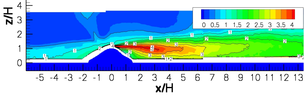
Figure 4.19.: The longitudinal standard deviation of the wind velocity \sigma_U [m/s] around the steep hill.
