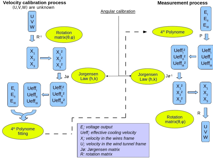
Figure A.6.: Summary of the calibration and the measurement procedure for three components HWA.
