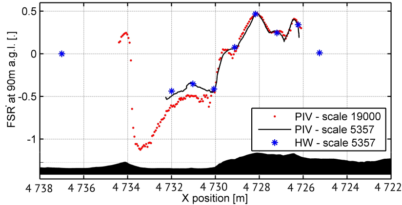
Figure 5.51.: FSR obtained over the Alaiz mountain from wind tunnel testing in VKI-L1 at 1/5357 scale and in VKI-L2 at 1/19 000 scale. The test performed in VKI-L2 wind tunnel uses the Flate Plate inlet conditions (FP).
