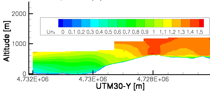
Figure 5.44.: Velocity ratio, U/U_{R1}(90m) , from the 3D CFD computation performed by CENER [17].
