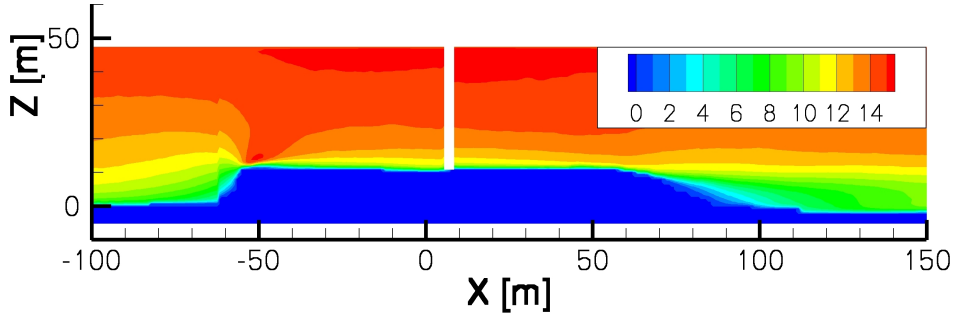
Figure 5.9.: Longitudinal wind speed U [m/s].
