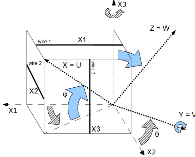
Figure A.5.: Wire frame ( X_1, X_2, X_3 ) and probe frame ( X, Y, Z ) of the DANTEC 55P91 triple wire probe.
