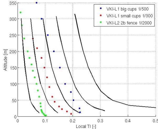
Figure 3.17.: Turbulence intensity profile in the wind tunnels. Possible scales for different configurations.
