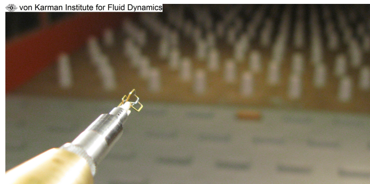
Figure A.4.: Picture of the 3C HWA probe measuring the ABL in L1 test section.
