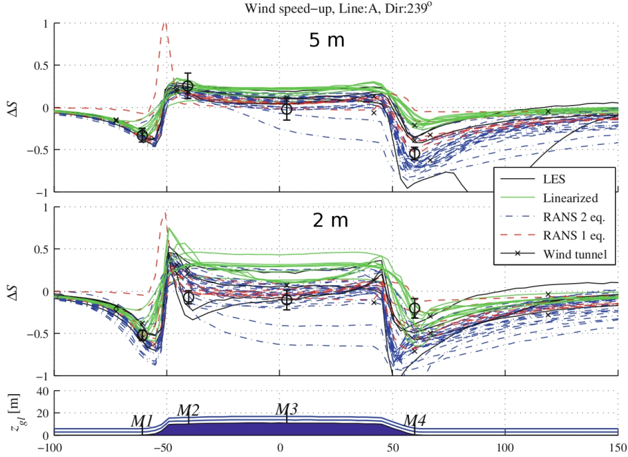
Figure 5.4.: Comparison of the FSR ( \Delta S ) computed by linearised models, CFD, measured by wind tunnel experiments and measured in the fields (black dots) at 2 m and 5 m on the “line A”. From [8].
