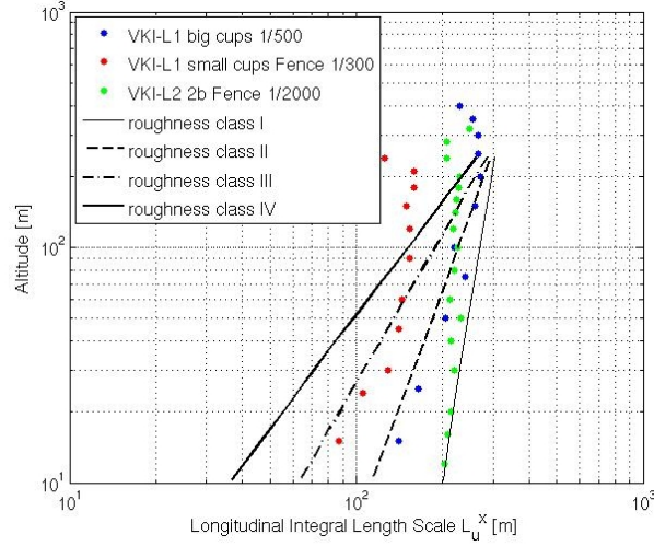
Figure 3.18.: Integral length scale profile in the wind tunnels.
