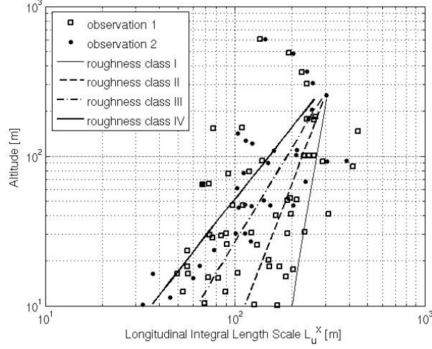
Figure 2.4.: Integral length scale profile observed in the field and approximation proposed by Counihan [29].
