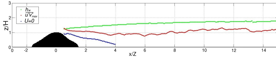
Figure 4.22.: Measurement of the recirculation area (blue), the wake height (green) and the height of the maximum Reynolds stress (red) after a steep hill in function of the distance.
