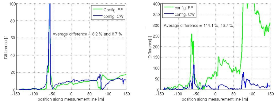
Figure 5.21.: Quantification of the effect of the inlet conditions. Percentage of error along the terrain for the FSR (left) and the turbulence kinetic energy \Delta k increase (right).
