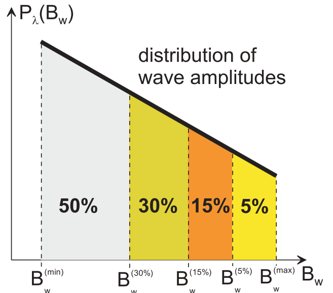
Figure 2. The scheme of the four part separation of the B_w distribution.
