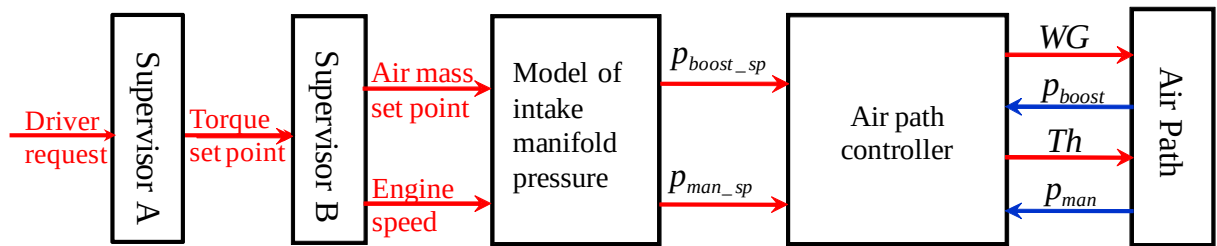
Fig.1.24 Scheme of gasoline engine control
