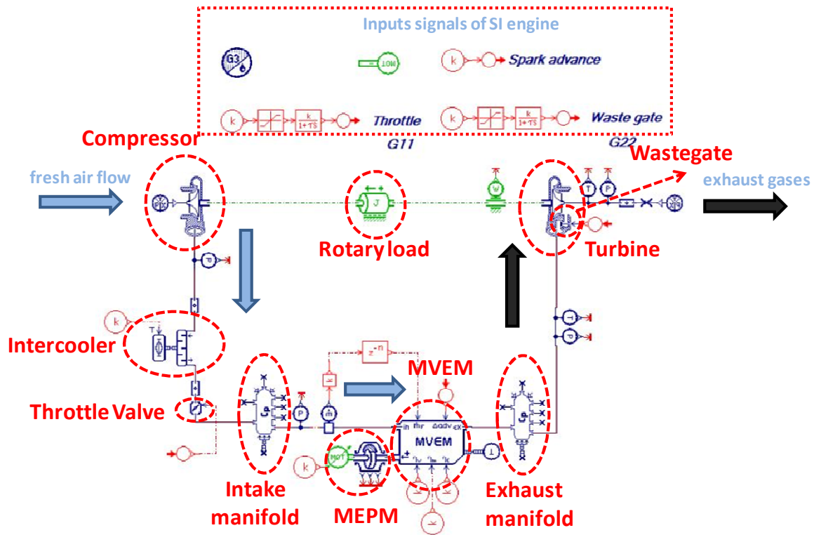
Fig.3.6 Air path model of a turbocharged gasoline engine
