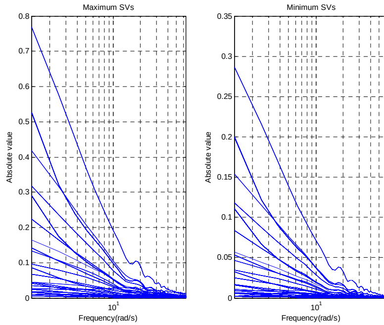
Fig.3.18 SVs of 2x2 crossing MIMO system for two loops
