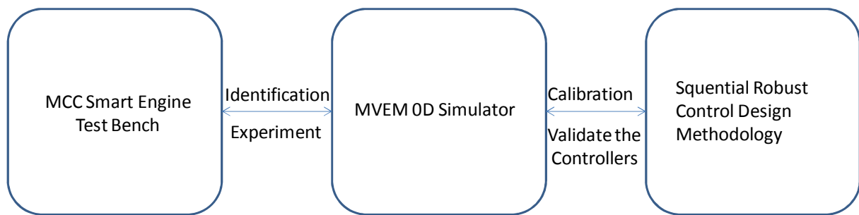
Fig.3.7 Interaction in different models for gasoline engine control
