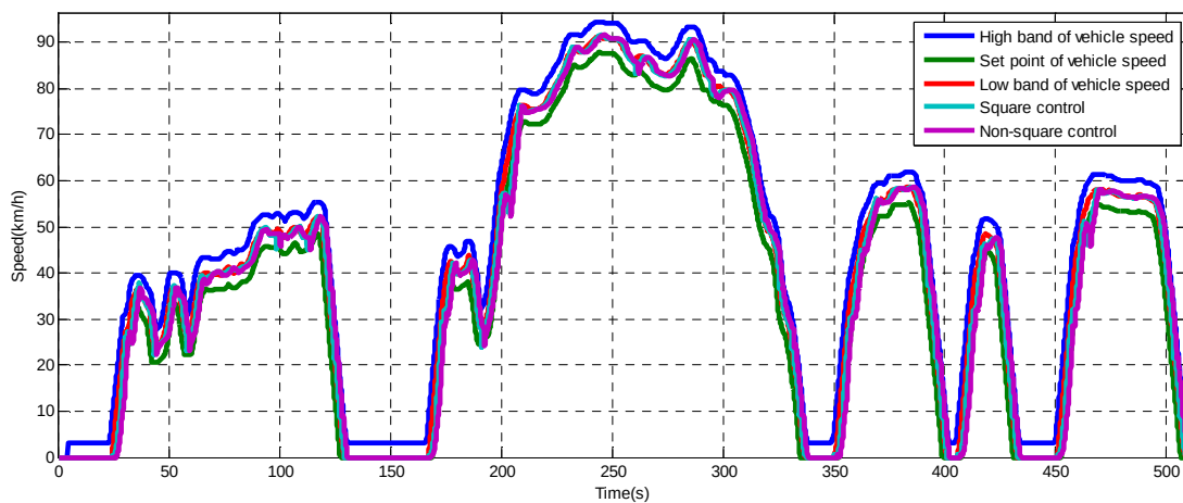
Fig.4.44 The vehicle speed response in FTP 75 Test Cycle: square and non-square control
