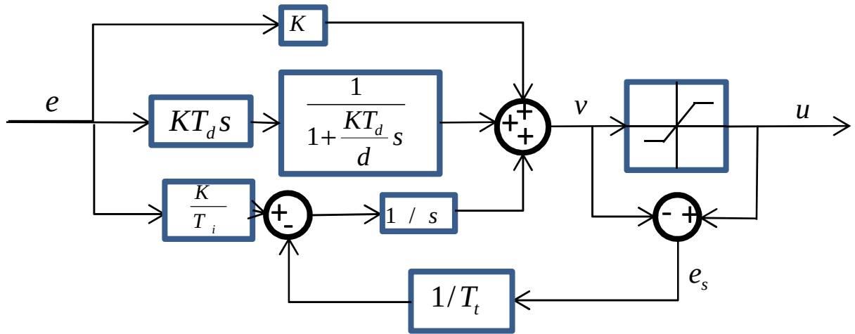
Fig.2.18 PID Anti-windup
