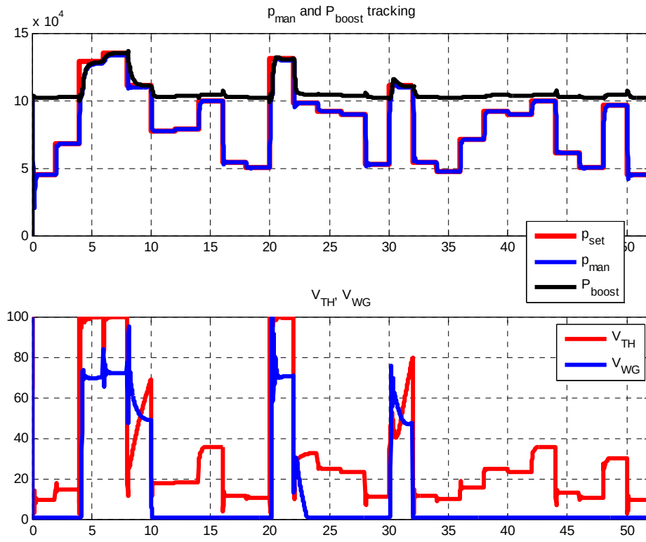
Fig.3.32 p_{man} and p_{boost} (top), V_{WG} and V_{EGR} (bottom) at 3000 rpm
