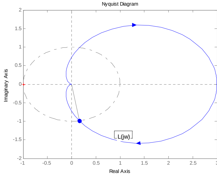
Fig.2.21 Nyquist stability theorem. in this diagram, n_c = n_+ = n_0 = 0 .
