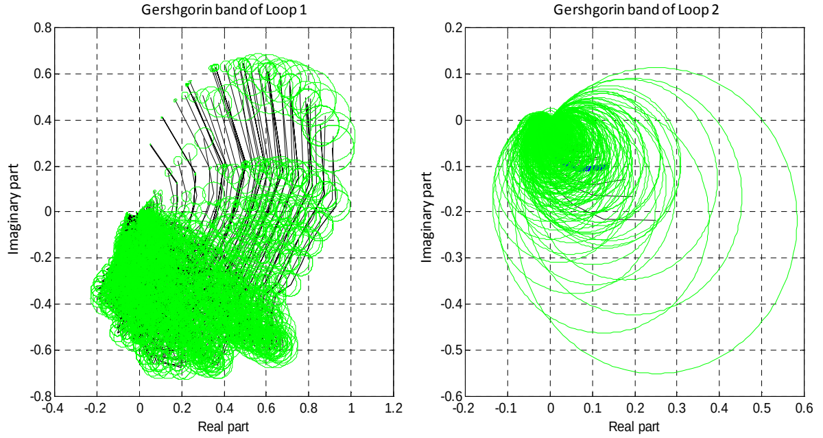
Fig.3.23 GB of open-loop 2x2 MIMO system for two loops (gasoline)
