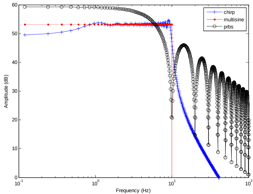
Fig.2.8 Responses of three signal excitations
