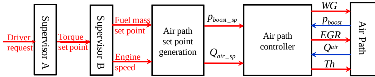
Fig.1.25 Scheme of diesel engine control with Waste-gate (WG) turbocharger
