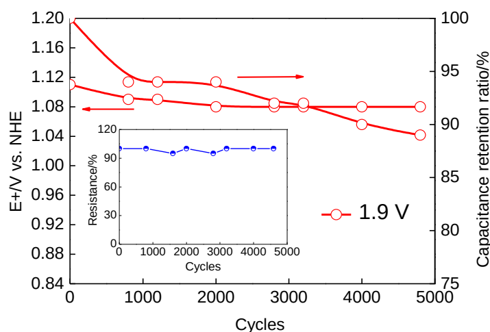
Figure 45 Capacitance retention ratio ( C_n/C_1 \cdot 100 , where C_n is the capacitance at n^{\text{th}} cycle and C_1 at 1^{\text{st}} cycle) or maximum potential ( E^+ ) of the positive electrode vs. NHE during galvanostatic ( 200 \text{ mA g}^{-1} ) cycling of a symmetric ACH/ACH supercapacitor. Electrolyte: 2 \text{ mol L}^{-1} \text{ Li}_2\text{SO}_4 . Inset: resistance variation ratio ( R_n/R_1 \cdot 100 , where R_n is the resistance at n^{\text{th}} cycle and R_1 at 1^{\text{st}} cycle).
