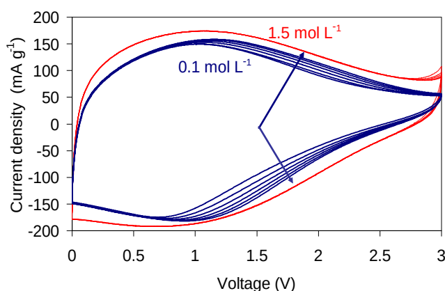
Figure 14 Cyclic voltammograms (CVs, 5 \text{ mV s}^{-1} ) for symmetric PC/PC capacitors in 0.1 and 1.5 \text{ mol L}^{-1} tetraethylammonium tetrafluoroborate solutions [65].
