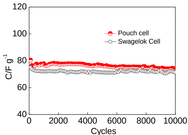
Figure 56 Evolution of discharge capacitance during galvanostatic ( 1 \text{ A g}^{-1} ) cycling of symmetric ACX/ACX Swagelok and pouch cells operating at 2.1 V in 2 \text{ mol L}^{-1} \text{ Li}_2\text{SO}_4 electrolyte.
