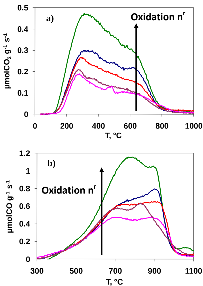
Figure 59 Gases evolved during the TPD analysis of cellulose-based carbons oxidized by \text{H}_2\text{O}_2 after different numbers of oxidation/thermal treatment cycles a) \text{CO}_2 ; b) \text{CO} .
