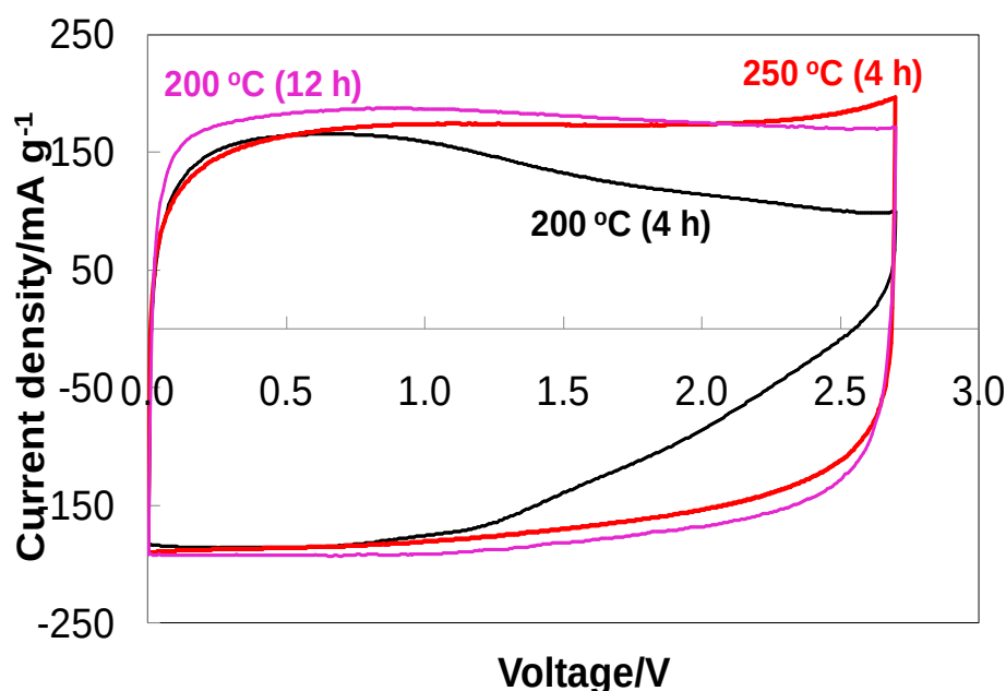
Figure 69 Cyclic voltammograms ( 5 \text{ mV s}^{-1} ) of supercapacitors using carbons prepared by oxidation/desorption at different oxidation temperatures or times. Electrolyte: 1 \text{ mol L}^{-1} TEABF 4 in acetonitrile.
