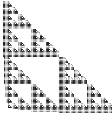
(b) Version auto-assemblante [Lathrop et al. 2009, Fig. 2].
