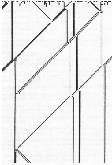
Figure 4: The k = 4 , r = 2 universal cellular automaton of table 4 simulated starting from a random initial state. The symbols 0, 1, 2, 3, and 4 are represented by
