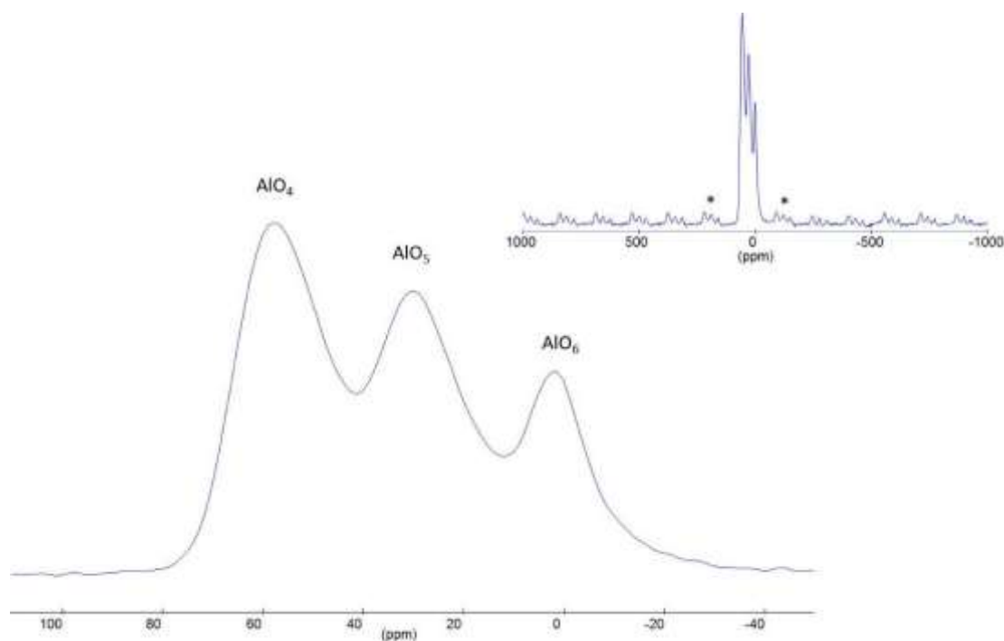
Figure 147. Spectres ^{27}\text{Al} MAS du verre BAlLa ( B_0=17,6 T, \nu_r=33 kHz).
