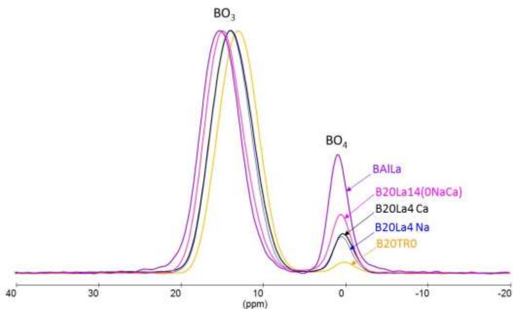
Figure 92. Spectres RMN MAS ^{11}\text{B} des verres B20TRO, B20La4Na, B20La4Ca, SiAlLa, BAlLa ( B_0=18,8\text{ T} , \nu_r=20\text{ kHz} ).
