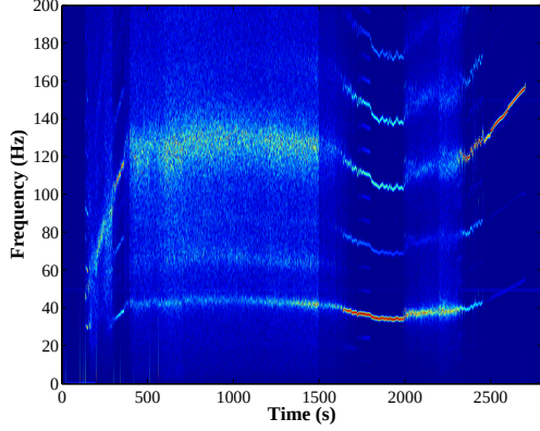
Figure 4.40: Fourier spectrogram of the AC component for a Krypton plasma.
