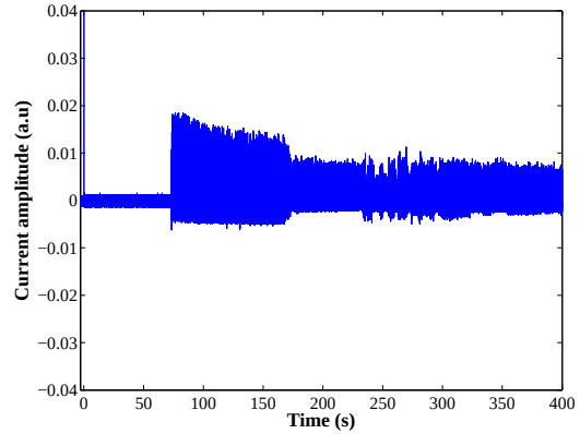
Figure 4.39: Amplitude of the RF current (AC component) for an Argon plasma.
