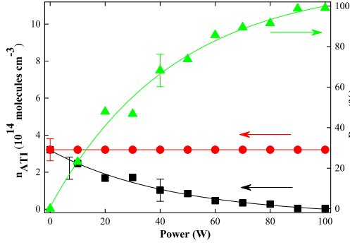
Figure 7.5: Concentration of ATI with - \blacksquare and without - \bullet plasma operation as well as the degree of dissociation - \blacktriangle as a function of the discharge power in an Ar/ATI plasma, p = 6 Pa, ratio Ar/ATI = 2/1.
