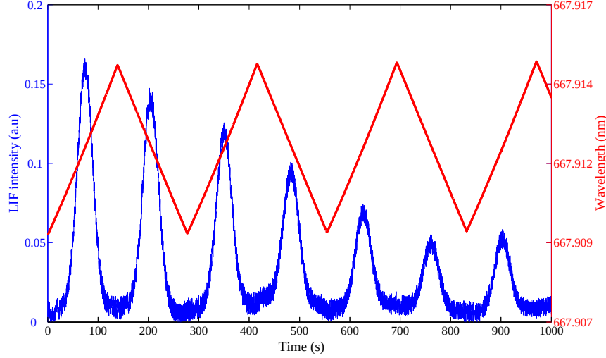
Figure 6.3: Evolution of the fluorescence as a function of the wavelength, for different positions with different properties in the bulk.
