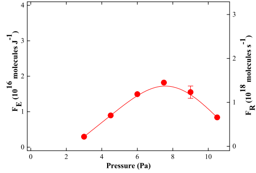
Figure 7.8: Fragmentation efficiency and fragmentation rate, both - ●, of ATI as a function of the total pressure in an Ar/ATI plasma. P_{\text{Plasma}} = 80 W, gas ratio Ar/ATI= 2/1.
