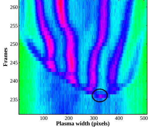
Figure 5.11: Line profile of plasma glow at the vicinity of the electrode showing the appearance of a spheroid and then its splitting (16000 fps).
