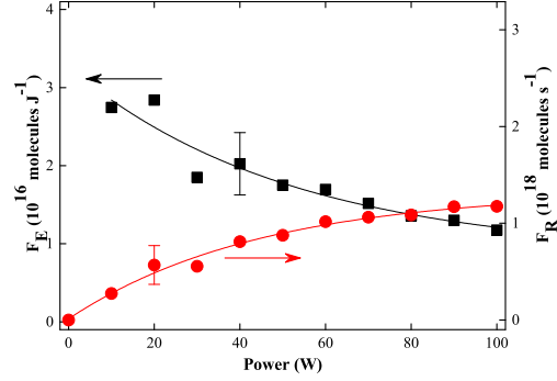
Figure 7.6: Fragmentation efficiency F_E - \blacksquare and fragmentation rate F_R - \bullet of ATI as a function of the discharge power in an Ar/ATI plasma. p_{total} = 6 Pa, ratio Ar/ATI = 2/1.
