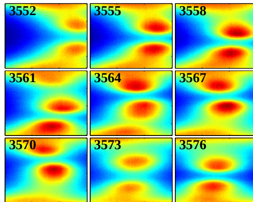
Figure 5.14: Interaction between plasma spheroids leading to the up and down motion of the central spheroid. The central spheroid moves in the direction of the other spheroids. Frames from a movie taken at 16000 fps and presented in false colors from dark blue to red. Each image is about 2.3 cm height and 1 cm width.
