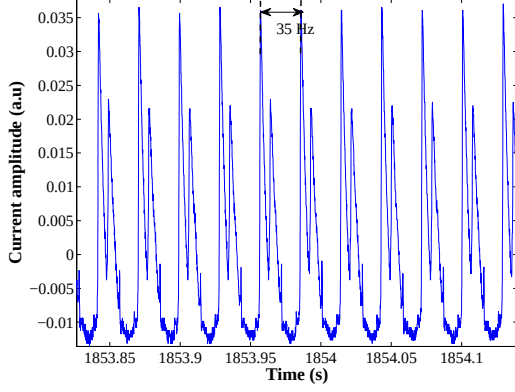
Figure 4.8: A part of the electrical signal during the frequency drop regime.
