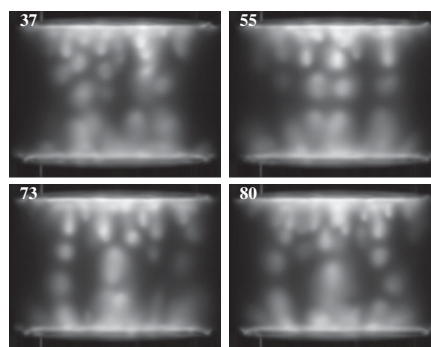
FIG. 1. Plasma spheroids in the plasma bulk. Well-defined regions with an enhanced emission are clearly observed in between the electrodes (dark regions on the top and bottom separated by 3 cm). The numbered frames are from a movie taken at 8000 fps [27].
