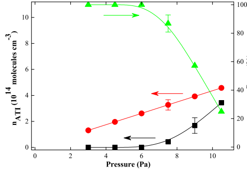
Figure 7.7: Concentration of ATI with - ■ and without - ● plasma operation as well as the degree of dissociation - ▲ as a function of the total pressure in an Ar/ATI plasma. P_{\text{Plasma}} = 80 W, gas ratio Ar/ATI= 2/1.
