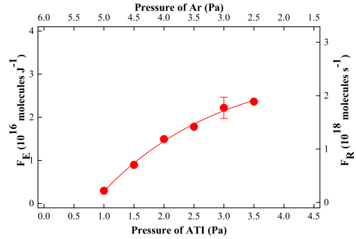
Figure 7.10: Fragmentation efficiency and fragmentation rate, both - ●, of ATI as a function of the mixing gas ratio of Ar and ATI. p_{\text{total}} = 6 Pa and P_{\text{plasma}} = 80 W.
