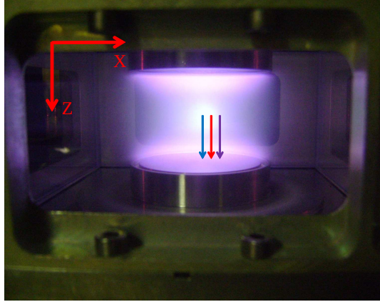
Figure 6.10: Enhanced emission of the central void in an argon plasma. The three arrows show the measurement positions and directions.
