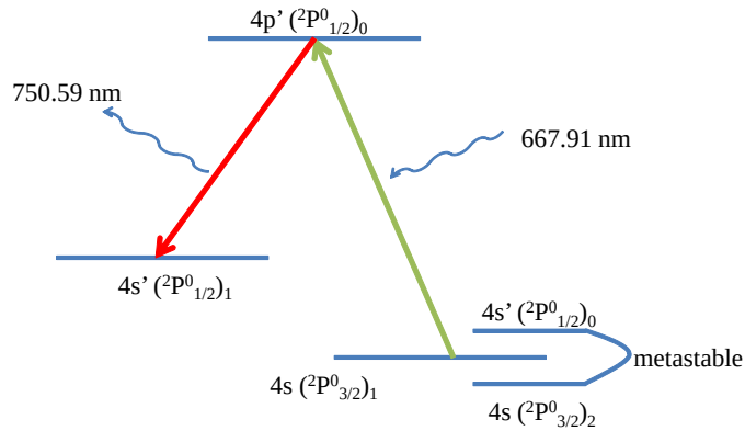
Figure 3.6: Diagram of argon LIF scheme.
