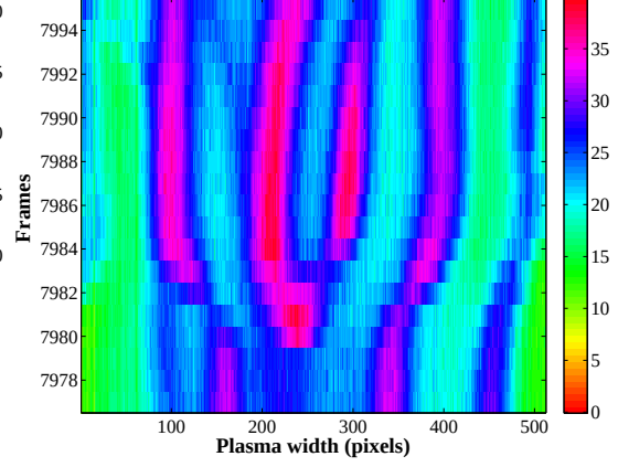
Figure 5.12: Line profile of plasma glow at the vicinity of the electrode showing spheroid appearances and their trajectories (16000 fps).
