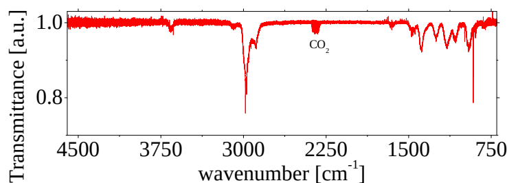
Figure 7.2: Spectrum of ATI measured at 2 Pa with a resolution of 0.075\text{ cm}^{-1} .
