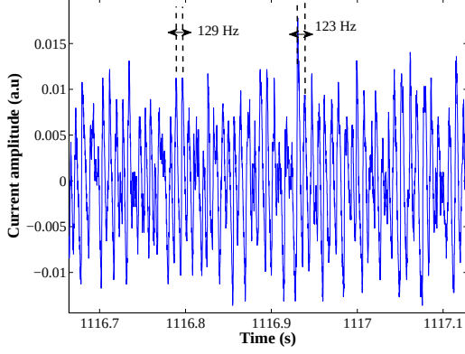
Figure 4.6: A part of the electrical signal during the long stochastic regime.
