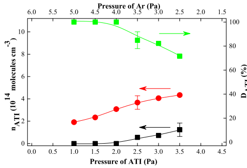
Figure 7.9: Concentration of ATI with - ■ and without - ● plasma operation as well as the degree of dissociation - ▲ as a function of the mixing gas ratio of Ar and ATI, given in pressure values. p_{\text{total}} = 6 Pa, P_{\text{Plasma}} = 80 W.
