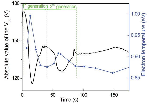
Fig. 5. Temporal evolutions of the absolute value of the DC self-bias voltage and of the electron temperature.
