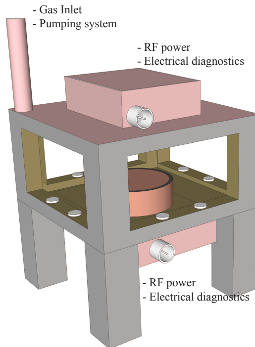
Figure 3.1: Schematic of the PKE-Nefedov reactor.
