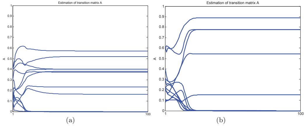
Figure 3.12: Estimation of the transition matrix A from K-DATA-1011 and the initial parameter vector: (a) \theta^{(1,0)} ; (b) \theta^{(2,0)} .
