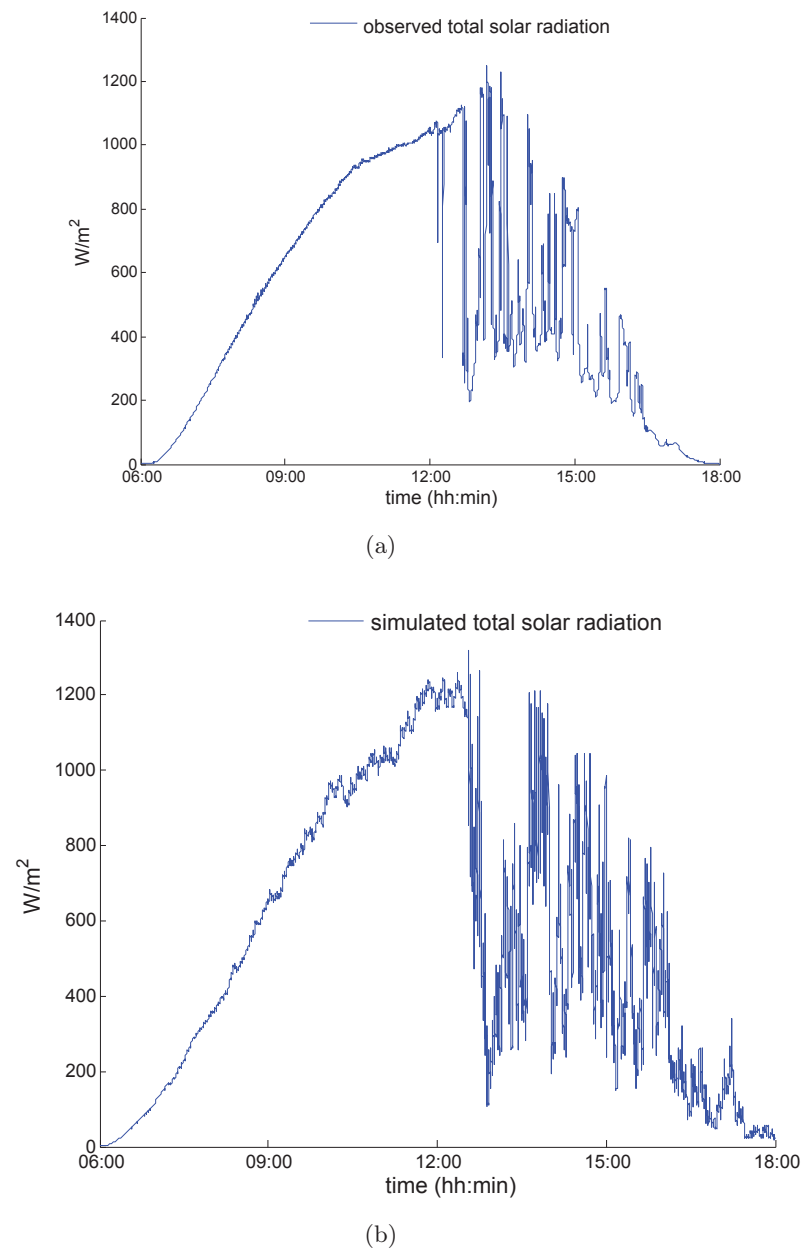
Figure 4.14: (a) Graph of observed data y-DATA-day-II; (b) A simulation for y-DATA-day-II.
