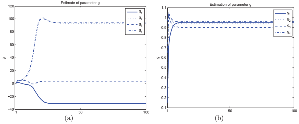
Figure 4.11: Estimation of parameter vector g : (a) from y-DATA-II.1; (b) from y-DATA-II.2.
