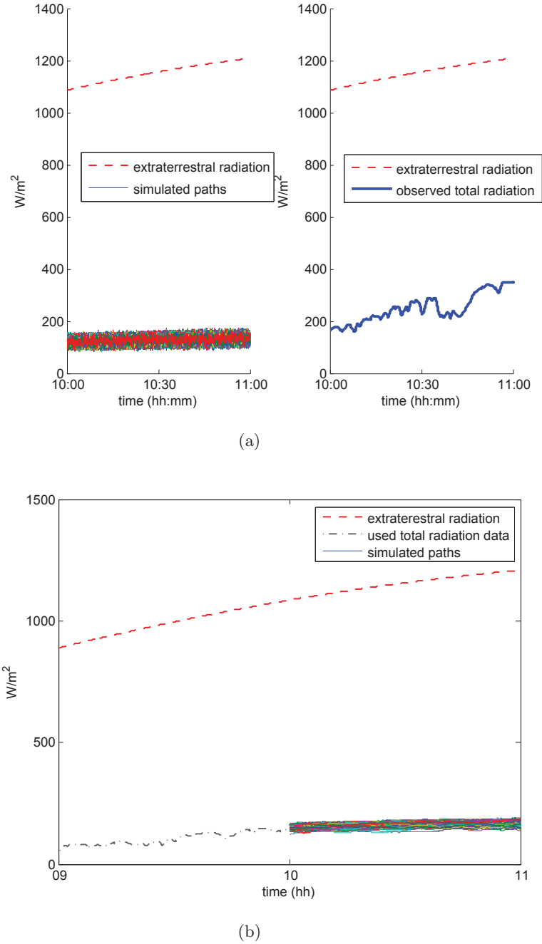
Figure 5.13: (a) left: Simulated paths in 10h-11h generated by CTM-k with parameters estimated from observations in 09h-10h, day 285 (type III, cloudy day), 2006, Guadeloupe (k-DATA-III.2), right: Observed data. (b) Simulated paths in 10h-11h generated by CTM-y with parameters estimated from y-DATA-III.2.
