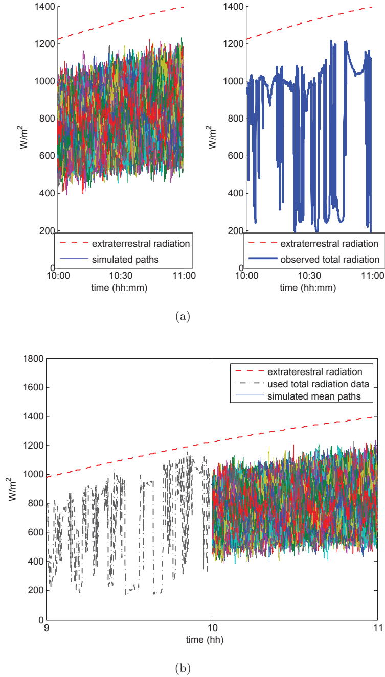
Figure 5.15: (a) left: Simulated paths in 10h-11h generated by CTM-k with parameters estimated from observations in 09h-10h, day 118 (type II, partially cloudy day), 2006, Guadeloupe (k-DATA-II.1), right: Observed data. (b) Simulated paths in 10h-11h generated by CTM-y with parameters estimated from y-DATA-II.1.
