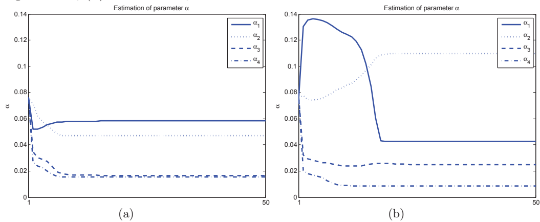
Figure 3.11: Estimation of parameter vector \alpha from daily CIS measured in: (a) August 2009, (b) March 2010, La Réunion-France.
