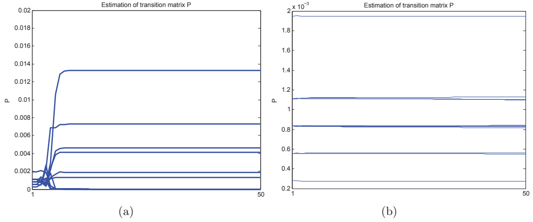
Figure 3.16: Estimation of transition probability matrix P from: (a) k-DATA-III.3; (b) k-DATA-II.2.
