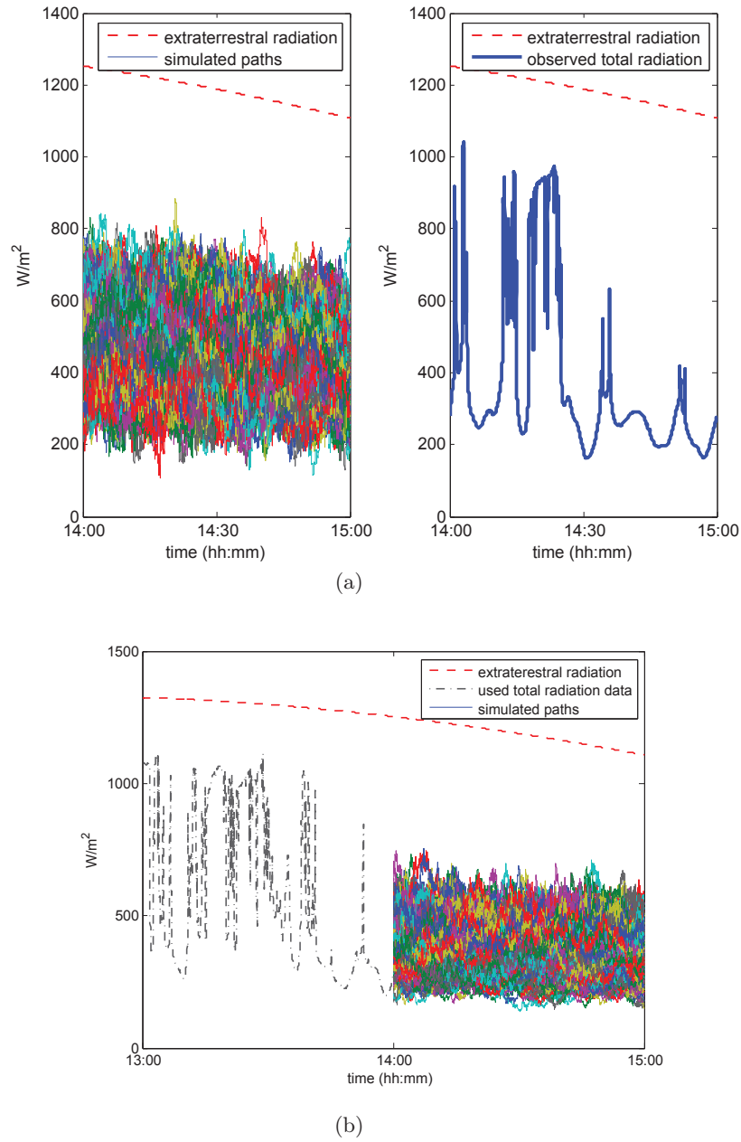
Figure 5.8: Paths simulated from 14h to 15h (a) using CTM-k with parameters estimated from k-DATA-II.2 (left), observed data (right), (b) using CTM-y with parameters estimated from y-DATA-II.2.
