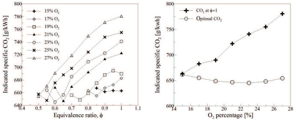
Figure 2-11a. IMEP=400kPa
