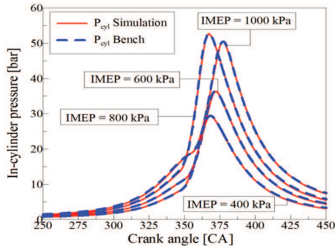
Figure 4-9b. \phi=1 , 21% O 2
