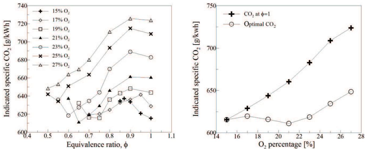
Figure 2-11c. IMEP=800kPa
