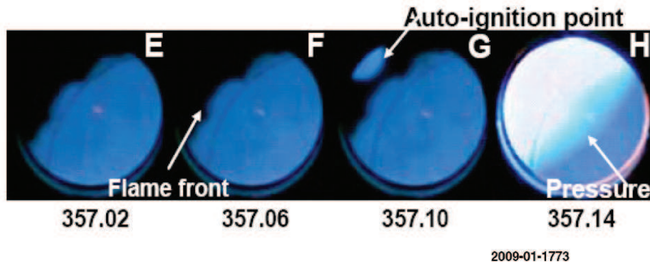
Figure 1-9. Time-series of high speed direct combustion images with the H_2-O_2-Ar mixture (equivalence ratio=1.0, P_0=40kPa , T_0=323K , \theta_i = 355 deg and knock intensity KI = 1.173Mpa )(Kawahara 2009)
