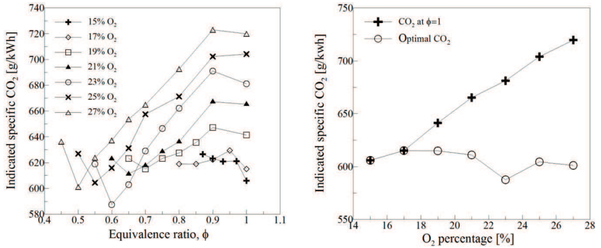
Figure 2-11b. IMEP=600kPa
