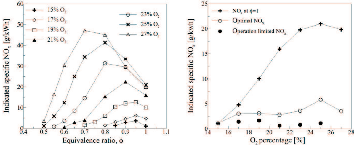
Figure 2-7a. IMEP=400kPa
