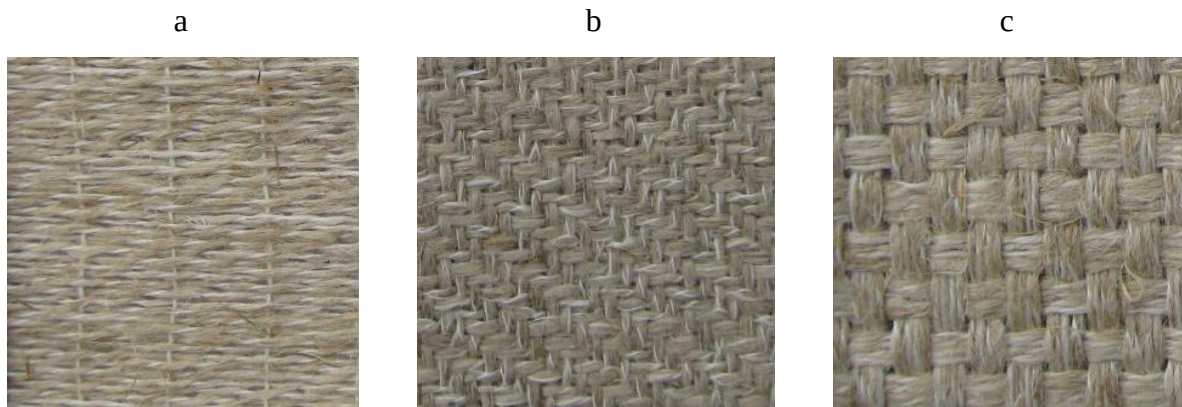
Figure 1-2: Armures bidimensionnelles: a) quasi-unidirectionnel, b) sergé 2x2, c) hopsack 4x4 [3].
