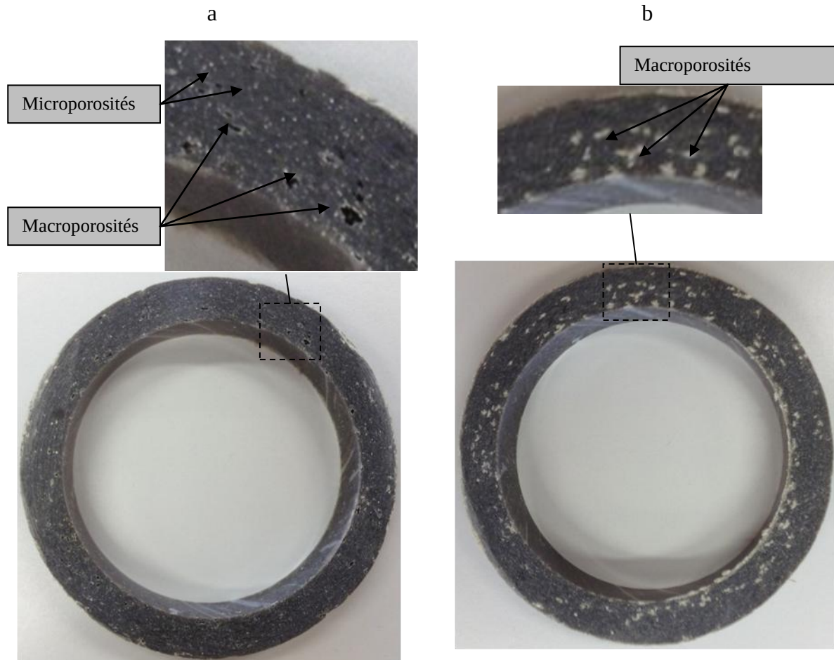
Figure 4-15: Section transversale du prototype 2.
