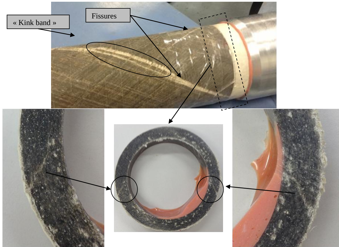
Figure 4-20: Faciès de rupture en flexion, prototype 2.
