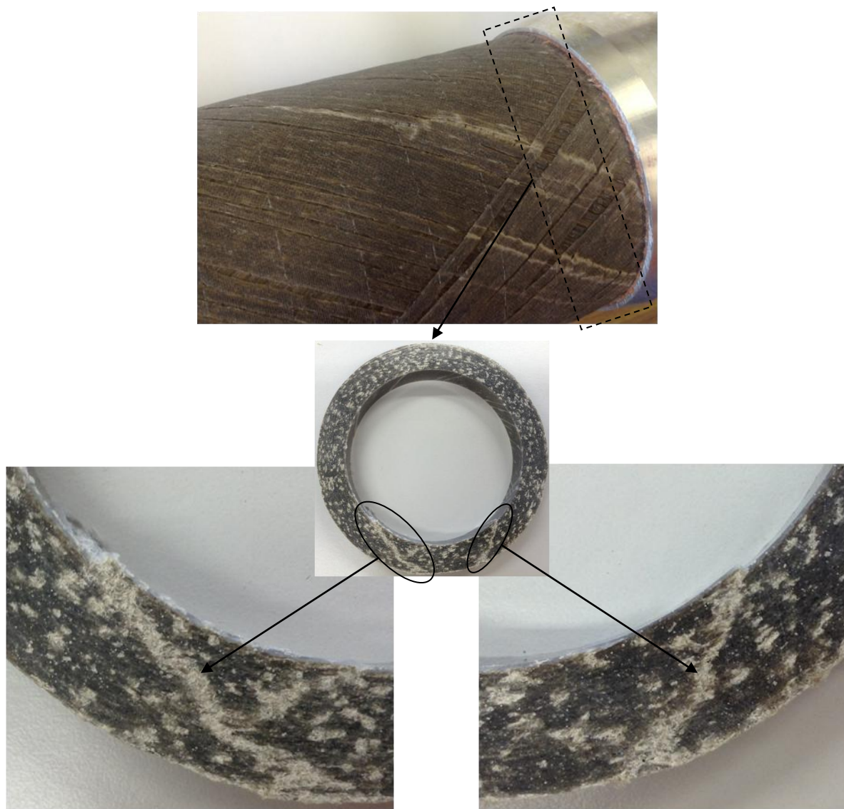
Figure 4-25: Faciès de rupture en torsion, prototype 2.
