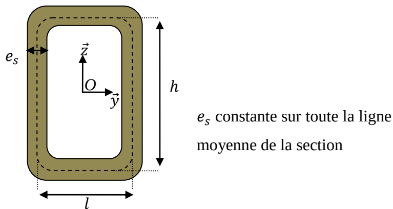
Figure 2-3: Section transversale rectangulaire creuse
