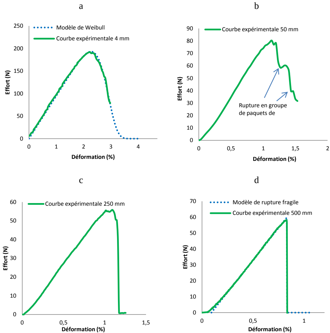
Figure 3-14: Comportement de la mèche: a) 4 mm, b) 50 mm, c) 250 mm and d) 500 mm.
