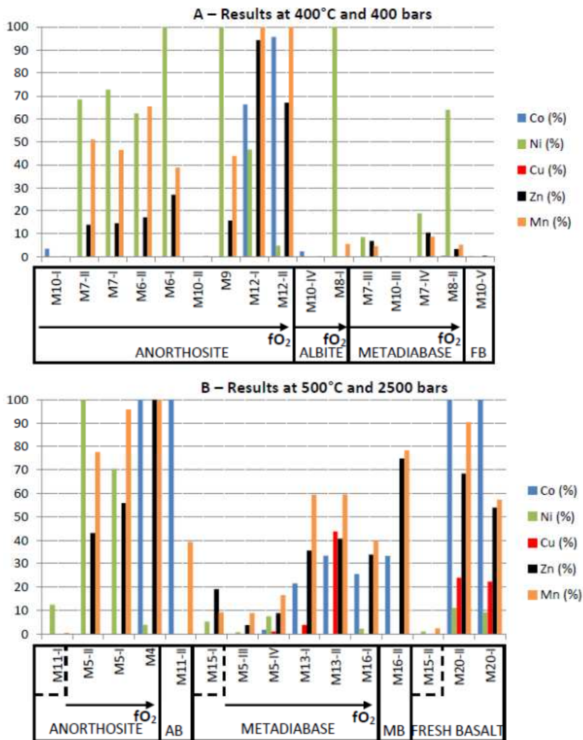
Figure 3.2: Percentages of metals (Co, Ni, Cu, Zn and Mn) leached from starting materials at 400°C and 400 bars (A) and 500°C/2500 bars (B). Black narrows represent supposed increasing fO_2 according to capsule alloy and the presence or not of HM buffer. Experiments using a synthetic seawater are represented by dashed boxes. CaCl_2 was used in all other experiments. Abbreviations: AB = albite; FBA = fresh basalt; MB = metabasalt.
