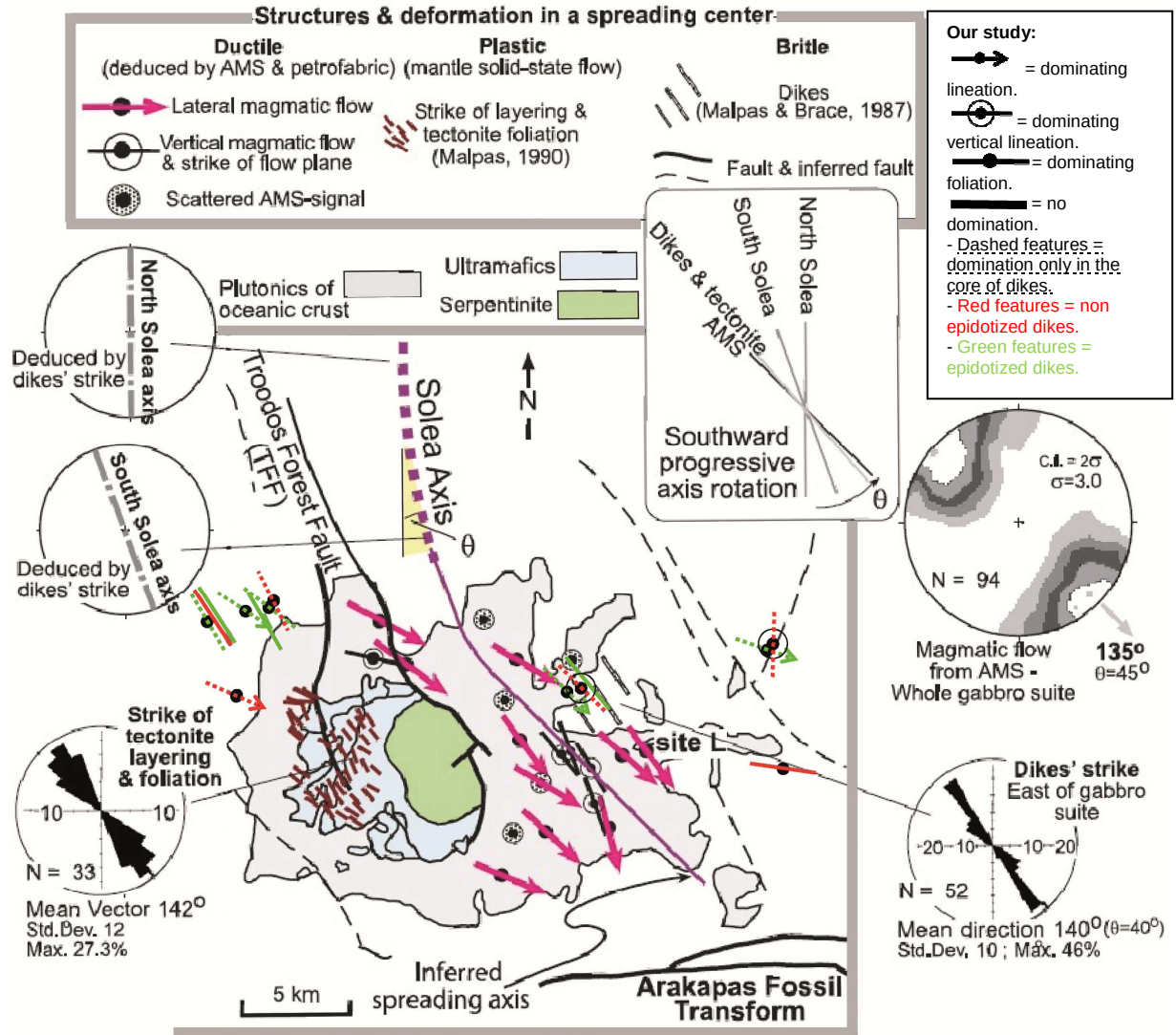
Fig. 2.52: Structural characteristics of the fossil ridge-transform intersection around the Solea graben of Troodos ophiolite (figure modified from Abelson et al., 2002). The axis of the Solea graben (thick dashed purple line) is taken from Varga and Moores (1985) and Hurst et al. (1994). Our results have been added to the study of Abelson et al. (2002) on AMS in the gabbro suite.
