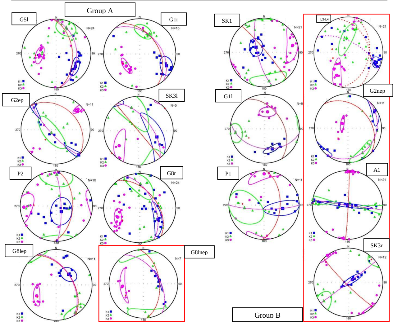
Figure 2.51: Directions of AMS principal axes of all dikes plotted in equal area stereograms.
