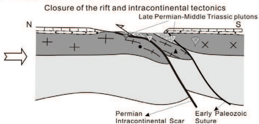
Fig.6-3-1 The Paleozoic tectonic evolutionary mode in central Inner Mongolia
