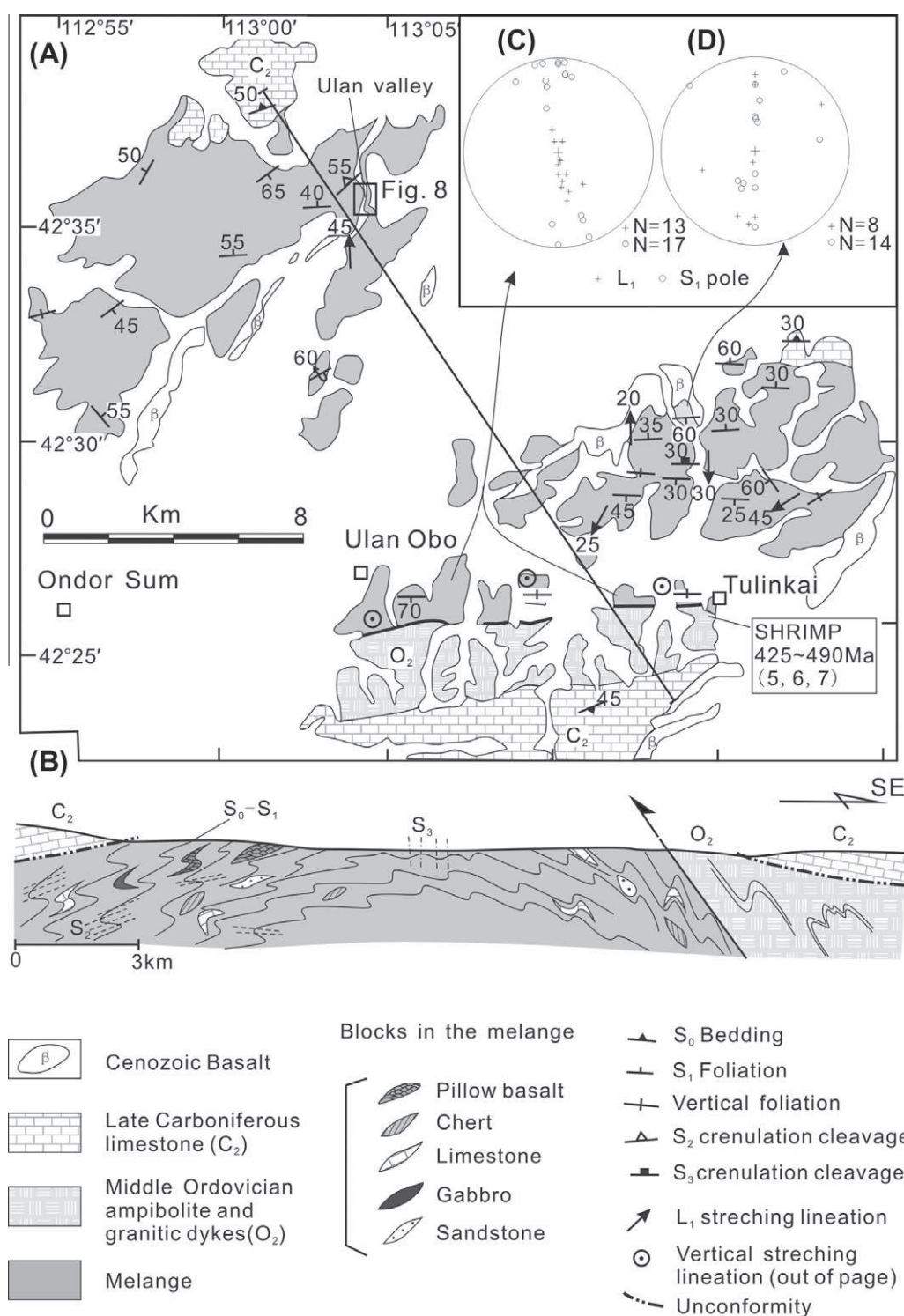
Fig. 7. Sketch map (A), cross section (B), and structural elements of Ondor Sum area (C, D; lower hemisphere projection), modified after IMBGM (1976). The Cenozoic trap basalts must not be confused with the basaltic blocks included in the mélangé.
