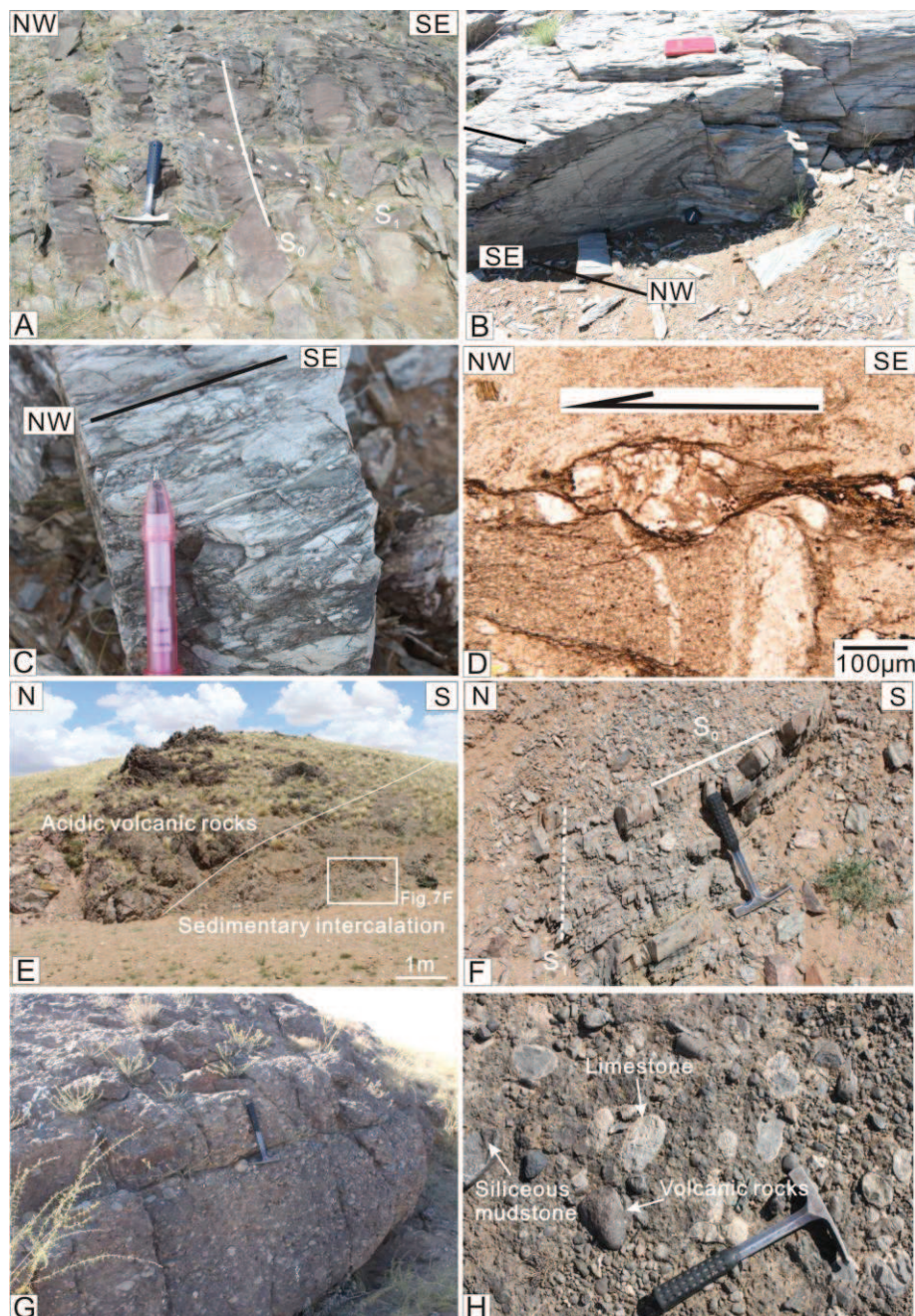
Fig.7 Field pictures of the deformation style. (A) Ta, Tac, Tcd division of Bouma; the bedding ( S_0 )-cleavage( S_1 ) angular relationships and upward fining bedding indicate NW ward vergence; (B) intrafolial fold in turbidites composed of dark grey thin bedded sandstone and grey medium bedded siltstone; In the inverted limb, the sandstone shows graded bedding; (C) NW-SE elongated pebble in turbidite (Ta), indicating NW shearing; (D) Pressure shadow at the margins of feldspar clast, showing top-to-the NW sense of shear; (E-F) the volcanic bedding of the Dashizhai Formation steep dipping while sedimentary intercalation with well developed cleavage. (G-H) the Zhesi Formation is gentle dipping with pebbles of limestone, volcanic rock and mudstone of underlying strata.
