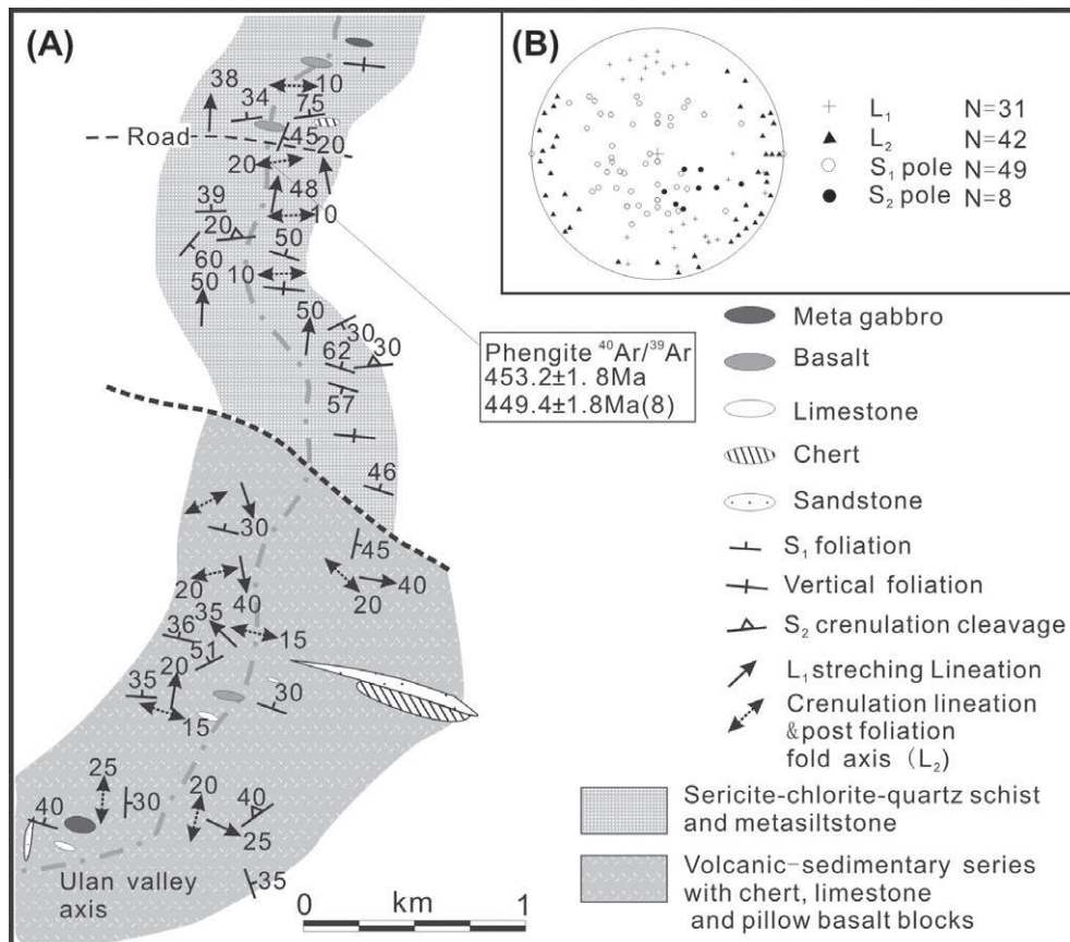
Fig. 9. Structural map of the microtectonic data observed in the Ulan valley (modified after Xiao et al., 2003).
