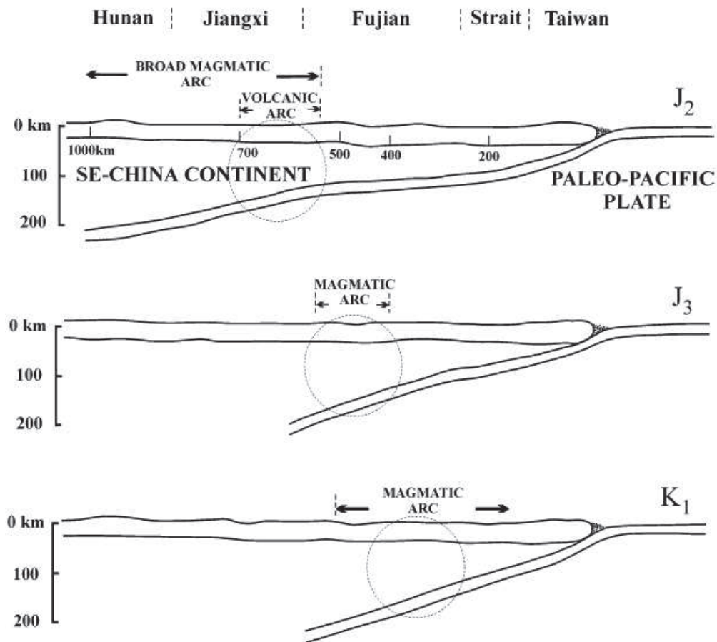
Figure 1 1: Hypothesis of deepening of subduction angle and back-arc extension retreat
