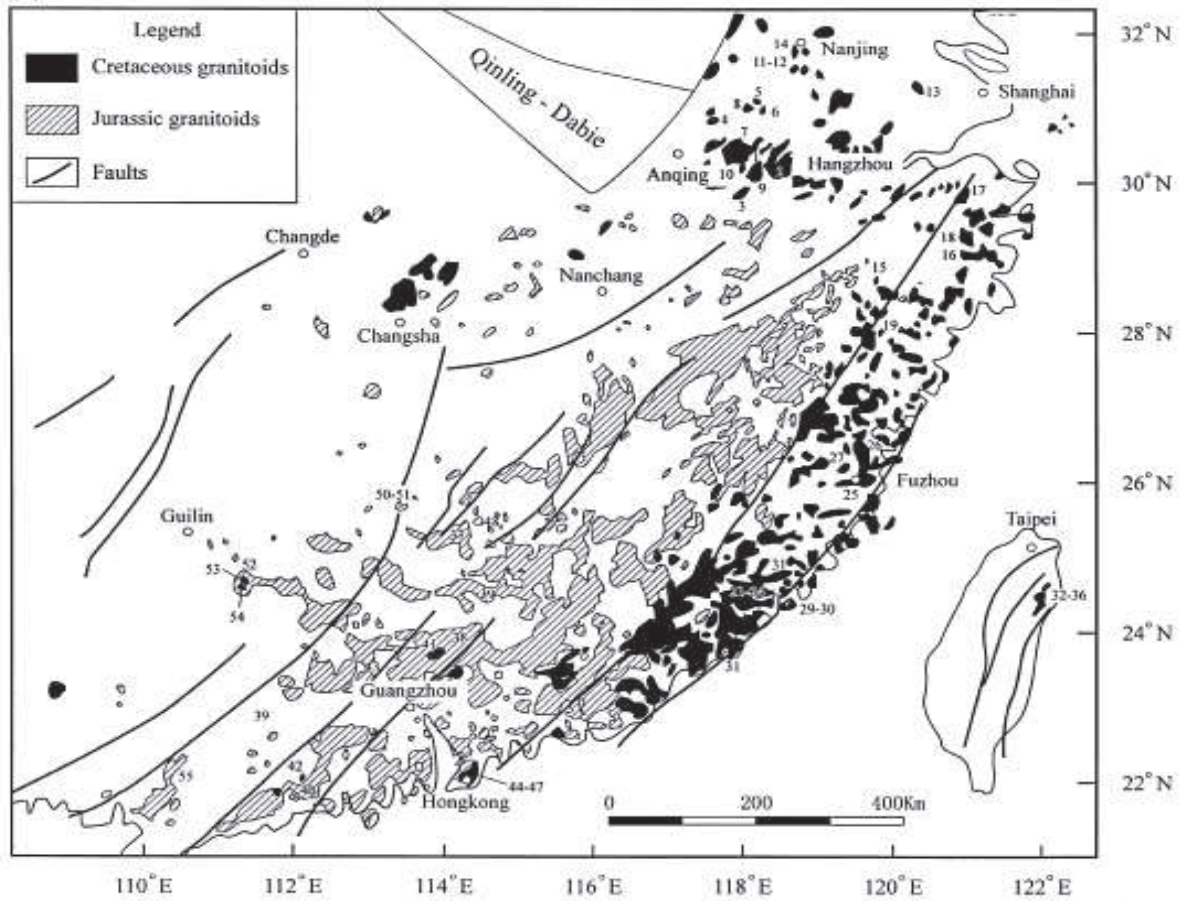
Figure 2 2: Distribution of Late Mesozoic Plutons in the South China
