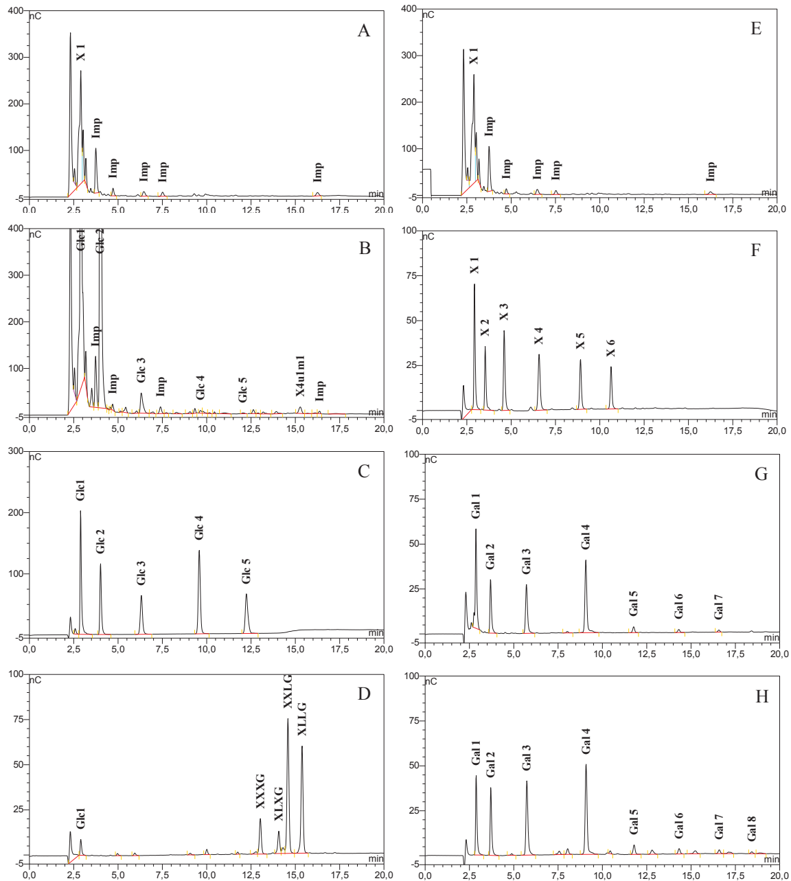
Figure 2. HPAEC-PAD chromatograms of A, untreated G-layer. B, endo-1,4-glucanase degradation products from the G-layer under mild conditions (30 min of hydrolysis). C, a commercial celloextrin. D, mixture of standard xyloglucans oligomers. E, endo-1,4- \beta -xylanase degradation products from the G-layer. F, mixture of standard xylo-oligomers and G, endo-1,4- \beta -galactanase degradation products under mild conditions (30 min of hydrolysis) from G-layer and from H, a commercial pectic galactans. Nomenclature is as follow: Hexose containing oligosaccharides attributed to glucomannans were noted H for Hexose. Pentose containing oligosaccharides recovered after xylanase degradation was noted X for Xylose. In all oligomer codes, extension with the letter u, m and a refers to substitution by an uronic acid, a methyl and acetyl group, respectively. The number following the letter codes denoted the number of building hexosyl or xylosyl units and the number of methyl or acetyl groups in the oligosaccharides (i.e. H3a1 corresponds to 3 hexosyl units and 1 acetyl group).
