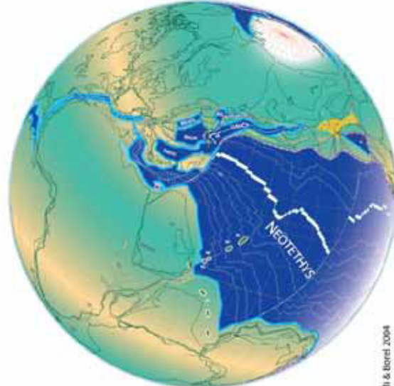
180 Ma - Toarcian-Aalenian
