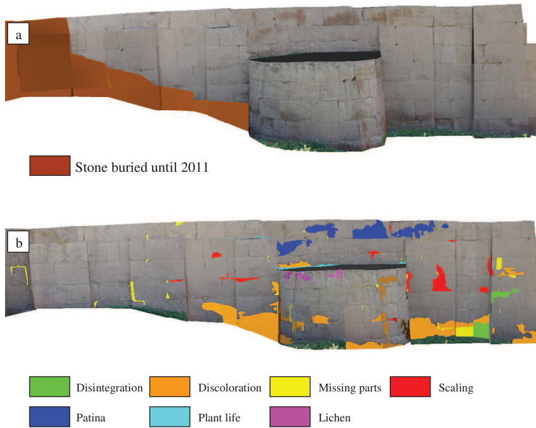
Fig. III-31. Part of Al-Ziggurat wall showing: (a) the state of the burial in 2011; (b) the state both of the recently uncovered and the degraded stones that projected on the created 3D model.
