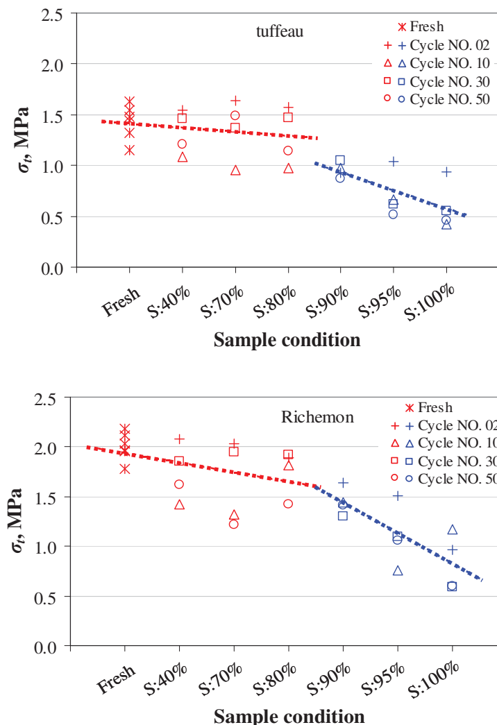
Fig. II-29. Indirect tensile strength for fresh and aged samples of tuffeau and Richemont stone.
