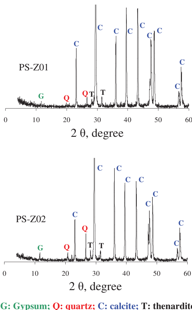
Fig. III-18. XRD patterns for the powder samples at the surface of the degraded stone.
