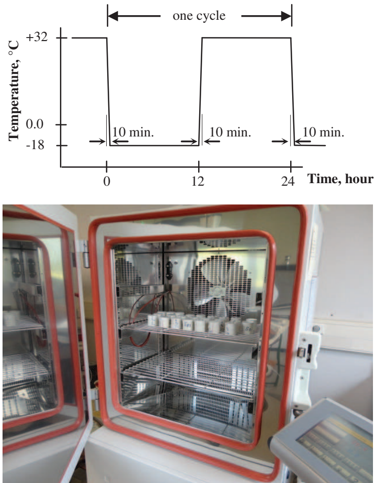
Fig. II-26. Schematic for one freezing-thawing cycle ( top ), general setting of the tested samples inside the freezing chamber ( bottom ).
