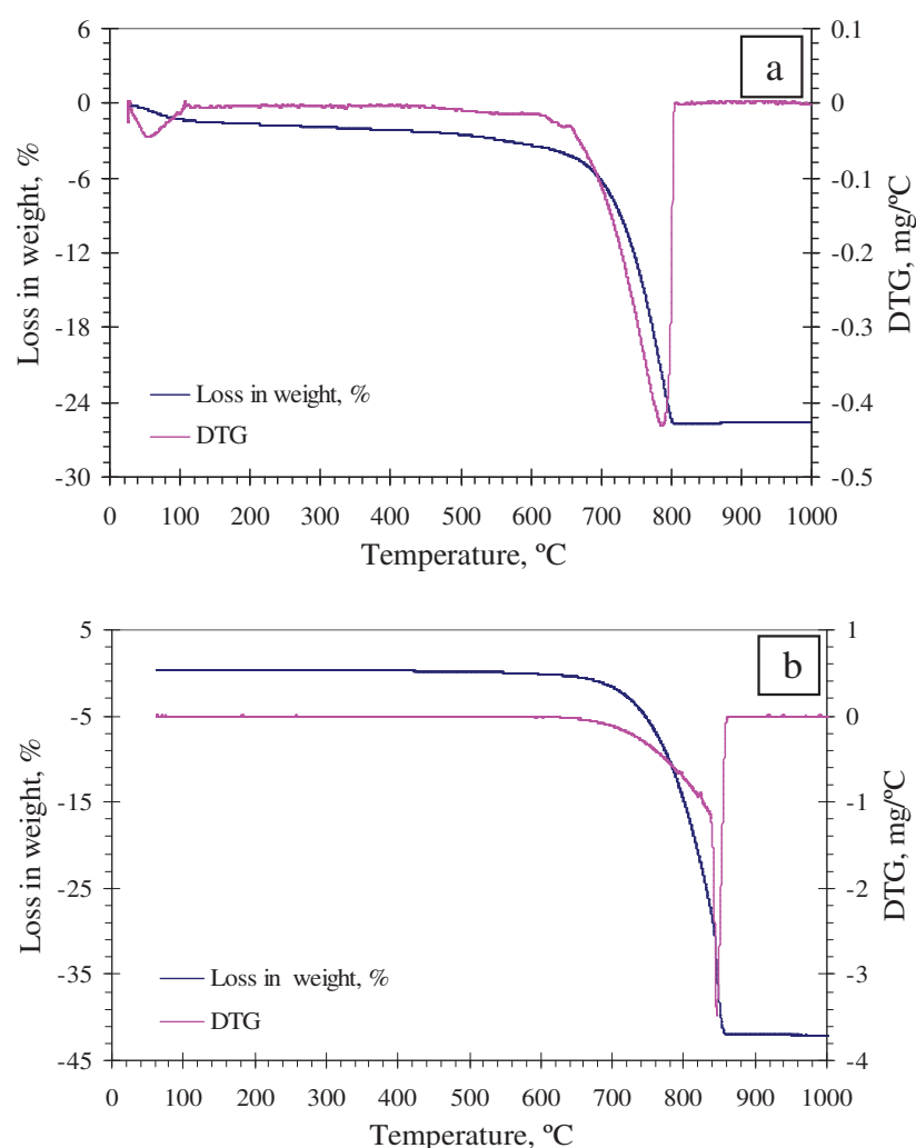
Fig. II-6. Thermo-gravimetric analysis of the limestones: (a) tuffeau; (b) Richemont stone.
