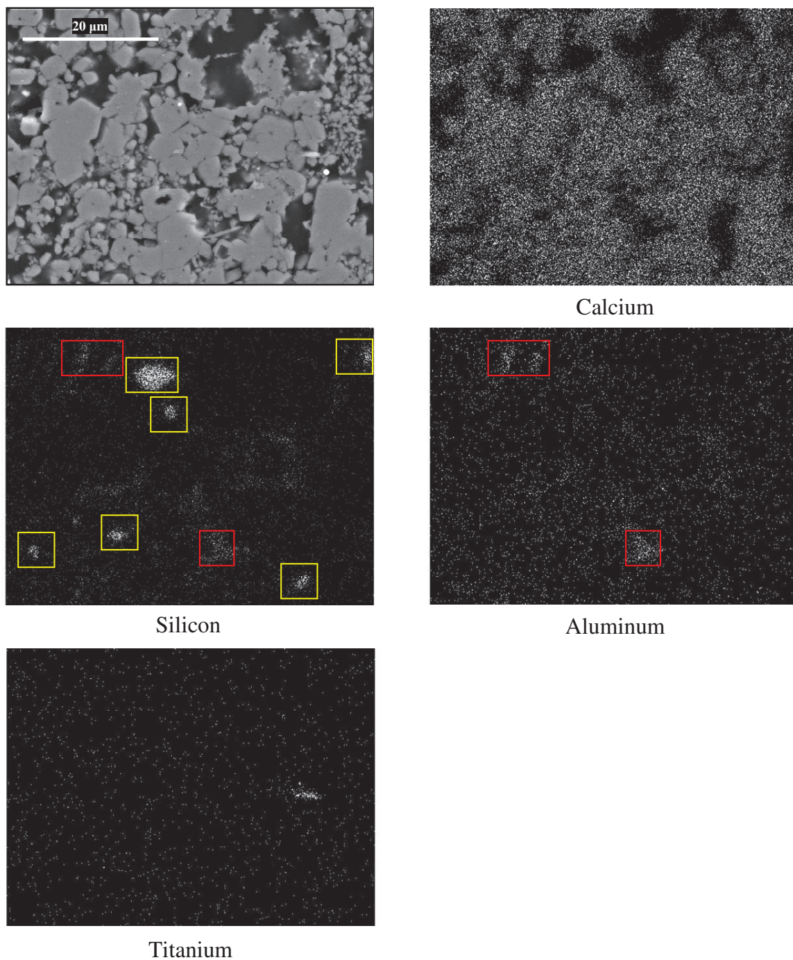
Fig. II-10. EDS maps showing the elemental compositions of Ca, Si, Al and Ti present in Richemont limestone.
