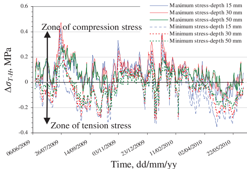
Fig. II-37. Maximum and minimum differential hygrothermal stresses at different depths inside the stone on the south wall for the period from June 2009 to June 2010.
