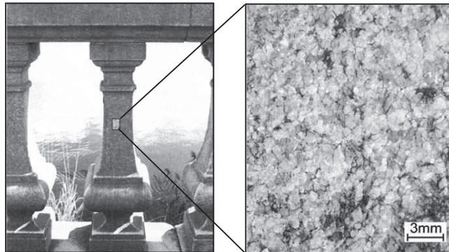
Fig. I-9. Cleavage planes due to thermal stress, Marmorpalais in Potsdam, Germany (marble) (Zeisig et al., 2002).
