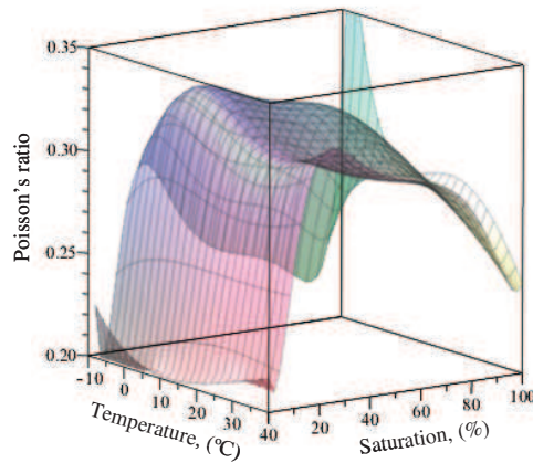
c) Poisson's ratio
