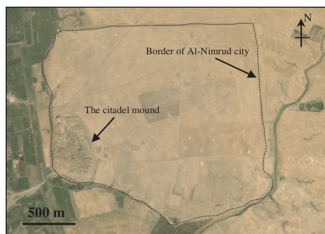
Fig. III-1. Map of Iraq showing the general setting of Al-Nimrud city ( top ); Google satellite image of Al-Nimrud city ( bottom ).
