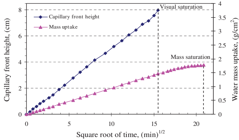
Fig. II-16. Curves of the capillary water absorption for Richemont stone.
