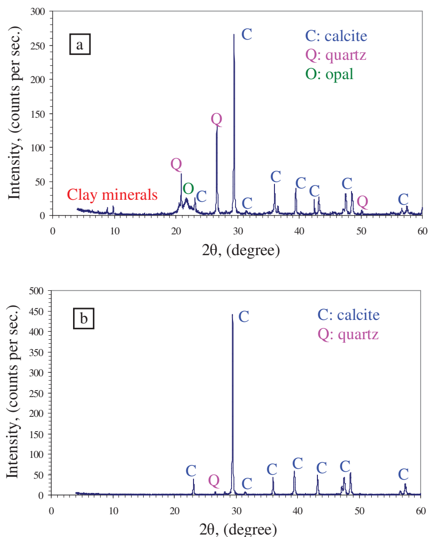
Fig. II-5. Diffraction patterns of the stones, (a) tuffeau; (b) Richemont stone.
