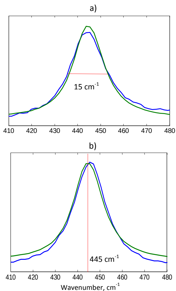
Figure 4.26. Comparison of experimental (blue-colored) Raman spectra from grains possessing the differences in measured and calculated T 2g intensities: observation of a) T 2g band enlargement and b) T 2g band upshift compared to those typical of stoichiometric UO 2 (green-colored spectra). Here, the red numbers indicate FWHM and \omega of T 2g band which are characteristic of stoichiometric UO 2 .
