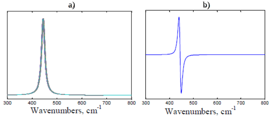
Figure 3.5. a) T_{2g} profiles simulated with the Lorentz function by changing a band position. b) PC2 loading extracted from these profiles.
