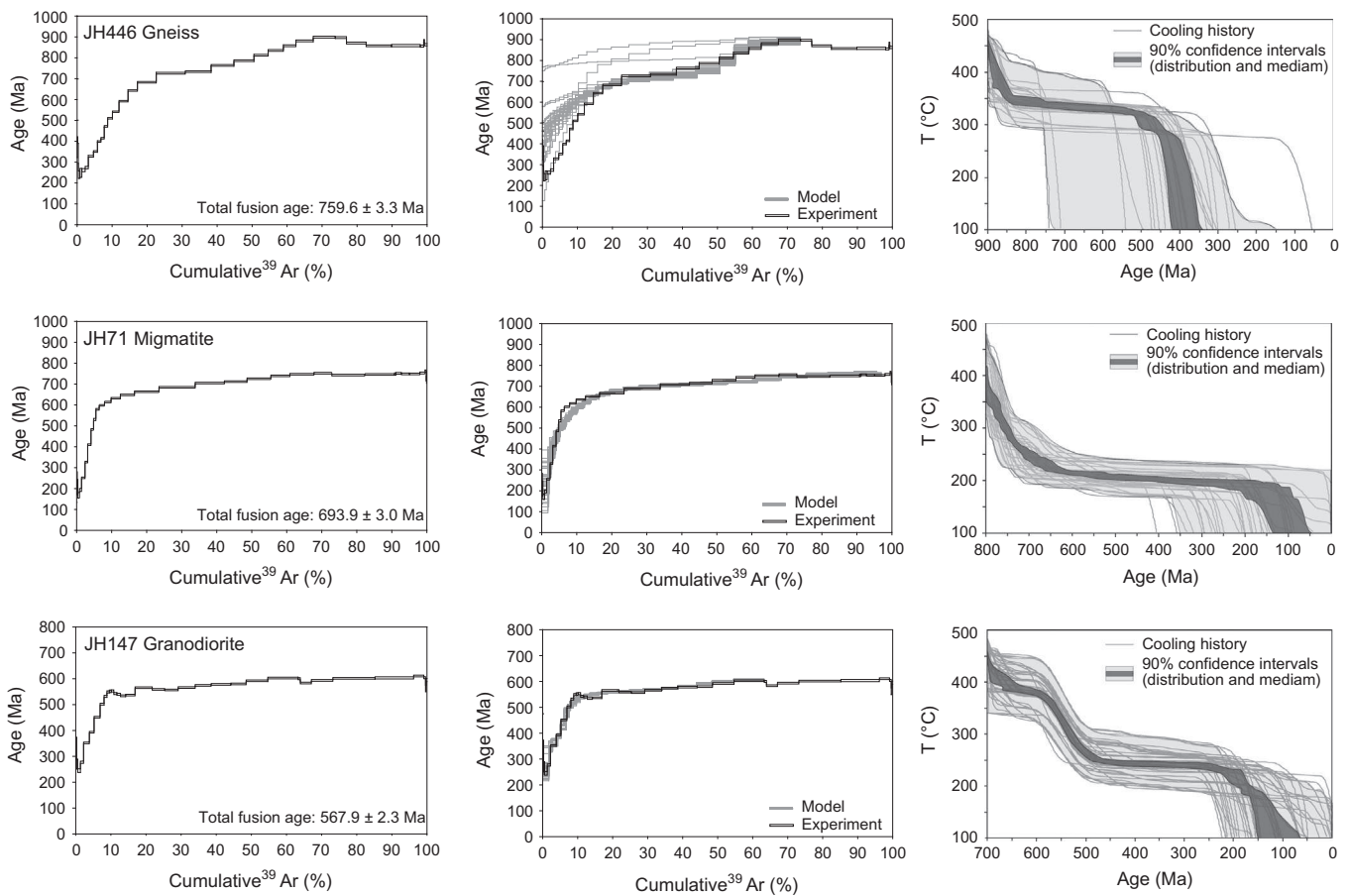
Fig. 9. ^{40}\text{Ar} – ^{39}\text{Ar} age spectra and the multi-domain diffusion (MDD) modeling results of K-feldspar from different rock types in the core of Huangling massif.
