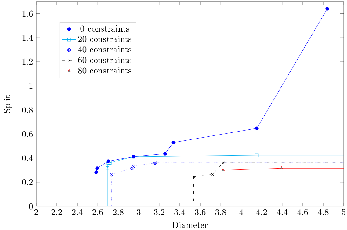
Figure 7.6: Bi-criteria constrained clustering with dataset Iris
