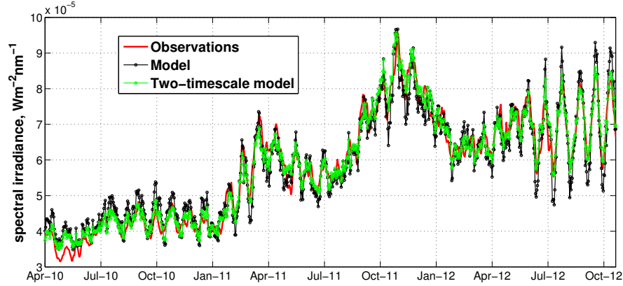
Figure 3.19: Comparison of the single timescale and two-timescales model fits of a wavelength at which the emission is optically thin (8 nm).
