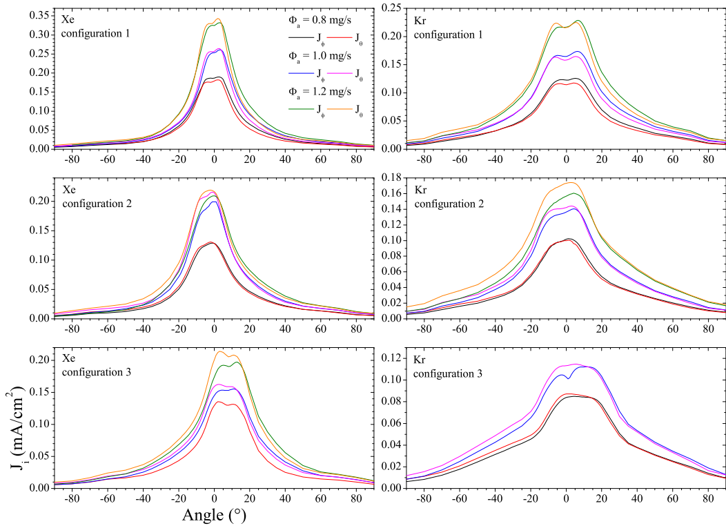
5.8.2: Ion current density profiles - anode flow rate series.
