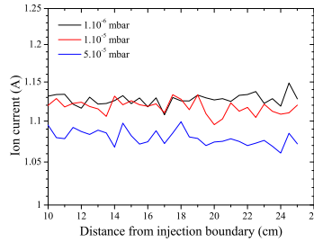
B.5.2: Ion current.
