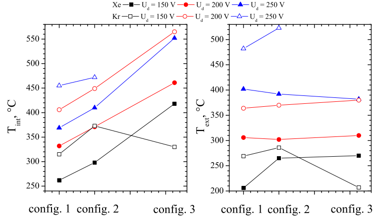
5.11.1: Temperature of the PPI-Mag ceramics - discharge voltage series.
