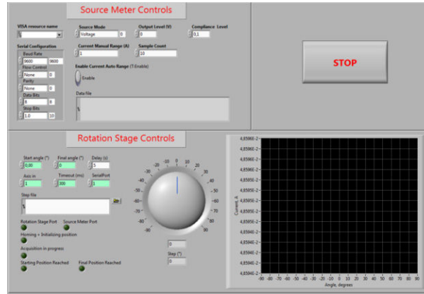
Figure 4.16: Front view of the Labview program for the probe measurements. The program controls the rotation stage and the measurement process, so that both act coherently with each other. The programme creates datafiles for postprocessing.
