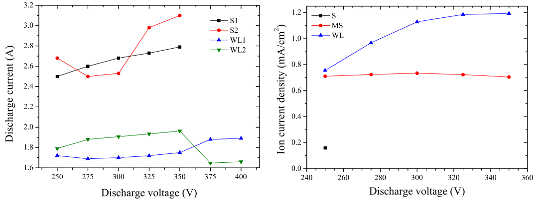
6.16.1: Current-voltage plots, for the PPS-Flex operating in 6.16.2: Ion current density in the plume of the PPS-Flex in WL mode.
