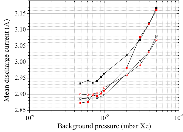
Figure 4.6: Influence of the background pressure on the discharge current mean value, for the PPS-Flex operating at various conditions. The discharge current plateaus below 7 \times 10^{-6} mbar-Xe.
