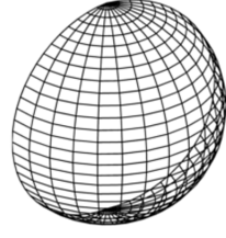
4.11.1: Surface elements of a spherical domain.
