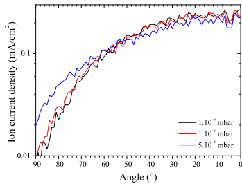
B.5.1: Ion current density.
