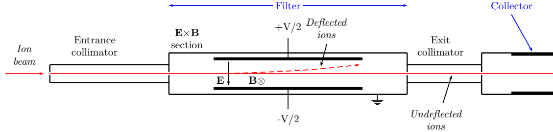
Figure 4.4: Schematic view of an E \times B probe.
