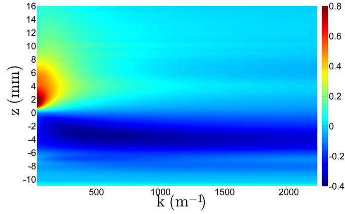
Figure 3.12: Growth rate mapping as a function of the mode wavenumber and axial position along the cavity axis. The colorbar is expressed in MHz.
