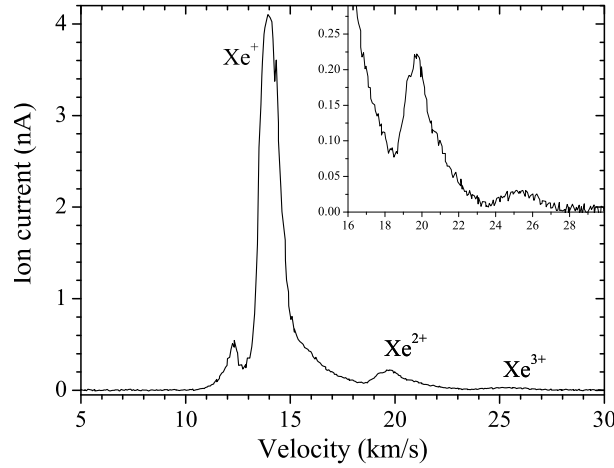
Figure 4.5: E \times B probe measurement 40 cm downstream of the PPI exit plane, under operation at 200 V and 1.0 mg/s of xenon. A small extra hump is seen before the main \text{Xe}^+ peak, and cannot be explained as of yet. This structure was also observed in previous works 16 .
