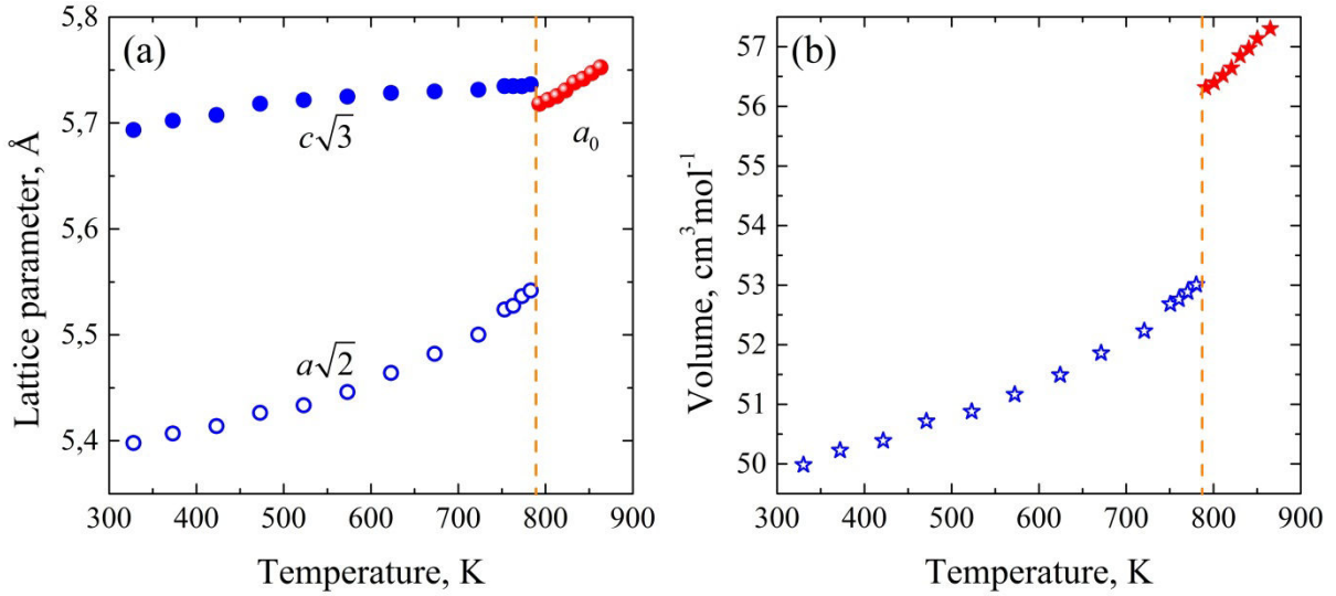
Fig. 4. (a) Variation of the scaled trigonal unit cell parameters ( a\sqrt{2} , c\sqrt{3} ) and the cubic unit cell parameter a_0 in LiNaSO 4 with temperature; (b) temperature dependence of the molar volume in LiNaSO 4 . Dashed line indicates the phase transition temperature.
