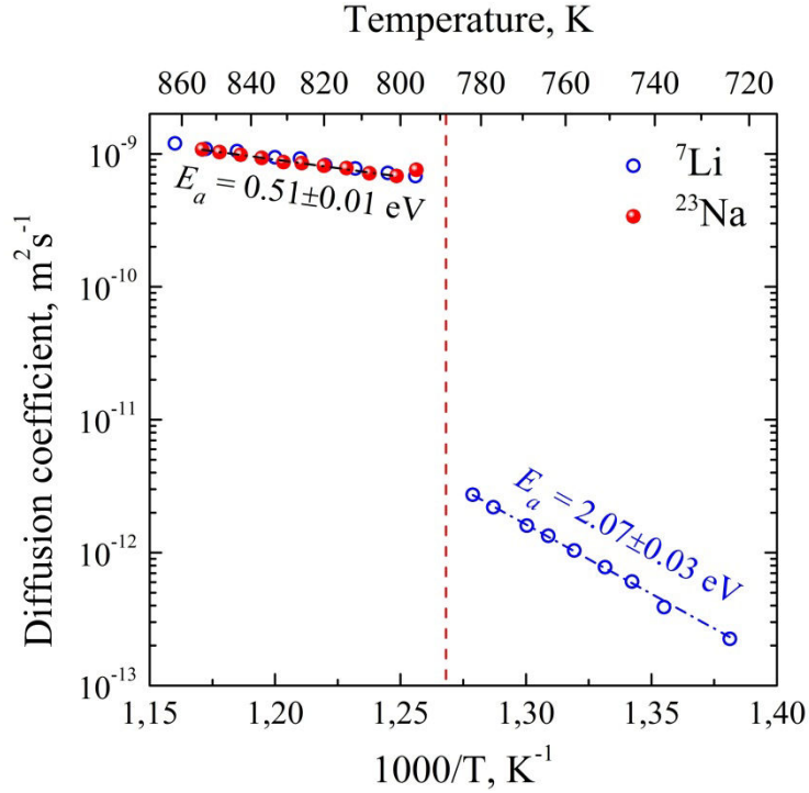
Fig. 28. Temperature evolution of ^7\text{Li} and ^{23}\text{Na} self-diffusion coefficients. Dashed line indicates the \alpha - \beta phase transition temperature.
