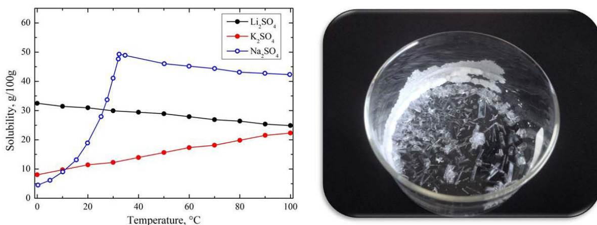
Fig. 20. Solubility curves of some alkali sulfates [118] (on the left) and crystalline aggregates of \text{LiNaSO}_4 grown by evaporation from the solution (on the right).
