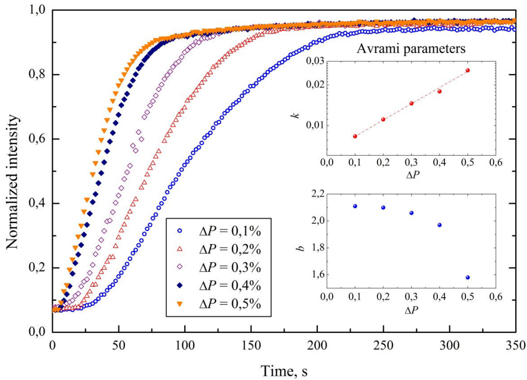
Fig. 35. Time evolution of the amount of the \beta phase during the \alpha - \beta phase transition in \text{LiNaSO}_4 . The dependence of Avrami parameters on the cooling rate (more precisely, on \Delta P ) is shown in the inserts.
