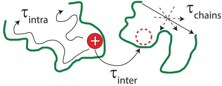
FIGURE 4.27: Three different timescales of \text{Li}^+ motion in polymers were divided by Borodin et al. [92] : \tau_{\text{intra}} ( \text{Li}^+ moves along one chain from head to tail), \tau_{\text{chains}} ( \text{Li}^+ moves cooperatively with the chains), \tau_{\text{inter}} ( \text{Li}^+ jumps between the chains) (figure adapted from ref [93])
