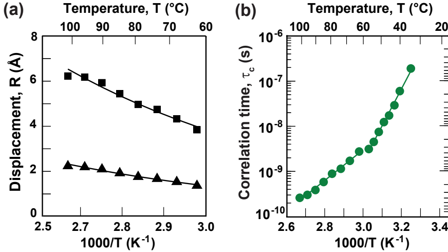
FIGURE 4.25: a. Displacement \sqrt{\langle R^2 \rangle} of Li + calculated from Eq. 4.17, ▲: calculated using \tau_1 , ■: calculated using \tau_2 ; b. The time \tau_{inter} between interchain jumps for Li + in PEO(LiTFSI), calculated using [93]. The lines are guides for the eyes.
