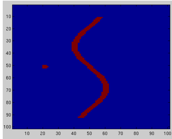
FIGURE 4.4.1 – Image initiale
