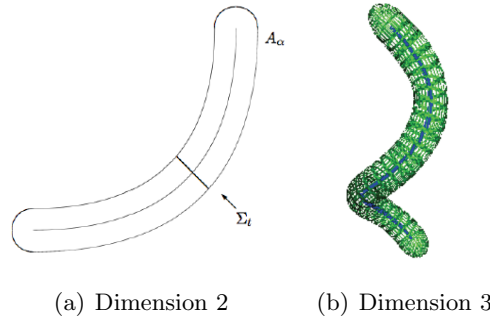
FIGURE 3.1. Tubes A_\alpha
