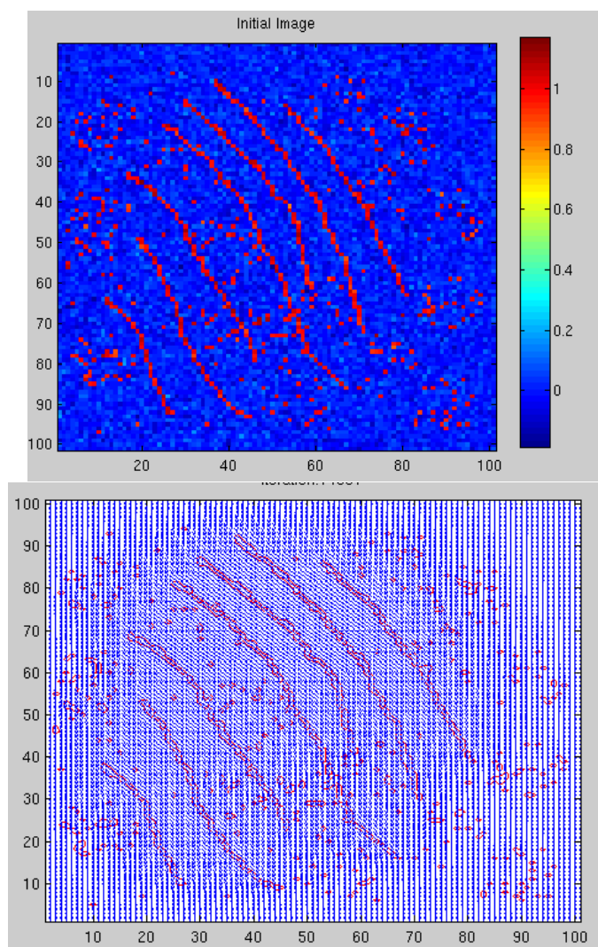
FIGURE 4.4.6 – Image initiale et champ c
