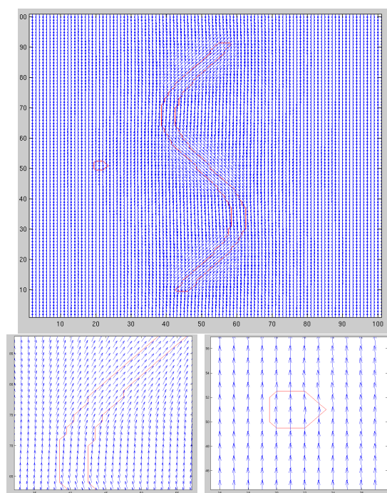
FIGURE 4.4.3 – Champ \mathbf{c}
