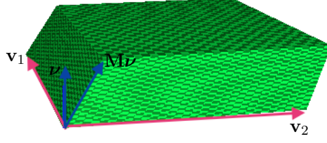
Figure 2.2: Simplex K
