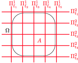
Figure 1.1: Construction of \mathcal{A}
