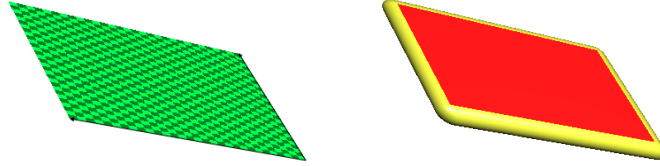
Figure 2.3: Simplex S and \{x : \text{dist}_\phi(x, S) < \langle \mathbf{M}\nu, \nu \rangle^{\frac{1}{2}}\}
