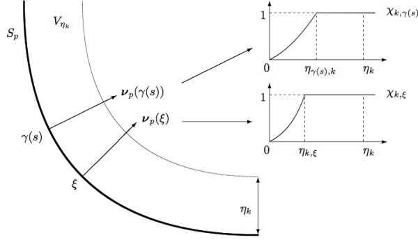
Figure 5.2: Construction of the solution on each slice
