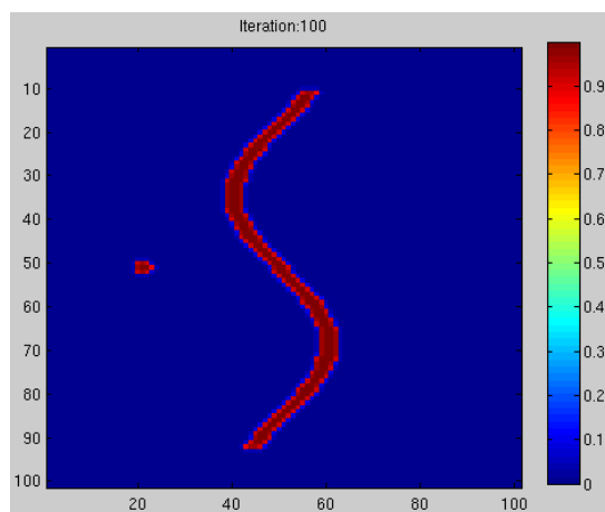
FIGURE 4.4.2 – Cas isotrope
