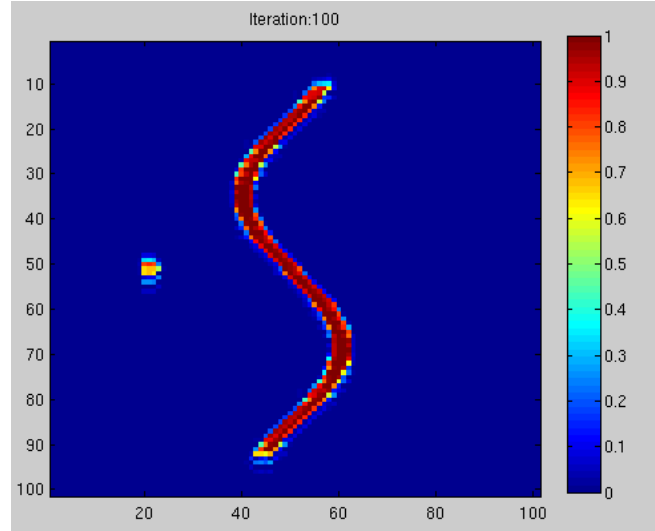
FIGURE 4.4.4 – Cas anisotrope
