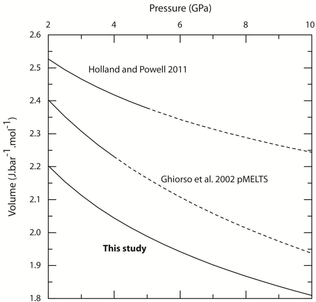
Figure S4: Molar volume of SiO 2 melt component as a function of pressure at 1300°C as recalibrated in this study (see Supplementary Information Part 3). Volumes from pMELTS (Ghiorso et al., 2002) and Holland and Powell (2011) are reported for comparison.
