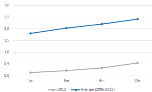
Figure 2.25: Yield curves
