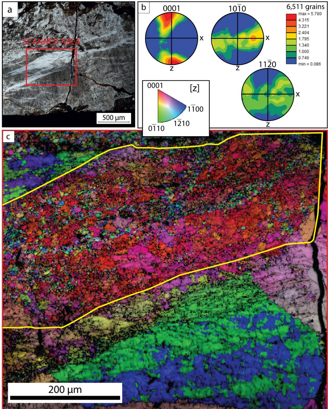
Figure 11. Quartz crystallographic fabrics in a shear band in the Hyuga Tectonic Mélange. A) Optical microscope image of the scanned area. B) Lower hemisphere pole figure of c \langle 0001 \rangle and a \langle 10\bar{1}0 \rangle axes and m (11\bar{2}0) -planes corresponding to the area highlighted by the yellow polygon in C). Note the strong c -axis maxima in Z direction (normal to the foliation plane). C) EBSD map of the shear zone (with a color code associated to inverse pole figure of Z direction), showing the preferential orientation of c -axes close to the Z -direction.
