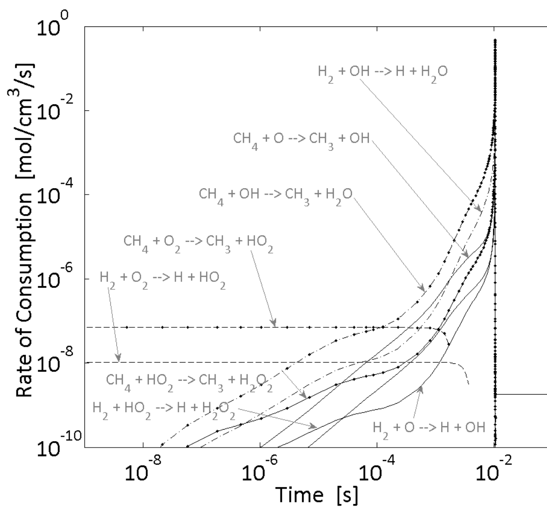
Figure 108. B. Rate of consumption for a mixture of methane and hydrogen (80/20) without ozone.
