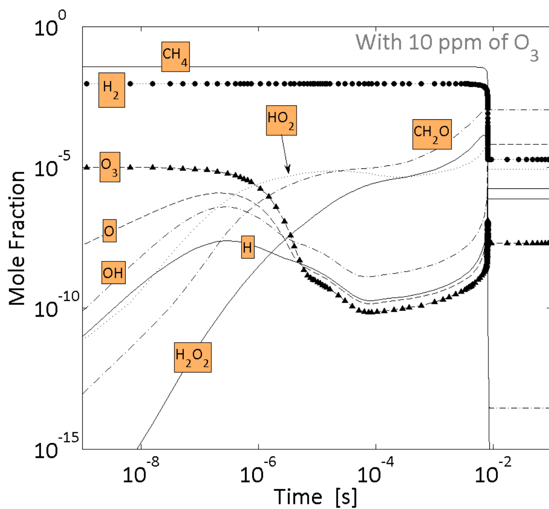
Figure 108. C. Mole fractions of the main radicals for a mixture of methane and hydrogen (80/20) with 10 ppm of ozone.
