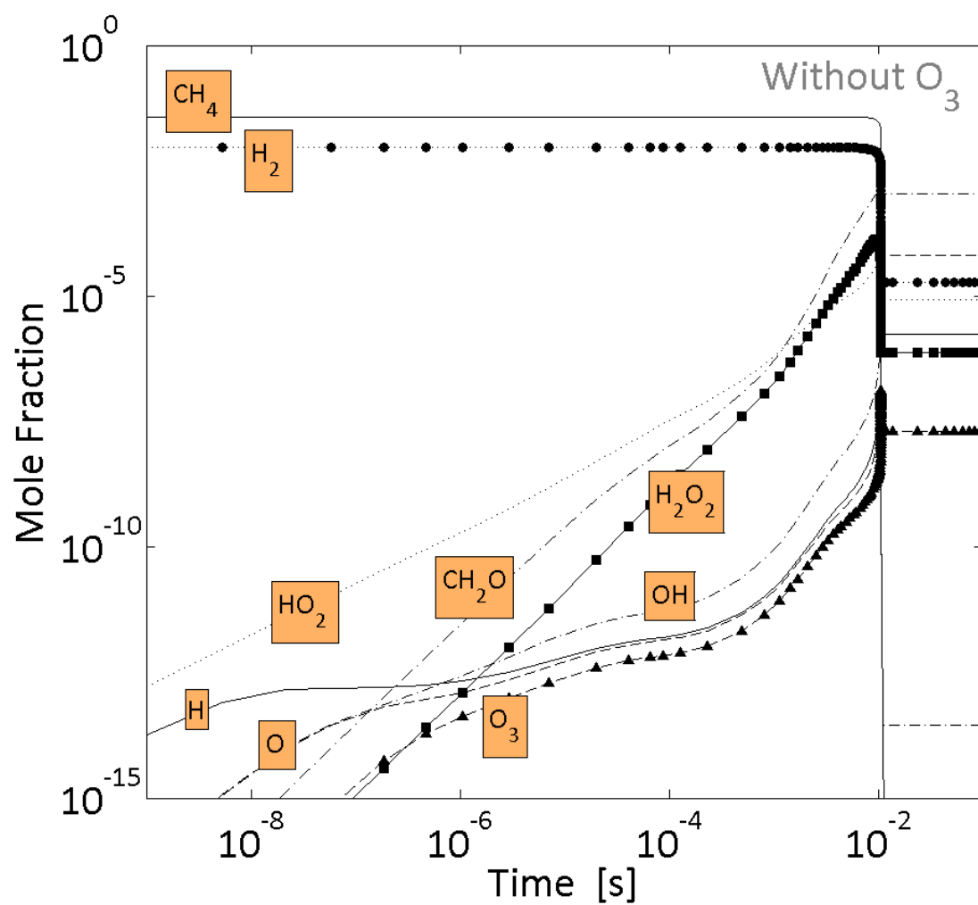
Figure 108. A. Mole fractions of the main radicals for a mixture of methane and hydrogen (80/20) without ozone.
