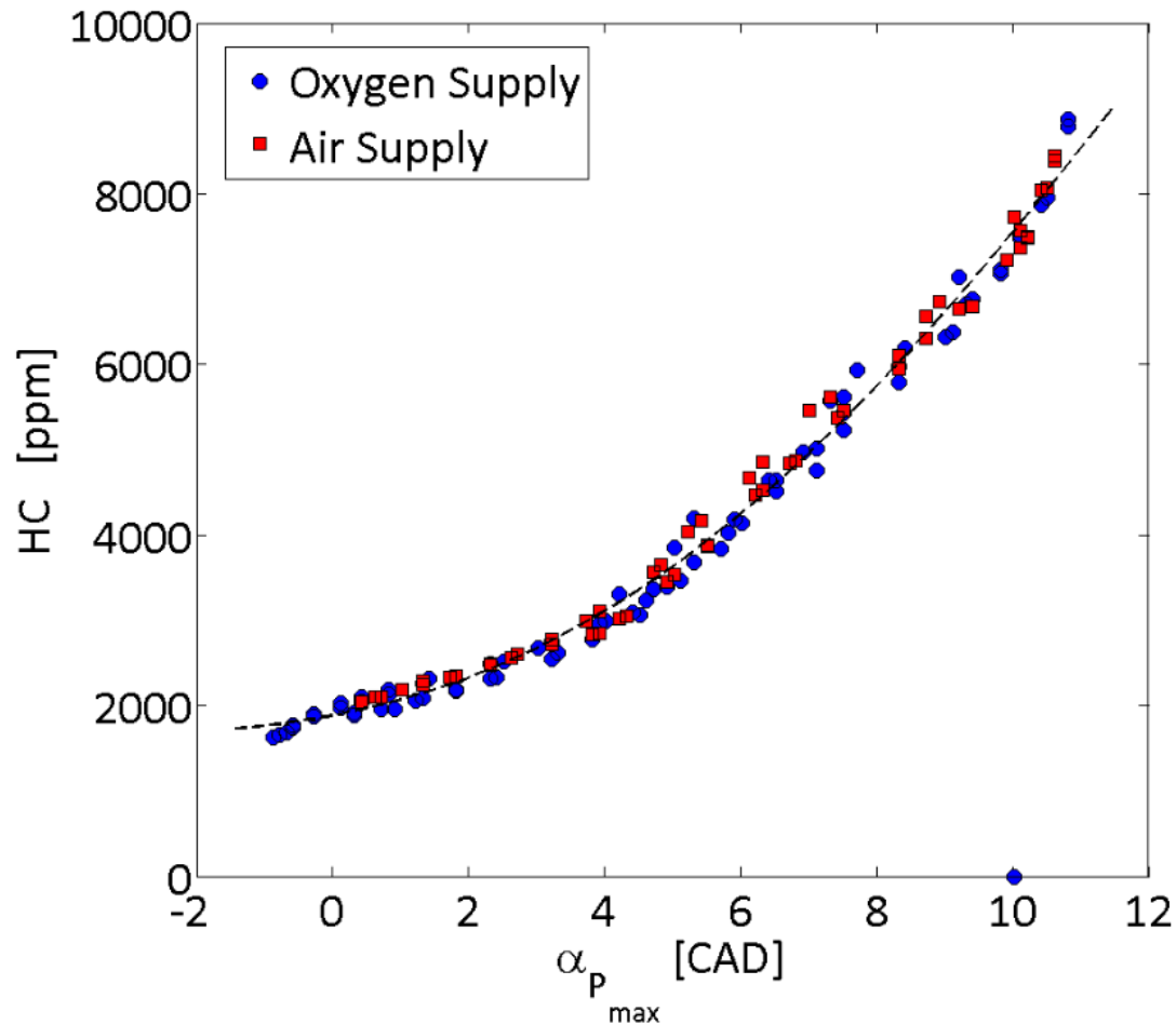
Figure 83. Unburned hydrocarbons trends as a function of the maximum pressure location for both gas supply and the three intake temperatures tested.
