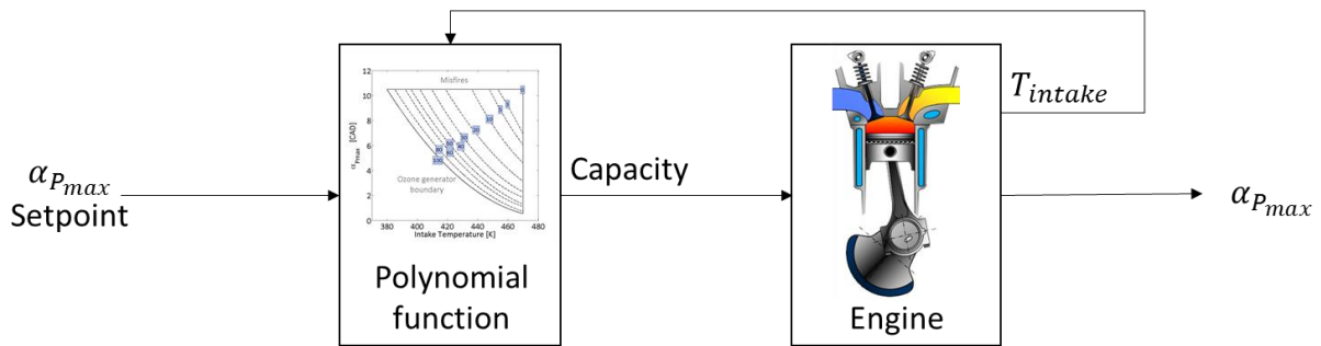
Figure 87. Scheme of the open-loop control.
