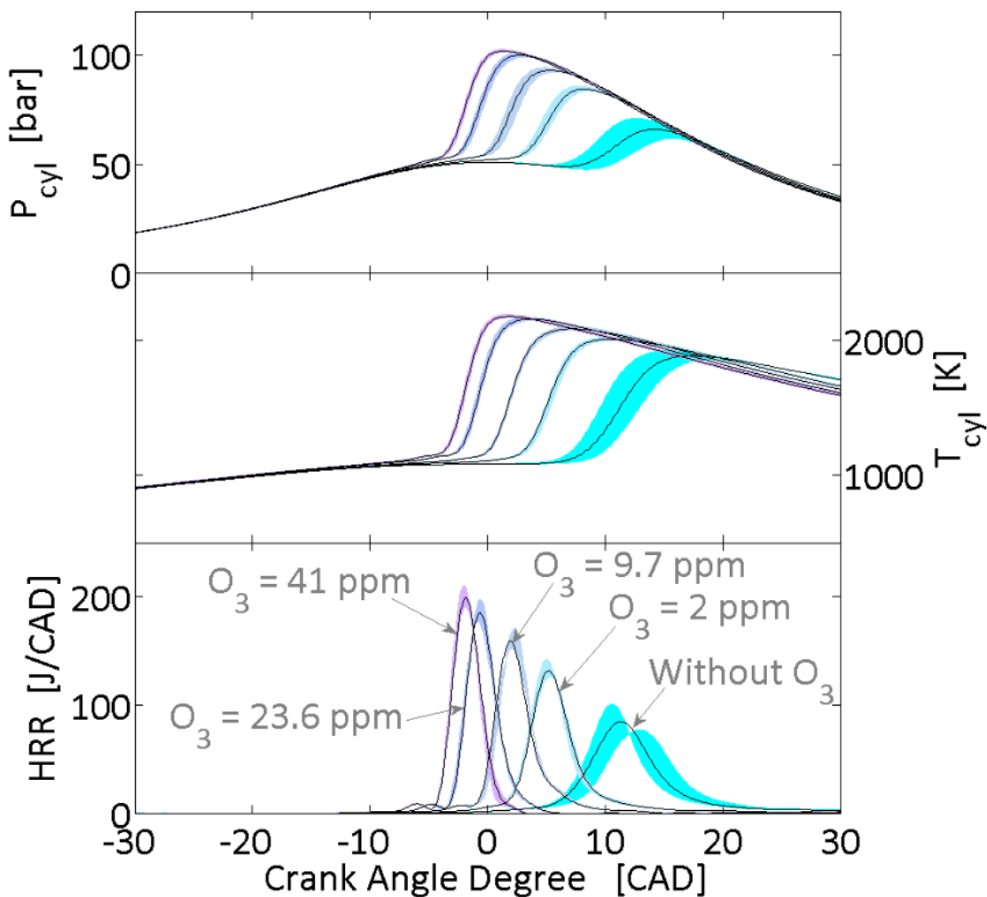
Figure 93. In-cylinder pressures, in-cylinder temperatures and heat release rates traces as a function of the ozone concentrations with an intake pressure of 1.5 bar and an intake temperature of 495 K.
