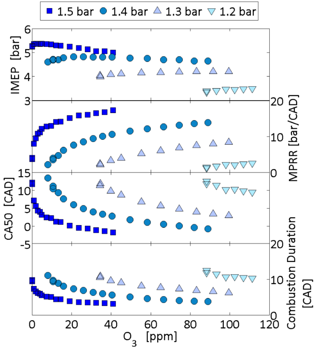
Figure 94. Engine outputs (IMEP, maximum pressure rise rate, CA50 and combustion duration) as a function of the ozone injected under various intake pressures and a constant intake temperature of 495 K.
