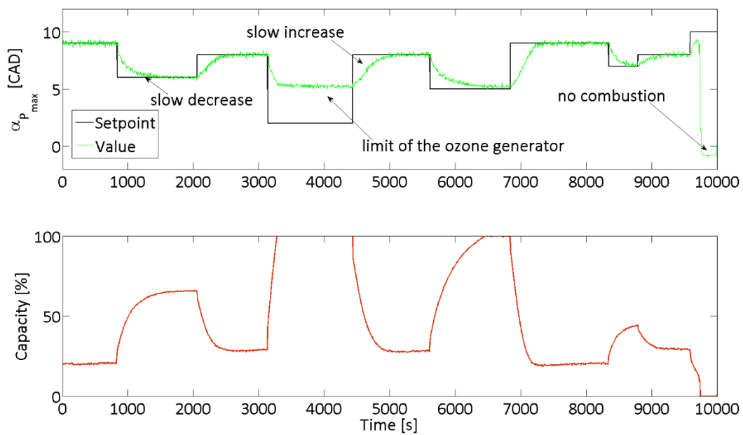
Figure 90. Dynamic control of the combustion phasing via a closed loop control approach an intake temperature of 150 °C.
