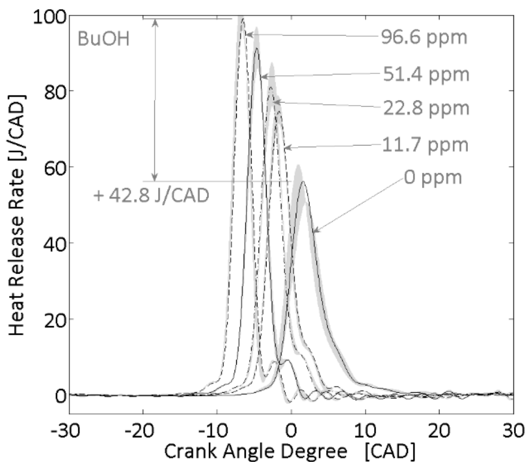
Figure 110. F. Heat release rate traces as a function of the ozone seeded for BuOH as fuel. Black curves correspond to the average of 100 cycles recorded and gray areas represent the variation of the same 100 cycles (the upper and the lower limits obtained).
