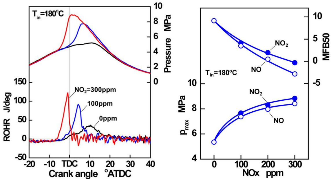
Figure 34. Effect of nitrogen dioxide on the in-cylinder pressure and heat release rate traces for natural gas as fuel (on the left). Comparison of \text{NO} and \text{NO}_2 effect on the maximum pressure and on the CA50 (on the right) [124].
