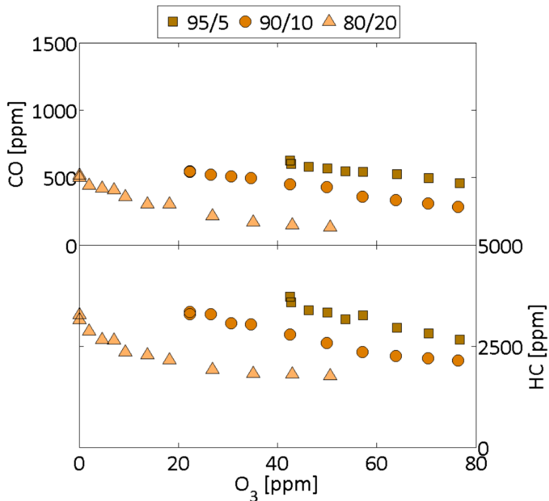
Figure 105. Carbon monoxide and unburned hydrocarbon emissions as a function of the ozone concentration under various mixtures of methane and hydrogen.
