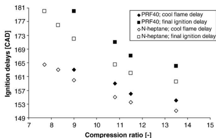
Figure 28. Influence of the compression ratio on the cool flame and main ignition delays of n-heptane and PRF40 for an intake temperature of 70 °C and an equivalence ratio of 0.33 [35].
