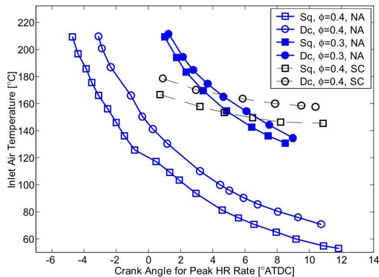
Figure 27. Intake air temperature versus combustion timing for two different piston geometries (Square: Sq and Disc: Dc). NA corresponds to Naturally Aspirated and SC to Supercharged [80].
