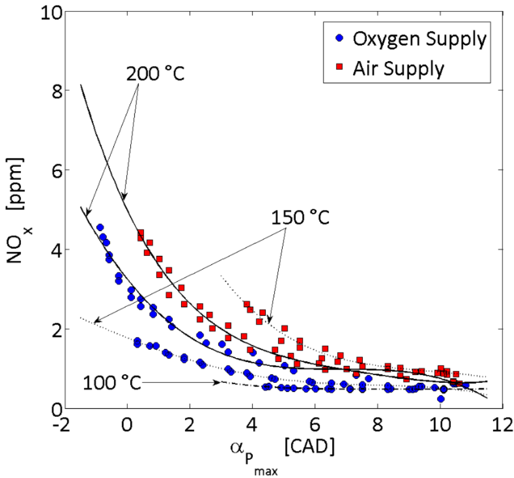
Figure 84. Nitrogen oxides trends as a function of the maximum pressure location.
