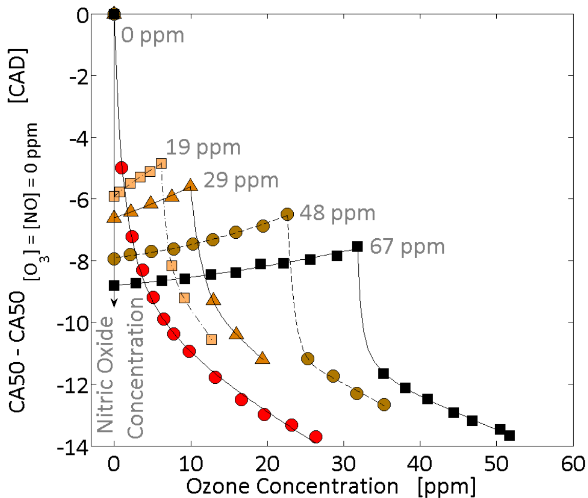
Figure 69. Shift of the CA50 in reference to the case without any seeding as a function of the nitric oxide (concentrations in grey on the graph) and ozone when the two oxidizing chemical species seed simultaneously the intake of the engine.
