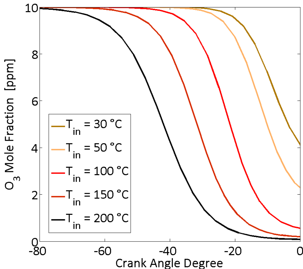
Figure 56. Computed ozone mole fraction during the compression stroke of an engine as a function of the crank angle degree under temperatures from 30 °C to 200 °C at a constant pressure of 1 bar.
