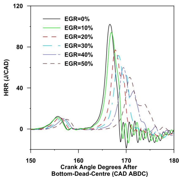
Figure 29. Effect of the EGR on the heat release rate traces for n -heptane as fuel [33].
