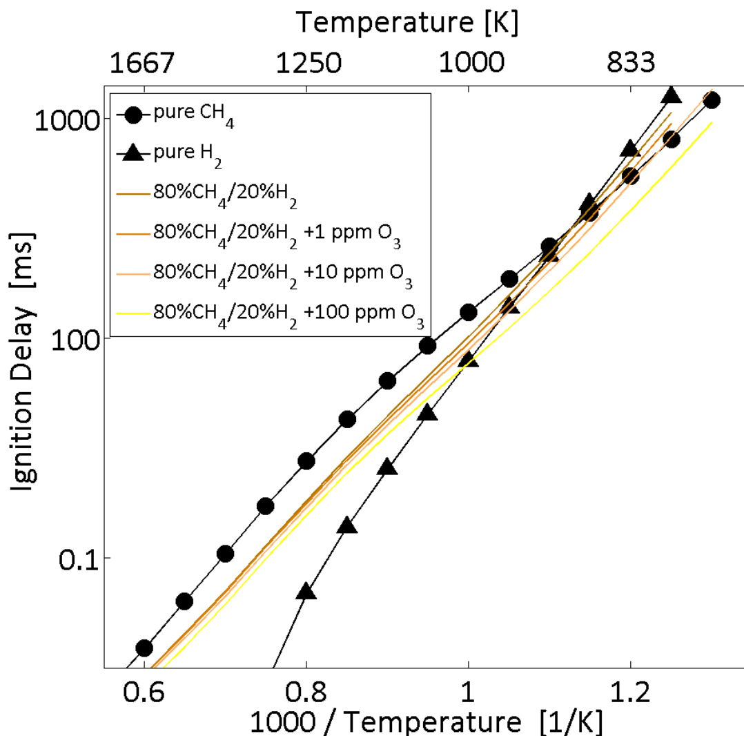
Figure 107. Ignition delays as a function of the inverse temperature for pure methane and pure hydrogen as well as mixture of methane and hydrogen with varying ozone concentrations.
