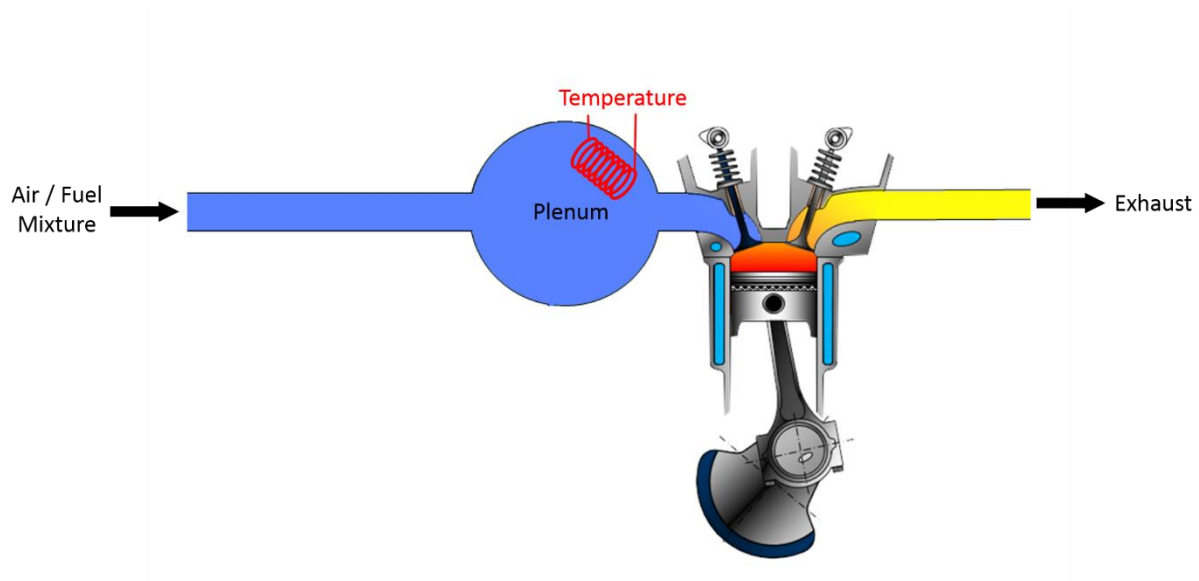
Figure 36. Scheme of the experimental setup in its normal configuration.
