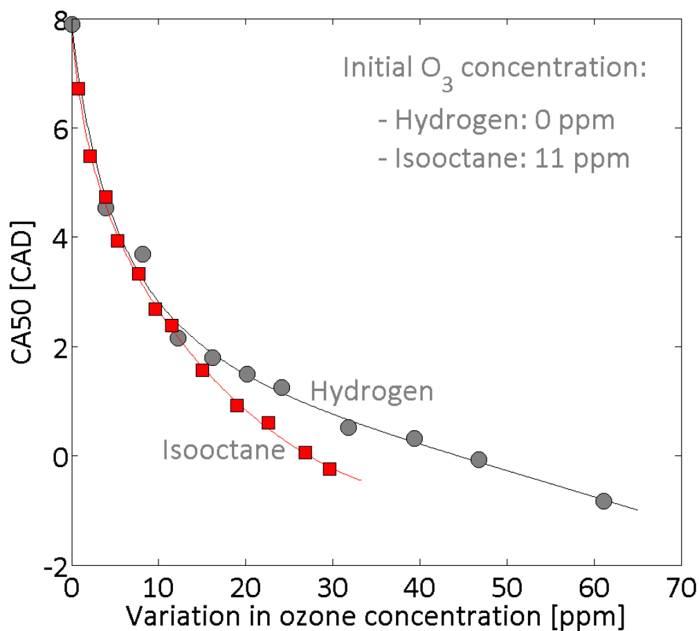
Figure 92. Effect of ozone on hydrogen and isooctane combustions for intake conditions fixed at 1 bar and 155 °C. Results for isooctane need a minimum ozone concentration to auto-ignite under these conditions. The ozone concentration axis for isooctane results were therefore shifted and adapted to start with the same initial CA50. The two trends must be therefore analyzed as a function of a variation of the ozone concentration.
