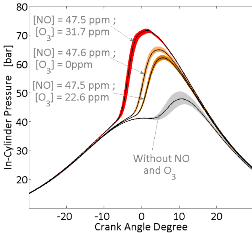
Figure 68. A. In-cylinder pressure traces as a function of the crank angle degree for several couple of concentration in ozone and nitric oxide simultaneously seeded in the intake of the engine.
