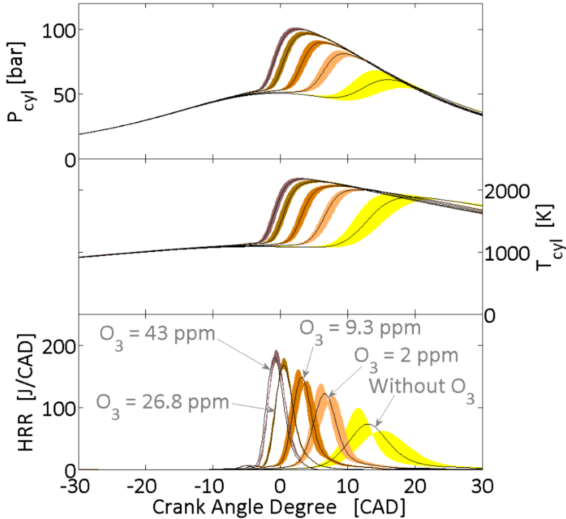
Figure 103. In-cylinder pressures, in-cylinder temperatures and heat release rates traces as a function of the ozone concentration for a mixture of methane and hydrogen (80/20), an intake pressure of 1.5 bar and an intake temperature of 495 K.
