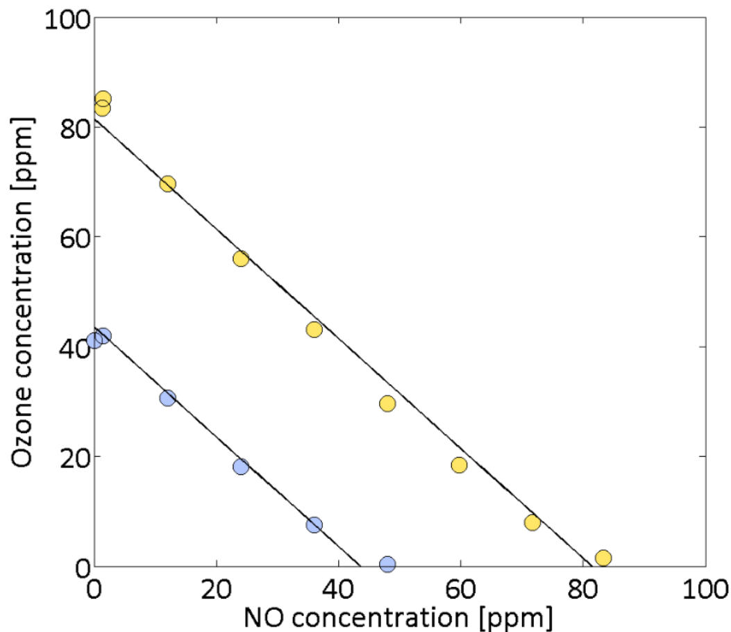
Figure 71. Ozone concentrations measured at the intake of the engine as a function of the nitric oxide concentration injected into the plenum for two different initial concentration of ozone. Blue markers correspond to an initial ozone concentration of approximately 40 ppm and yellow markers to an initial ozone concentration around 80 ppm.
