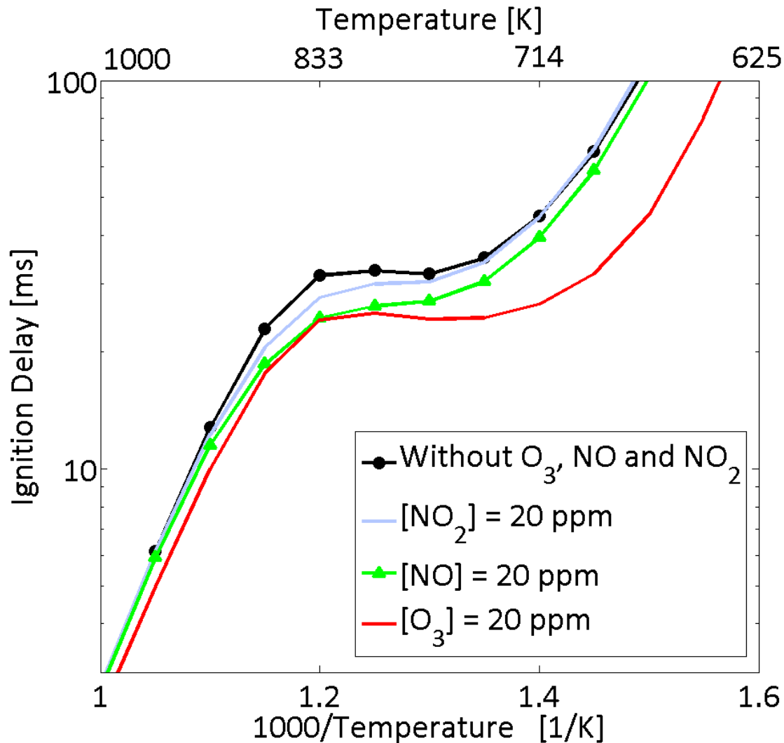
Figure 66. Ignition delays computed over a large temperature range, for isooctane as fuel with an equivalence ratio of 0.3, for an initial pressure of 40 bar and 20 ppm of each oxidizing chemical species studied.
