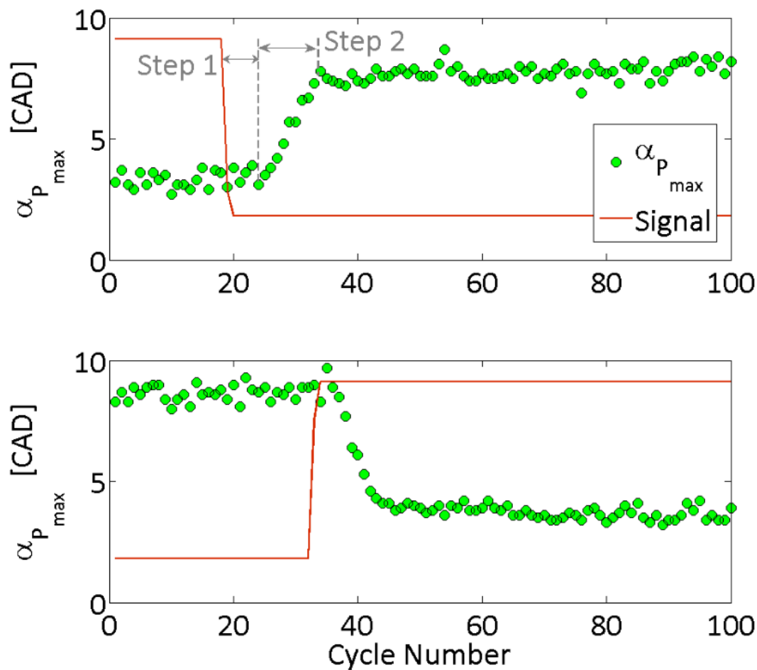
Figure 86. Cycle-to-cycle variations for an increase and a decrease of the combustion phasing. Dots correspond to the maximum pressure phasing at each cycle and lines correspond to the signal on the ozone generator. Step 1 and step 2 correspond to the transitional time.
