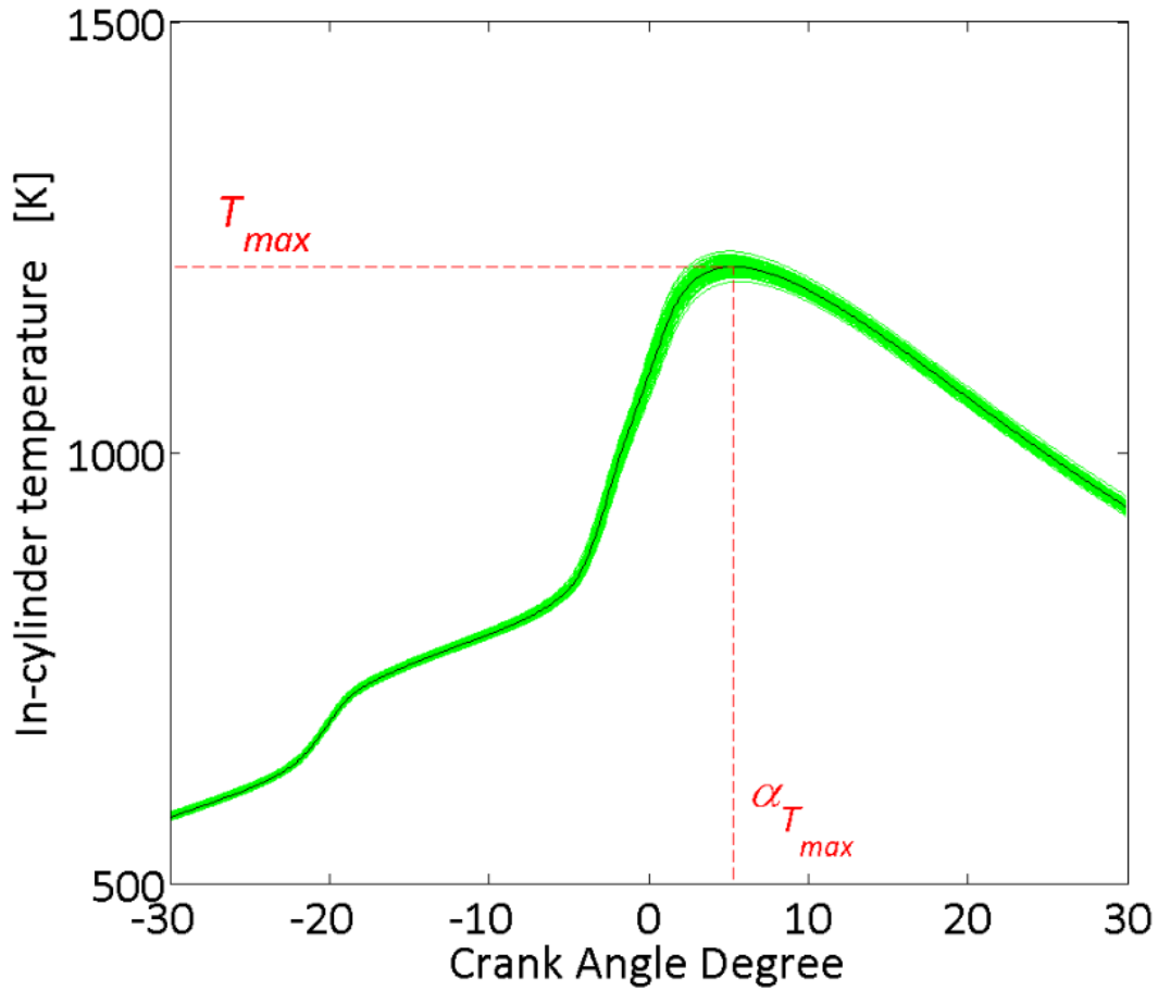
Figure 45. Example of an in-cylinder temperature trace as a function of the crank angle. Green area corresponds to the 100 cycles recorded while the black line corresponds to the average of the same 100 cycles. The maximum temperature ( T_{max} ) inside the combustion is determined from this average as well as its phasing ( \alpha_{T_{max}} ).
