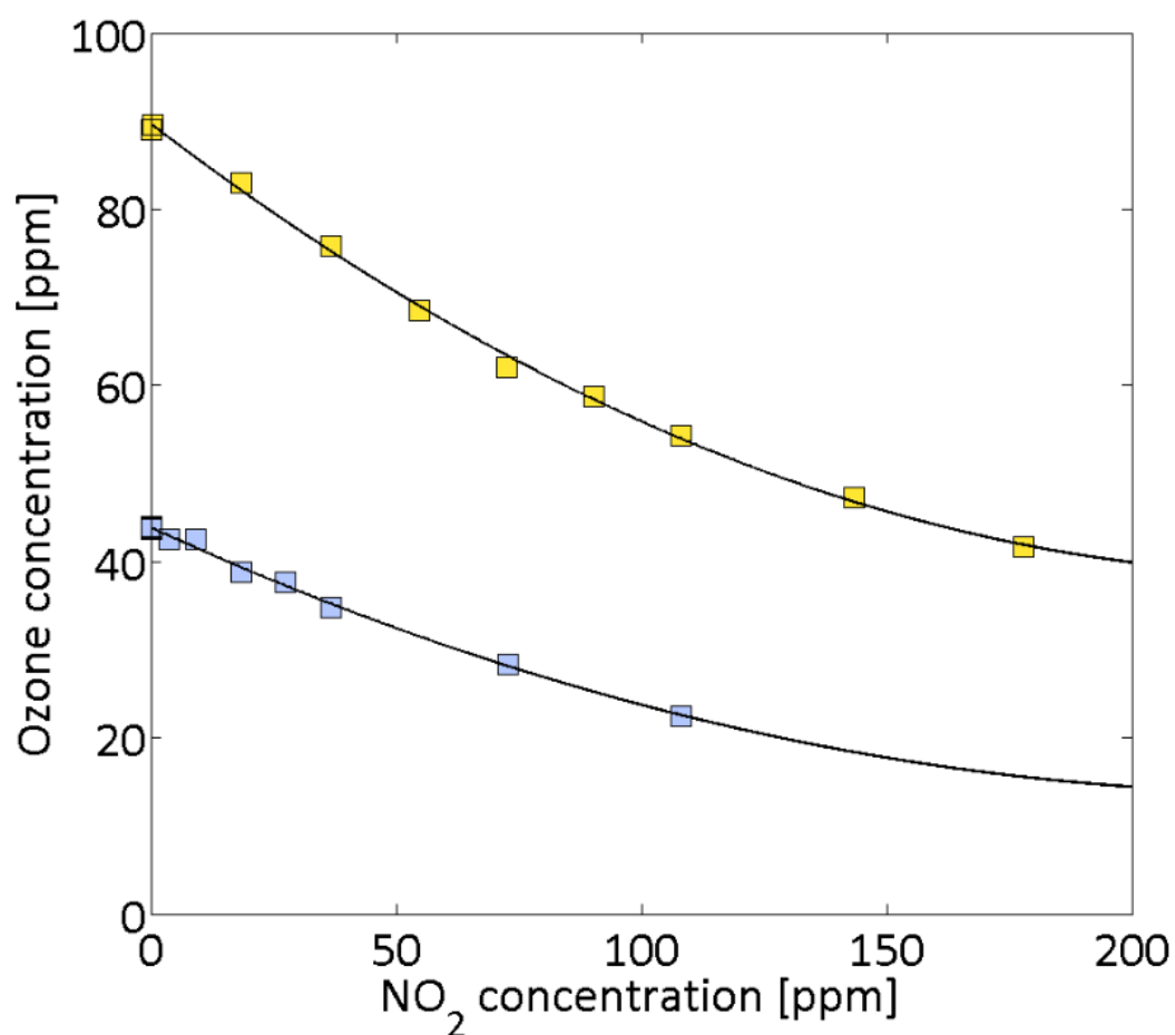
Figure 74. Ozone concentrations measured at the intake of the engine as a function of the nitrogen dioxide concentration injected into the plenum for two different initial concentration of ozone. Blue markers correspond to an initial ozone concentration of approximately 40 ppm and yellow markers to an initial ozone concentration around 90 ppm.
