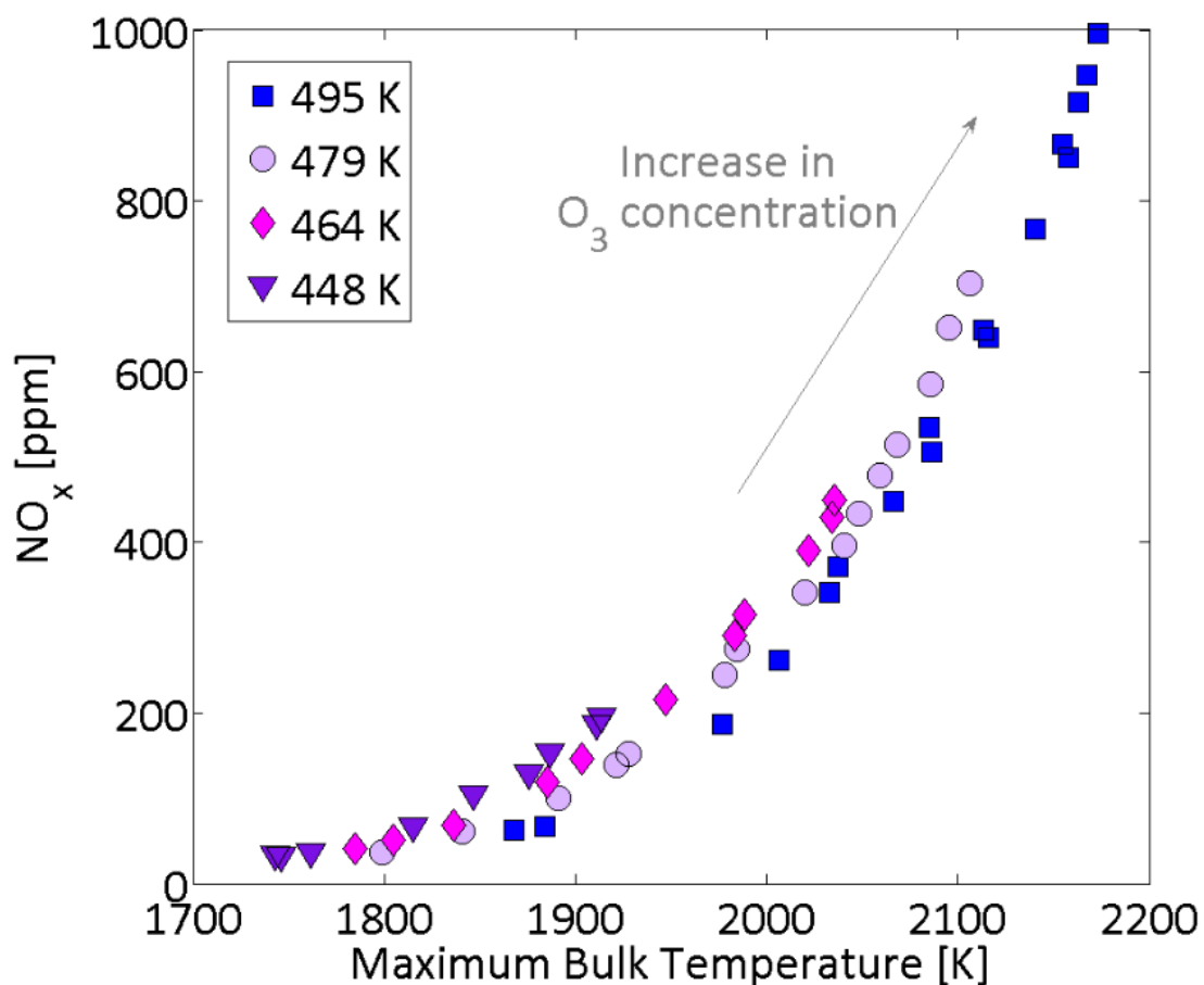
Figure 99. Emissions of nitric oxide measured at the exhaust of the engine as a function of the maximum bulk temperature estimated under a wide range of intake temperature and for a constant intake pressure of 1.5 bar.
