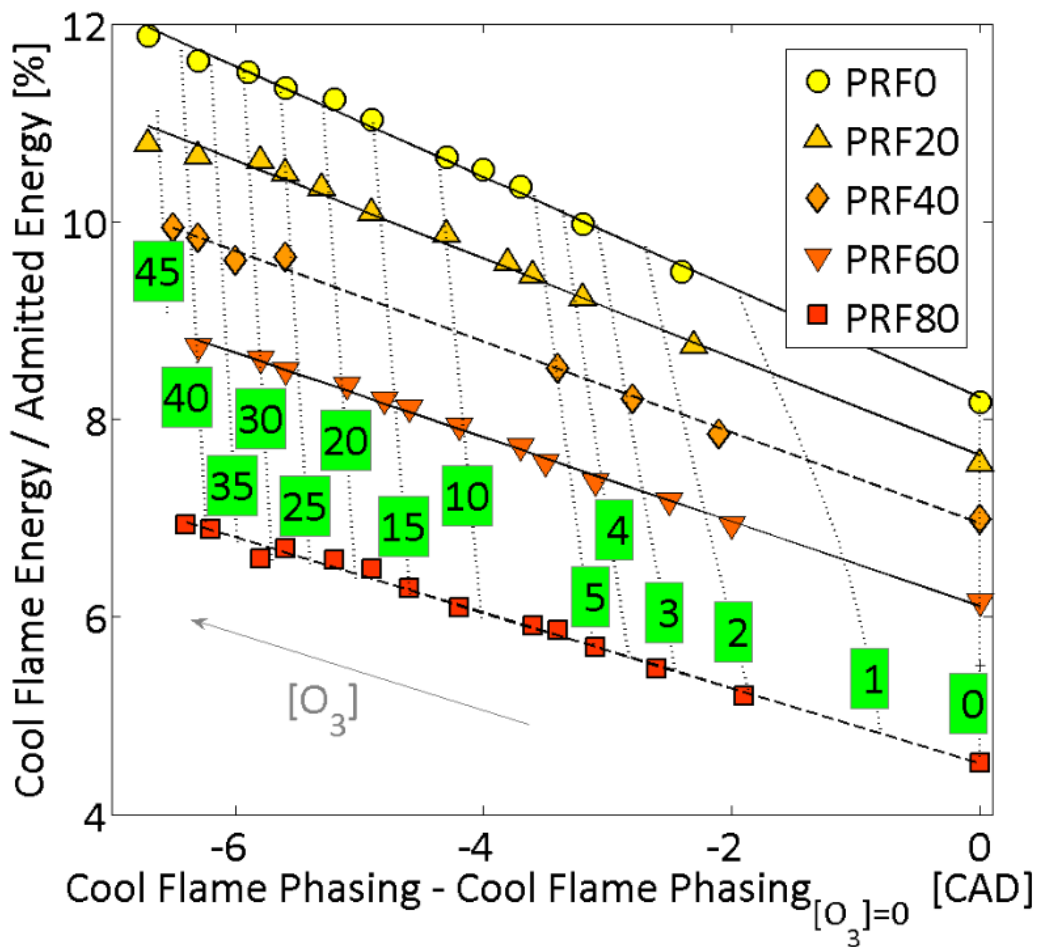
Figure 54. Ratio between the cool flame energy released and the total energy released as a function of the cool flame shift and the ozone seeding into the intake.
