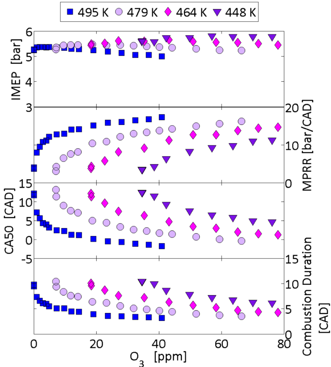
Figure 97. Engine outputs (IMEP, maximum pressure rise rate, CA50 and combustion duration) as a function of the ozone injected under various intake temperatures and a constant intake pressure of 1.5 bar.
