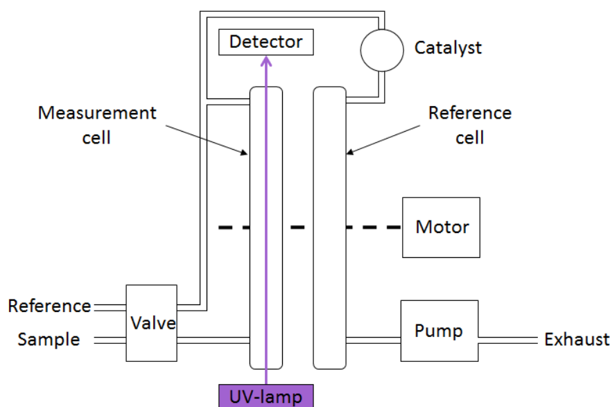
Figure 38. Scheme of the ozone analyzer used.
