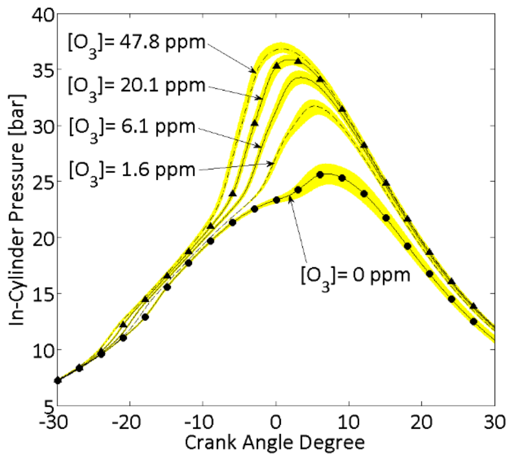
Figure 51. A. In-cylinder pressure evolutions as a function of the ozone concentration injected in the intake of the engine for n -heptane/PRF0 as fuel.
