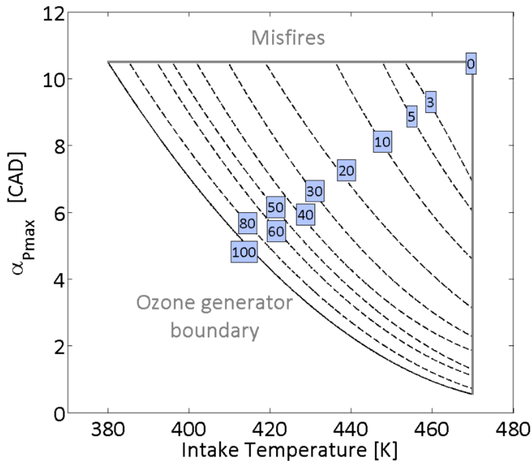
Figure 85. Cartography of the ozone generator capacity needed to achieve a maximum pressure location under various intake temperatures of the engine. This map is based on all the experimental data previously obtained with air as gas supply for the ozone generator and with extra ones near the boundaries displayed.
