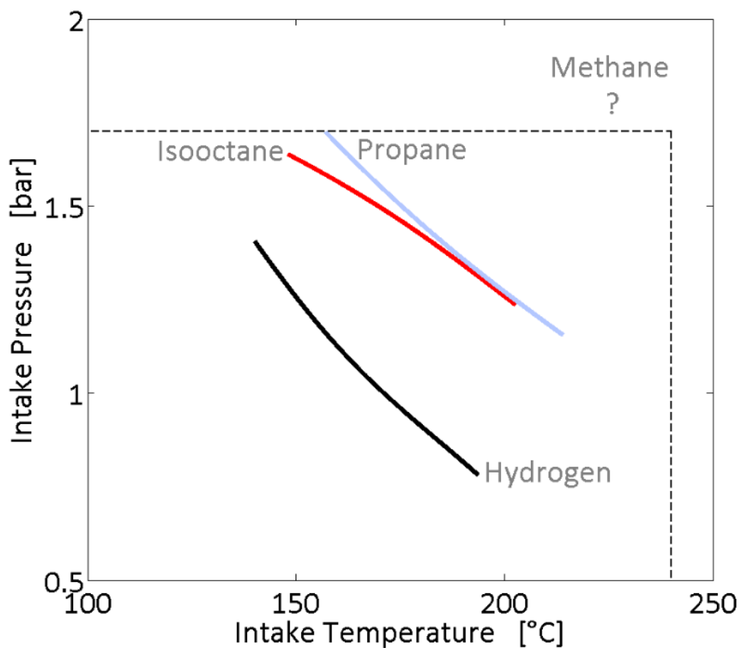
Figure 91. IsoCA50s located at the top dead center for the gaseous fuels selected as a function of the intake pressure and intake temperatures, an equivalence ratio of 0.3 and a rotation speed of 1500 rpm. Dotted lines correspond to the operating limits of the engine bench.
