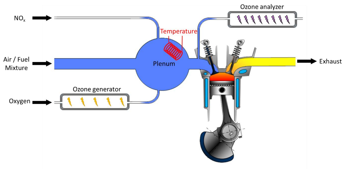
Figure 39. Scheme of the experimental setup with the injection locations of both ozone and nitrogen oxides and the position for the sample of the ozone analyzer.
