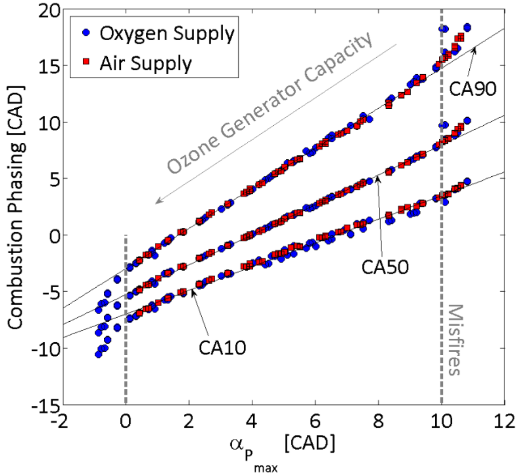
Figure 79. CA10, CA50 and CA90 as a function of the maximum pressure location for both types of gas supply, for an injection inside the intake pipe and the three intake temperatures tuned.
