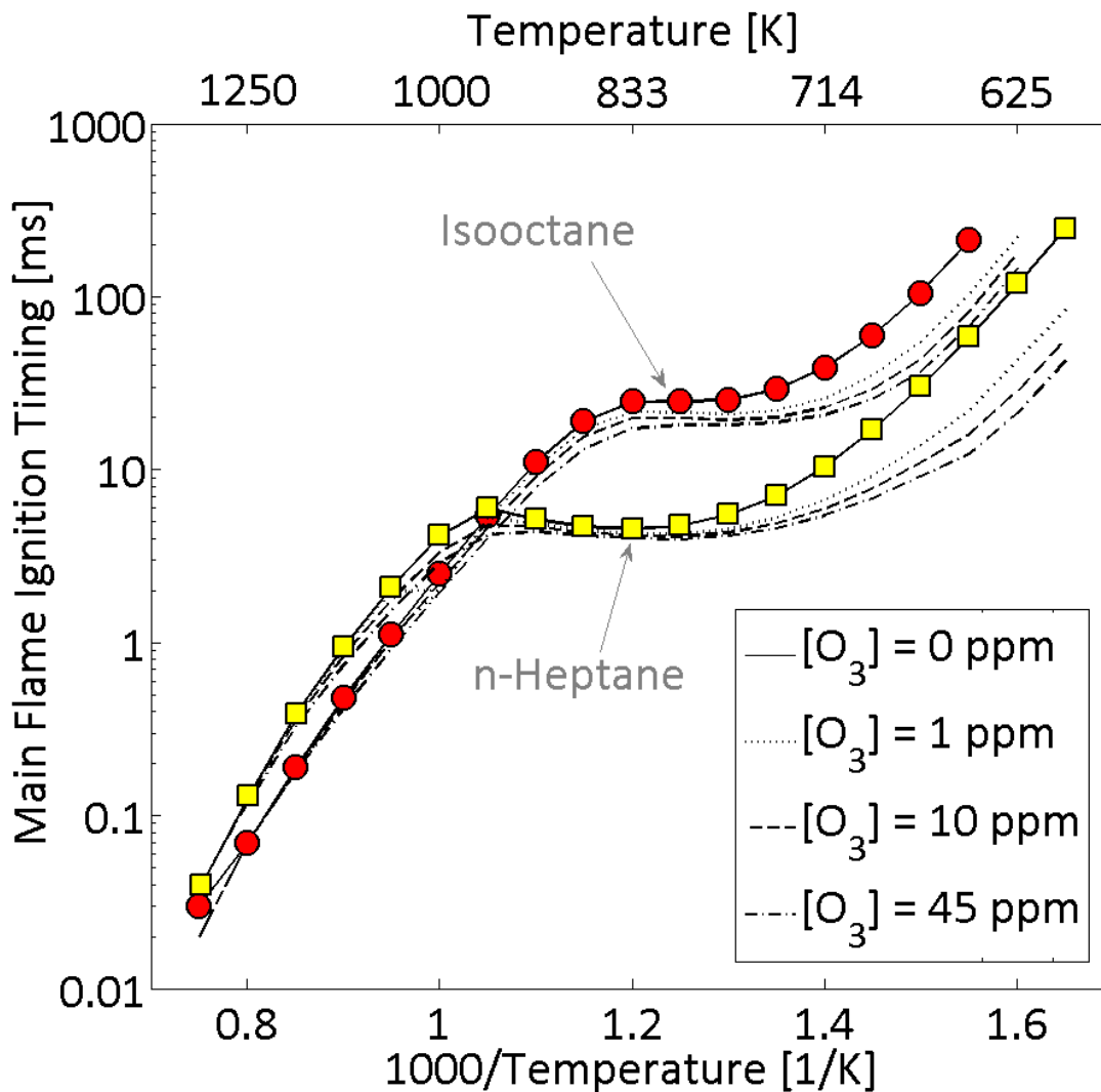
Figure 57. Computed main flame ignition timing as a function of the inverse temperature for various ozone concentrations. “□” symbols and curves under this result correspond to PRF0 as fuel, and “○” symbols and curves under this result correspond to PRF100 as fuel.
