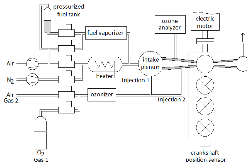
Figure 75. Scheme of the experimental setup for the application case. The ozone generator may be supplied either by pure oxygen or air and the ozone produced can be injected either inside the plenum or into one of the intake pipes.
