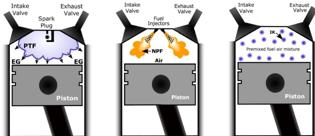
Figure 17. Scheme of both conventional engines combustion compared to the HCCI combustion. From the left to the right: Spark Ignition, Compression Ignition and Homogeneous Charge Compression Ignition [26]. (PTF: Premixed Turbulent Flame; EG: End Gases; NPF: Non-Premixed Flame; IK: Ignition Kernels)
