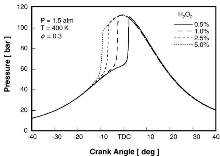
Figure 32. Impact of hydrogen peroxide additions on methane combustion [116].
