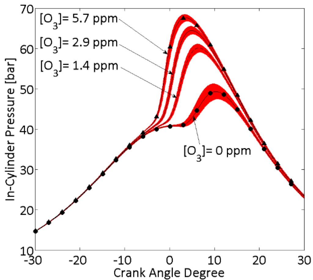
Figure 51. C. In-cylinder pressure evolutions as a function of the ozone concentration injected in the intake of the engine for isooctane/PRF100 as fuel.
