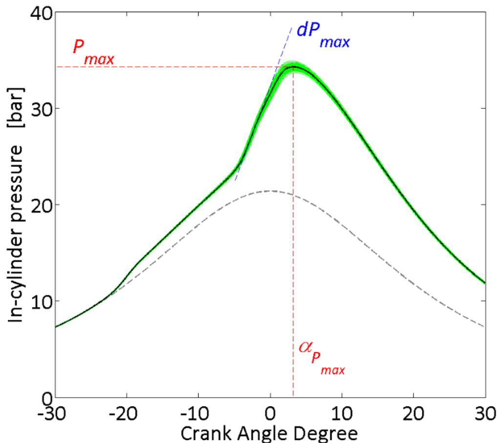
Figure 44. Example of an in-cylinder pressure trace as a function of the crank angle. Dotted line corresponds the motoring trace of the pressure in average inside the combustion chamber. Green area represents the 100 cycles recorded while the black line is the average of the same 100 cycles. From the average trace, the maximum in-cylinder pressure ( P_{max} ) is determined as well as its phasing ( \alpha_{P_{max}} ) and finally the maximum pressure gradient ( dP_{max} ) determines from the derivative of the in-cylinder pressure trace.
