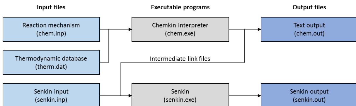
Figure 47. Structure of the Senkin program.
