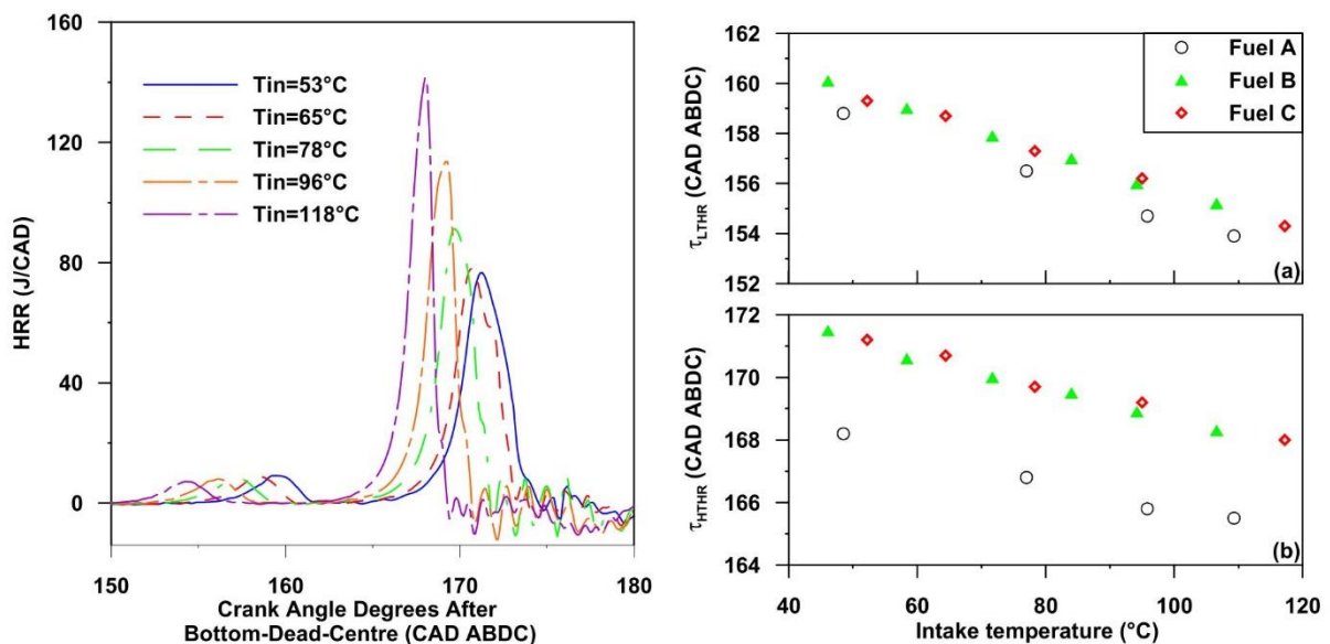
Figure 19. Effect of the intake temperature on heat release rate for TRF24 as fuel (on the left) and effect of the intake temperature on combustion timing (on the right). Results on the top correspond to the cool flame and those on the bottom to the main flame. Fuels A, B and C represent n -heptane, PRF25 and TRF24, respectively [33].
