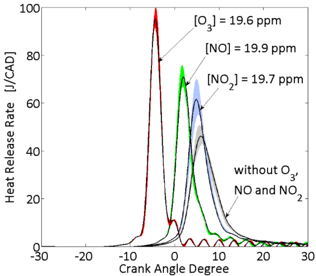
Figure 64. B. Heat release rate traces without any species seeded and with 20 ppm of each oxidizing chemical species ( O_3 : ozone, NO : nitric oxide and NO_2 : nitrogen dioxide) separately injected.
