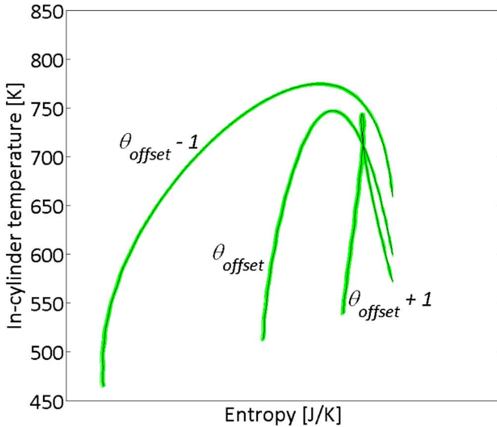
Figure 42. Temperature-Entropy diagram under various offset on the crank angle. A wrong offset creates an expansion of the diagram or a loop. Both results have no thermodynamic sense. A good offset results in the symmetry desired.
