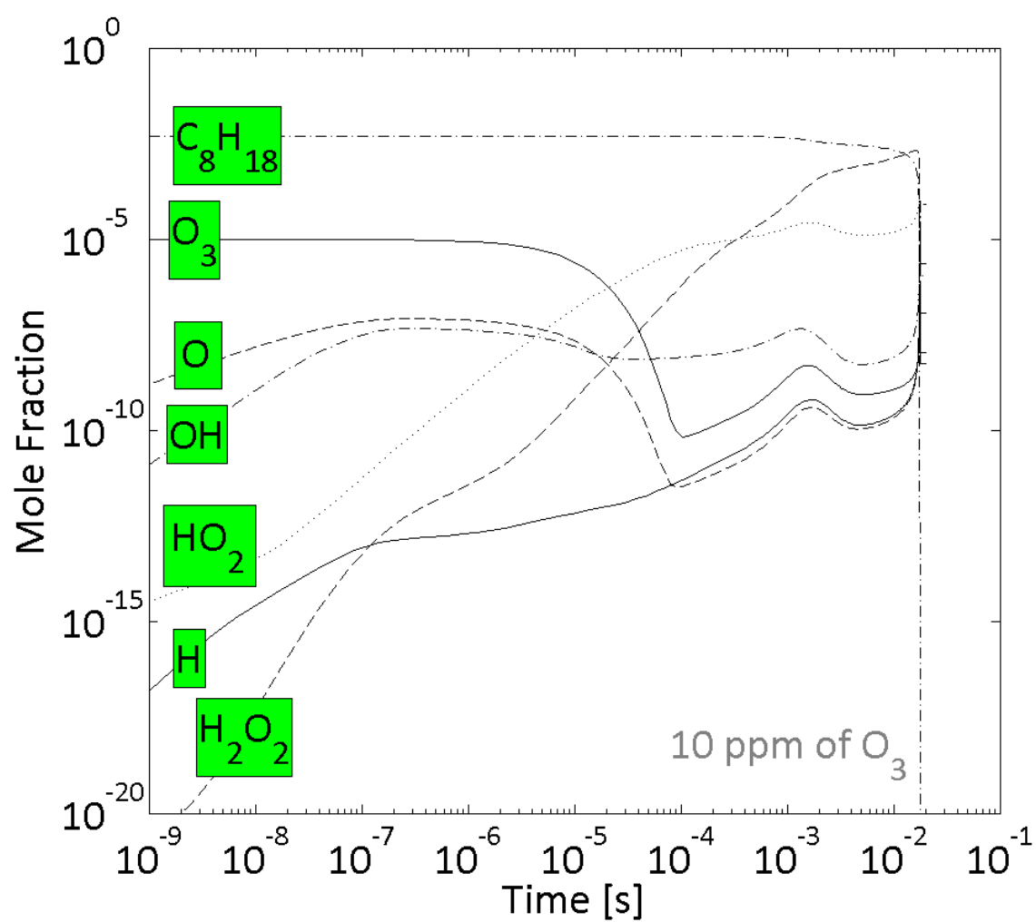
Figure 58. C. Mole fractions of the main radicals and the fuel for isooctane (PRF100) at an initial temperature of 800 K, initial pressure of 50 bar, an equivalence ratio of 0.3 and with 10 ppm of ozone.
