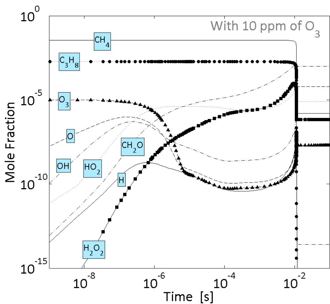
Figure 101. C. Mole fractions for a mixture of methane and propane (95/5) with 10 ppm of ozone.
