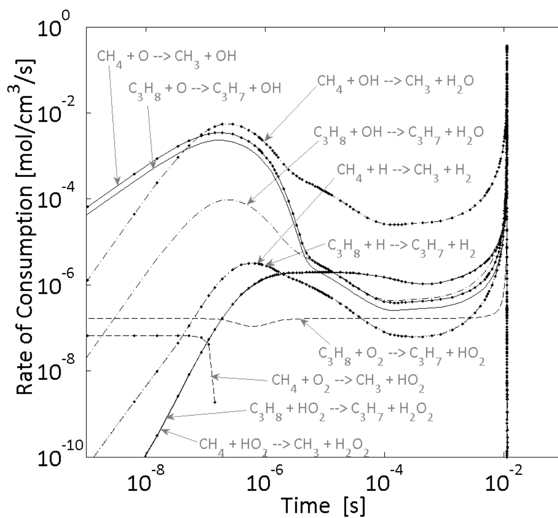
Figure 101. D. Rate of consumption for a mixture of methane and propane (95/5) with 10 ppm of ozone.
