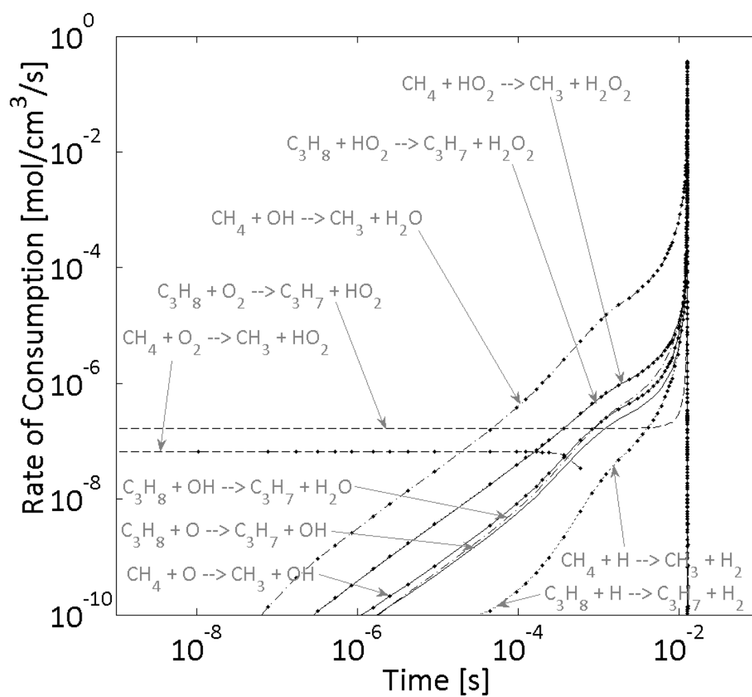
Figure 101. B. Rate of consumption for a mixture of methane and propane (95/5) without ozone.
