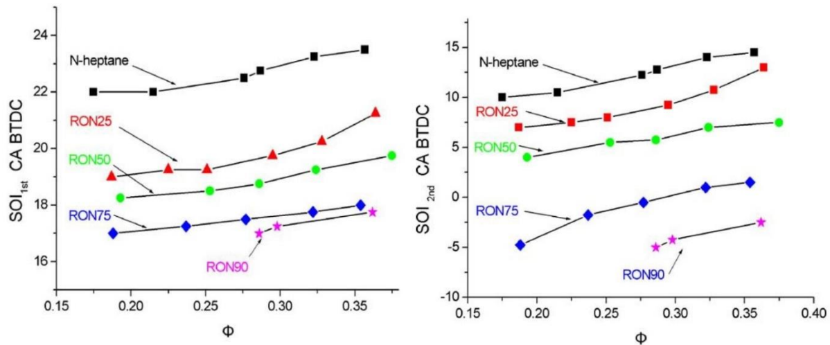
Figure 21. Ignition timing of both cool flames (on the left) and main flames (on the right) for several PRFs as a function of the equivalence ratio [49].
