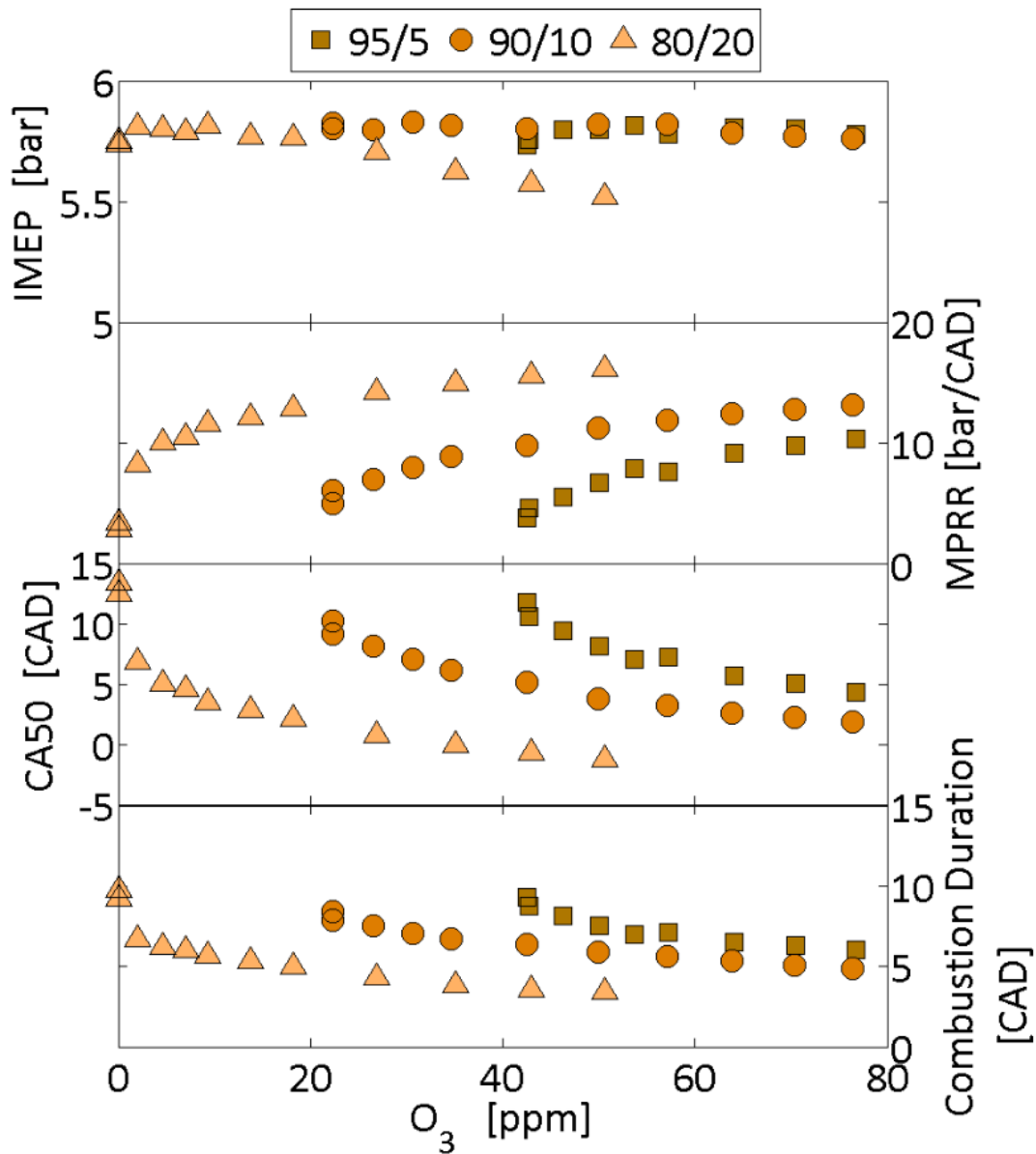
Figure 104. Engine outputs (IMEP, maximum pressure rise rate, CA50 and combustion duration) as a function of the ozone concentration under various mixtures of methane and hydrogen.
