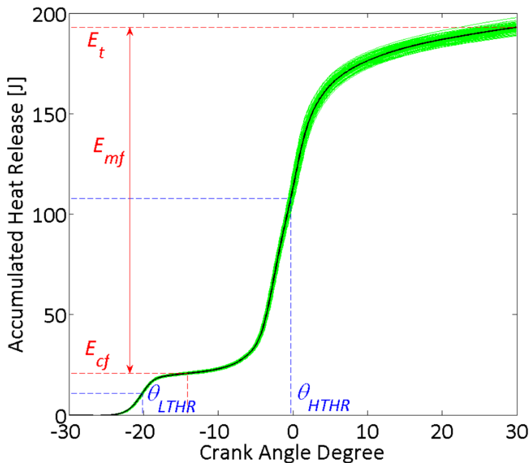
Figure 46. Example of an accumulated heat release as a function of the crank angle for a case with a cool flame. Green area corresponds to the 100 cycles recorded and the black line to the average of the same 100 cycles. The energy released by the cool flame is determined as the energy released from the start of the combustion up to the lower energy released between the two peaks of combustion observed on the heat release rate trace. The energy released by the main flame therefore corresponds to the difference between the total energy released and the energy released by the cool flame. Finally, phasing of each flame respectively corresponds to the crank angle where the half of the energy of each flame has been released.
