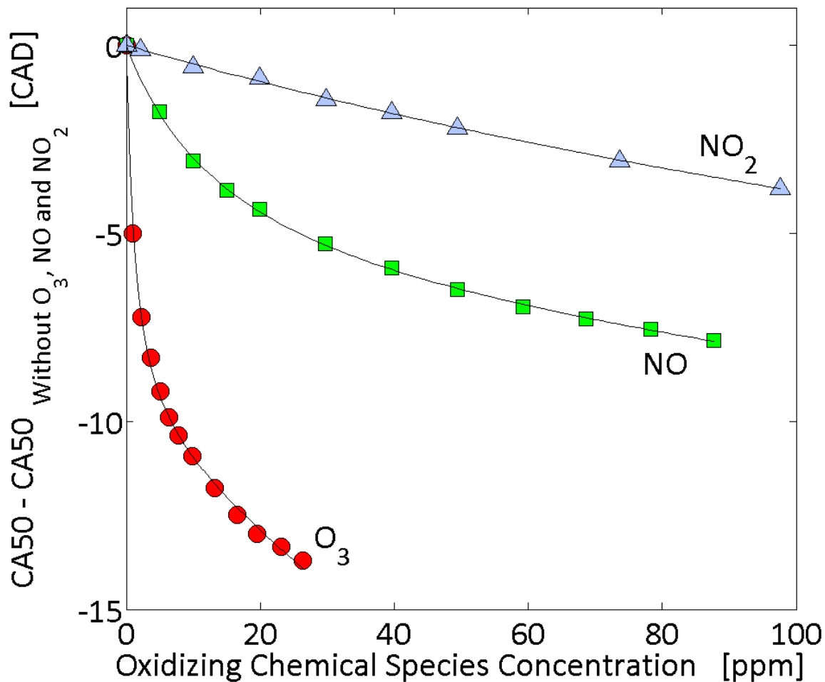
Figure 65. Shift of the CA50 as a function of the three oxidizing chemical species ( O_3 : ozone, NO: nitric oxide and NO_2 : nitrogen dioxide) when they are separately injected.
