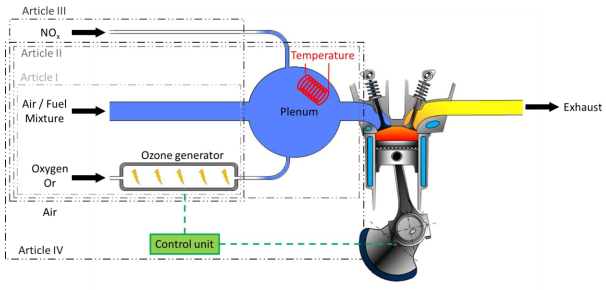
Figure 49. Graphical abstract on the plan of the chapter 3 from the published results.
