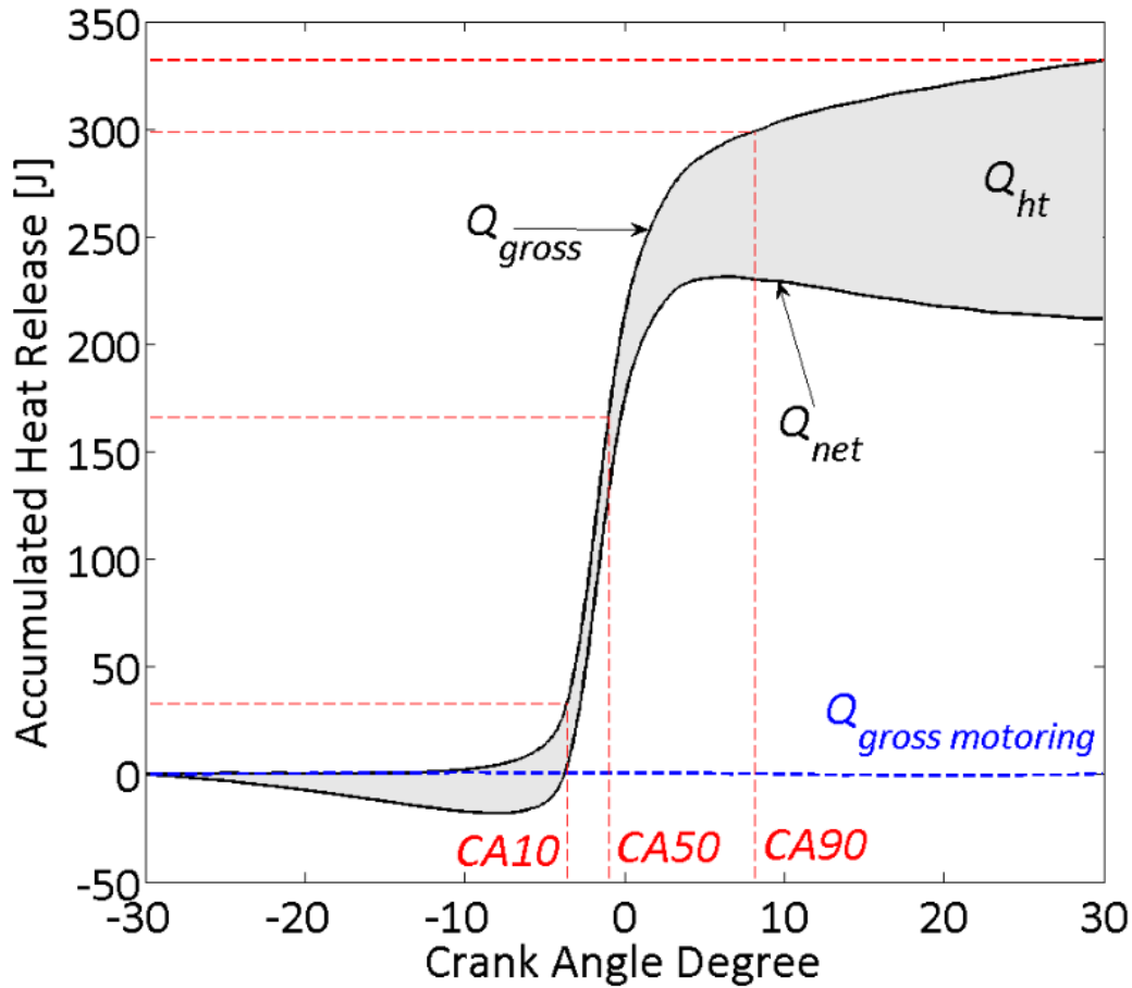
Figure 43. Example of an accumulated heat release as a function of the crank angle degree. Each curve corresponds to an average of the heat release. The blue one represents the gross heat release in the case of a motoring. For a combustion case, the gross heat release has been broken down into the net heat release and the heat transfers to the wall (grey area). CA10, CA50 and CA90 are respectively defined as the crank angle where 10, 50 and 90 % of the total energy released has been consumed.
