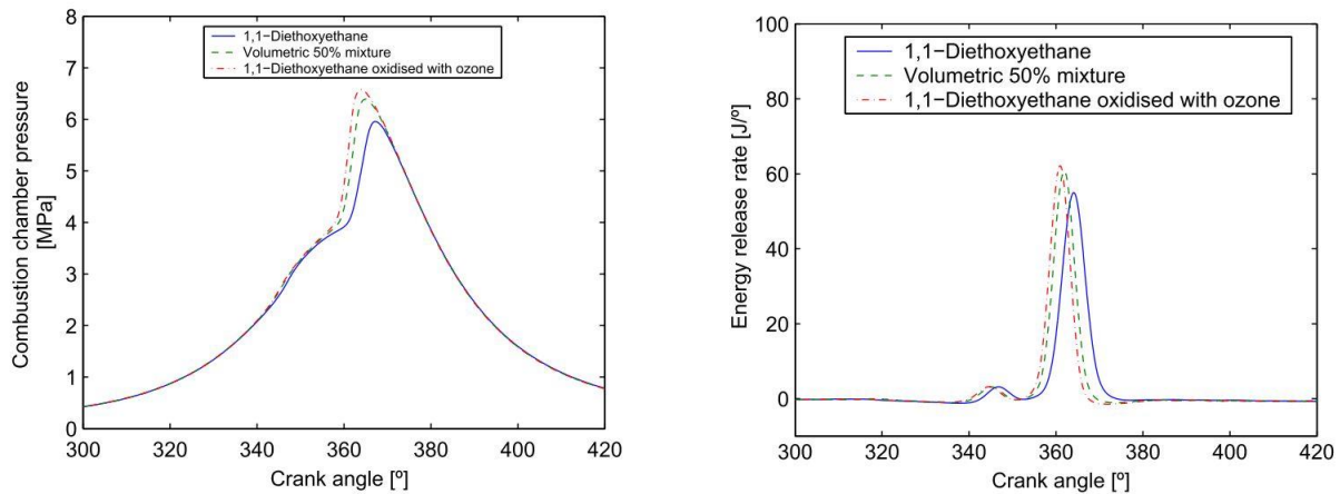
Figure 31. Impact of varying the proportion of pure fuel and modified fuel into an HCCI engine [113].
