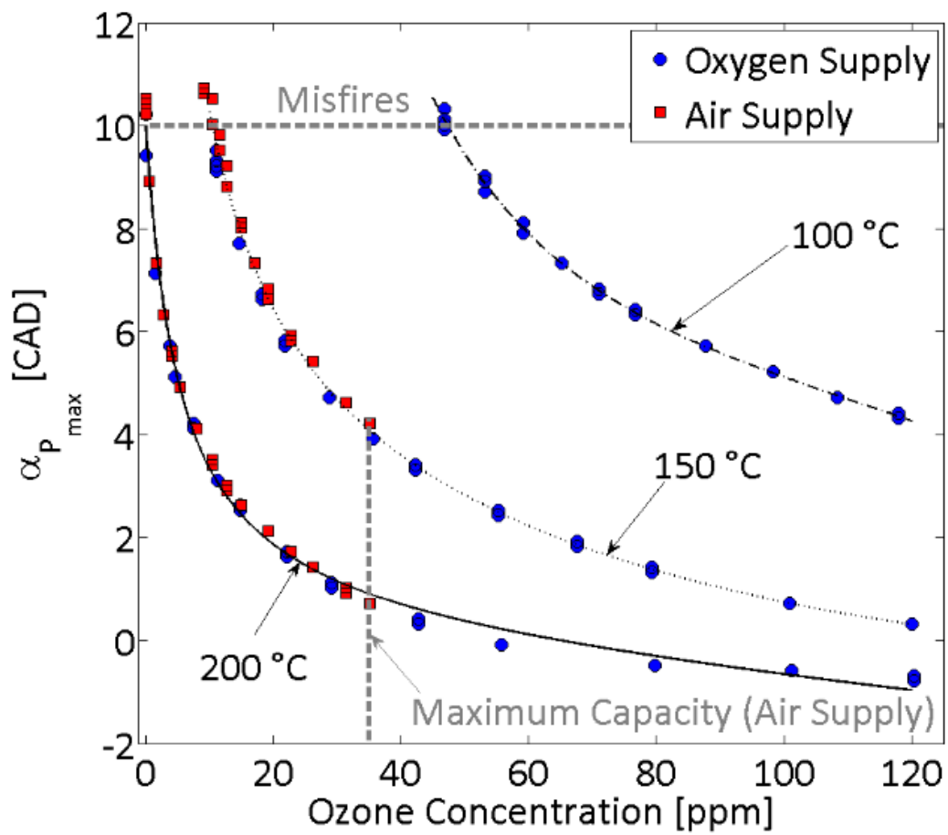
Figure 77. B. Phasing of the maximum pressure location as a function of the ozone concentration for an oxygen supply and an air supply.
