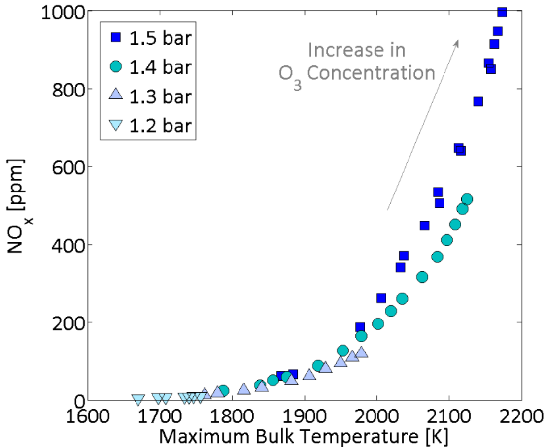
Figure 96. Nitric oxides measured at the exhaust of the engine as a function of the maximum bulk temperature estimated under various intake pressures and a constant intake temperature of 495 K.
