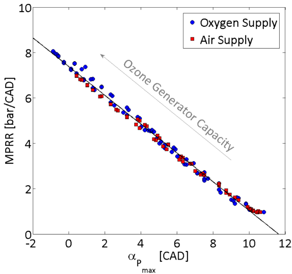
Figure 81. Maximum pressure rise rate as a function of the maximum pressure phasing for both types of gas supply, an injection inside the intake of the engine and the three intake temperatures selected.
