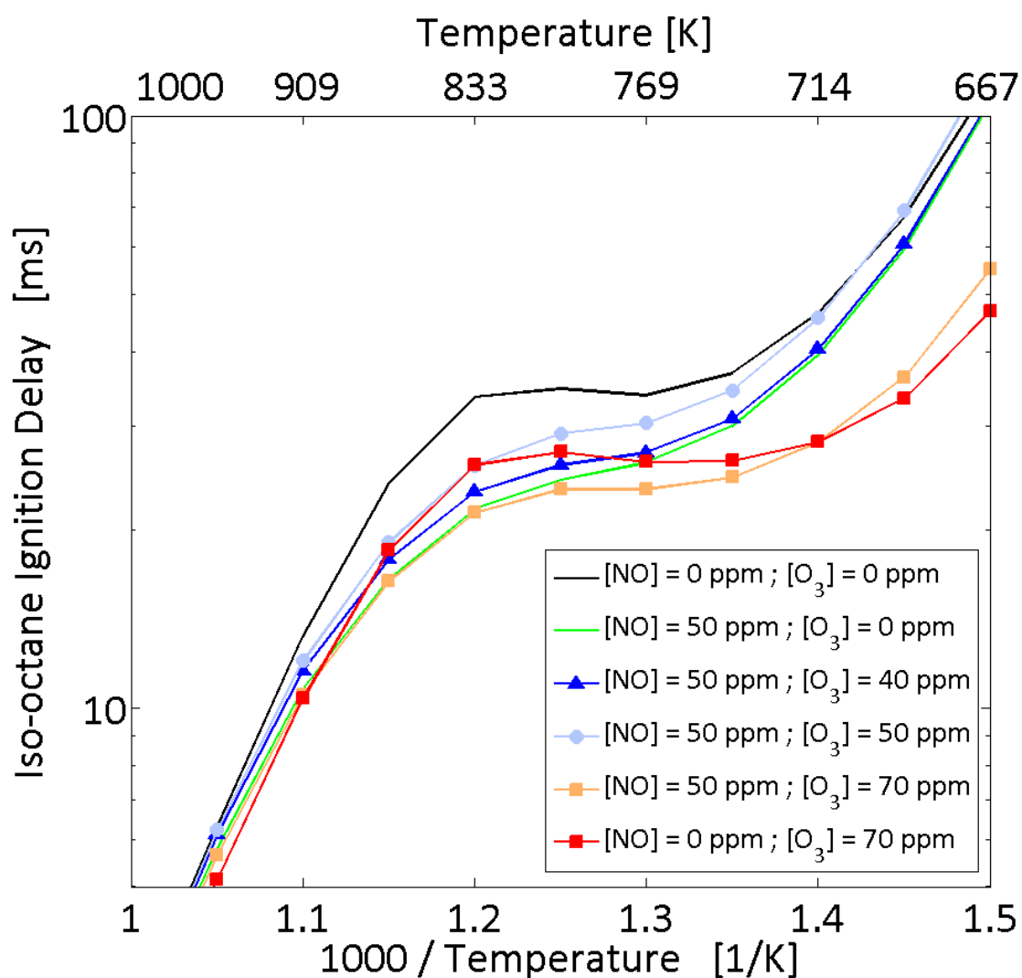
Figure 73. Ignition delays computed in two steps over a wide range of temperature and under various nitric oxide and ozone concentrations.
