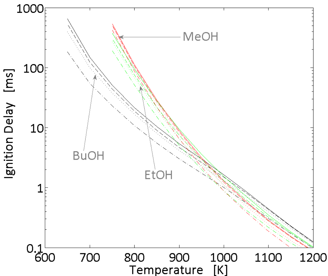
Figure 117. Ignition delays computed as a function of the temperature and the ozone concentration for the three alcohol fuels studied, for a pressure of 35 bar and an equivalence ratio of 0.3. Solid lines correspond to a concentration of 0 ppm, dashed lines to a concentration of 1 ppm, dotted lines to a concentration of 10 ppm and dash-dot lines to a concentration of 100 ppm.
