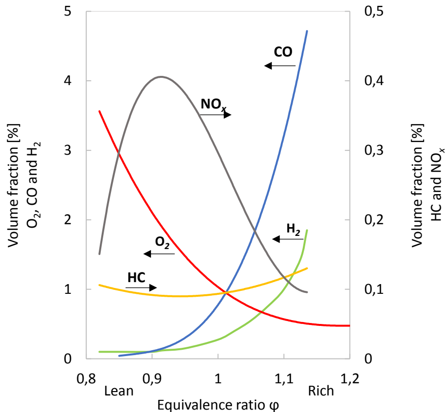
Figure 15. Typical emissions from SI engines as a function of the equivalence ratio [14].
