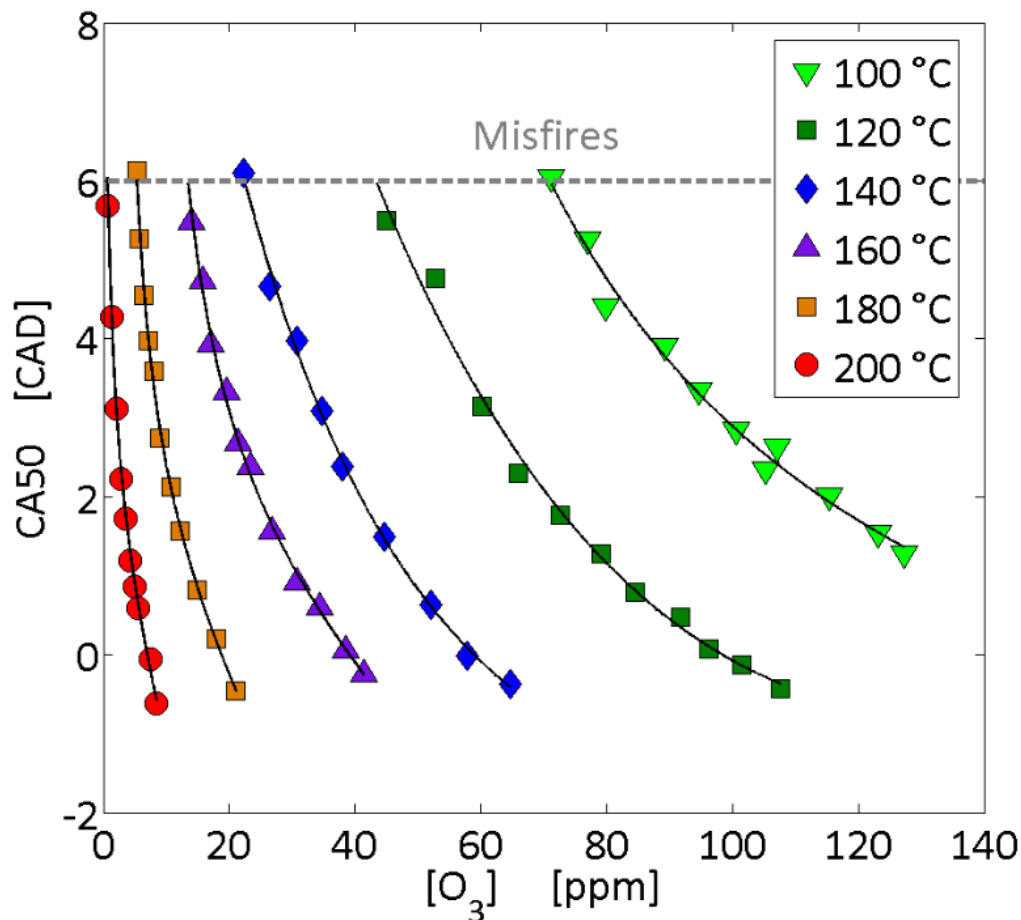
Figure 61. Evolution of the CA50 as a function of ozone concentrations for different intake temperatures at a constant pressure of 1 bar.
