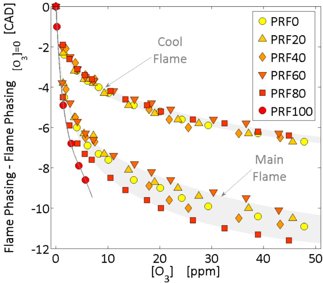
Figure 52. Shift of the low temperature heat release (LTHR) and high temperature heat release (HTHR) as a function of the ozone concentration at the intake of the engine for each PRF in reference to the initial combustion phasing of each one without ozone.
