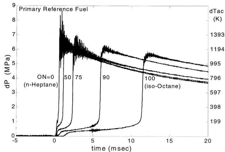
Figure 20. HCCI characteristics of PRFs for an equivalence ratio of 0.4, an intake pressure of 1 bar, an intake temperature of 318 K and a compression ratio of 16 [37].
