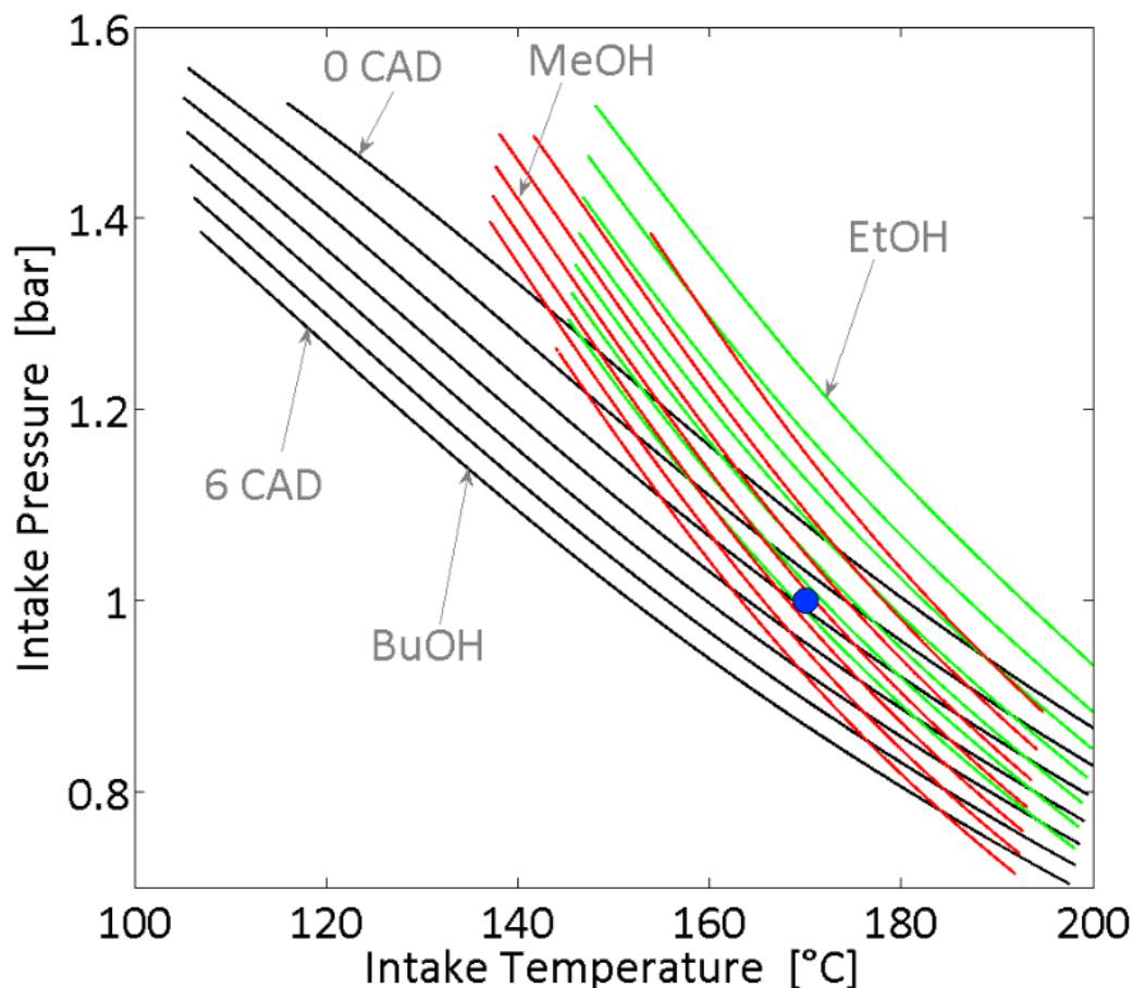
Figure 109. IsoCA50s from 0 to 6 CAD for the three alcohol fuels selected (MeOH, EtOH and BuOH) as a function of the intake pressure and the intake temperature of the engine, for an equivalence ratio of 0.3 and a rotation speed of 1500 rpm.
