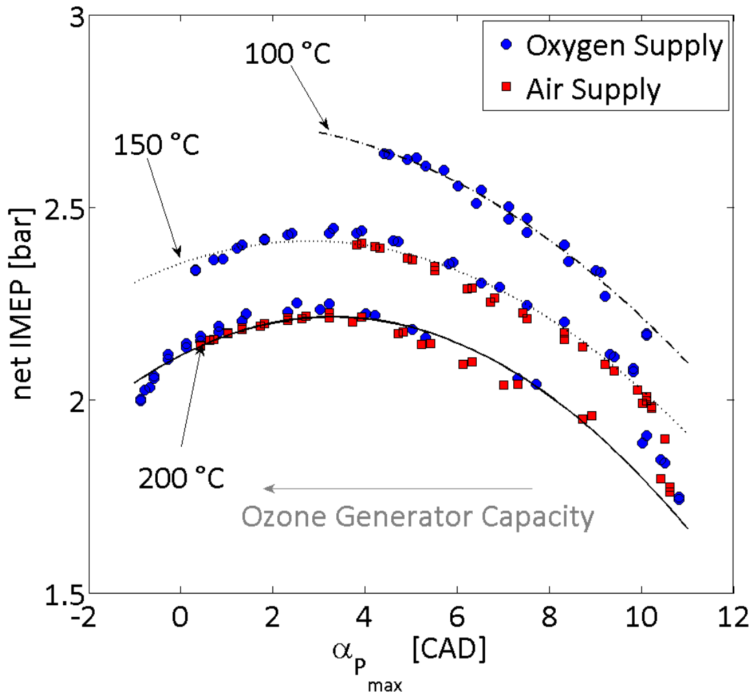
Figure 80. Net indicated mean effective pressure as a function of the maximum pressure location for both types of gas supply, an injection inside the intake pipe and the three intake temperatures.
