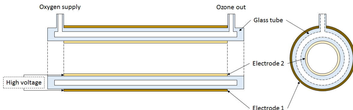
Figure 37. Scheme of the ozone generator.
