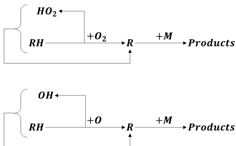
Figure 59. Initial reactions involving alkane fuel oxidation in the case without ozone seeding (top) and with ozone seeding (bottom).
