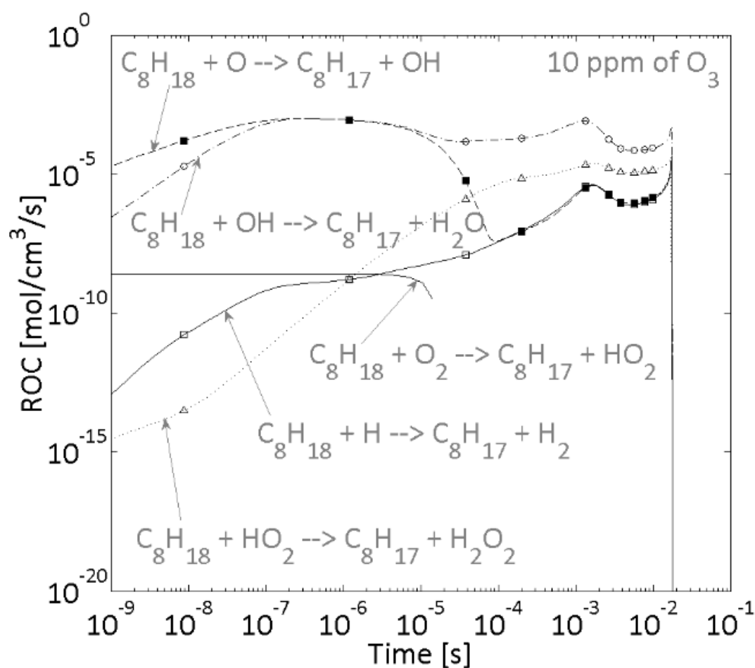
Figure 58. D. Reaction pathway analysis from rates of consumption for isooctane (PRF100) at an initial temperature of 800 K, initial pressure of 50 bar, an equivalence ratio of 0.3 and with 10 ppm of ozone.
