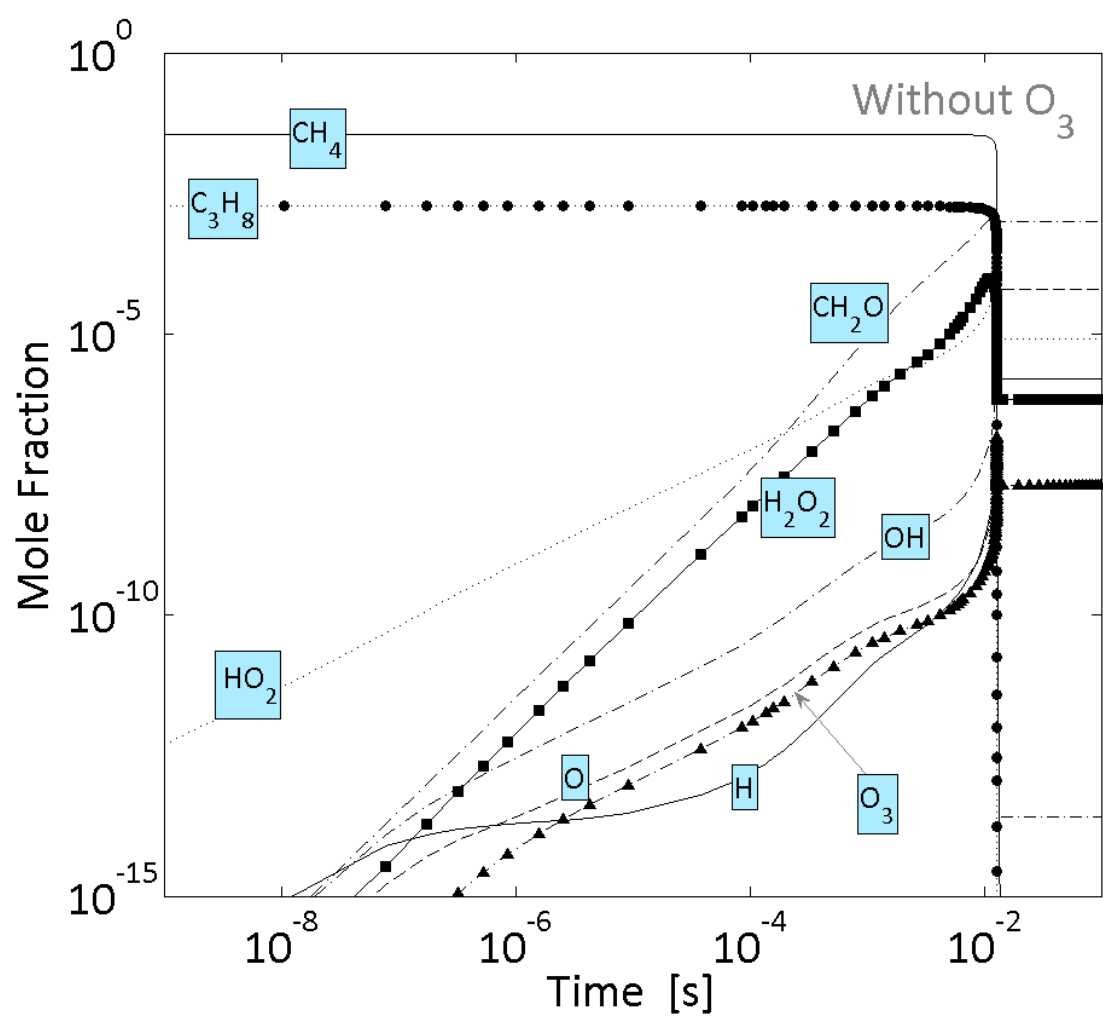
Figure 101. A. Mole fractions for a mixture of methane and propane (95/5) without ozone.
