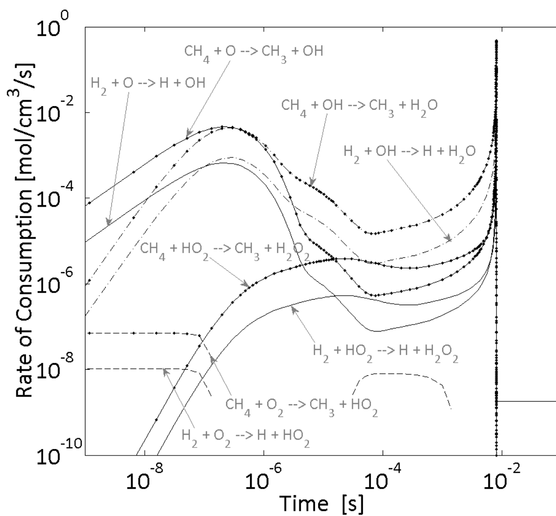
Figure 108. D. Rate of consumption for a mixture of methane and hydrogen (80/20) with 10 ppm of ozone.
