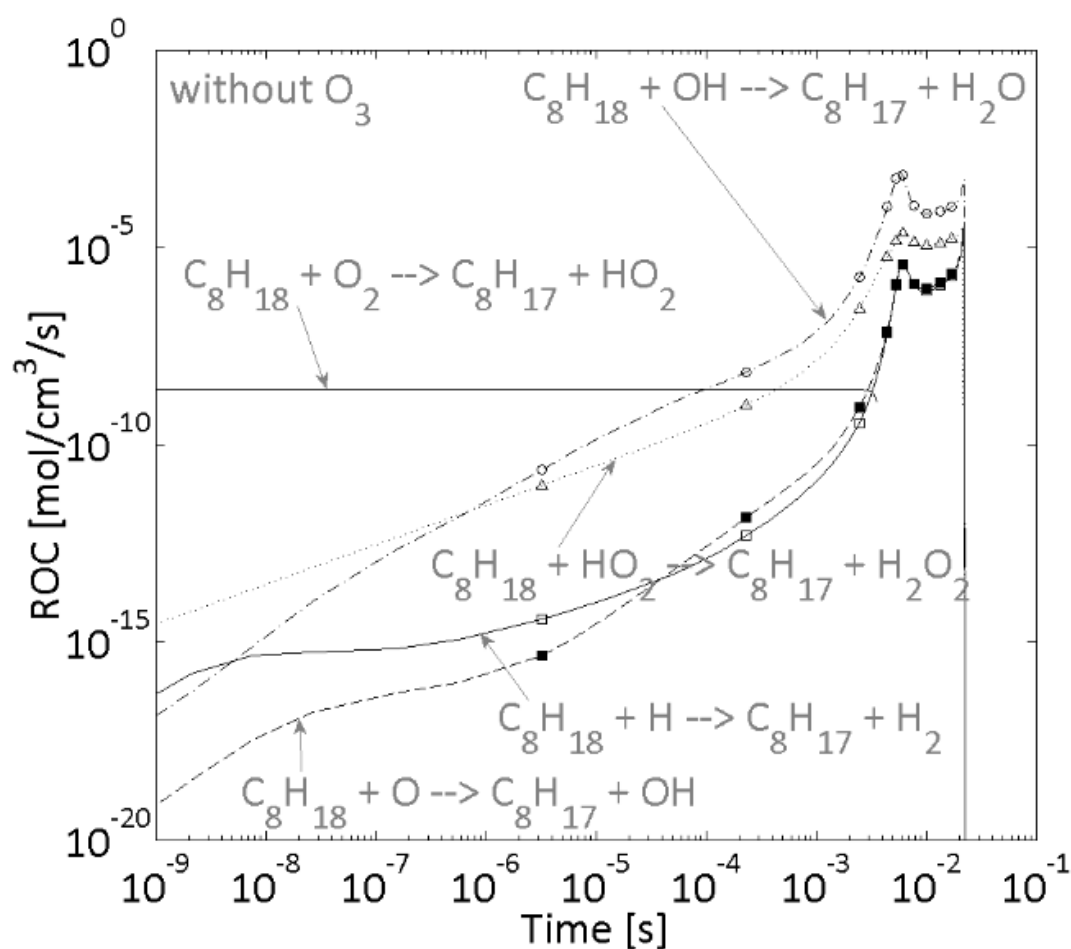
Figure 58. B. Reaction pathway analysis from rates of consumption for isooctane (PRF100) at an initial temperature of 800 K, initial pressure of 50 bar, an equivalence ratio of 0.3 and without ozone.
