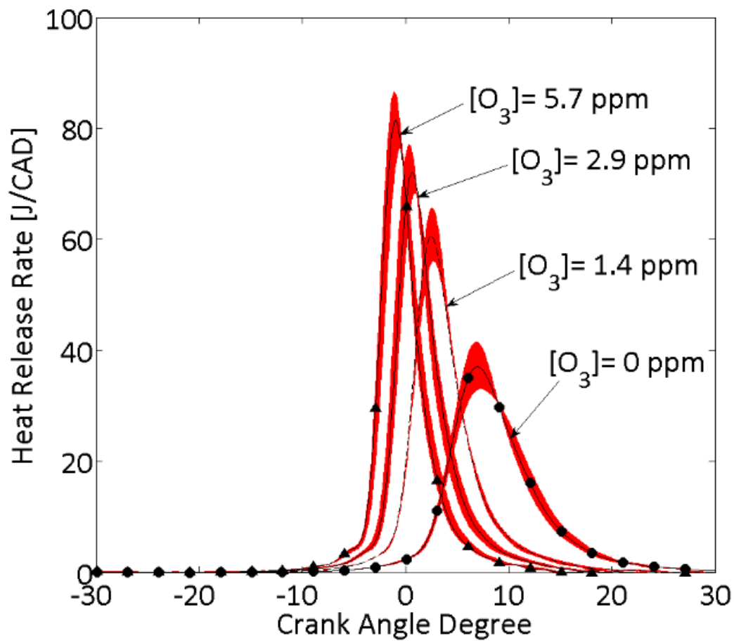
Figure 51. D. Heat release rate evolutions as a function of the ozone concentration injected in the intake of the engine for isooctane/PRF100 as fuel.
