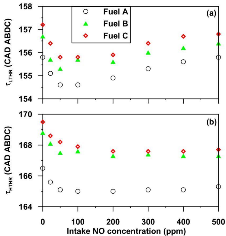
Figure 33. Impact of NO on ignition timings for the cool flame (on the top) and for the main flame (on the bottom) [33]. For three fuels: Fuel A: n -heptane, Fuel B: PRF25 75% n -heptane and 25% isooctane; Fuel C: TRF24 80% n -heptane and 20% toluene.
