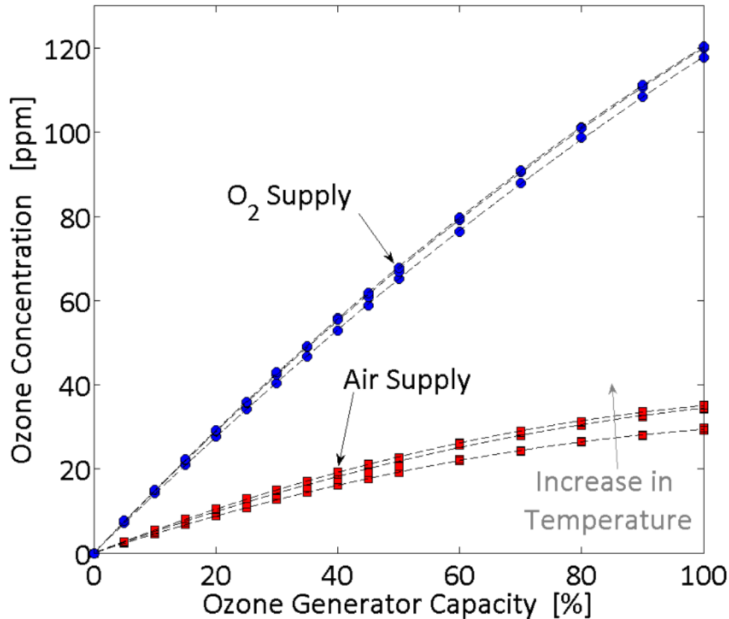
Figure 76. Calibration of the ozone concentration measured at the intake of the engine as a function of the gas supply (pure oxygen and air) and for three different intake temperatures (100 °C, 150 °C and 200 °C).
