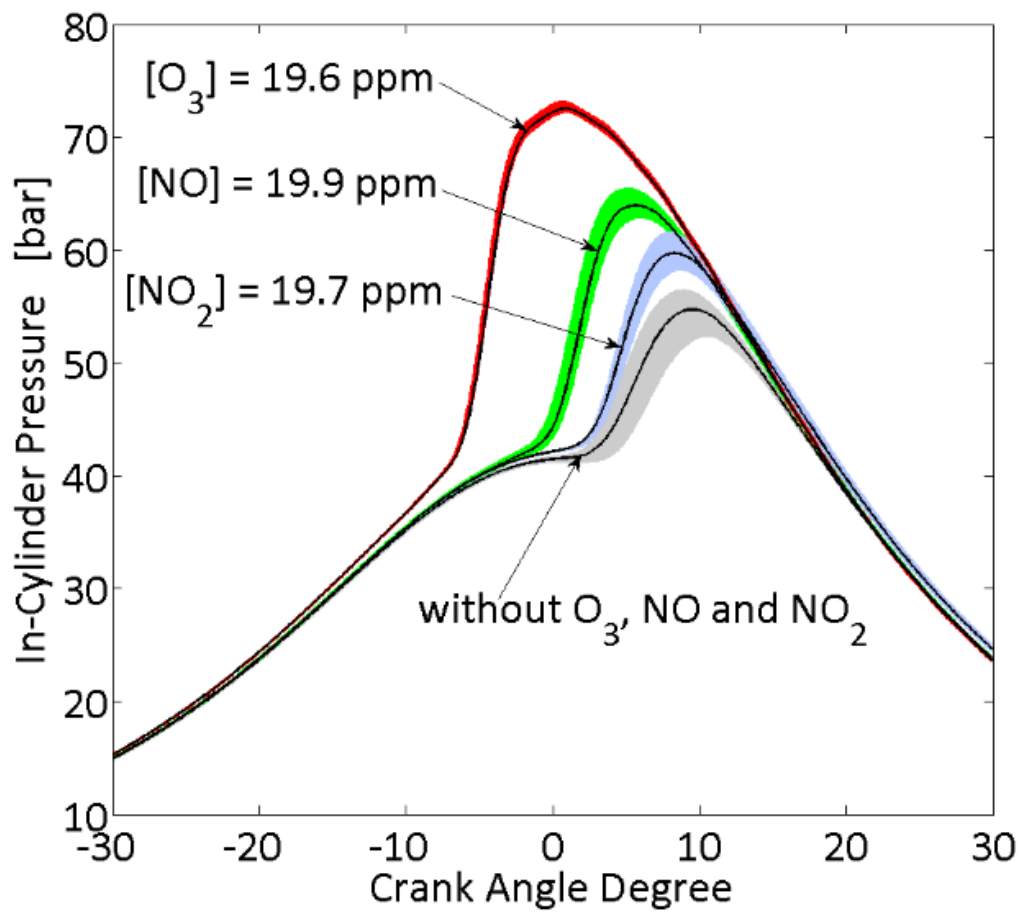
Figure 64. A. In-cylinder pressure traces without any species seeded and with 20 ppm of each oxidizing chemical species ( O_3 : ozone, NO : nitric oxide and NO_2 : nitrogen dioxide) separately injected.
