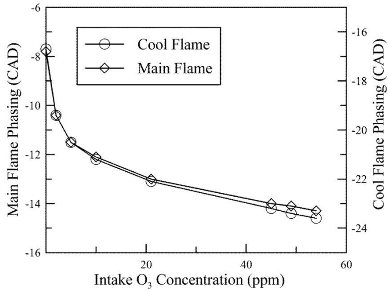
Figure 35. Cool and main flame phasing as a function of the ozone concentration seeded in the intake of an HCCI engine [9].
