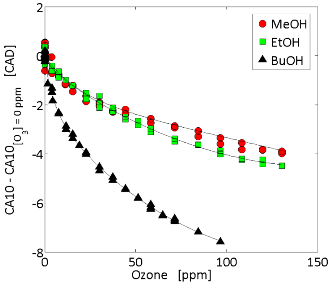
Figure 111. Effect of ozone on the shift of the CA10 with respect to the CA10 without ozone for the three alcohol fuels selected. Symbols represent the experiments and dashed lines the trends.
