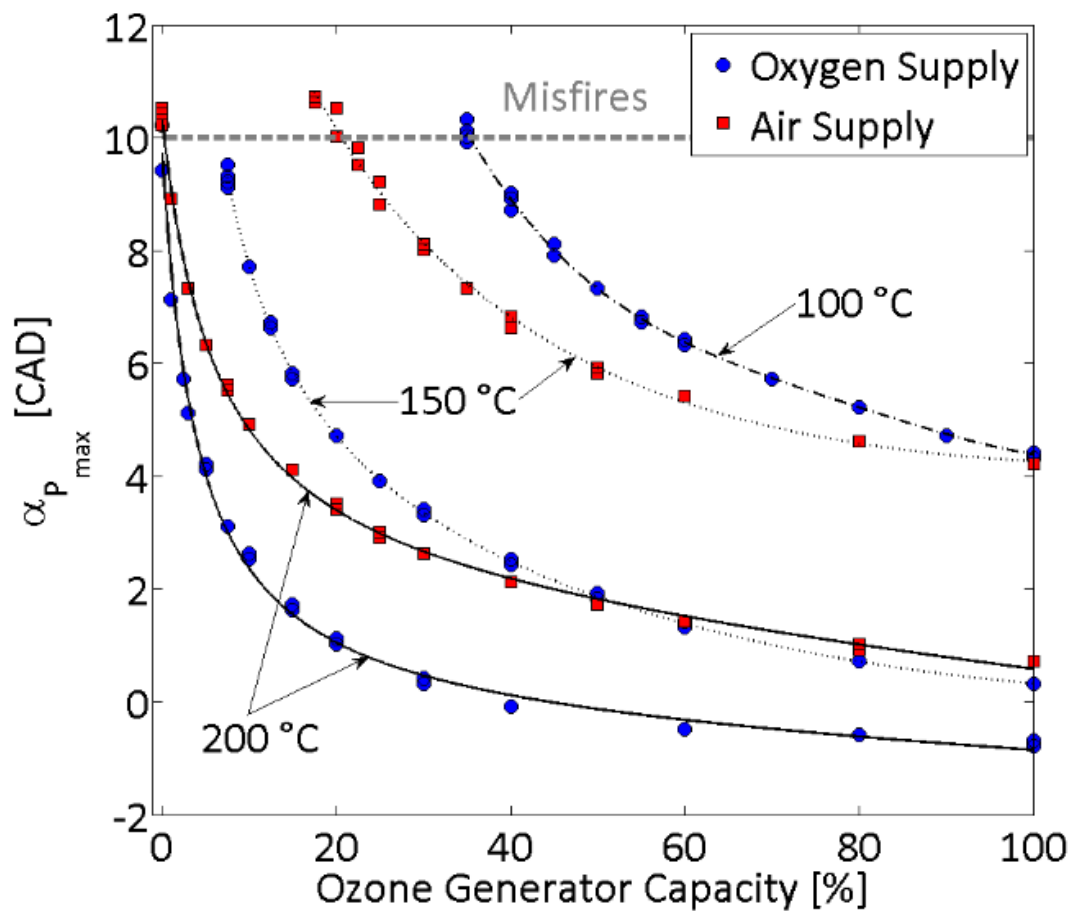
Figure 77. A. Phasing of the maximum pressure location as a function of the ozone generator capacity for an oxygen supply and an air supply
