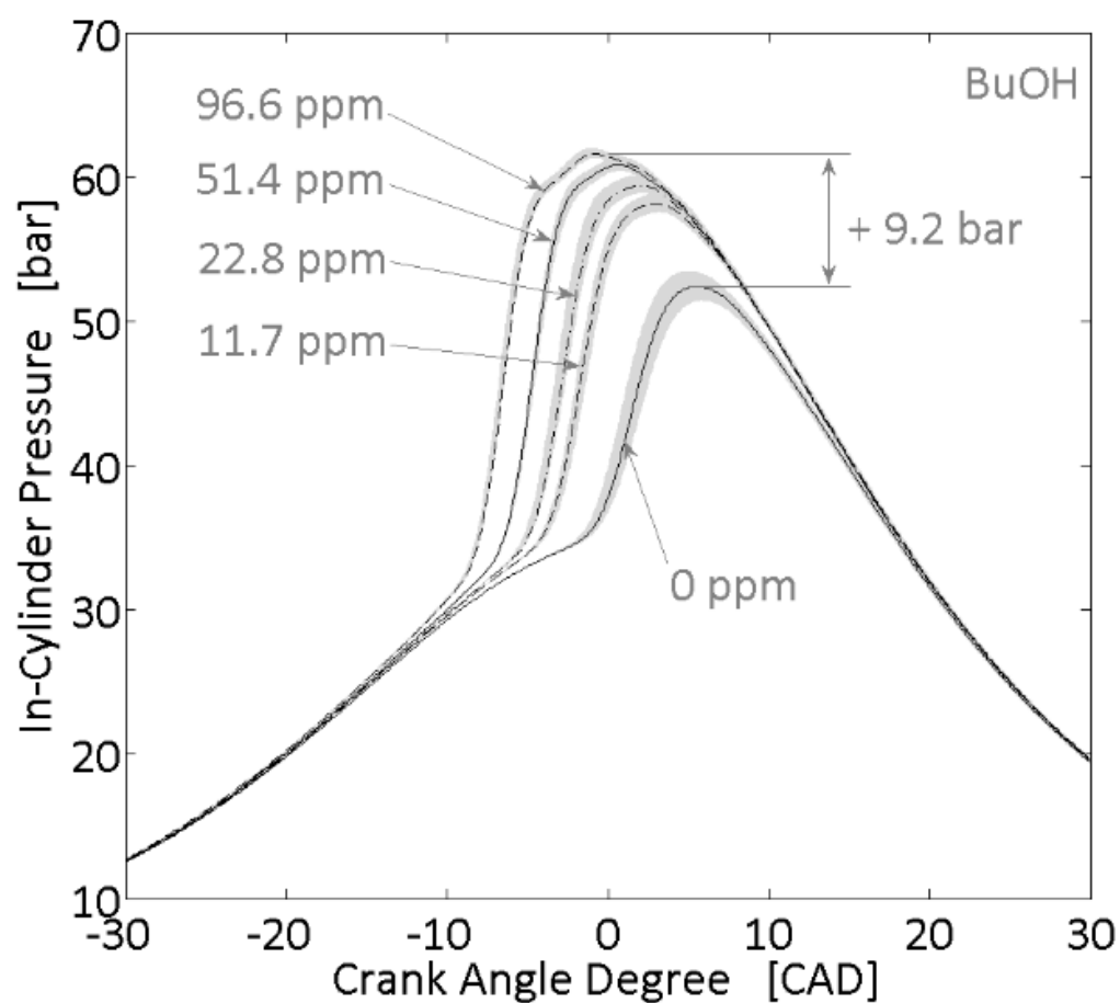
Figure 110. E. In-cylinder pressure traces as a function of the ozone seeded for BuOH as fuel. Black curves correspond to the average of 100 cycles recorded and gray areas represent the variation of the same 100 cycles (the upper and the lower limits obtained).
