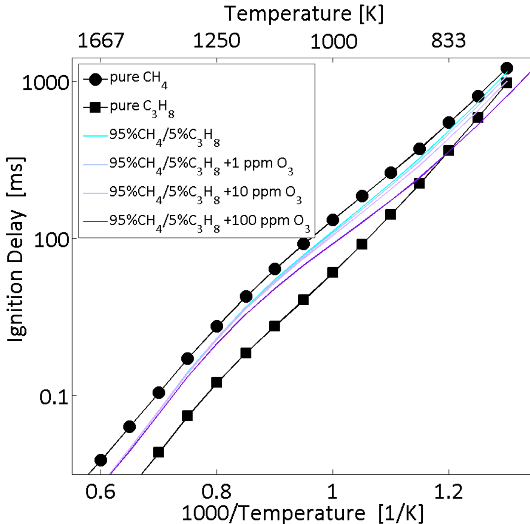
Figure 100. Ignition delays as a function of the inverse temperature of pure methane, pure propane and a mixture of both fuels without ozone and with mole fraction of 1, 10 and 100 ppm of ozone.
