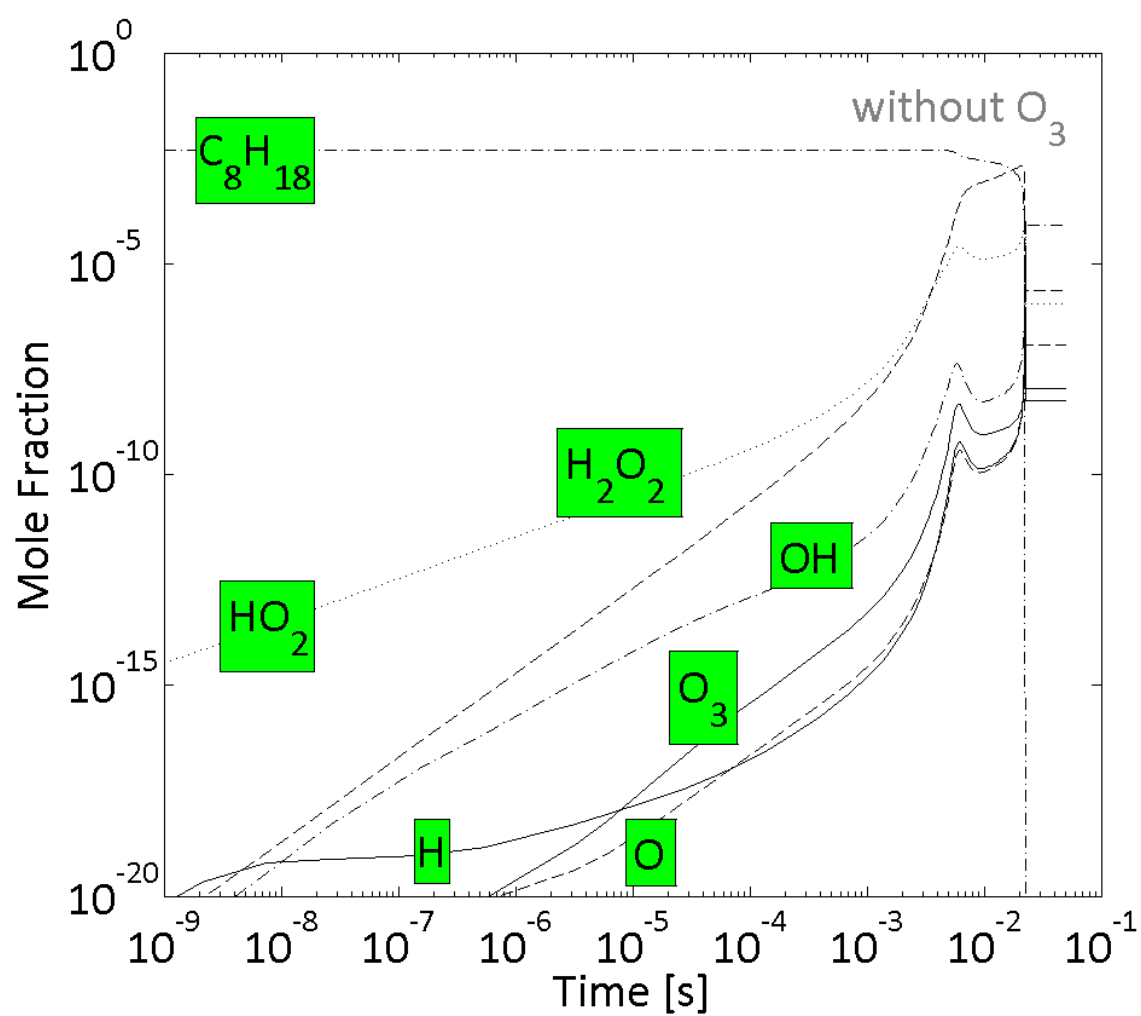
Figure 58. A. Mole fractions of the main radicals and the fuel for isooctane (PRF100) at an initial temperature of 800 K, initial pressure of 50 bar, an equivalence ratio of 0.3 and without ozone.
