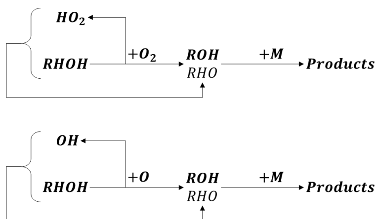
Figure 118. Summary of the alcohol fuels oxidation without ozone (on the top) and with ozone seeding (on the bottom).
