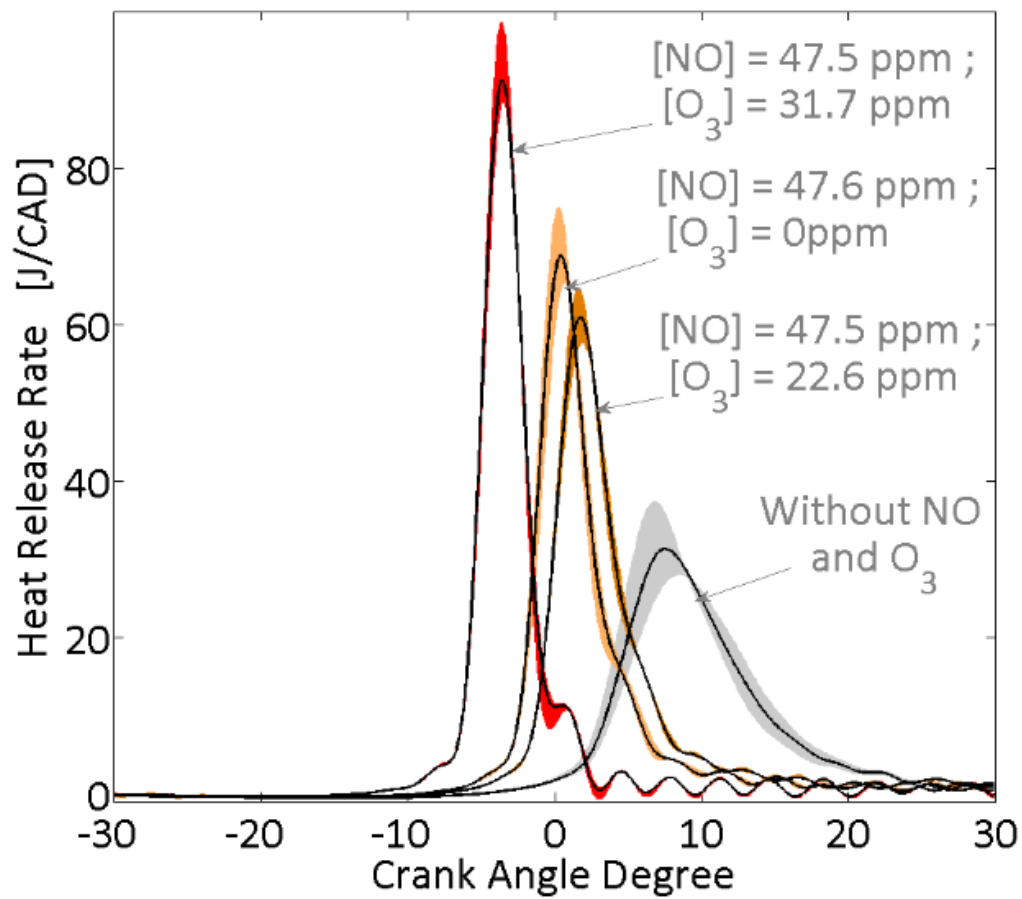
Figure 68. B. Heat release rate traces as a function of the crank angle degree for several couple of concentration in ozone and nitric oxide simultaneously seeded in the intake of the engine.
