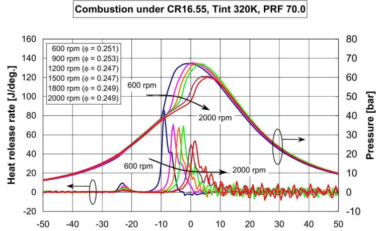
Figure 25. In-cylinder pressure and heat release rate traces as a function of the rotation speed for PRF70 as fuel and an equivalence around 0.25 [78].
