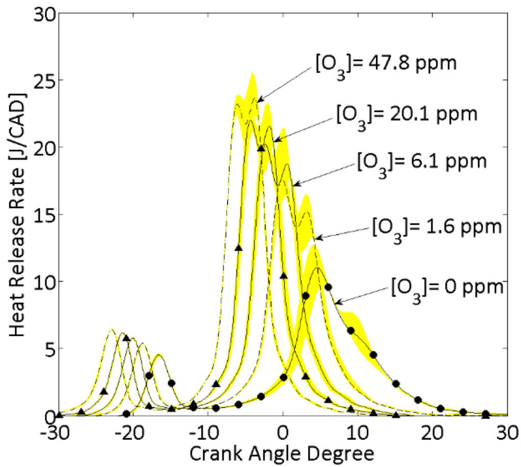
Figure 51. B. Heat release rate evolutions as a function of the ozone concentration injected in the intake of the engine for n-heptane/PRF0 as fuel.
